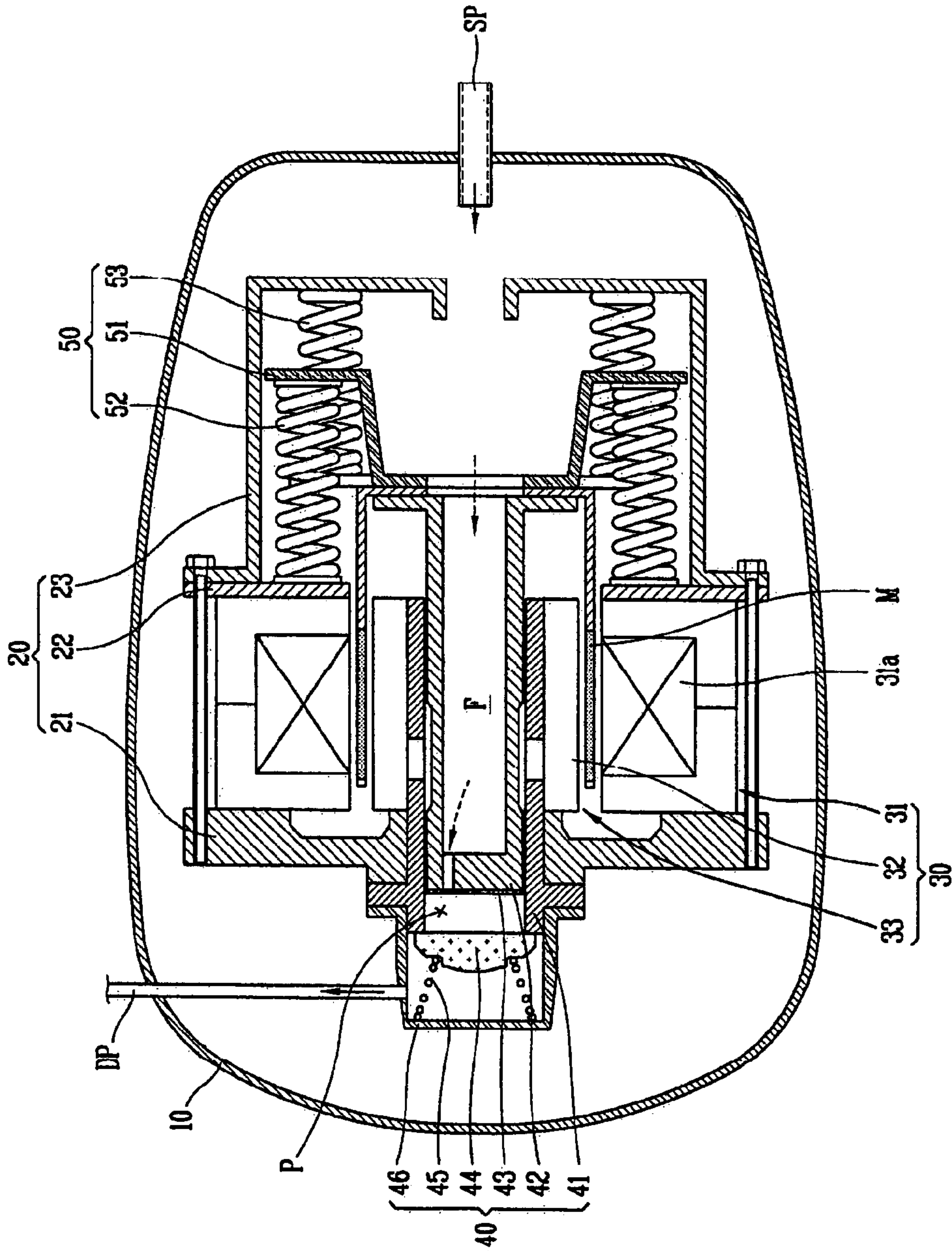
FIG. 1 CONVENTIONAL ART
