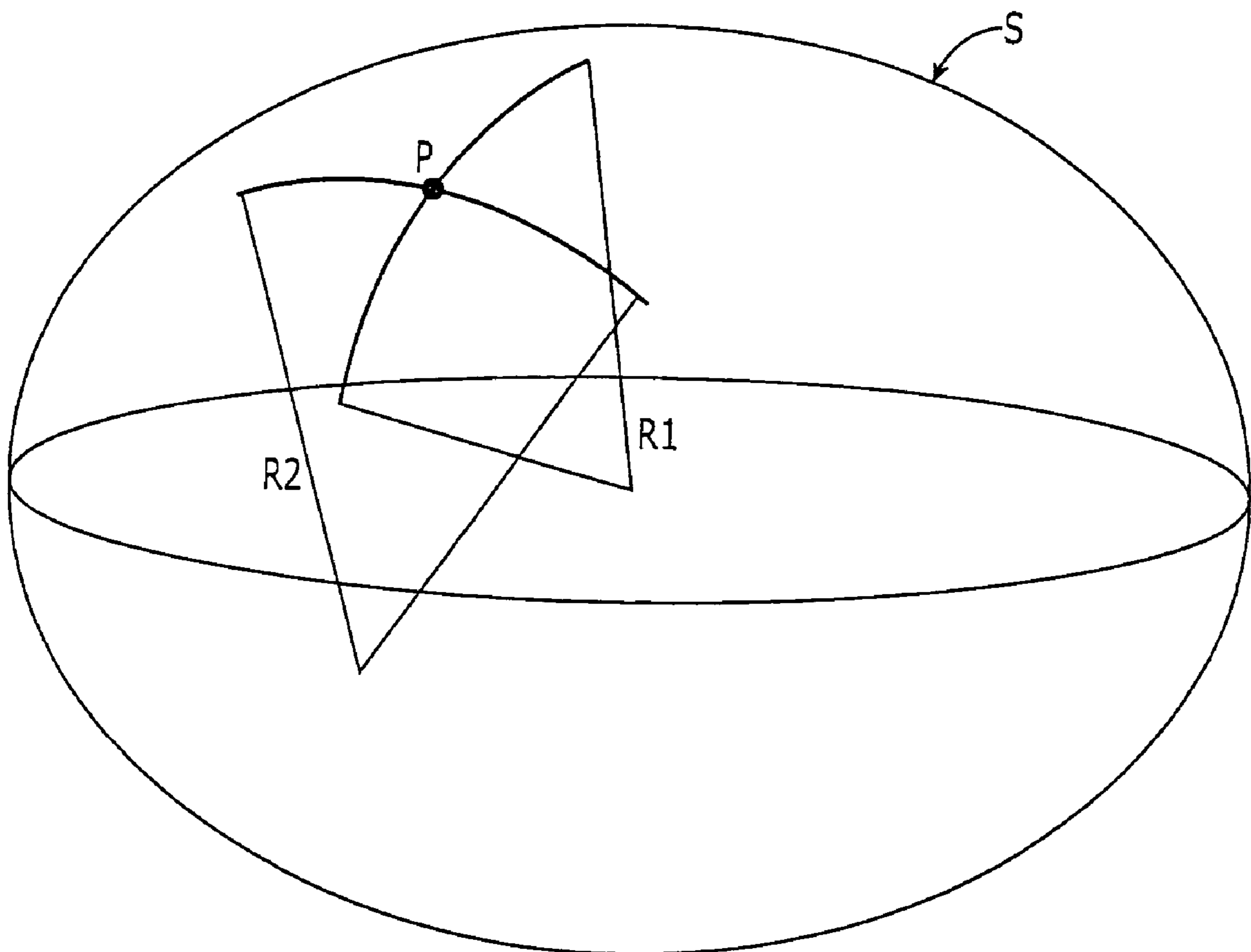
Surface Curvature at a Point
