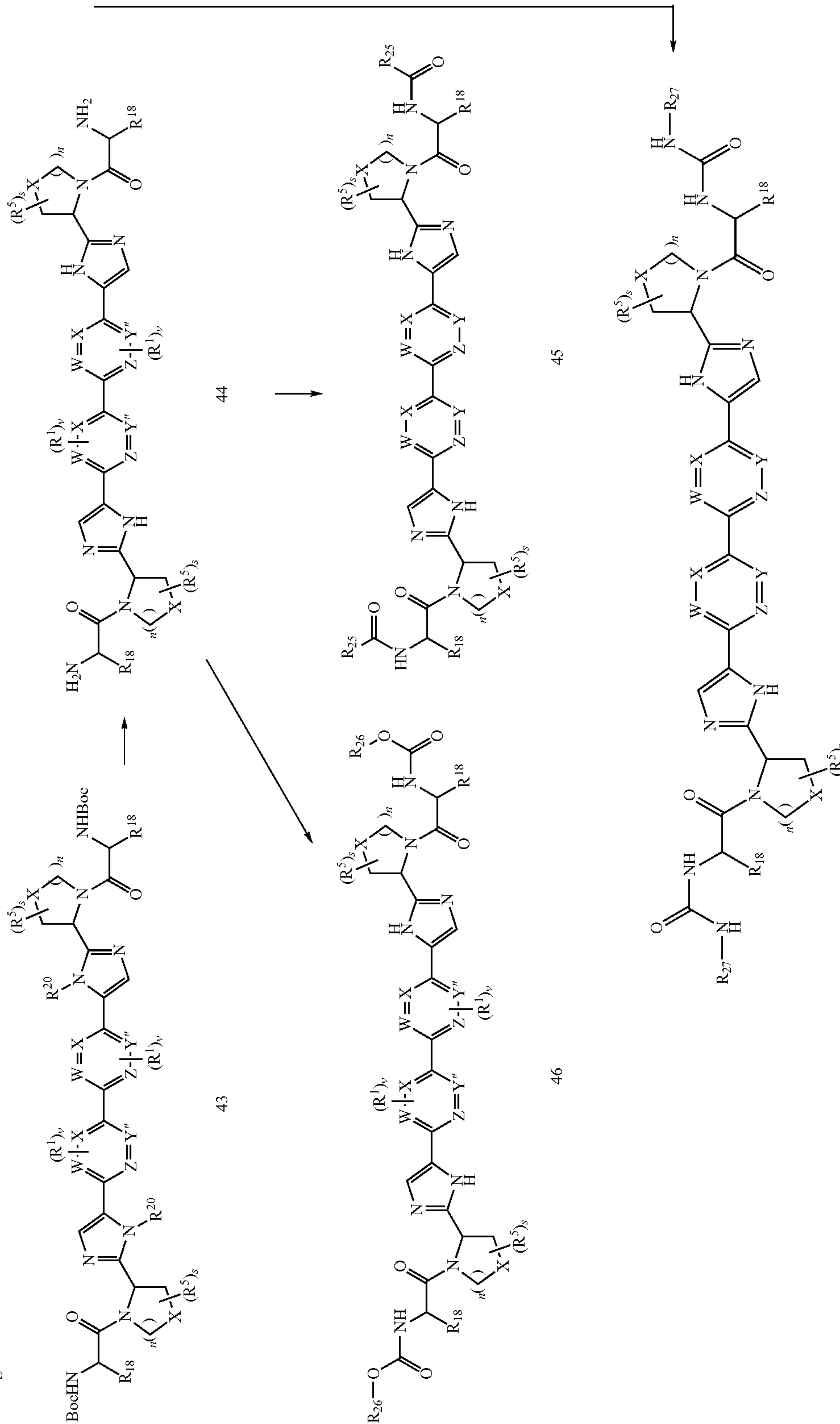
Scheme 10: Starting Material 29
