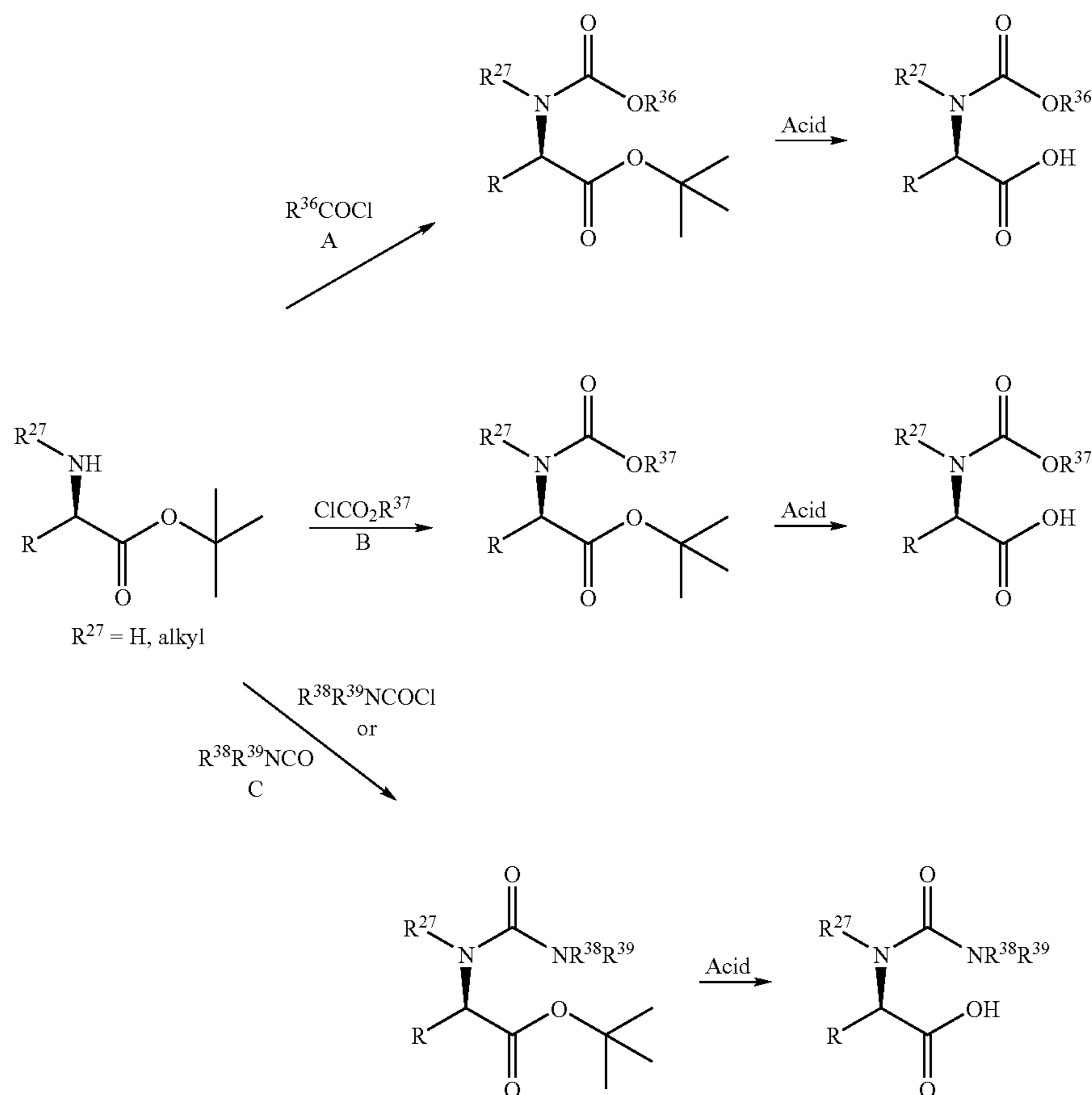
Scheme 13
