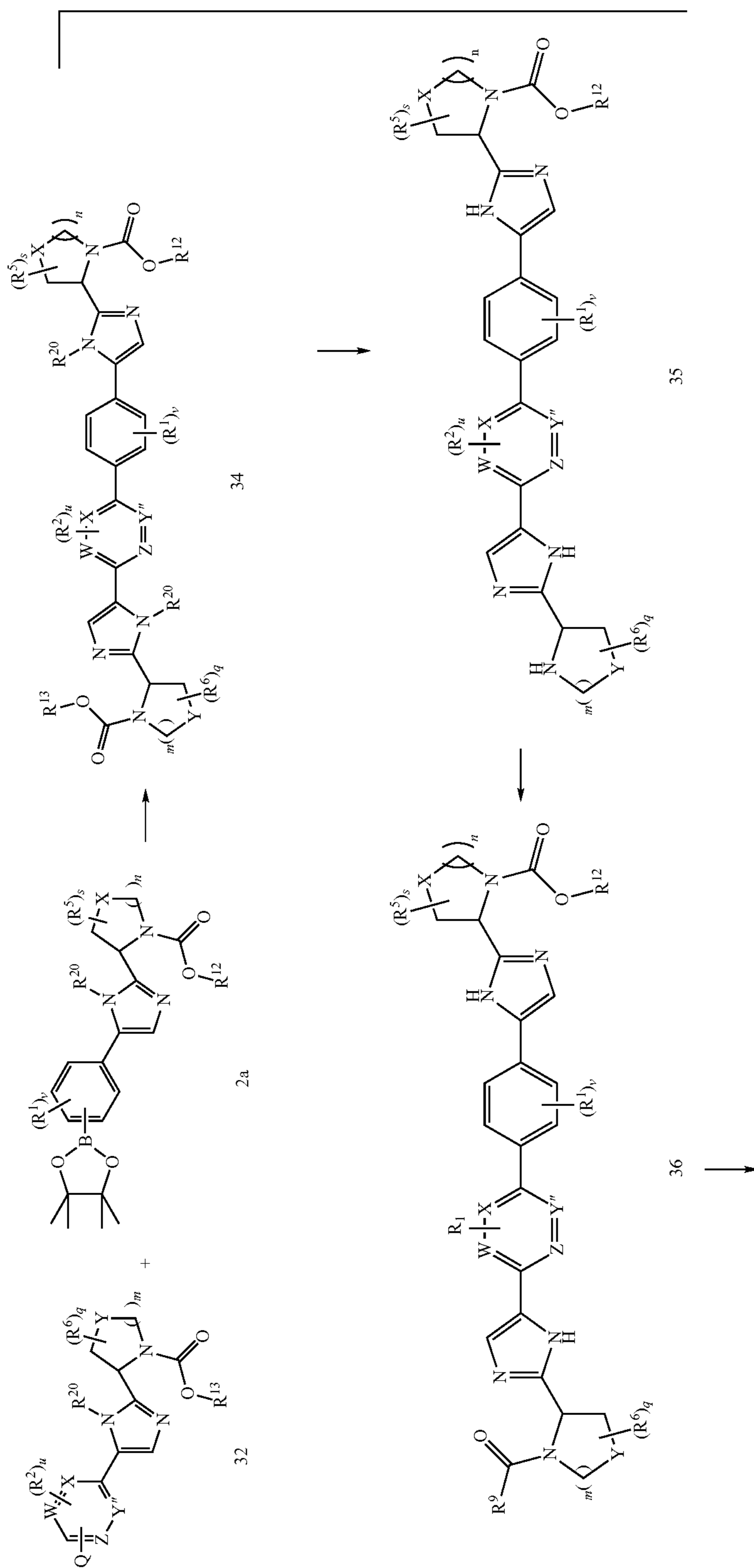
Scheme 8
