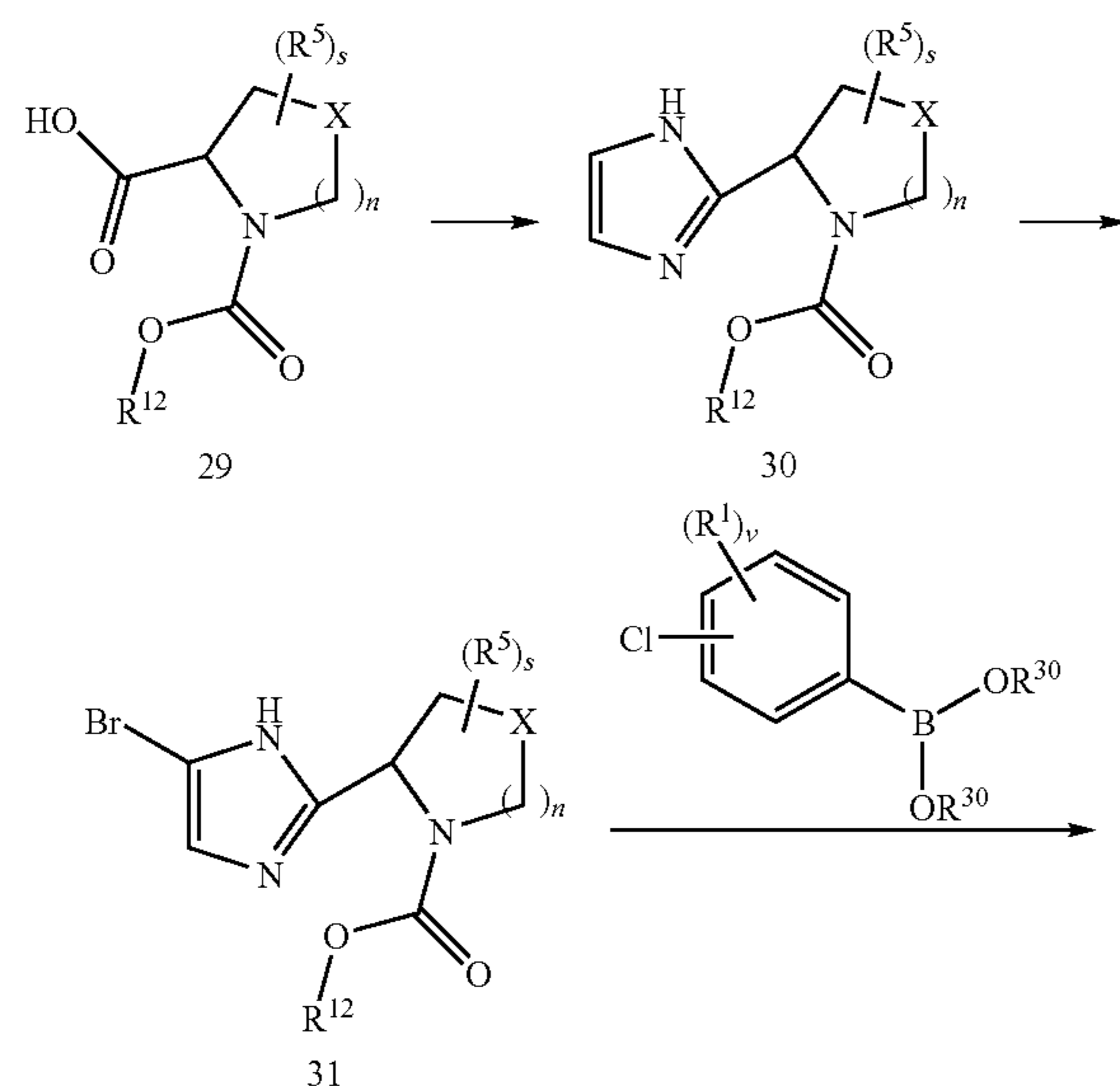
Scheme 7: Heteroaryls
