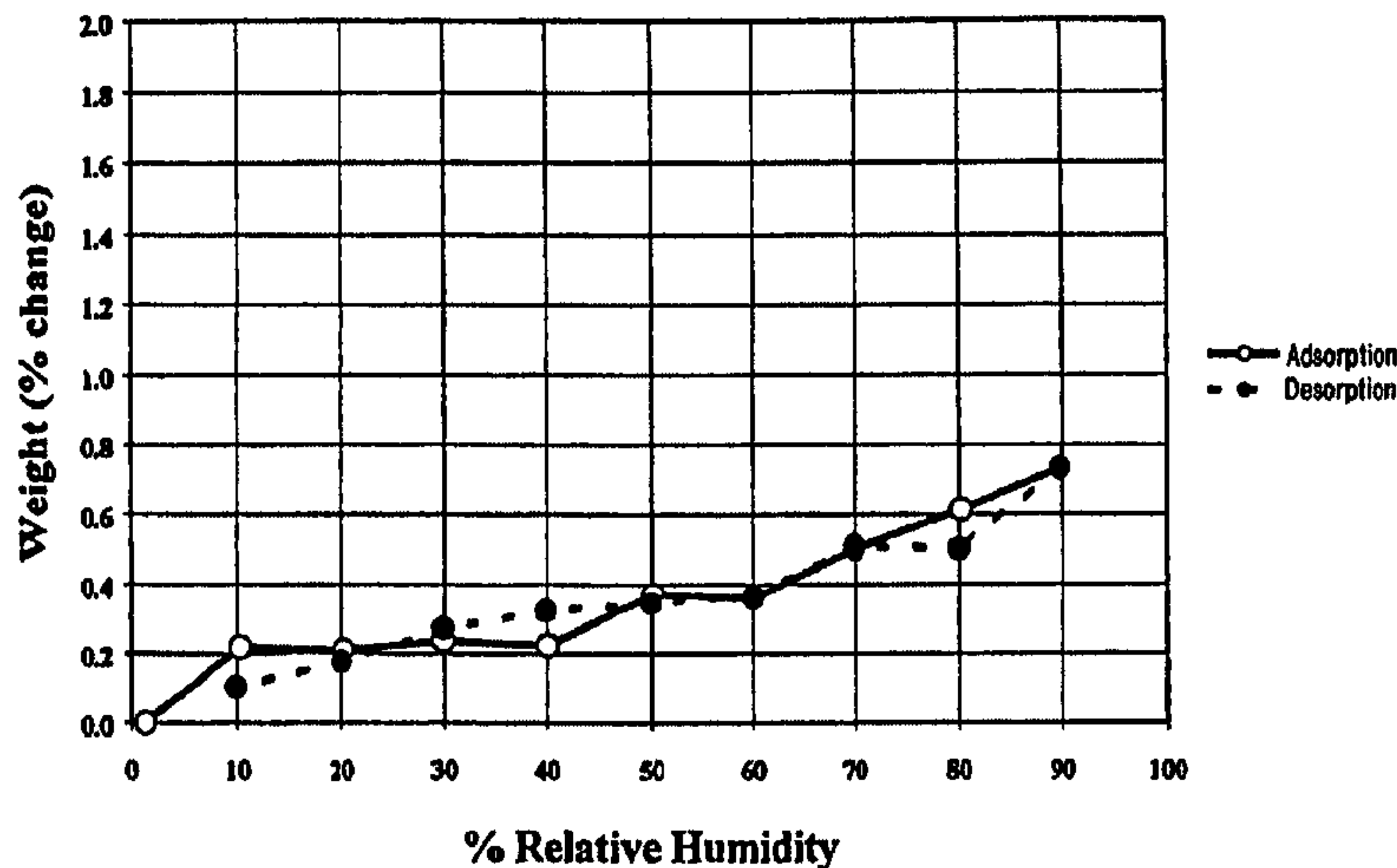
Adsorption/Desorption Isotherm
