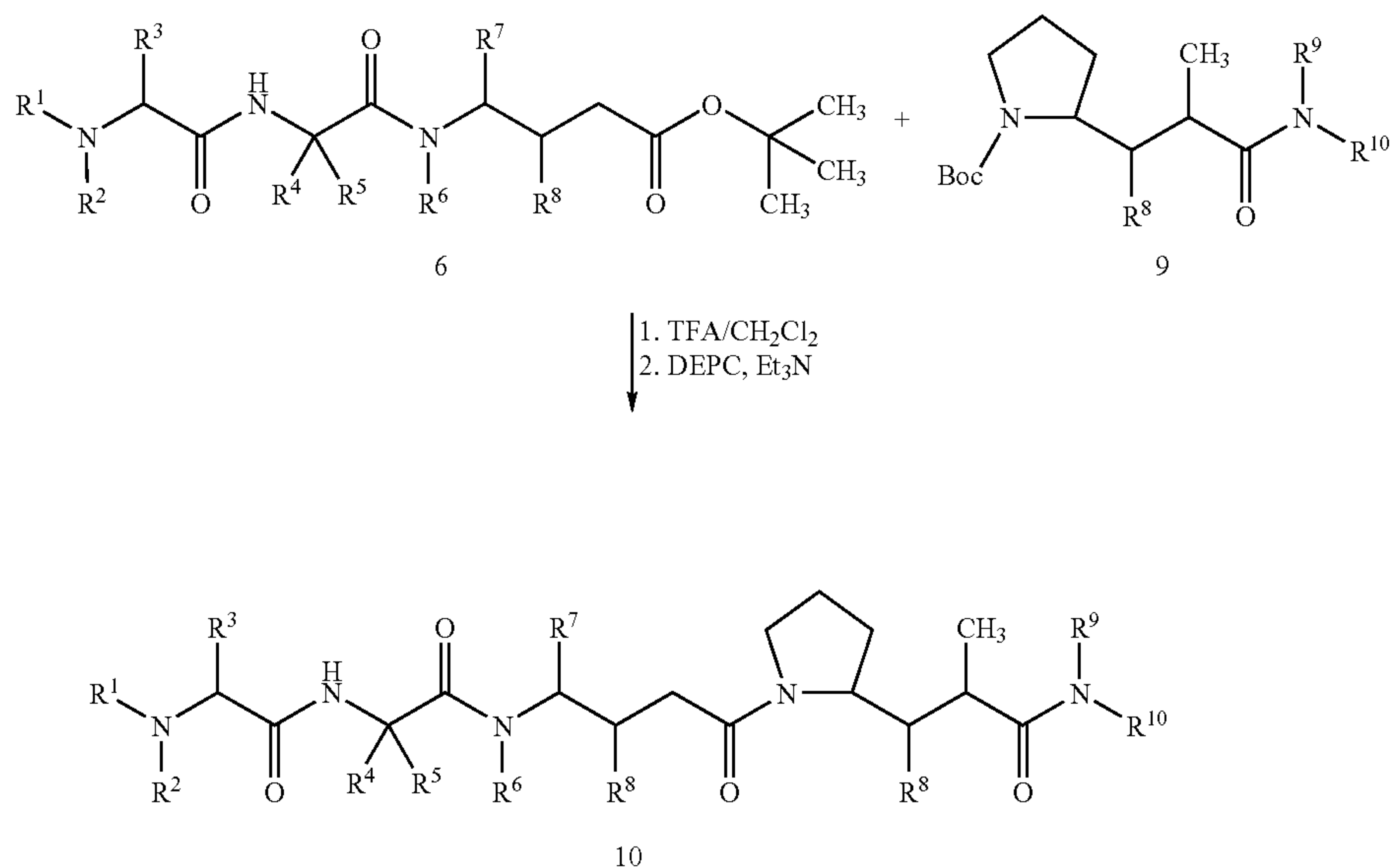
Scheme 7
