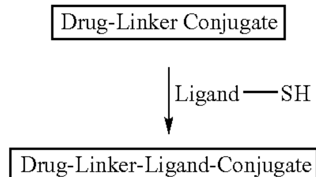
Scheme 17
