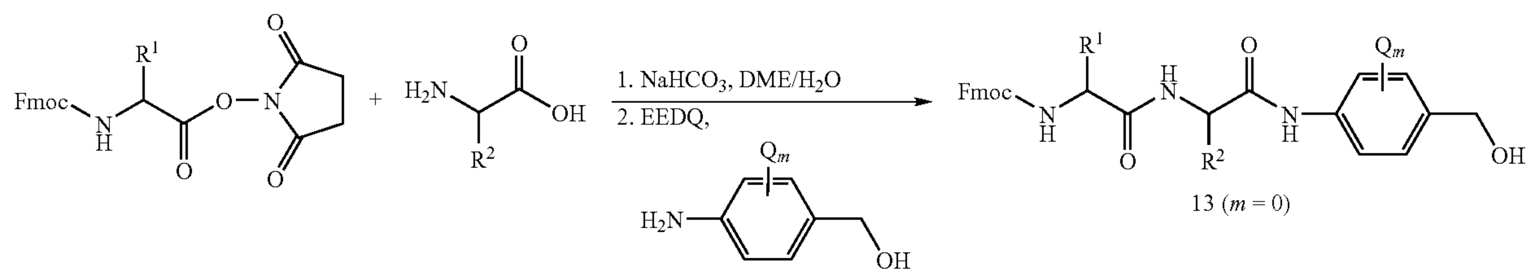
Scheme 10
