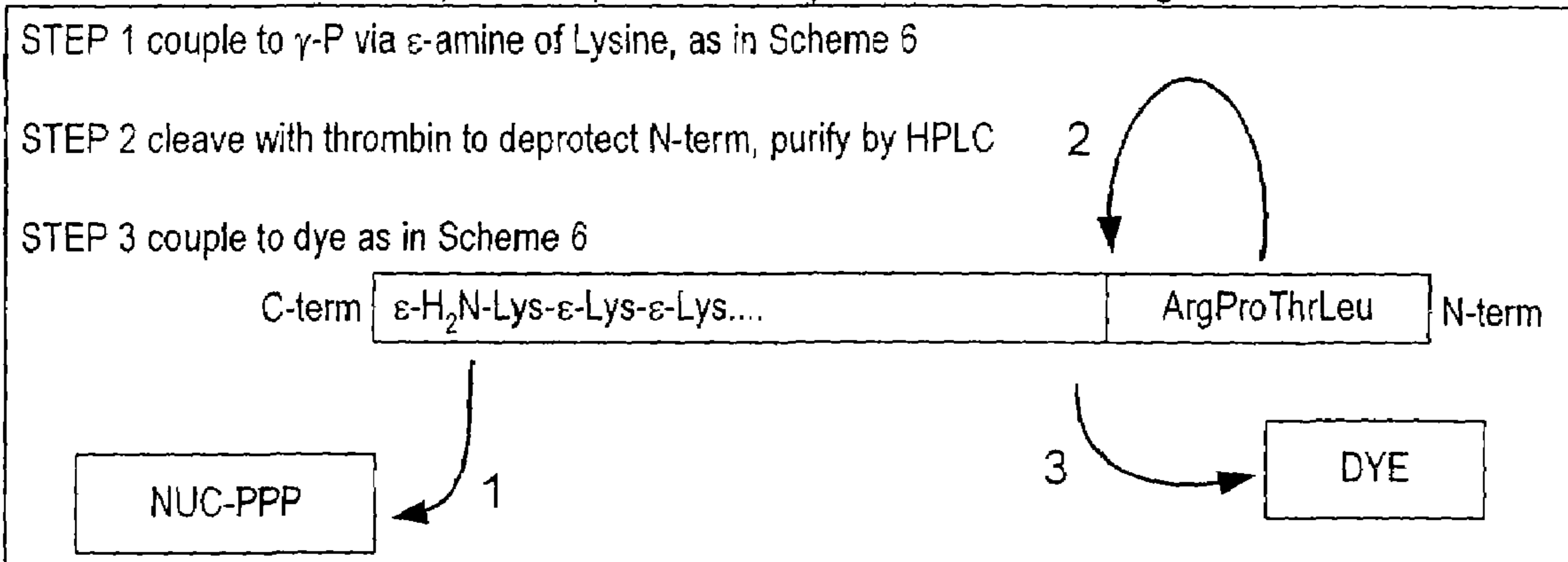
Scheme 8 - Peptide Deprotection By Thrombin Cleavage
