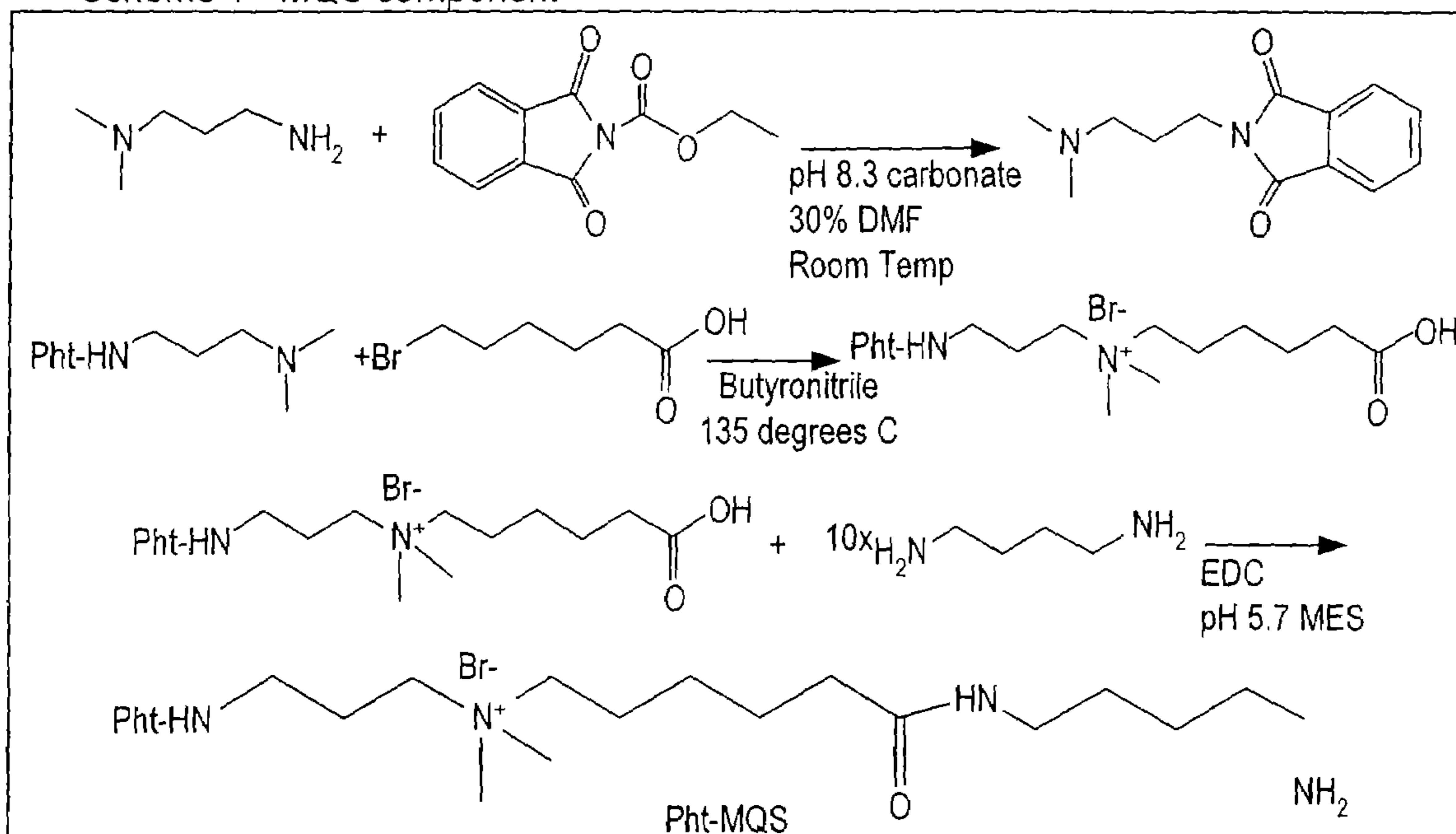
Scheme 2 - BQS linker
