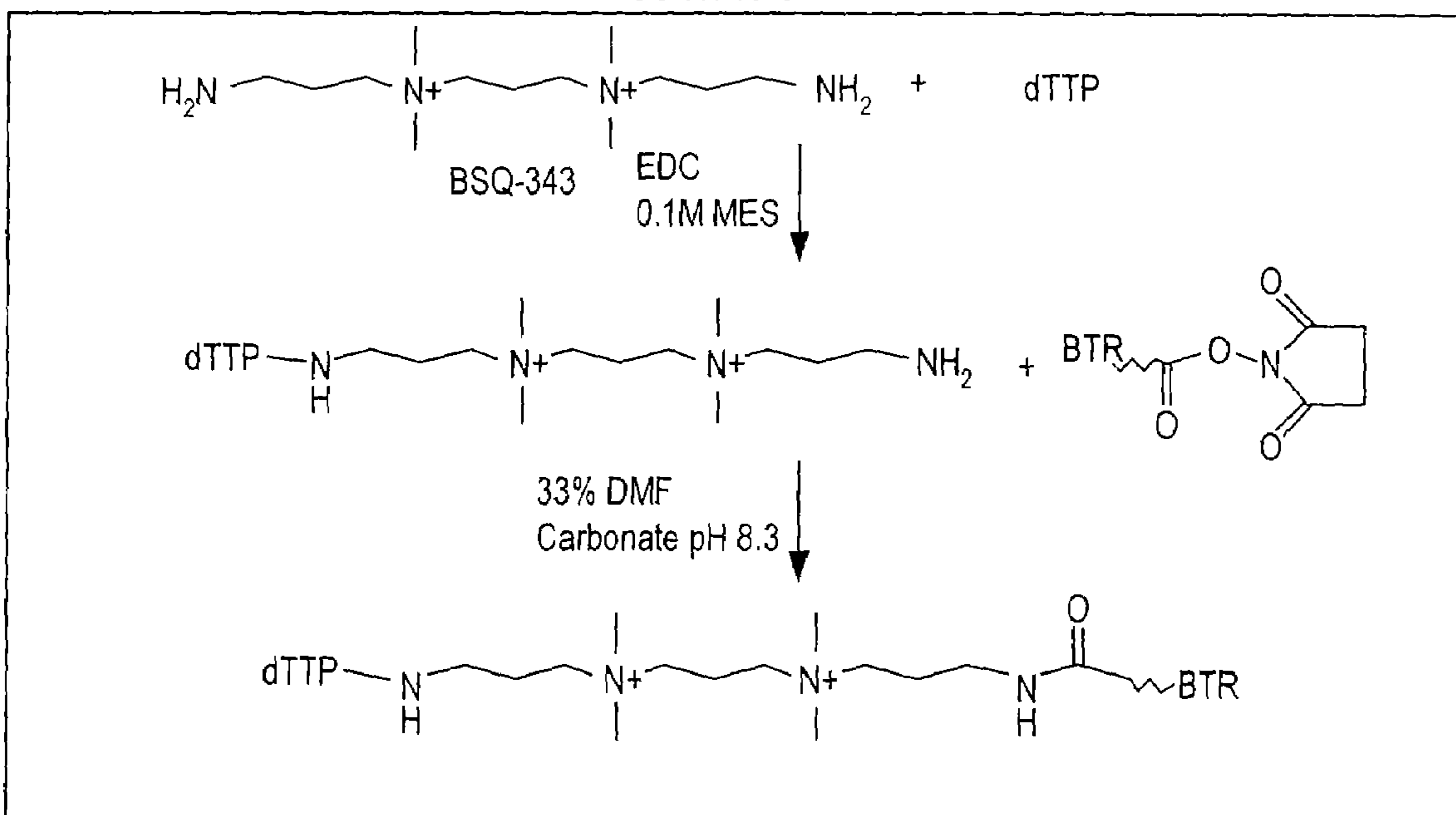
Scheme 6
