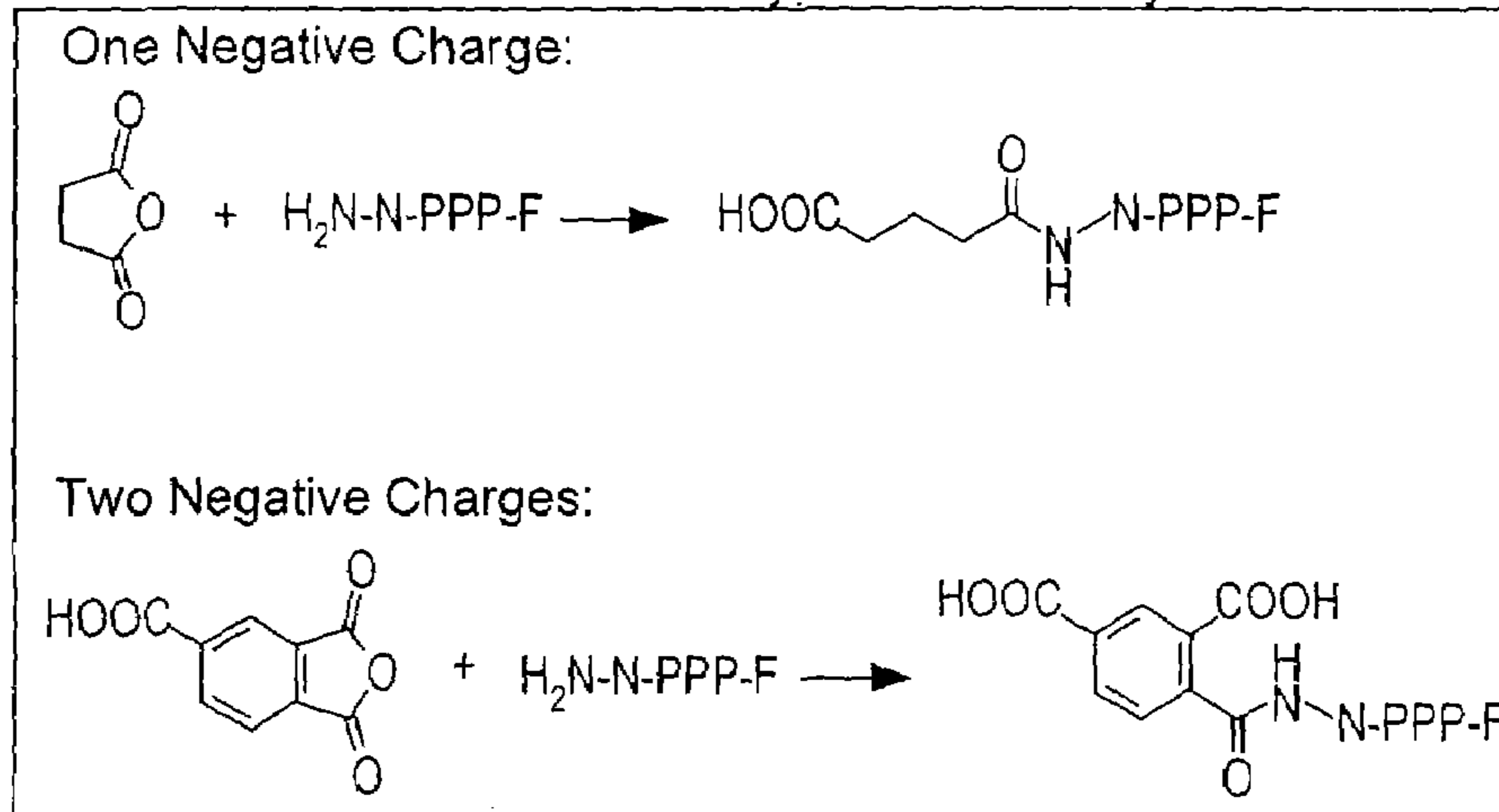
Scheme 10 - g-dNTP With Carboxylated Base
