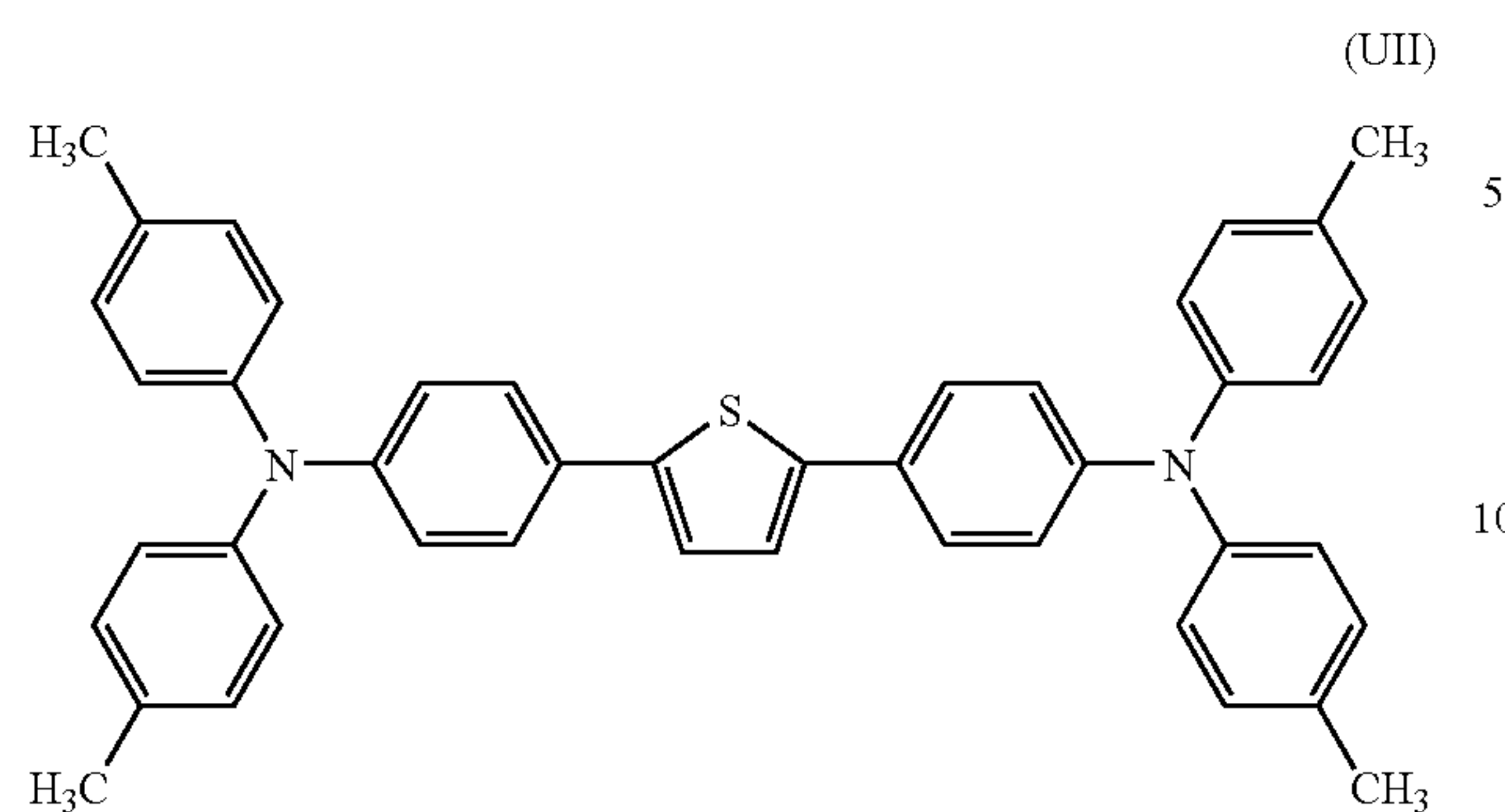
&lt;Compound (VII)&gt;
