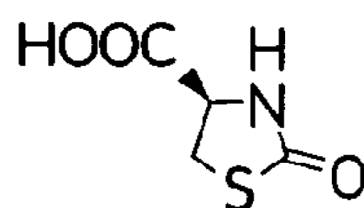
(-)-2-OXO-4-THIAZOLIDINE-CARBOXYLIC ACID
