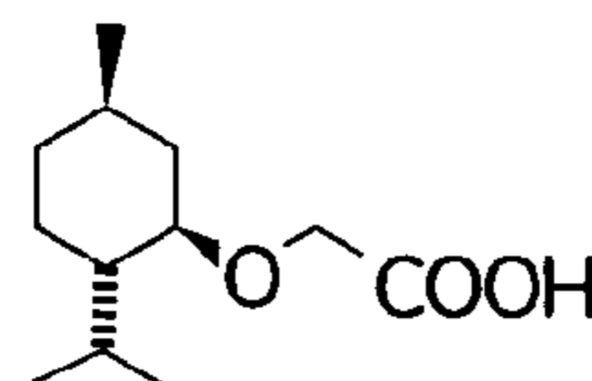
(-)-MENTHOXYACETIC ACID
