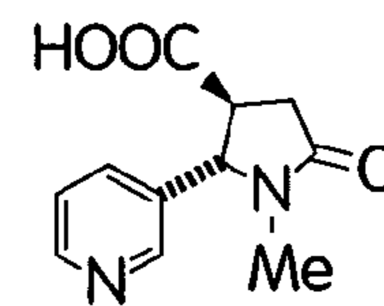
trans-4-COTININECARBOXYLIC ACID
