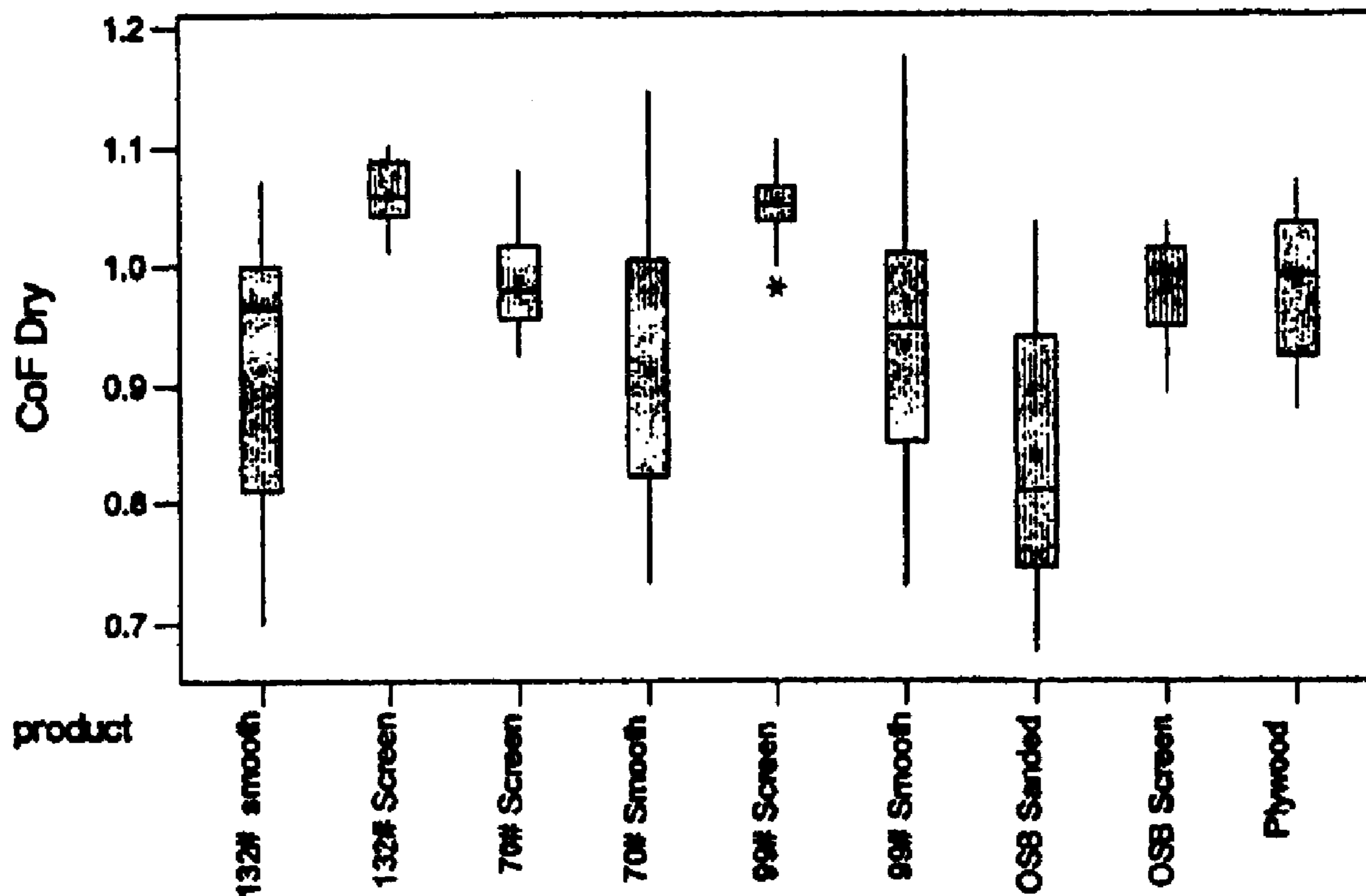
Boxplots of CoF Dry by product (means are indicated by solid circles)
