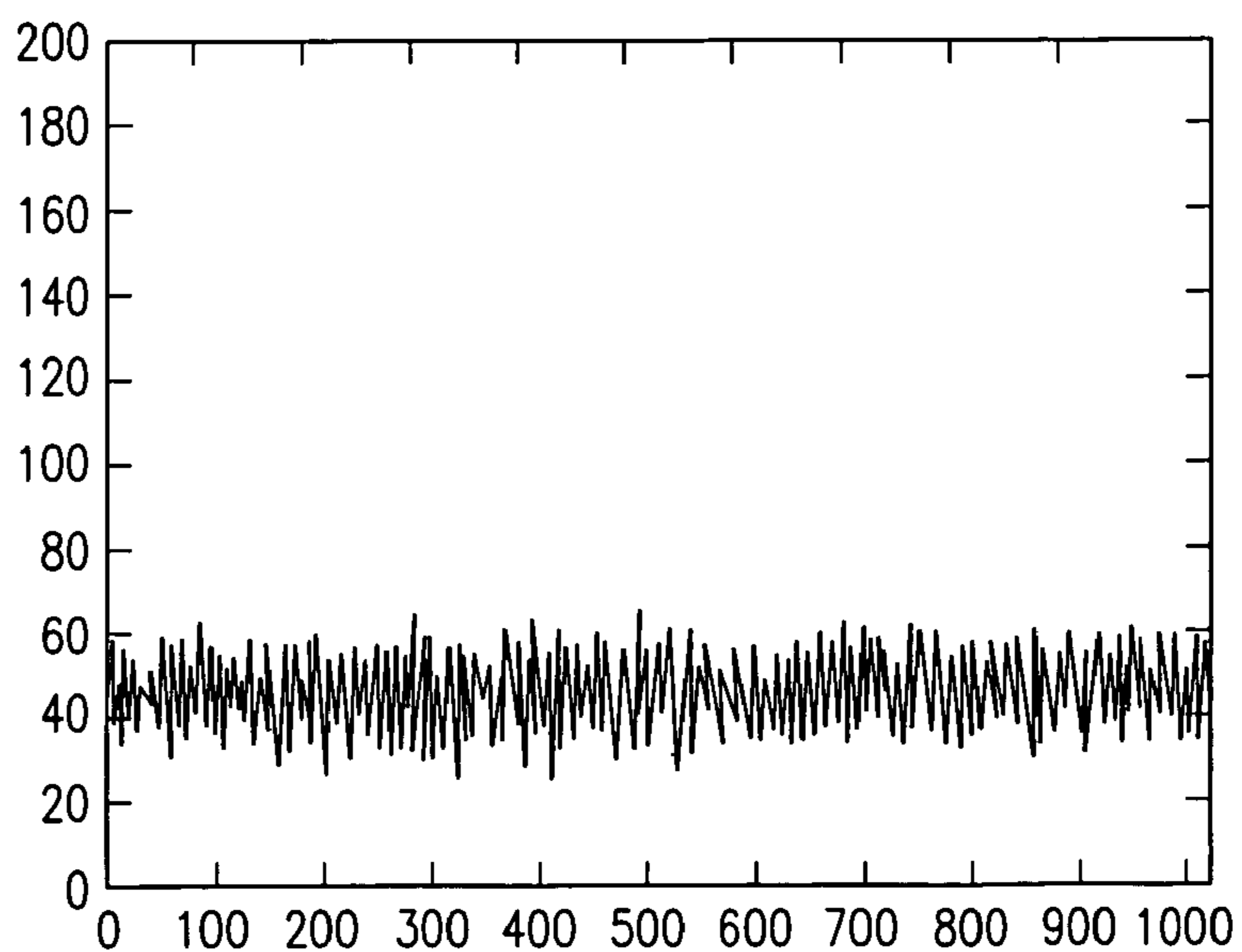
FIG. 10 APERIODIC CROSS-CORRELATION OF THE COMMA FREE CODES
