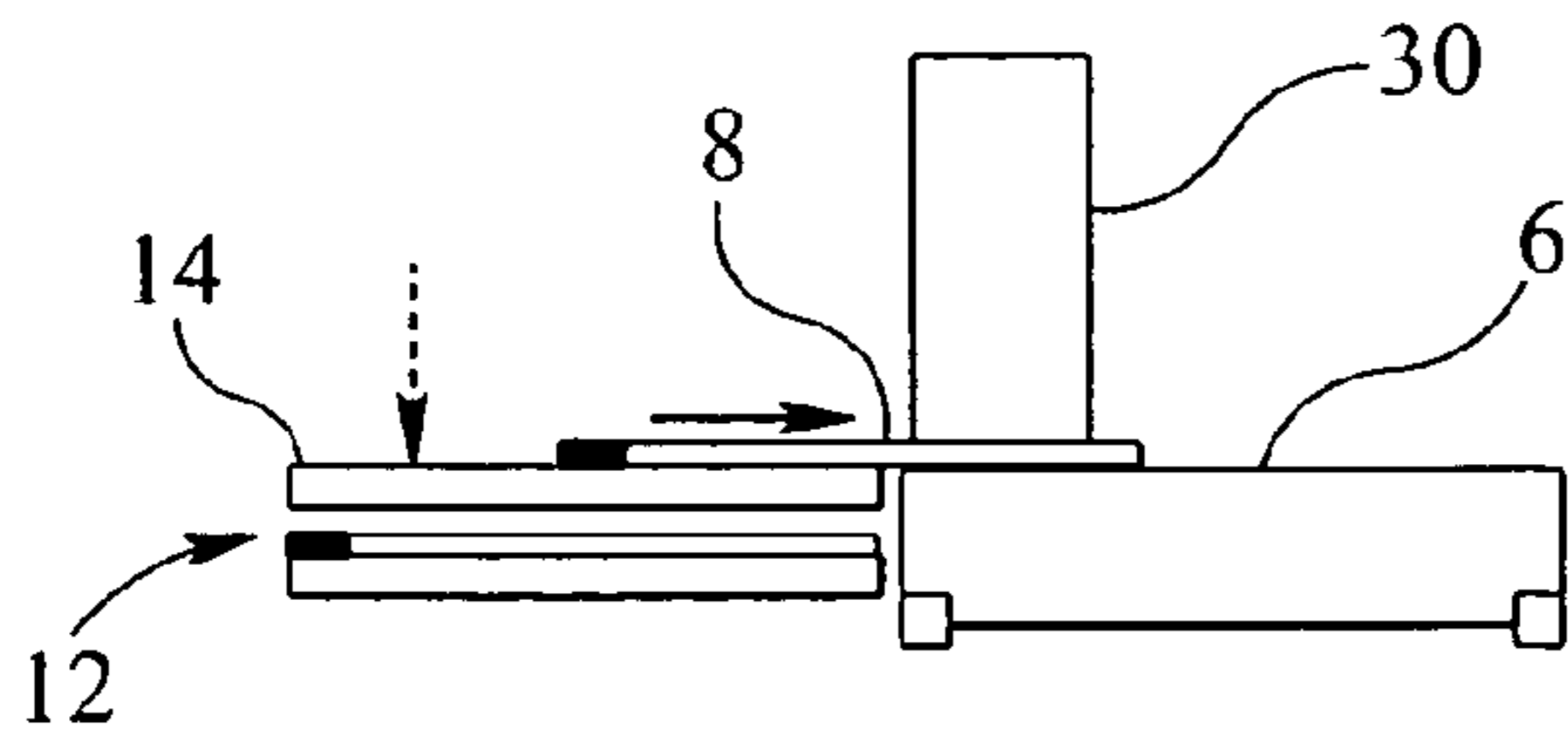
-Stage: receive new substrate -Handler: transport new substrate to stage FIG 10(a)
