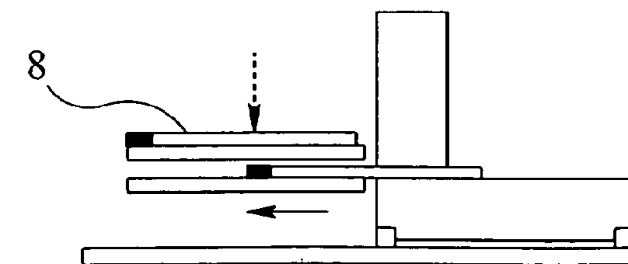
-Stage: exposed substrate to unloader -Handler: transport exposed substrate to unloader FIG 10(h)
