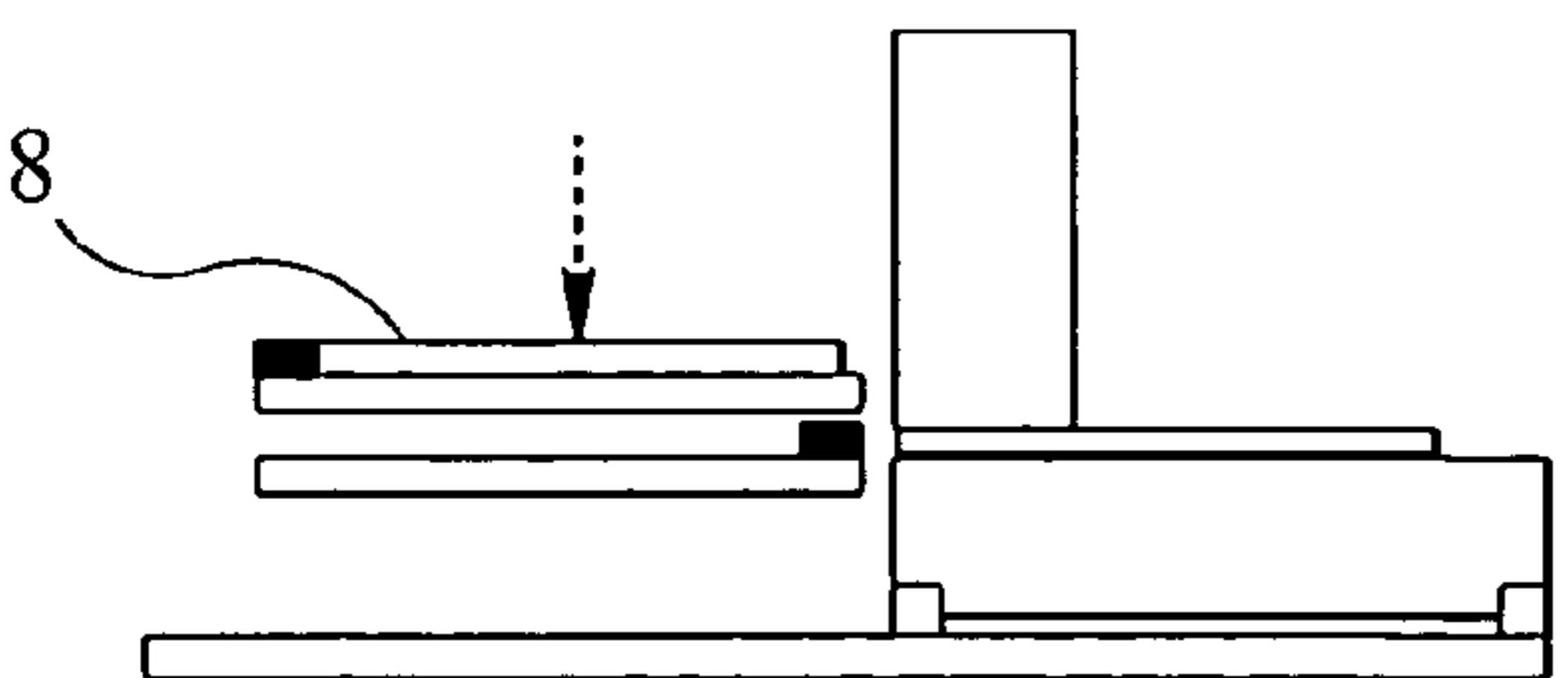
-Stage: Exchange position -Handler: Unload plate to exchange level FIG 10(g)
