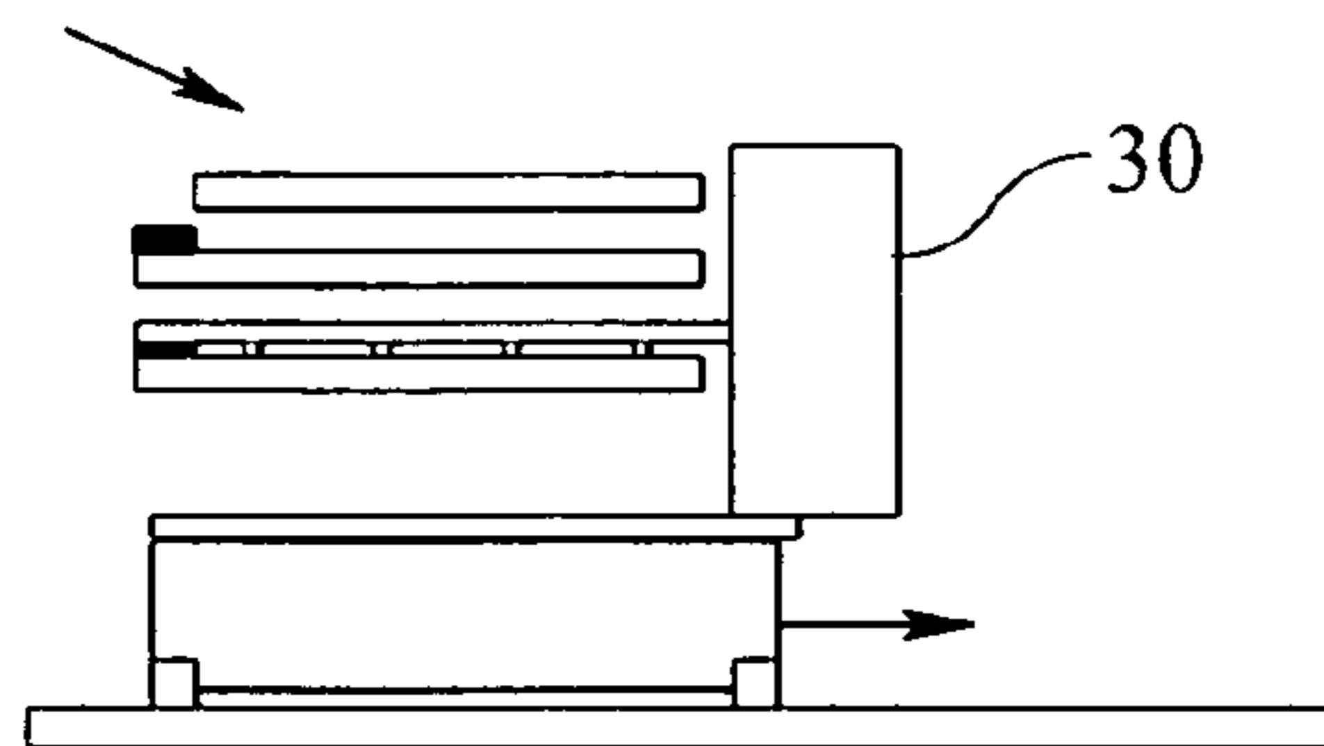
*Stage: start expose substrate *Handler: load new substrate FIG 10(d)
