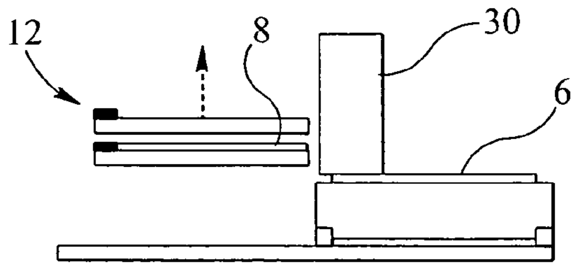
-Stage: wait at exchange position -Handler: move up FIG 10(b)
