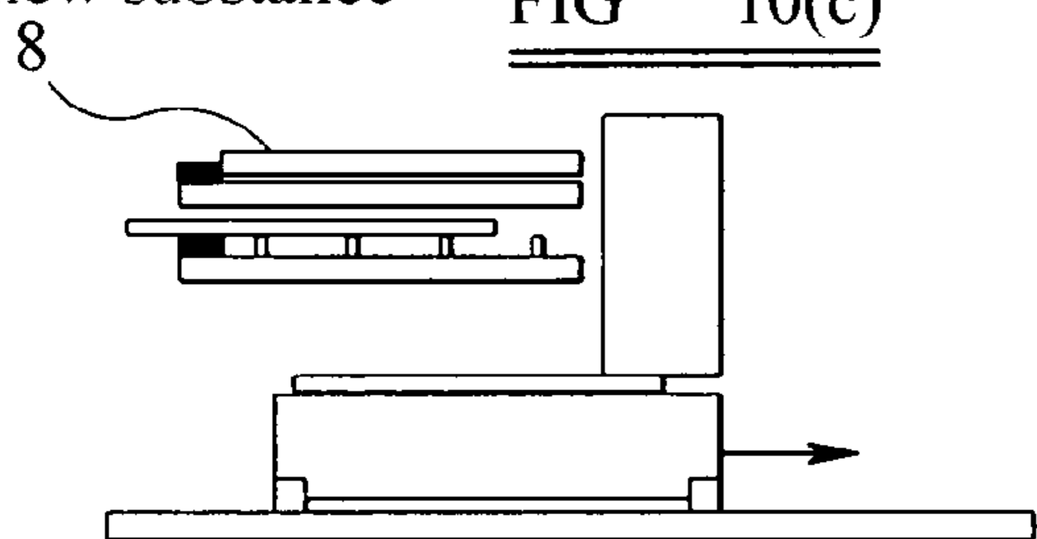
*Stage: continue expose substrate *Handler: unload exposed substrate FIG 10(e)
