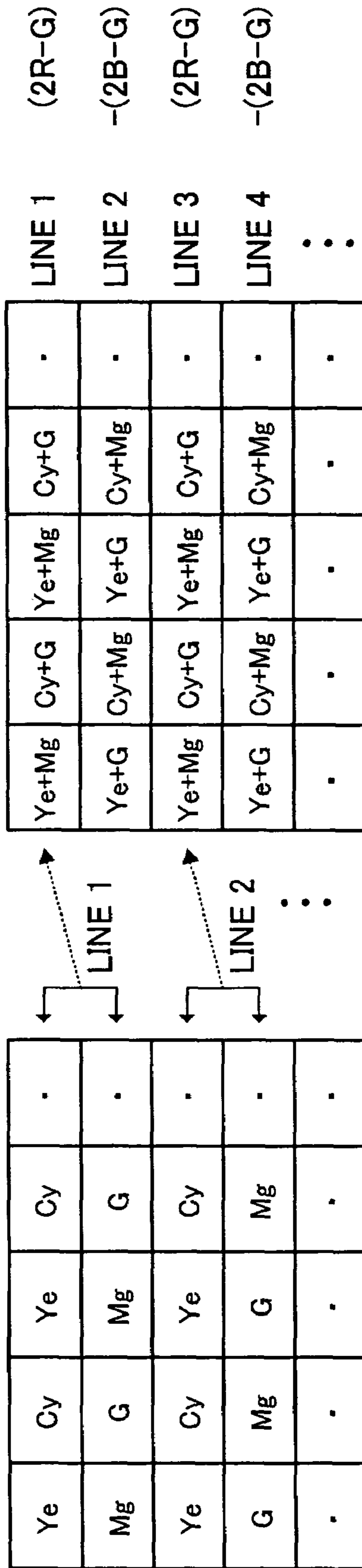
COMPLEMENTARY-COLOR COLOR FILTER
