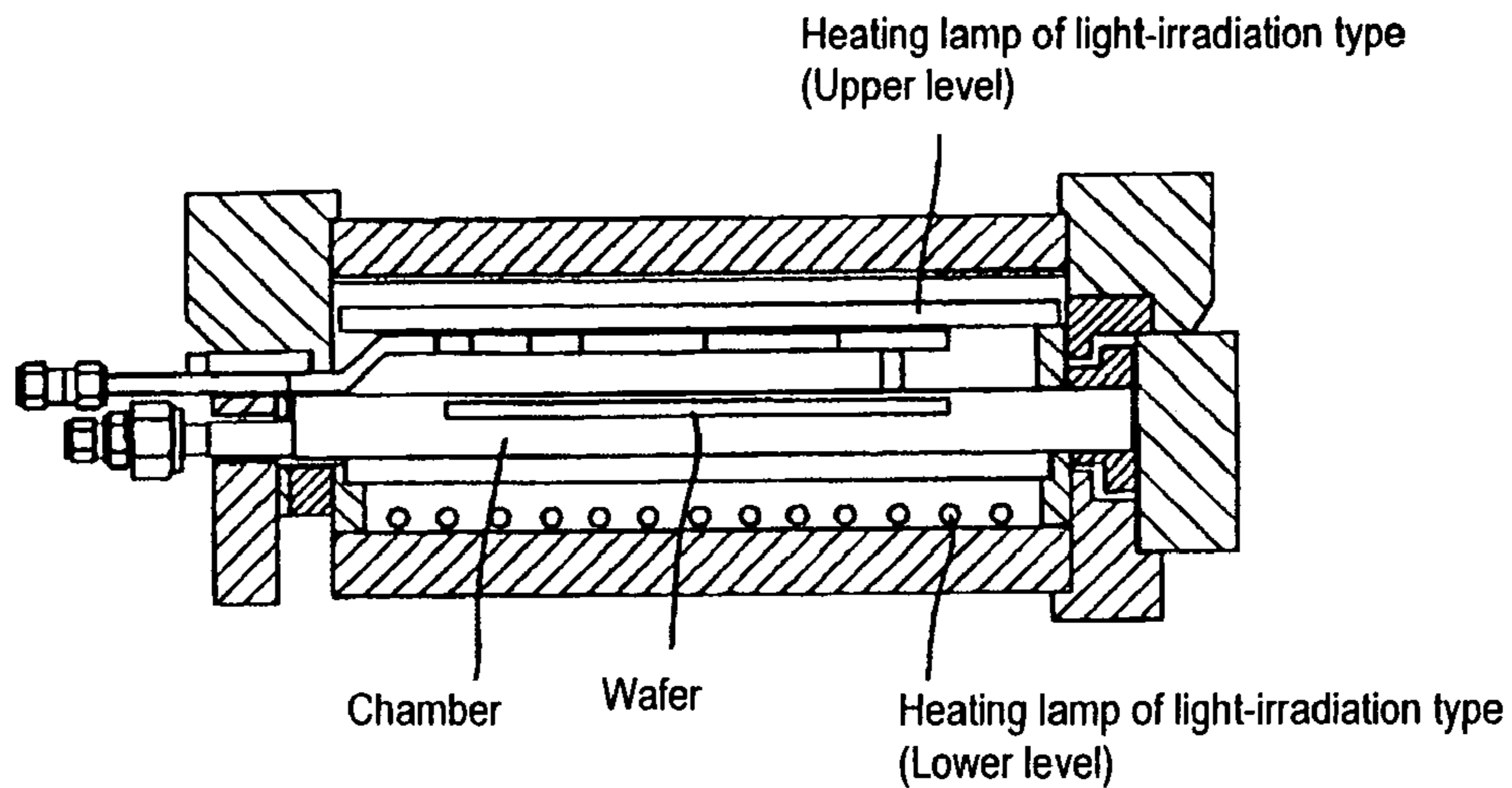
FIG. 11 (PRIOR ART)
