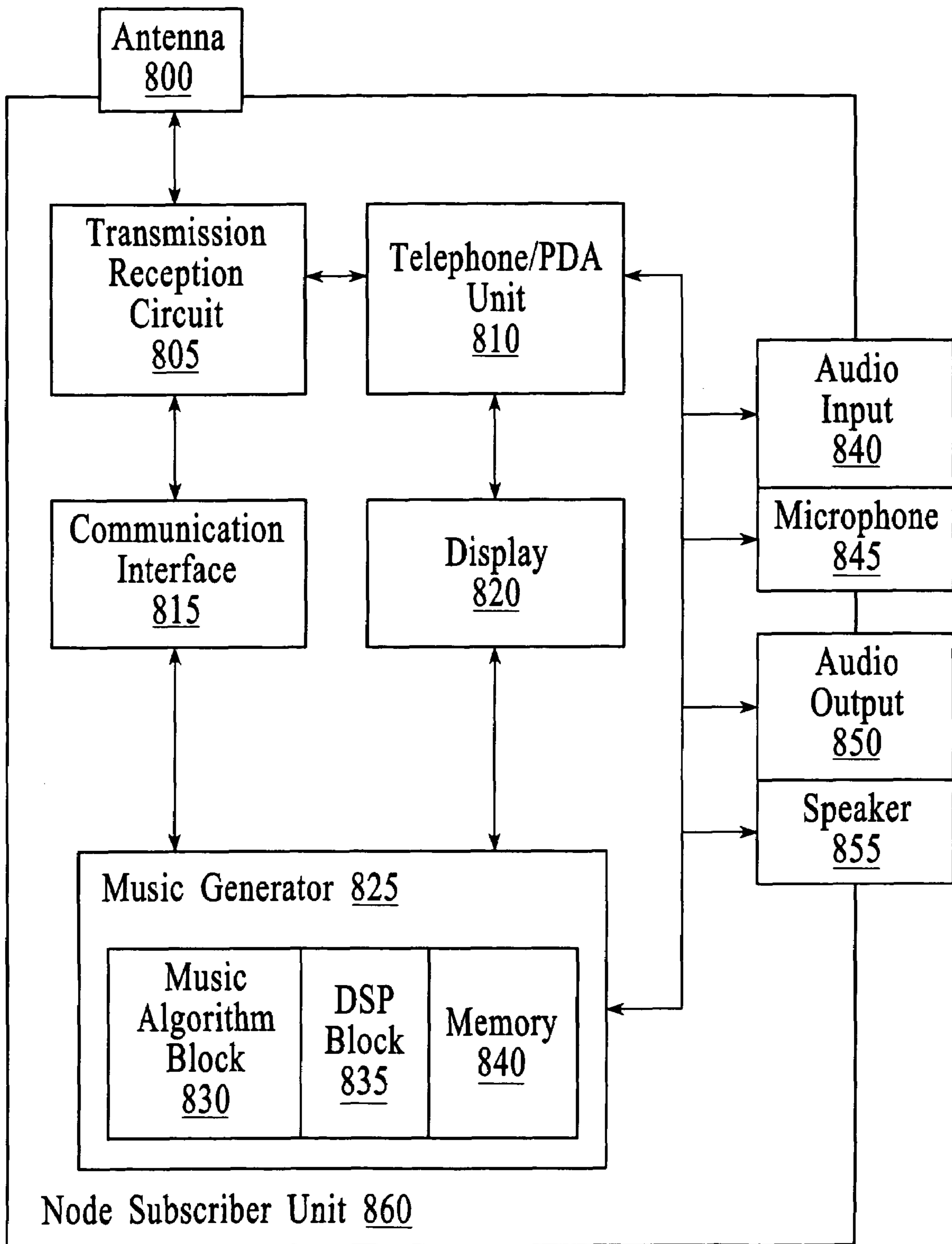
Node/Subscriber Unit Functional Blocks
