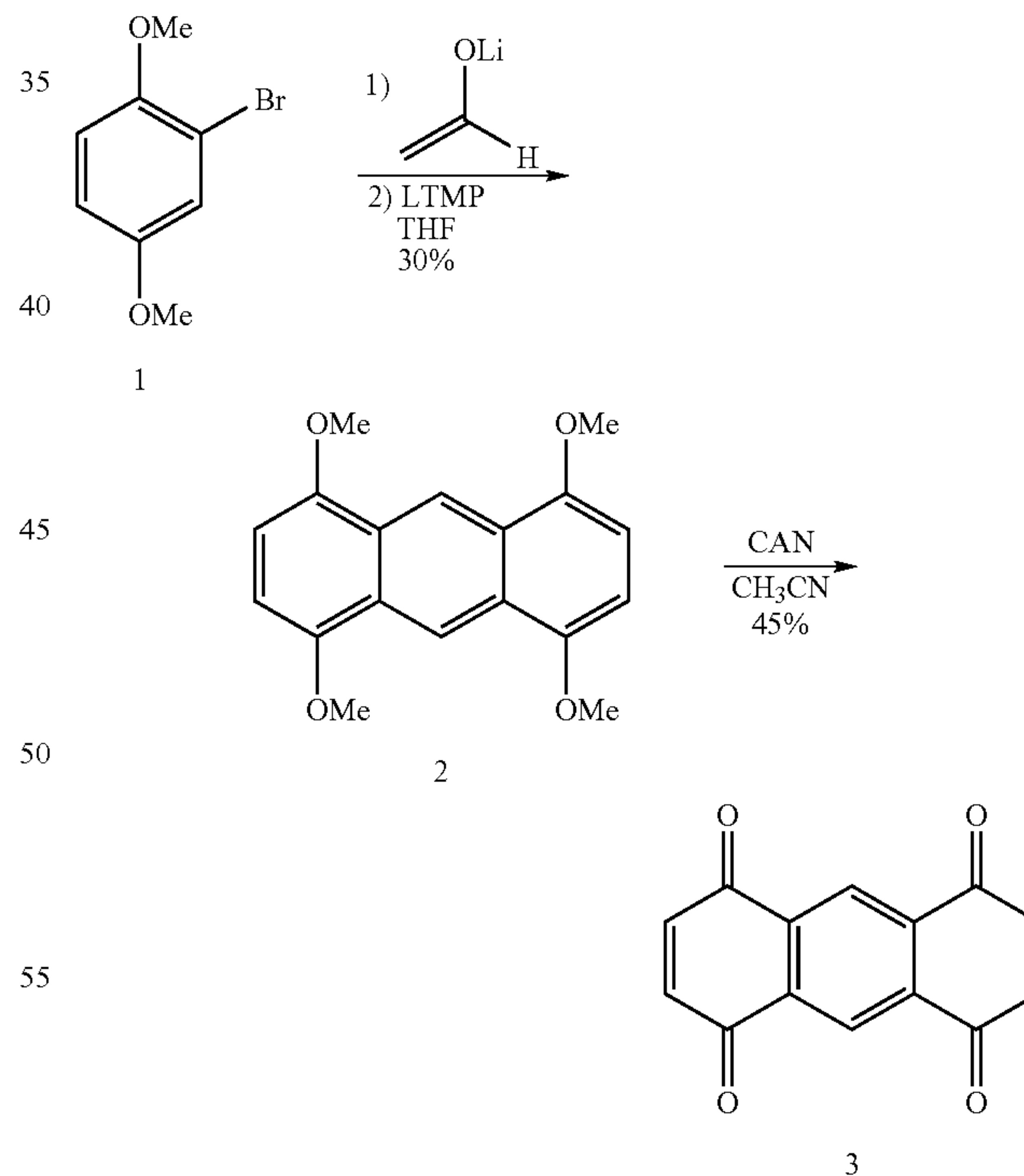
Scheme 3: Cory's preparation of 1,4,5,8-anthraquinone (3).
