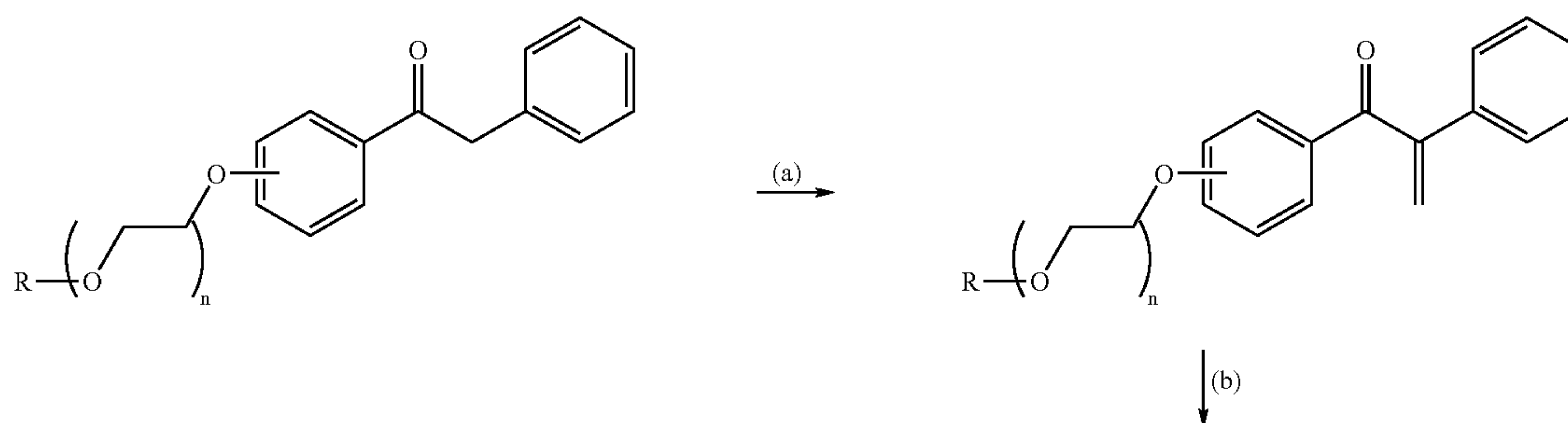
Scheme 9
