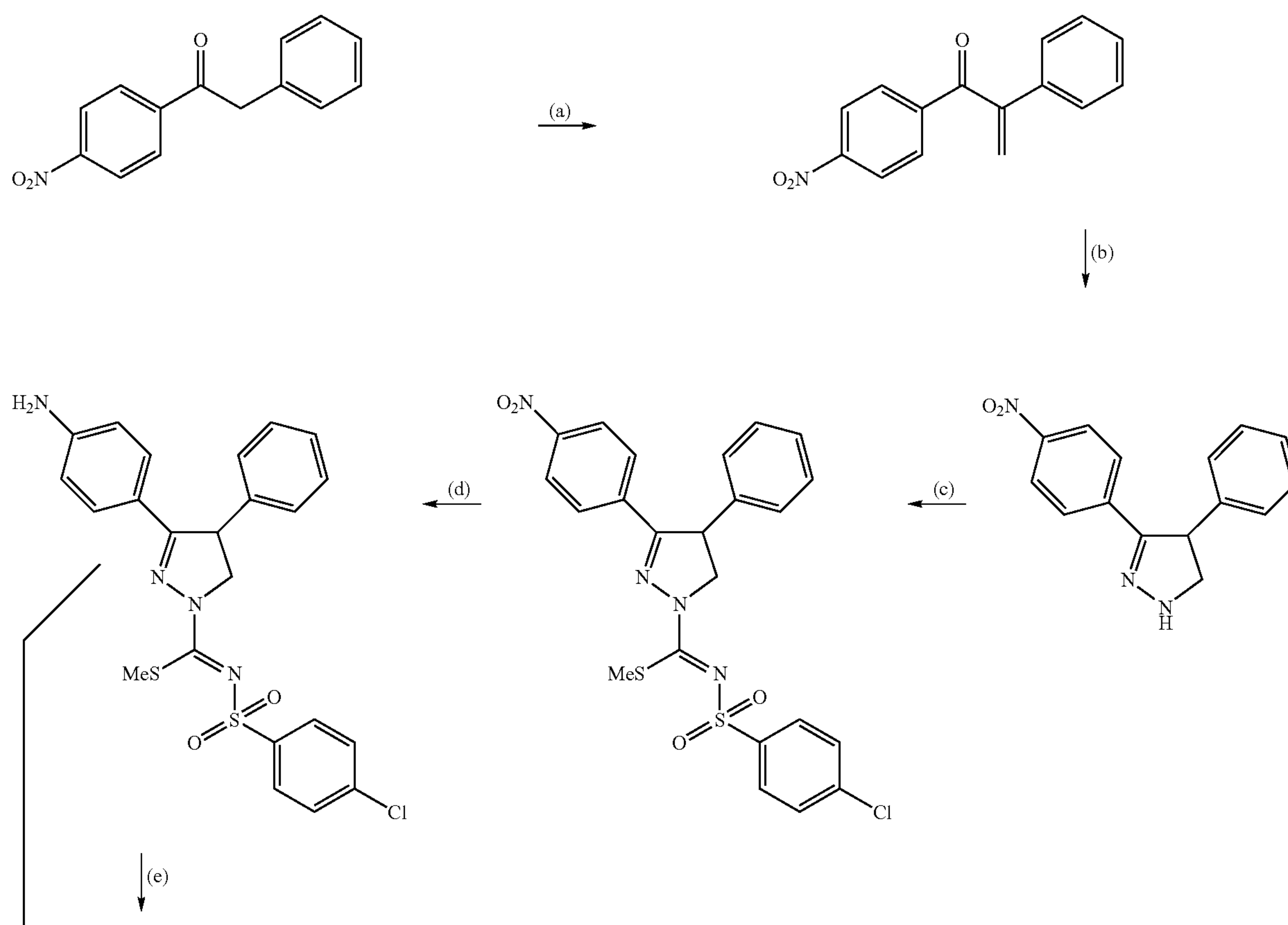
Scheme 7
