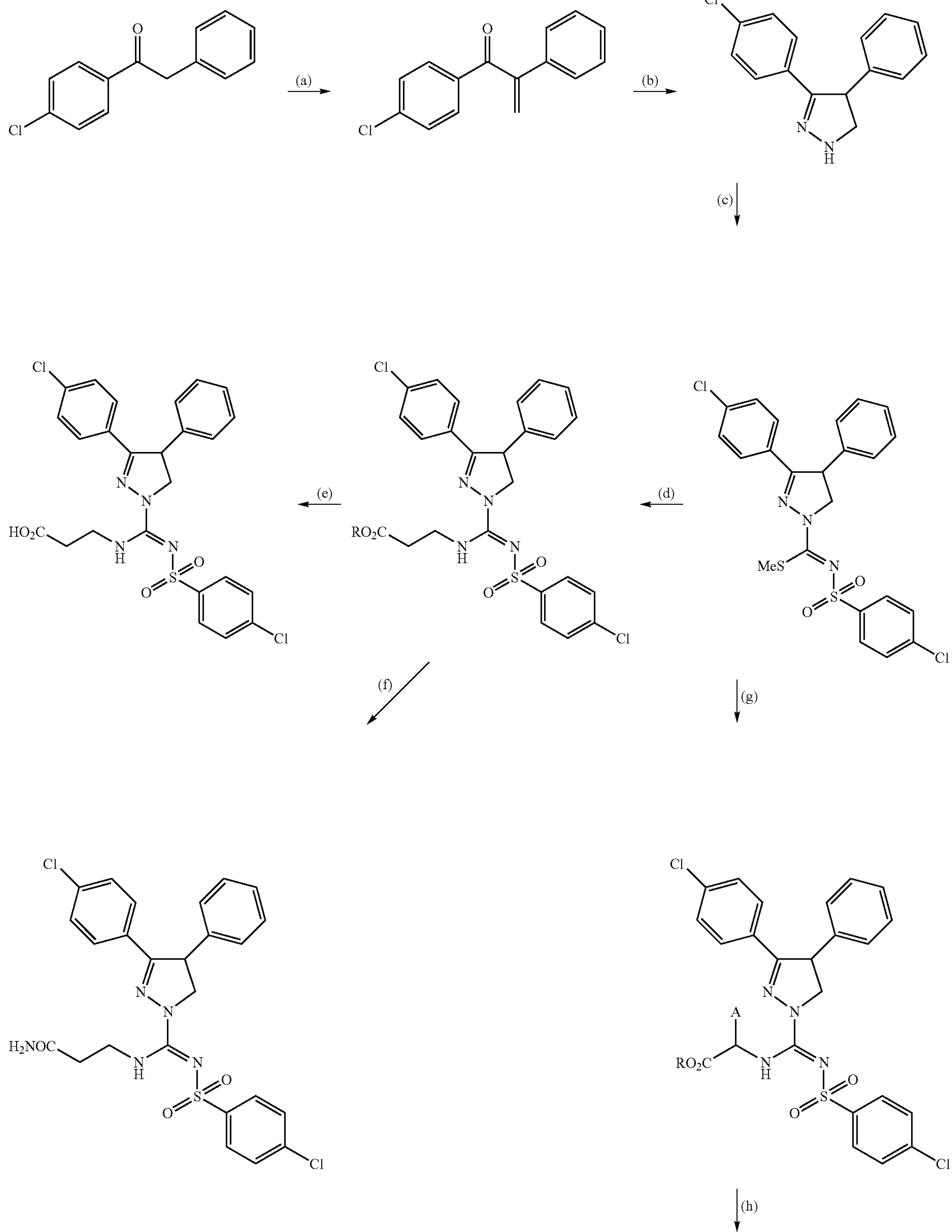
Scheme 3
