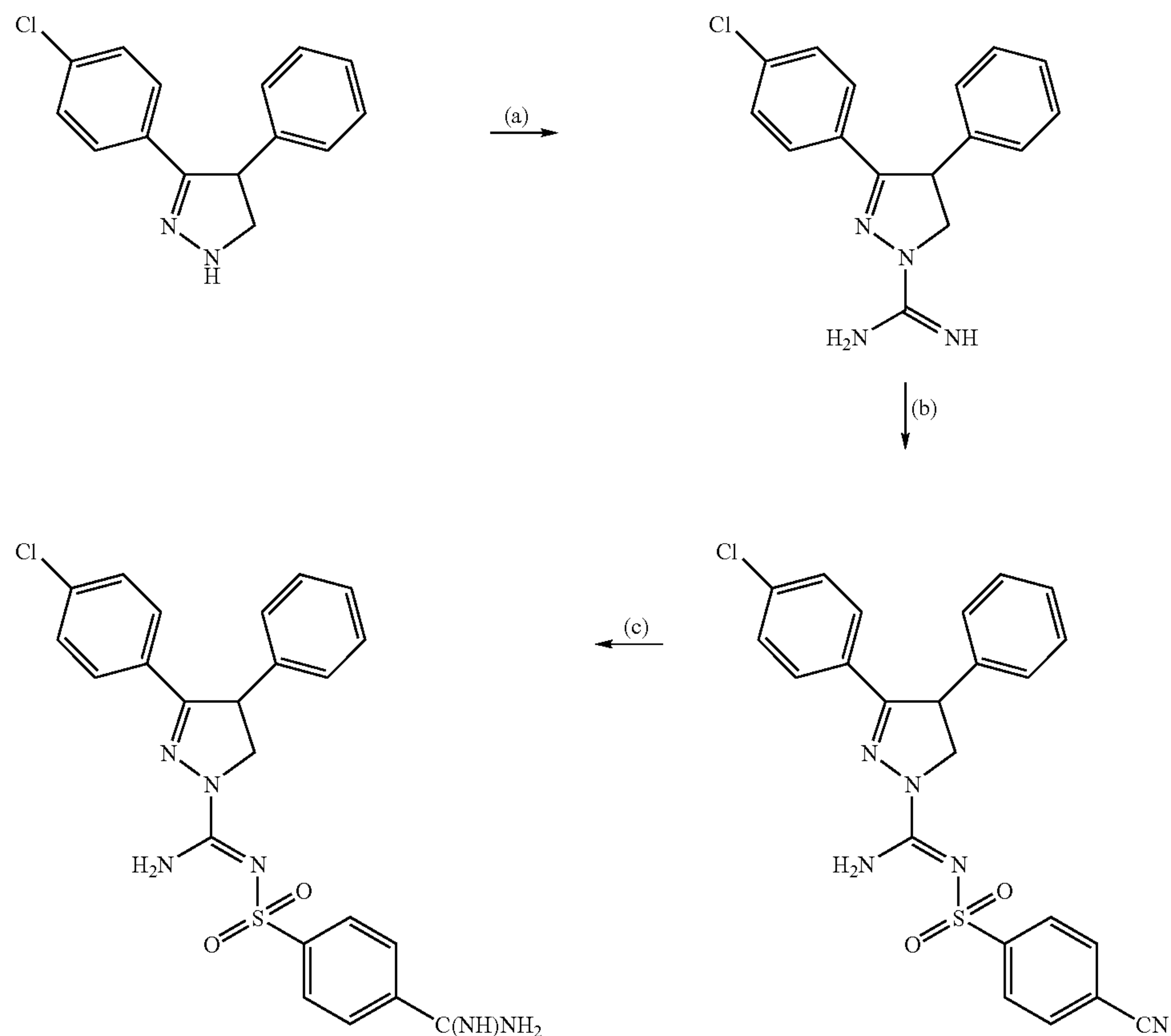
Scheme 5
