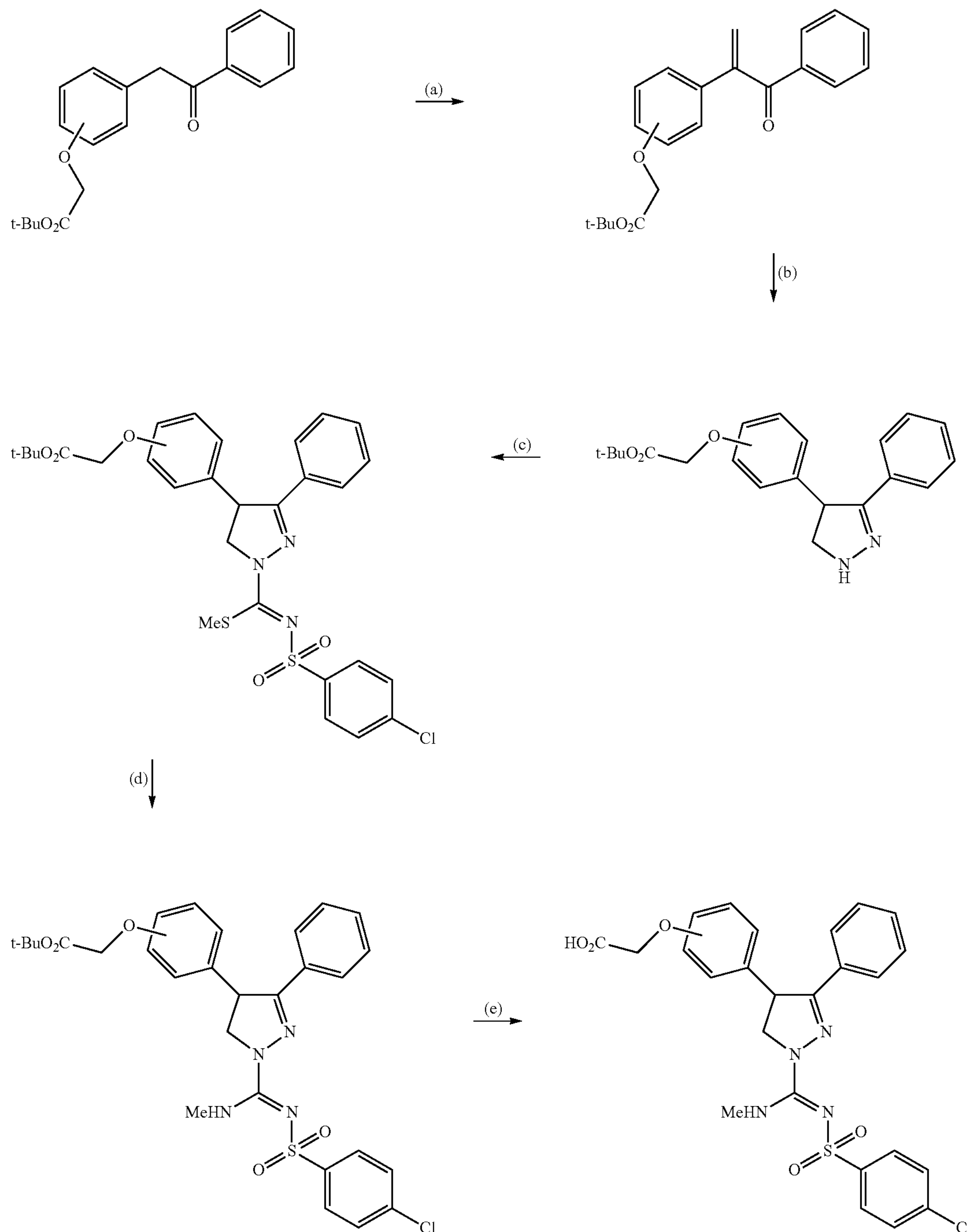
Scheme 2
