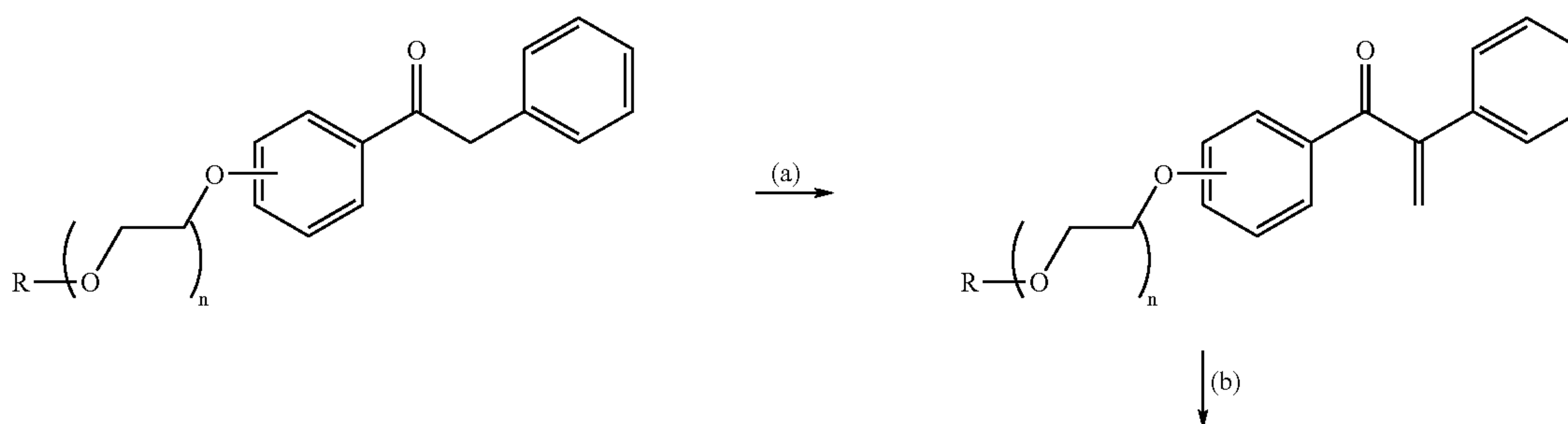
Scheme 9
