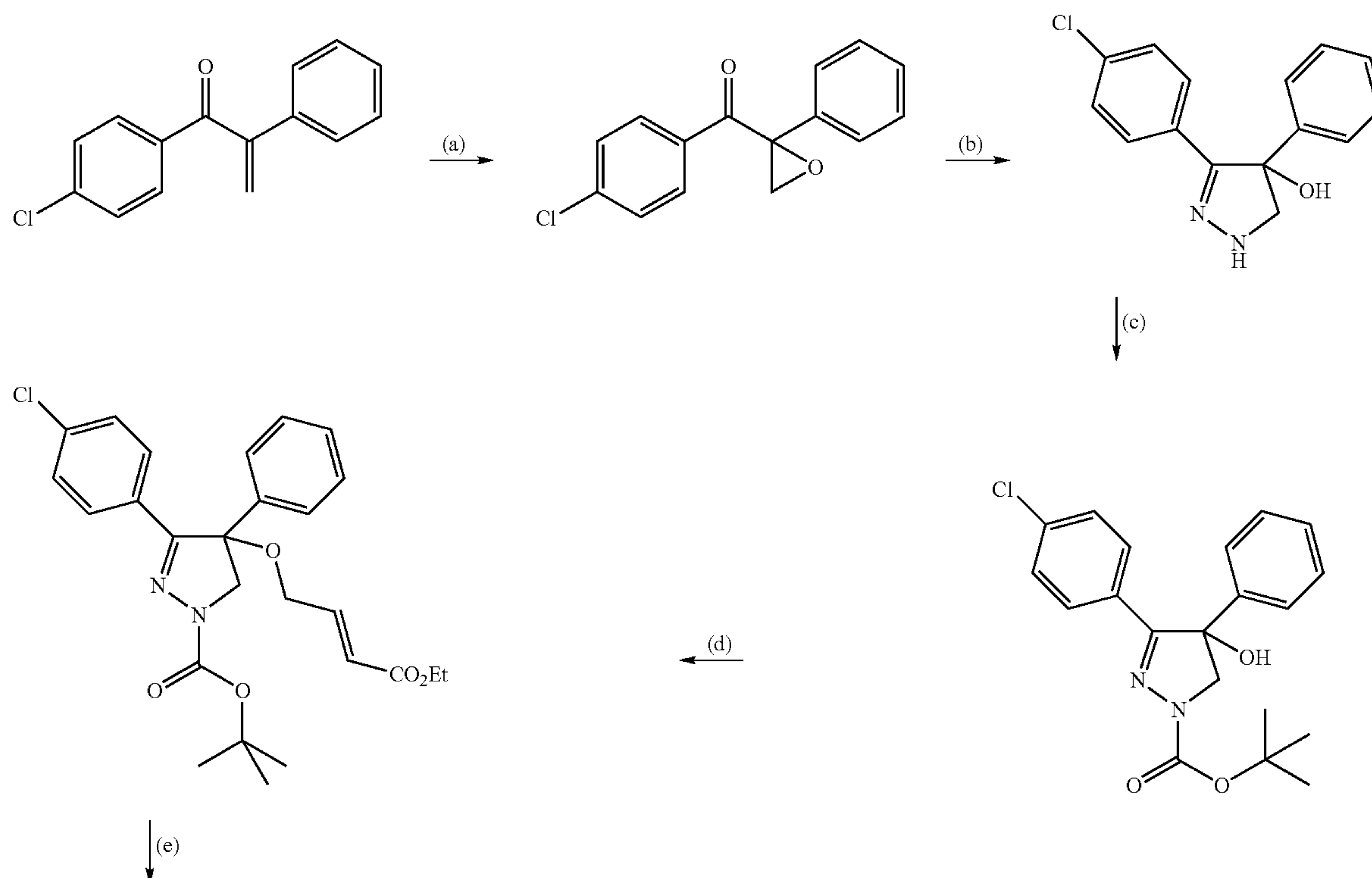
Scheme 4
