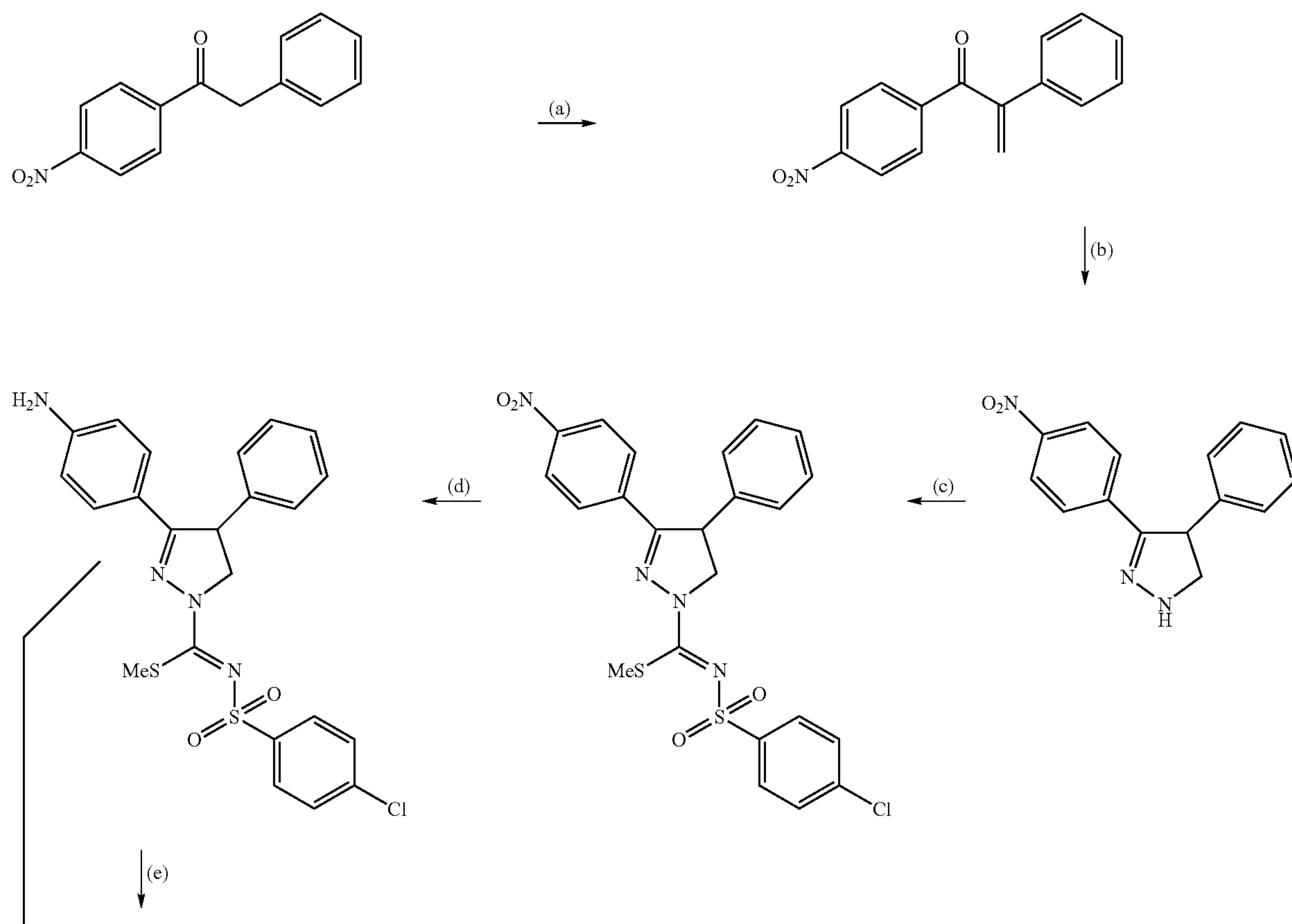
Scheme 7
