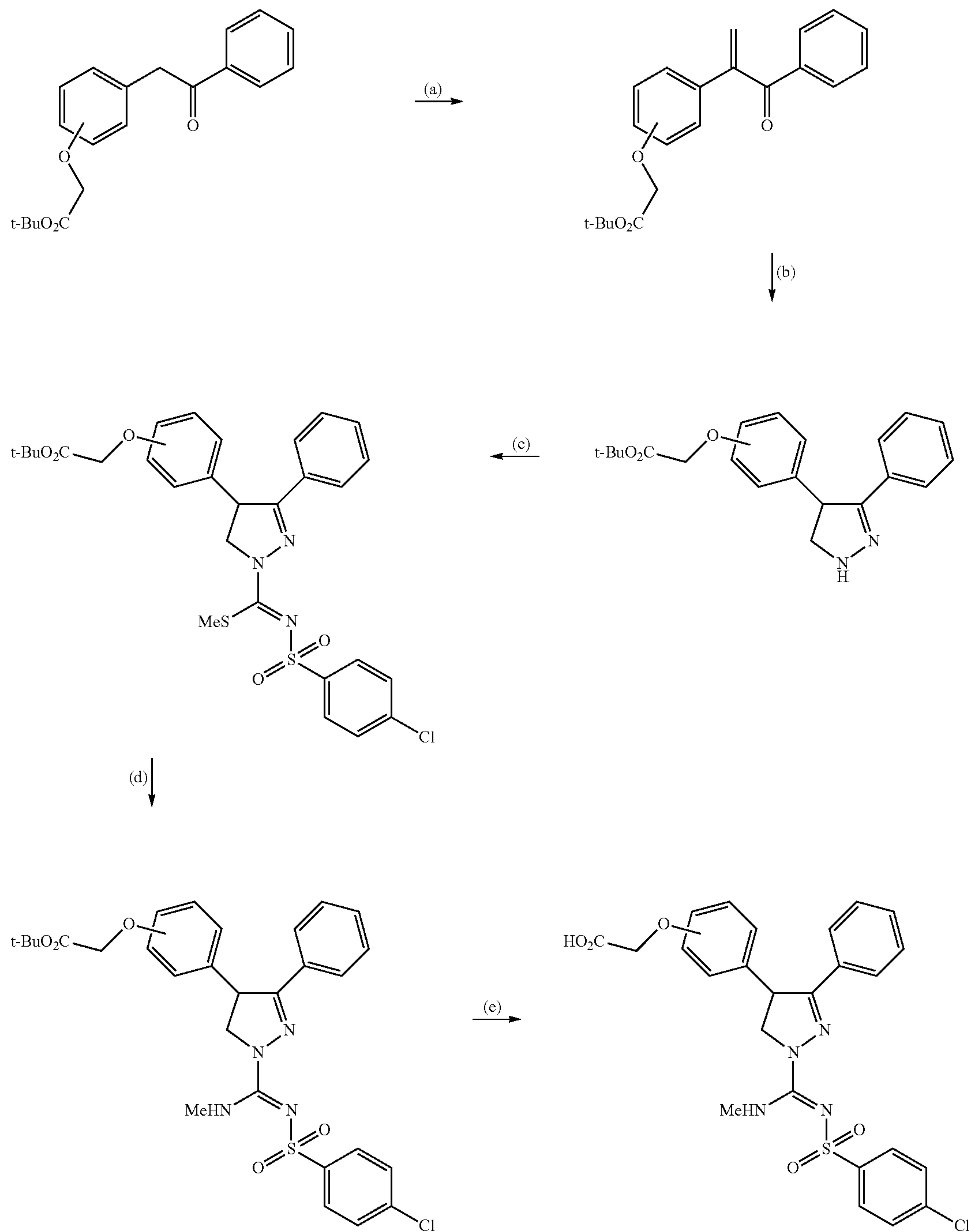
Scheme 2
