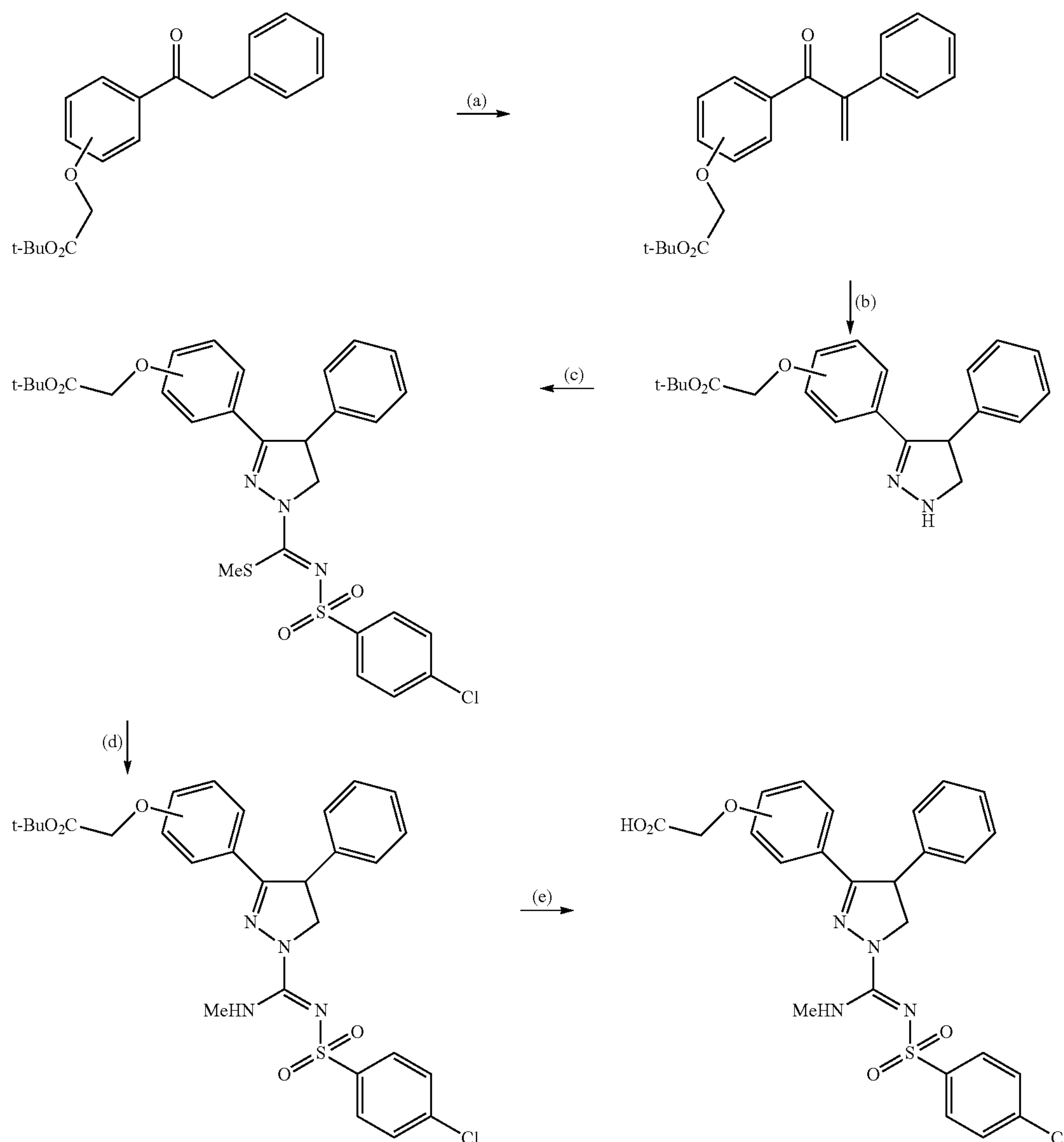
Scheme 1
