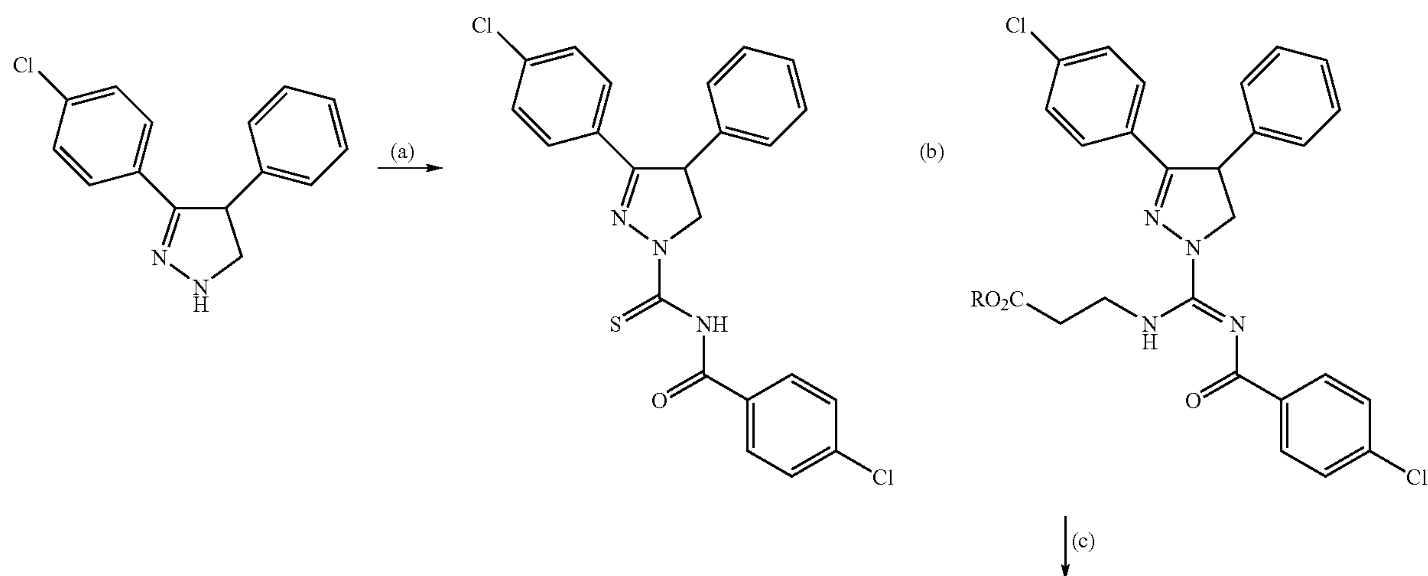
Scheme 6
