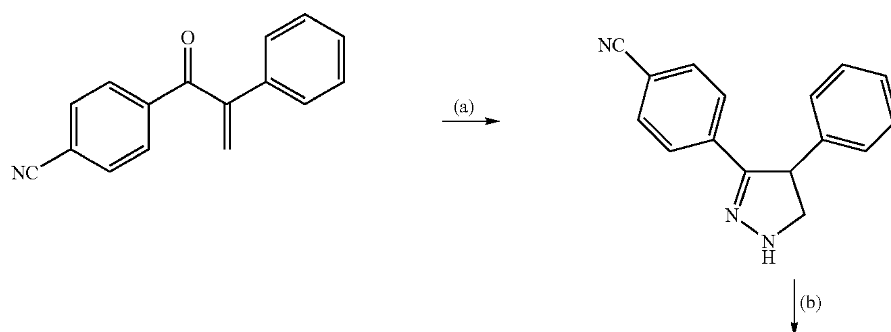
Scheme 8
