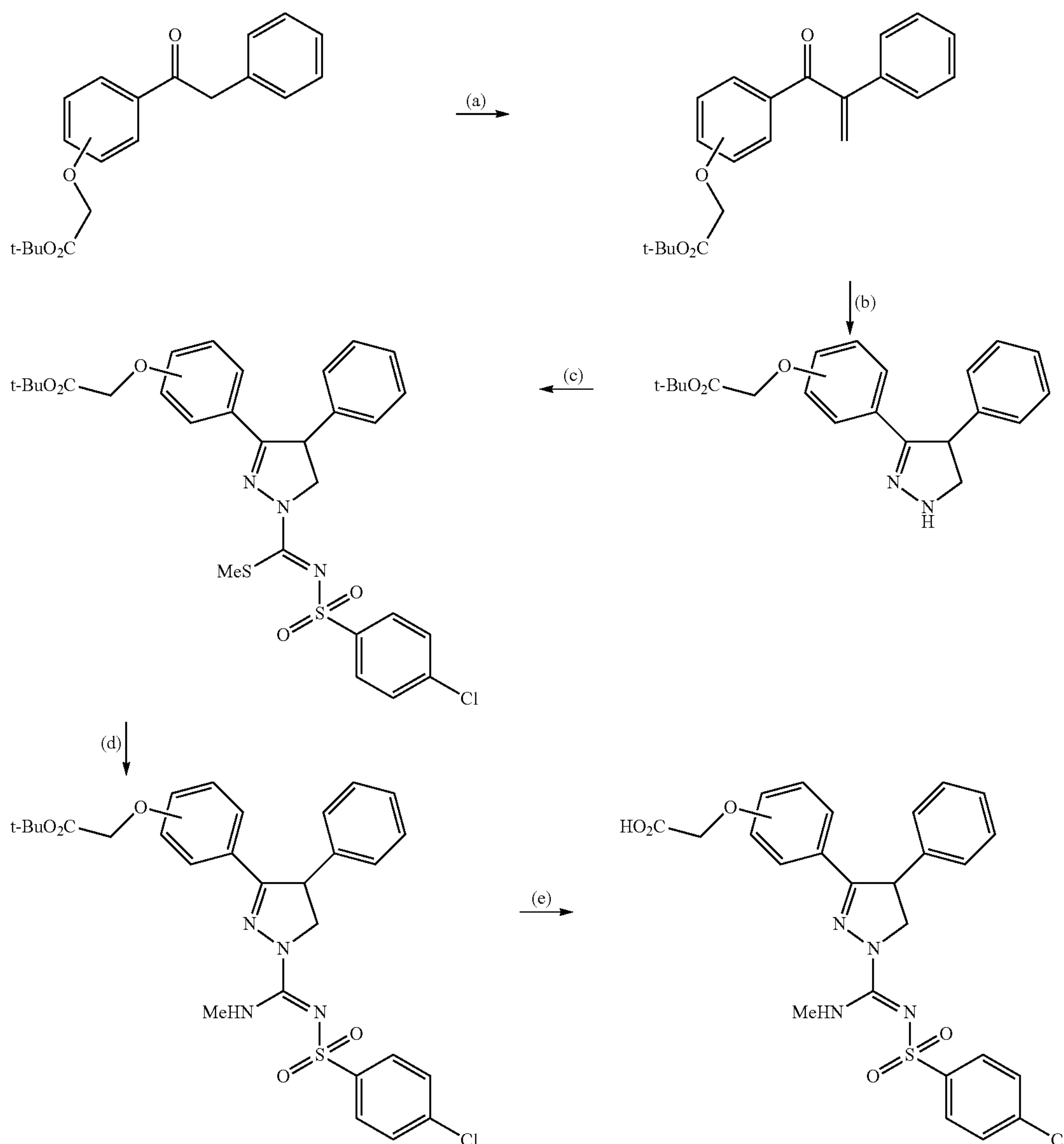
Scheme 1
