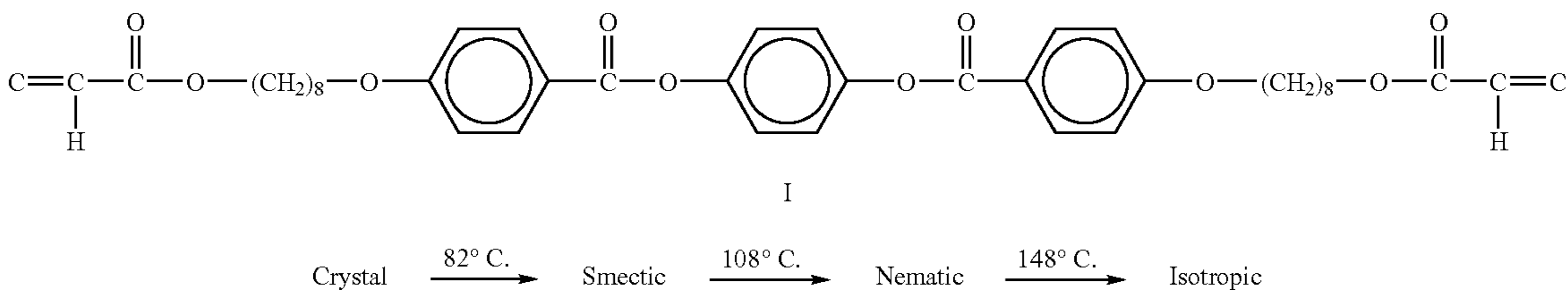
Formula 3: Liquid crystalline diacrylate
