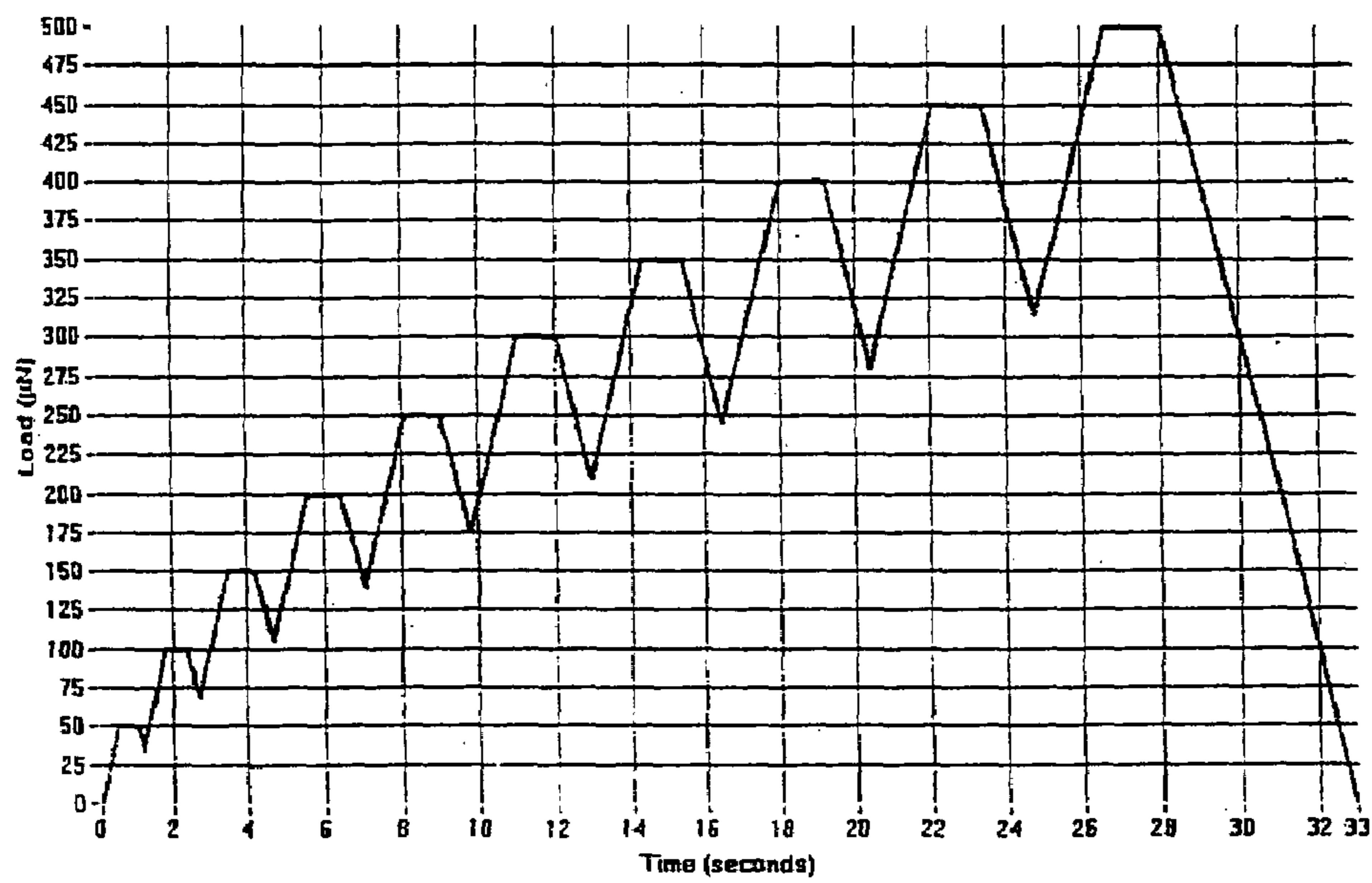
Figure 1. Typical Load-Function used for the indentation Experiments
