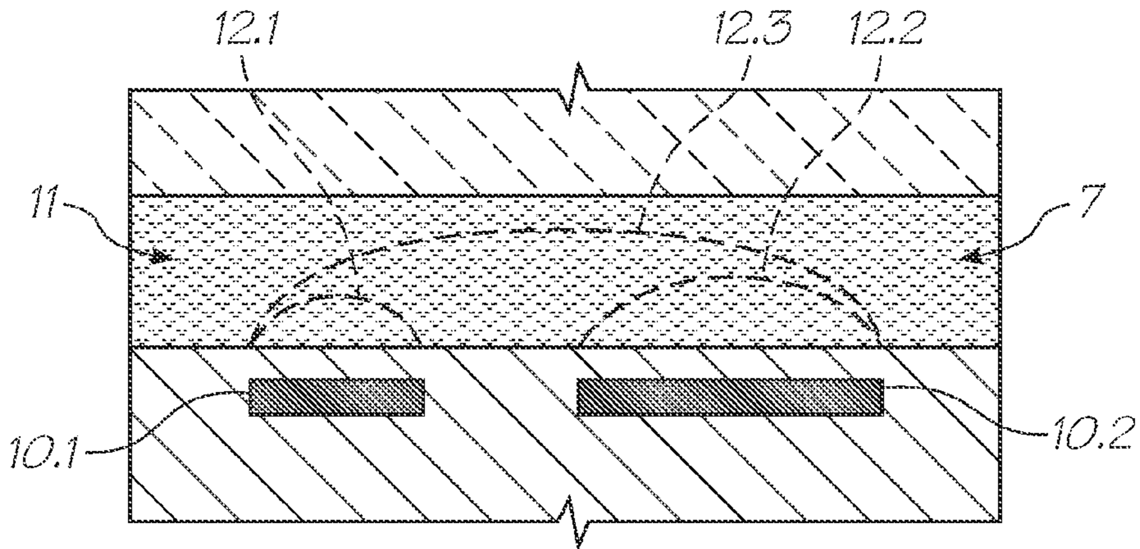
FIG. 52 (PRIOR ART)
