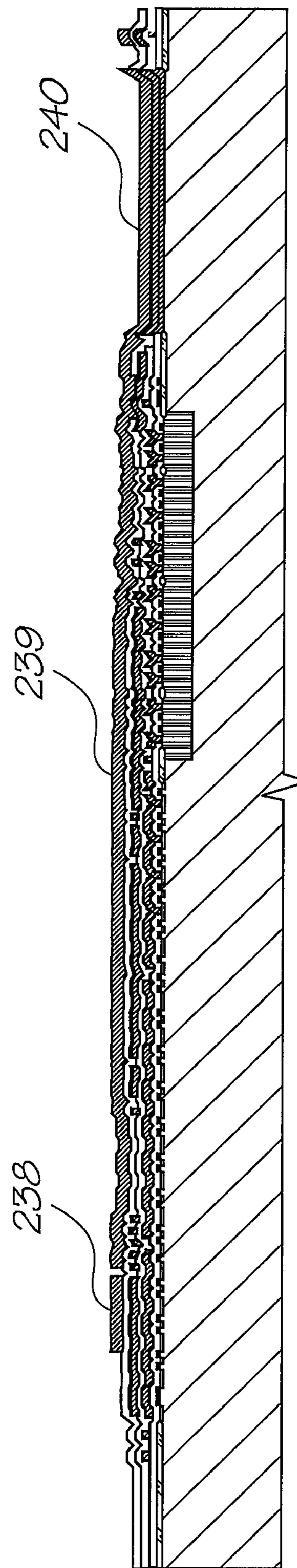
Deposit metal 3
