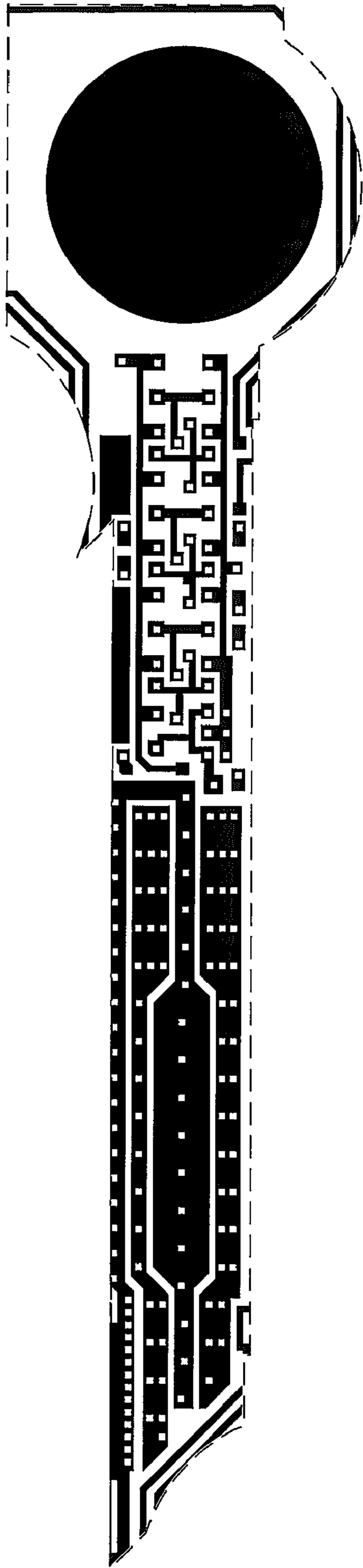
Metal 1 mask
