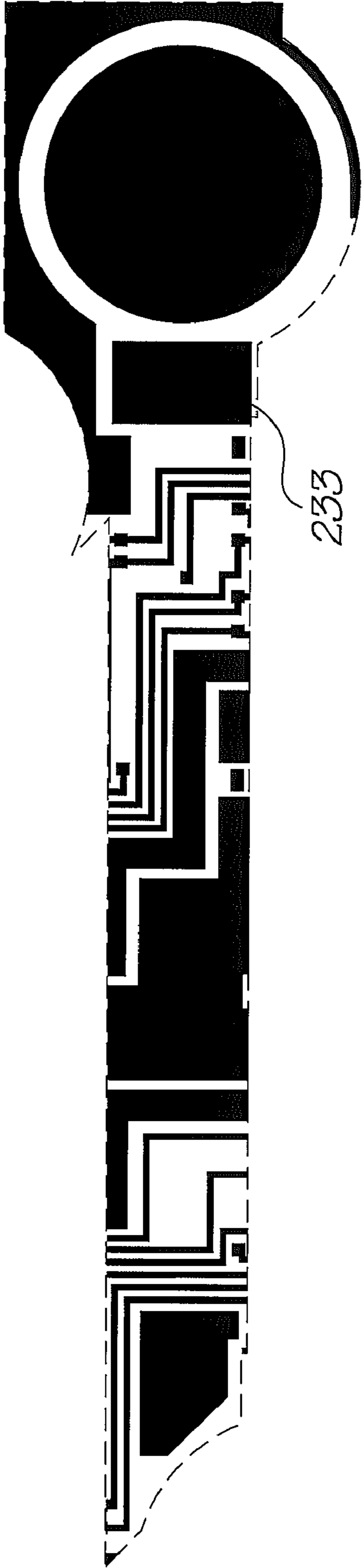
Metal 2 mask
