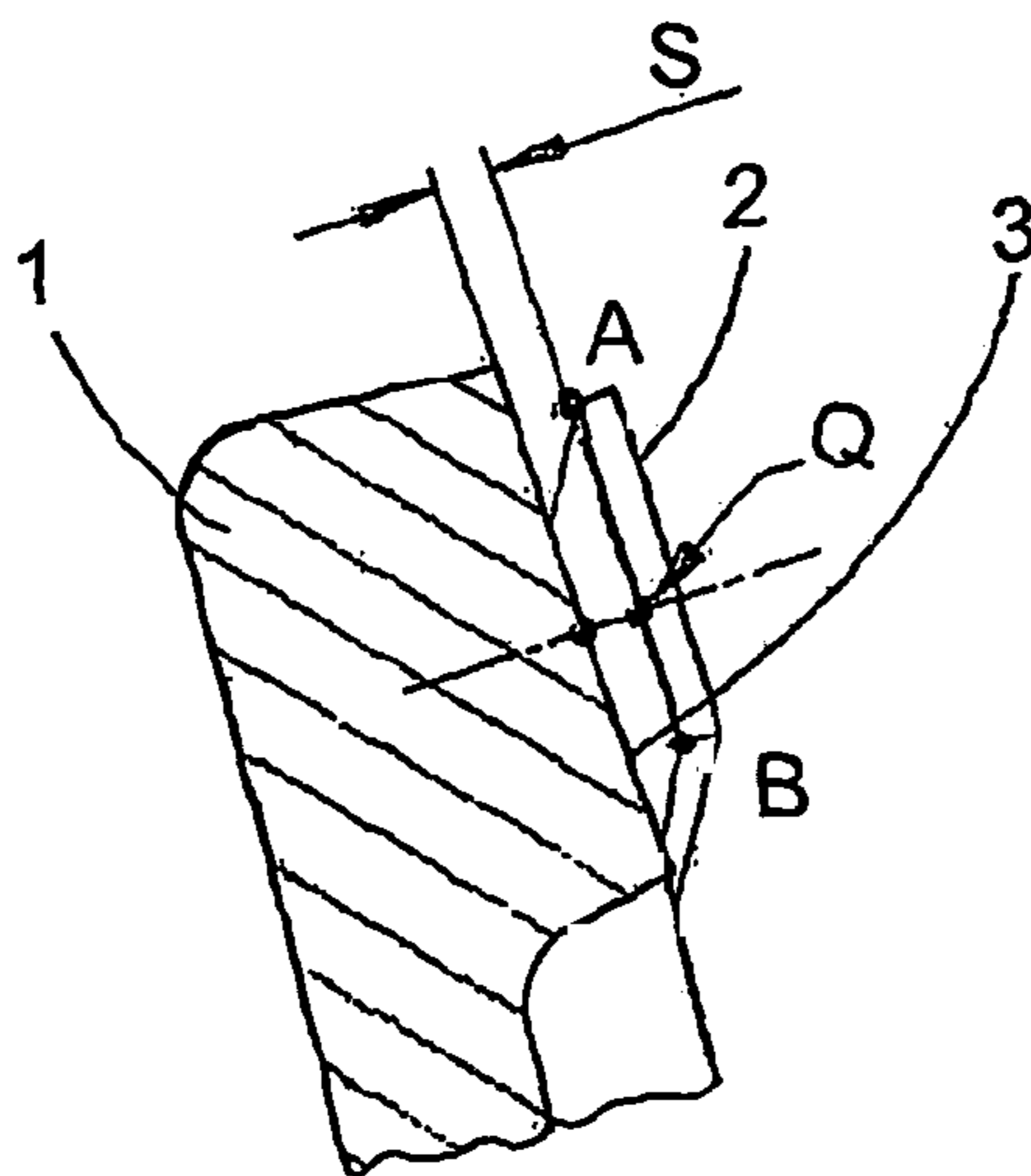
Fig. 3 (SECTION XX)
