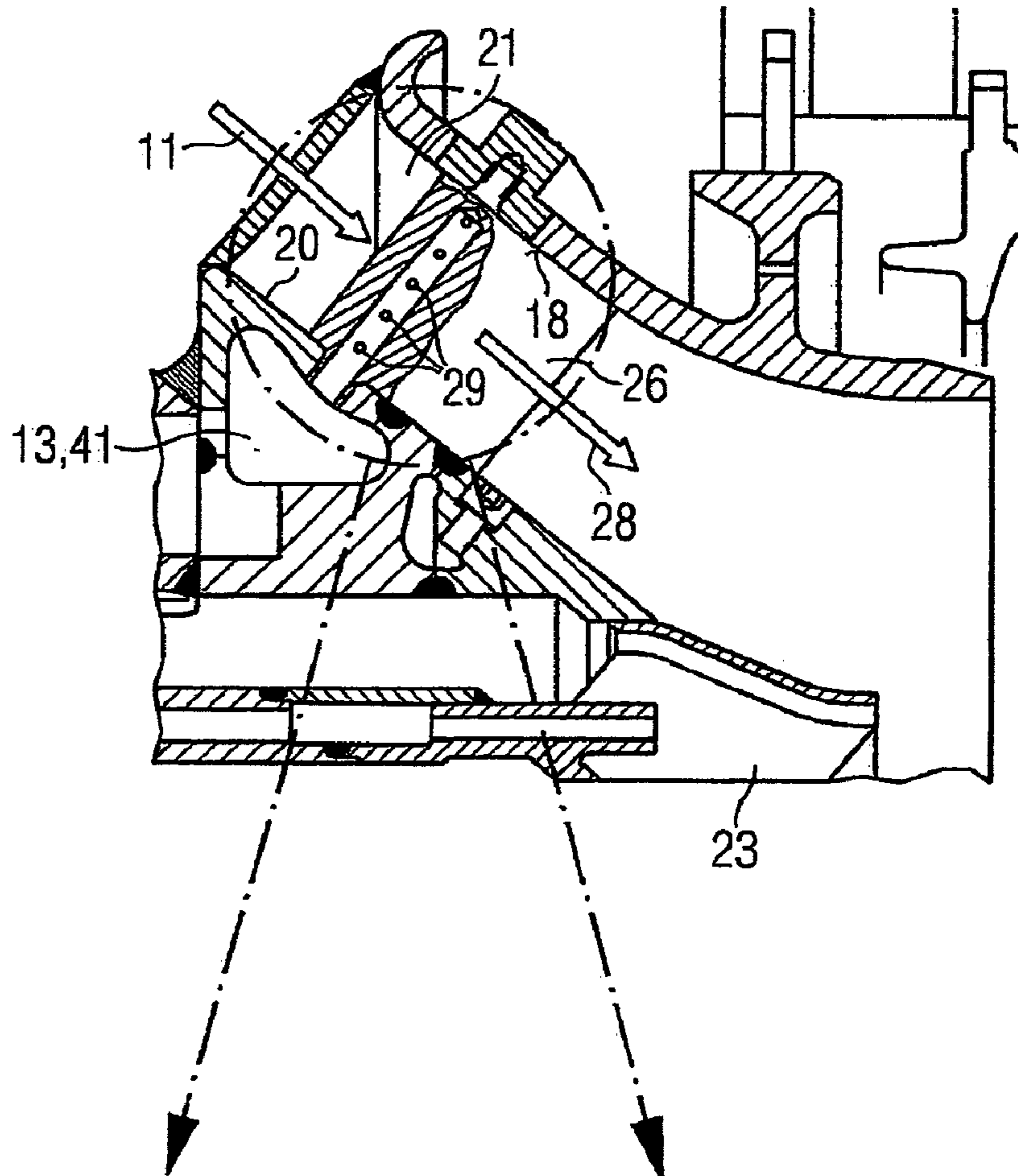
FIG 3 Prior art
