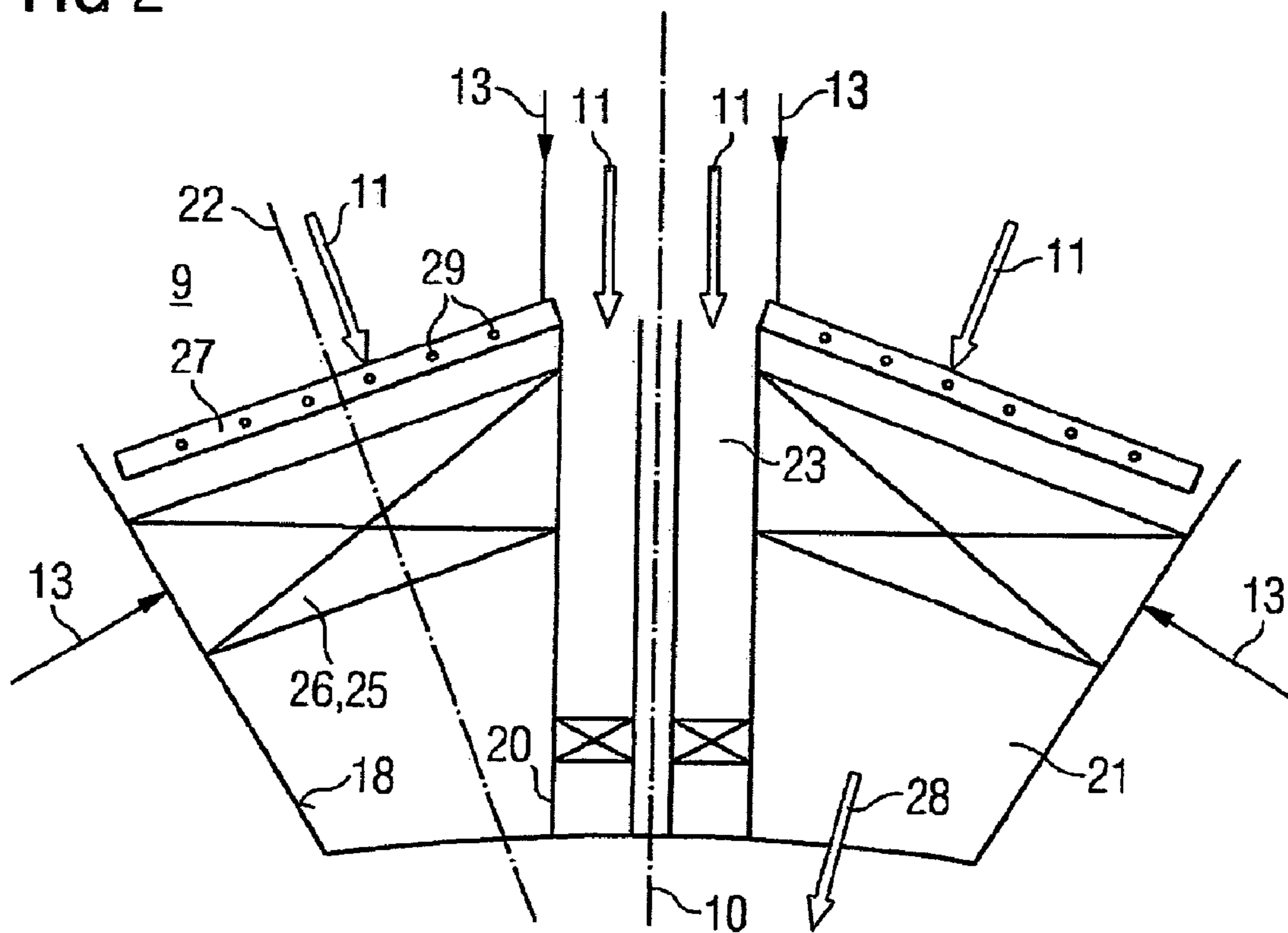
FIG 2 Prior art
