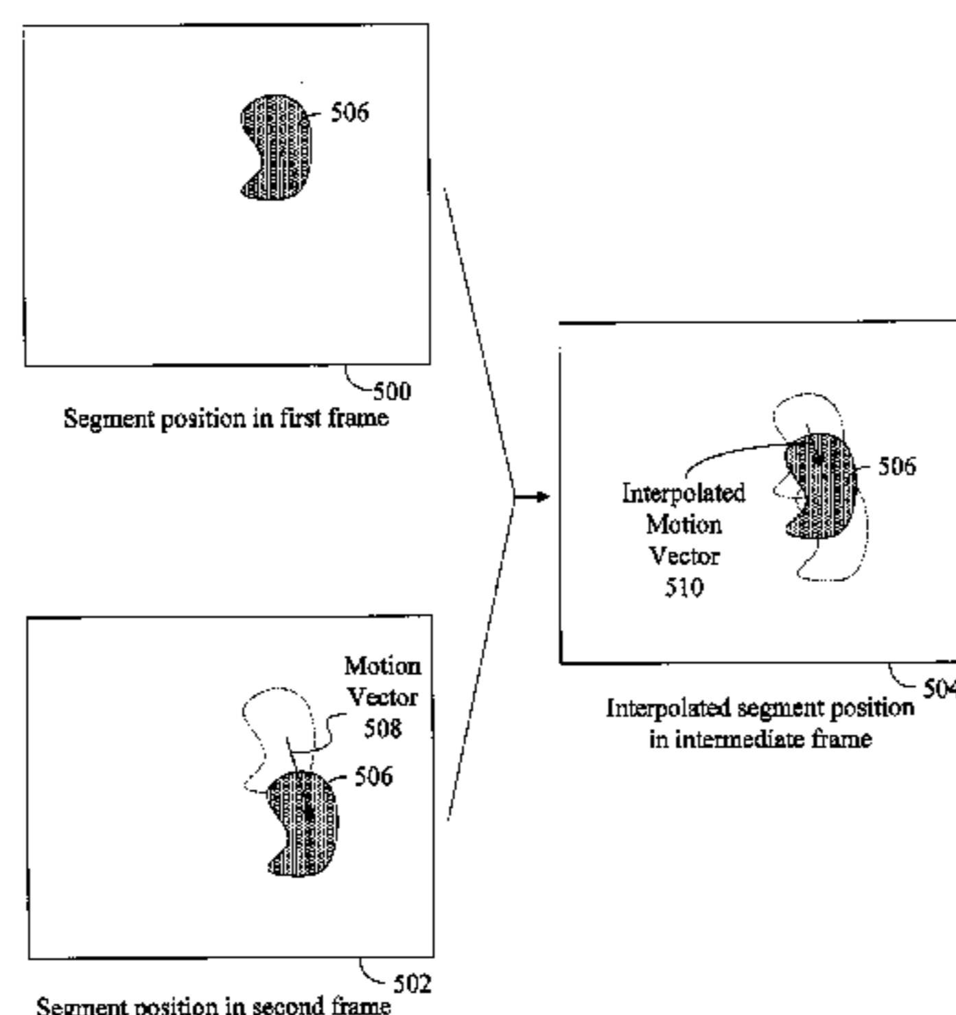
Intermediate Frame Interpolation
