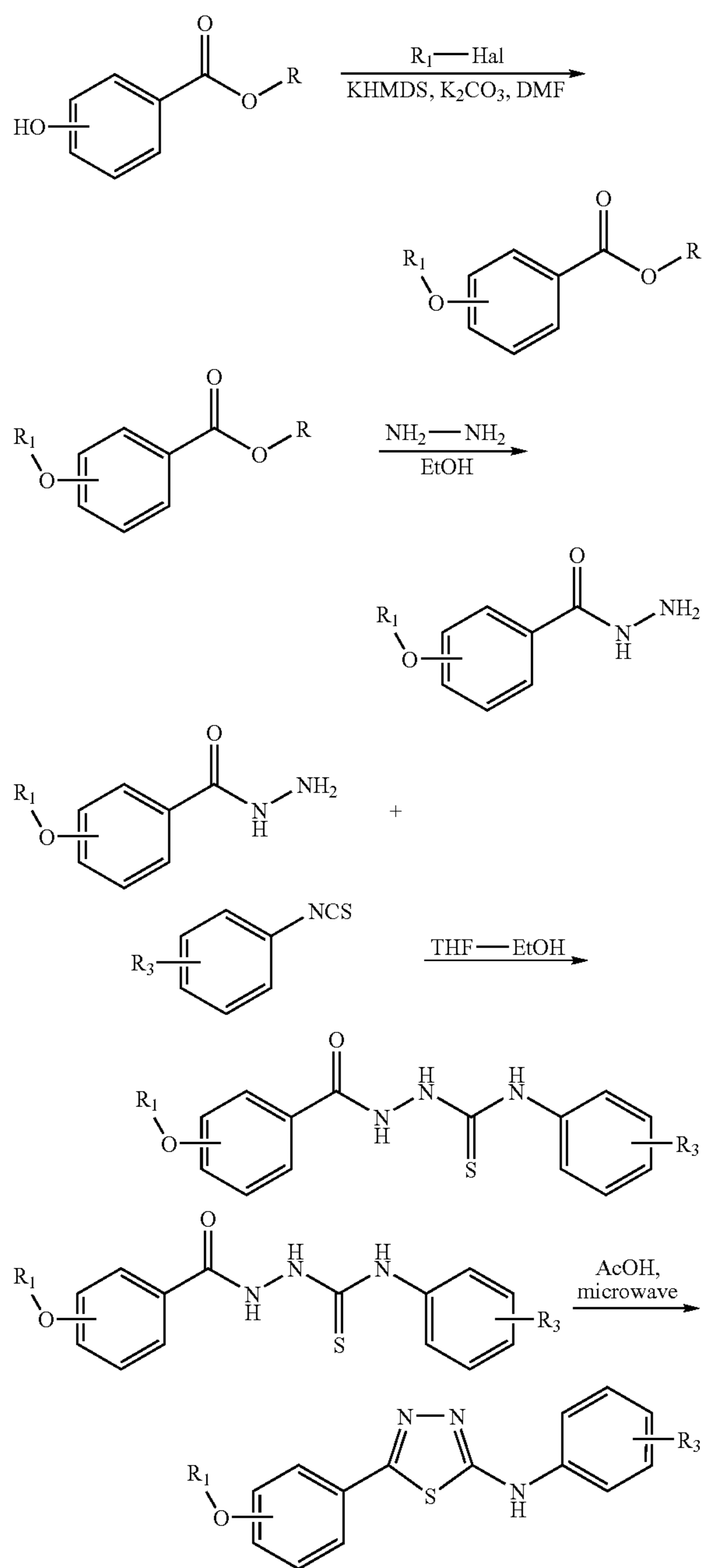
Scheme XV
