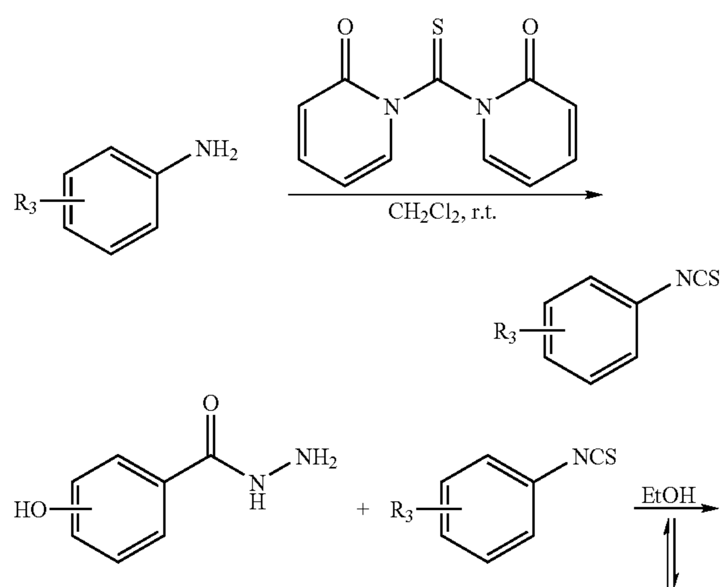
Scheme XI
