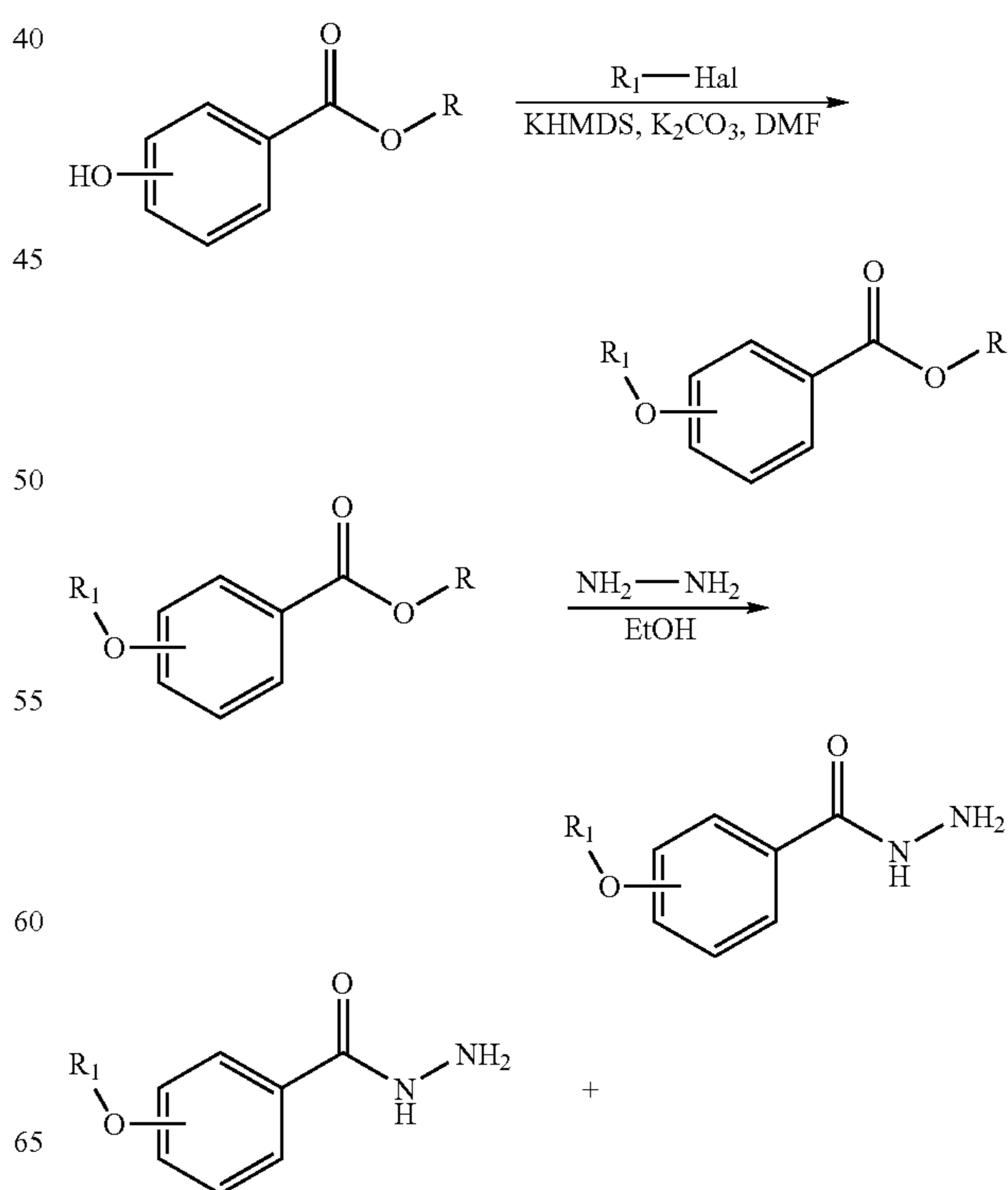
Scheme XII
