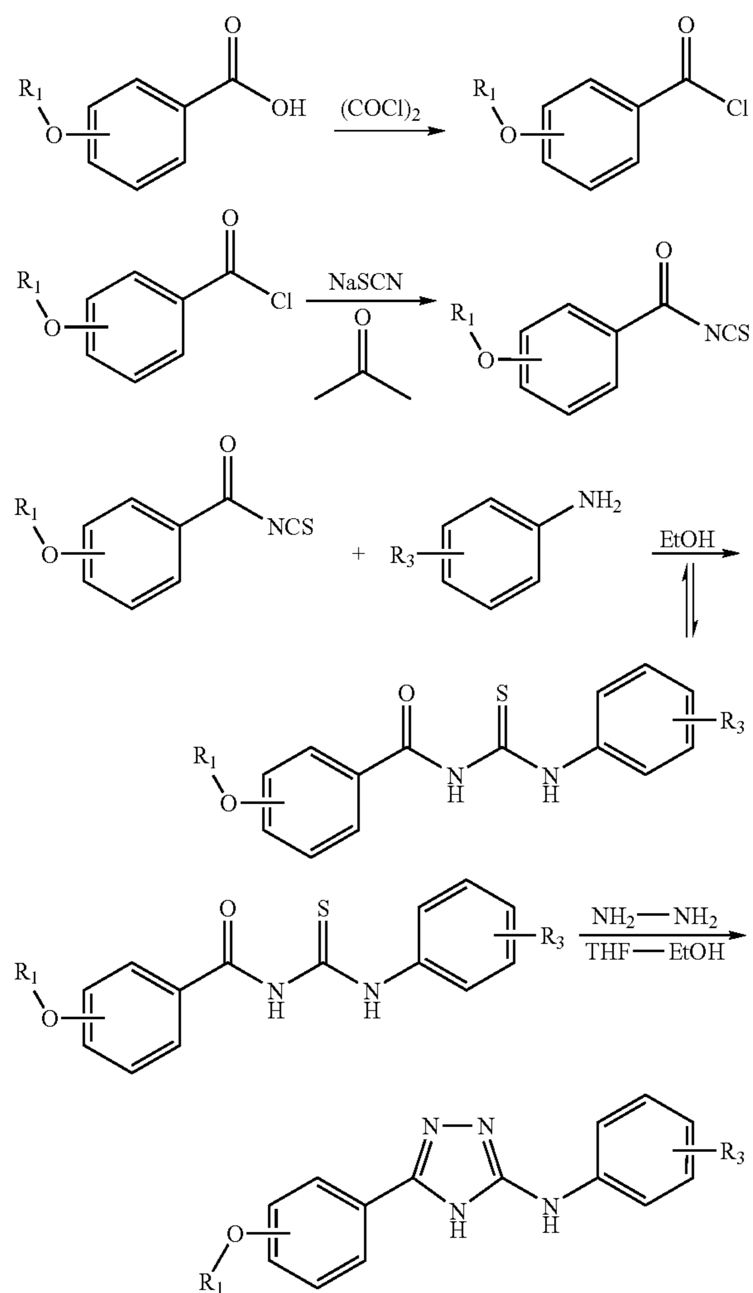
Scheme VII
