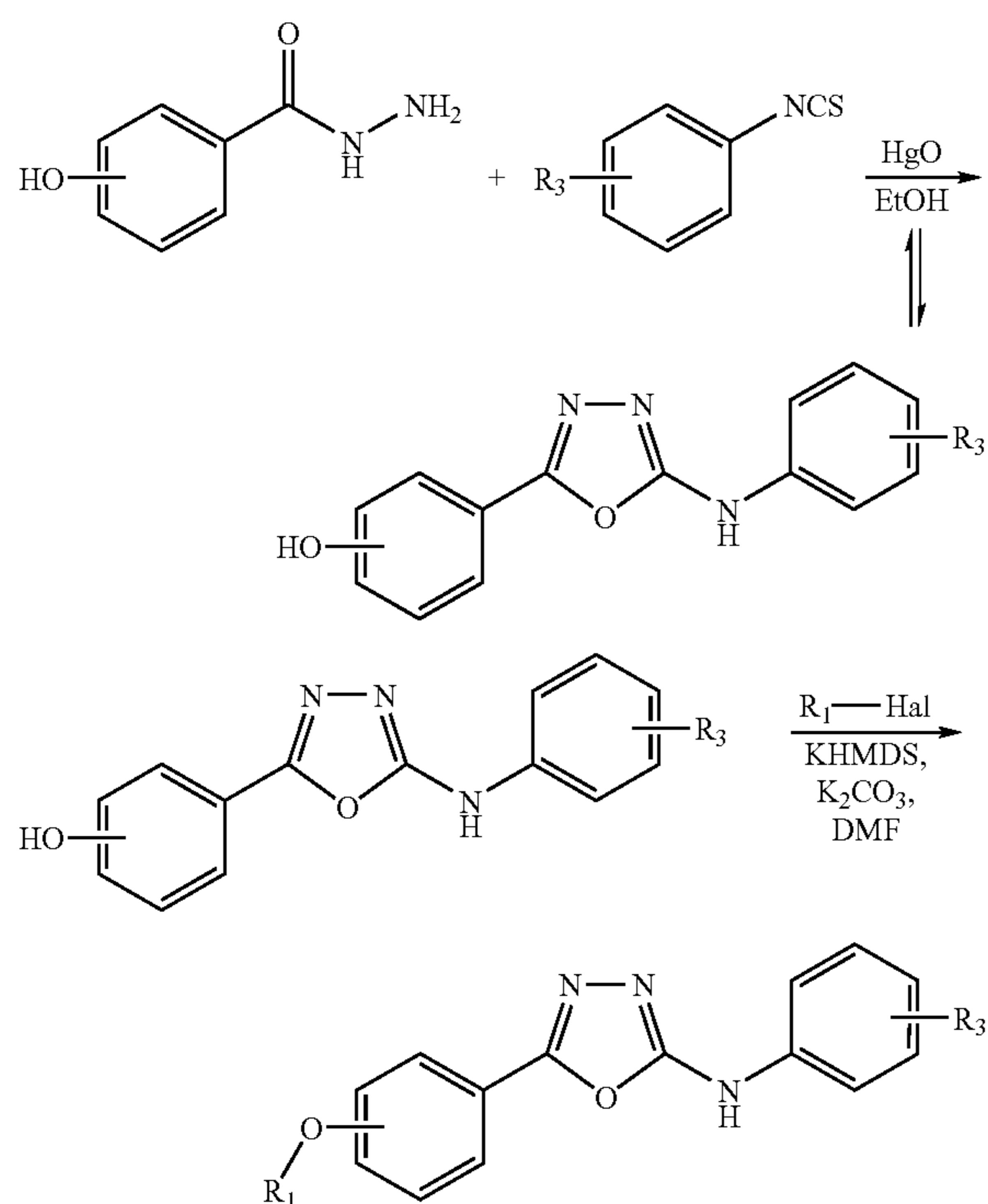
Scheme X
