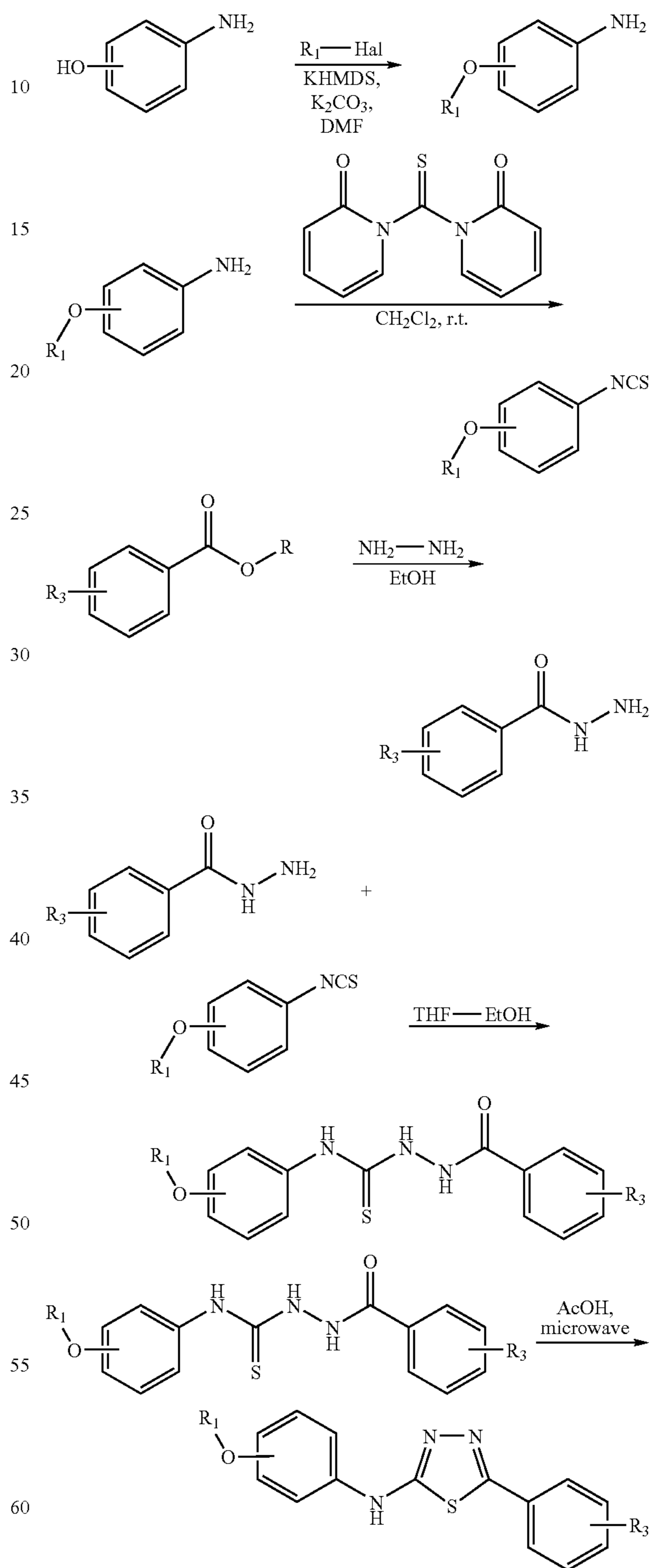
Scheme XVI
