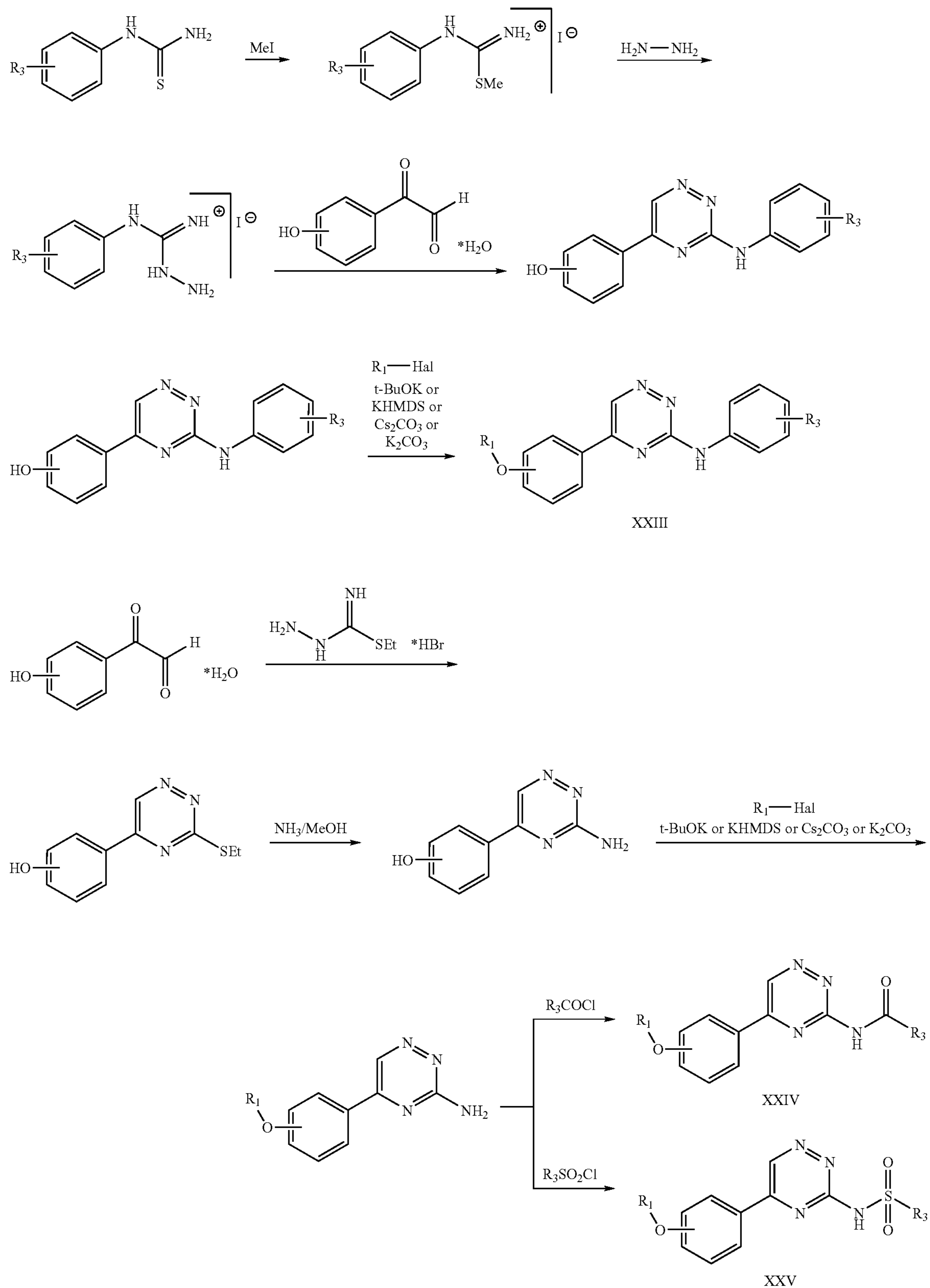
Scheme XXVII
