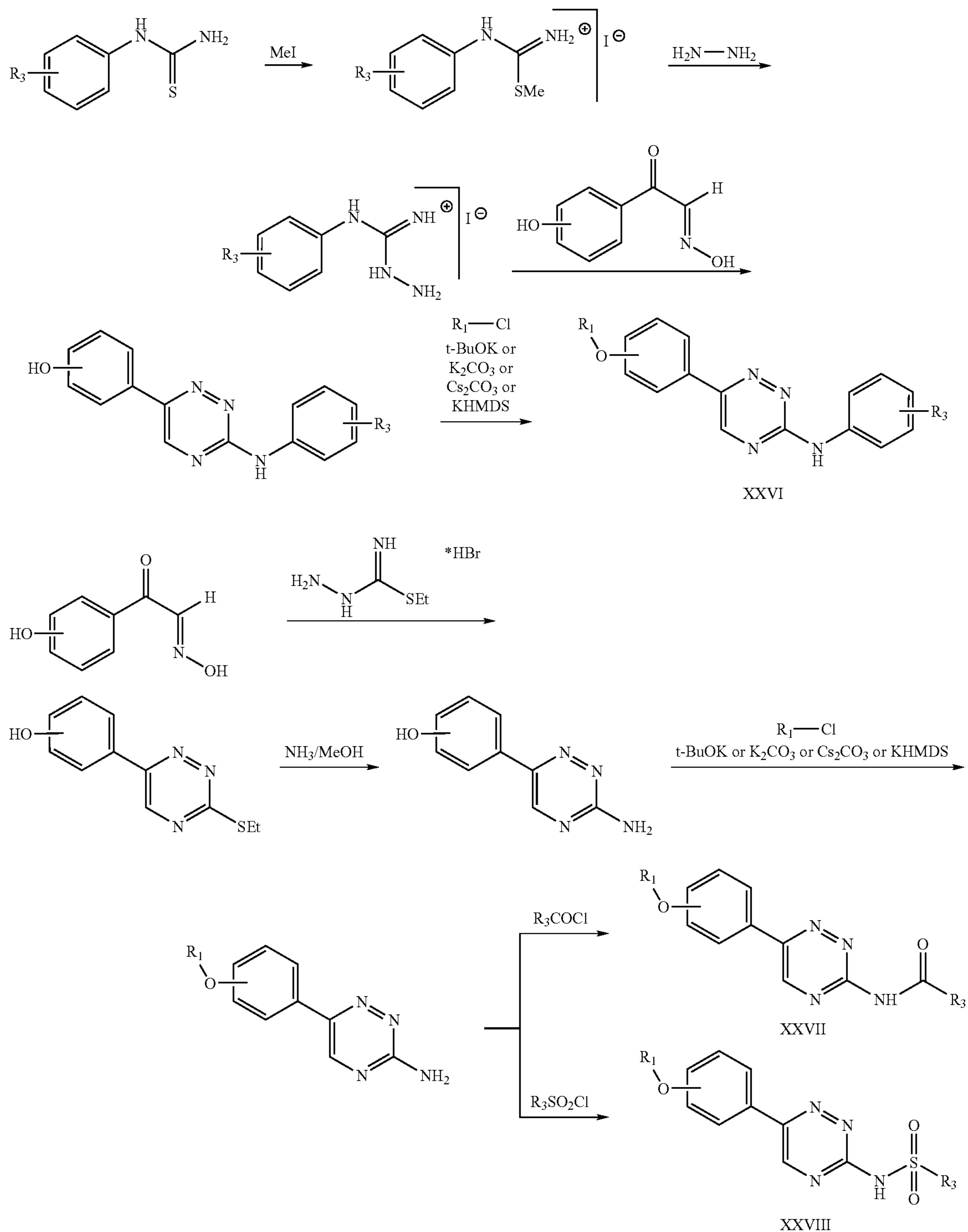
Scheme XVIII
