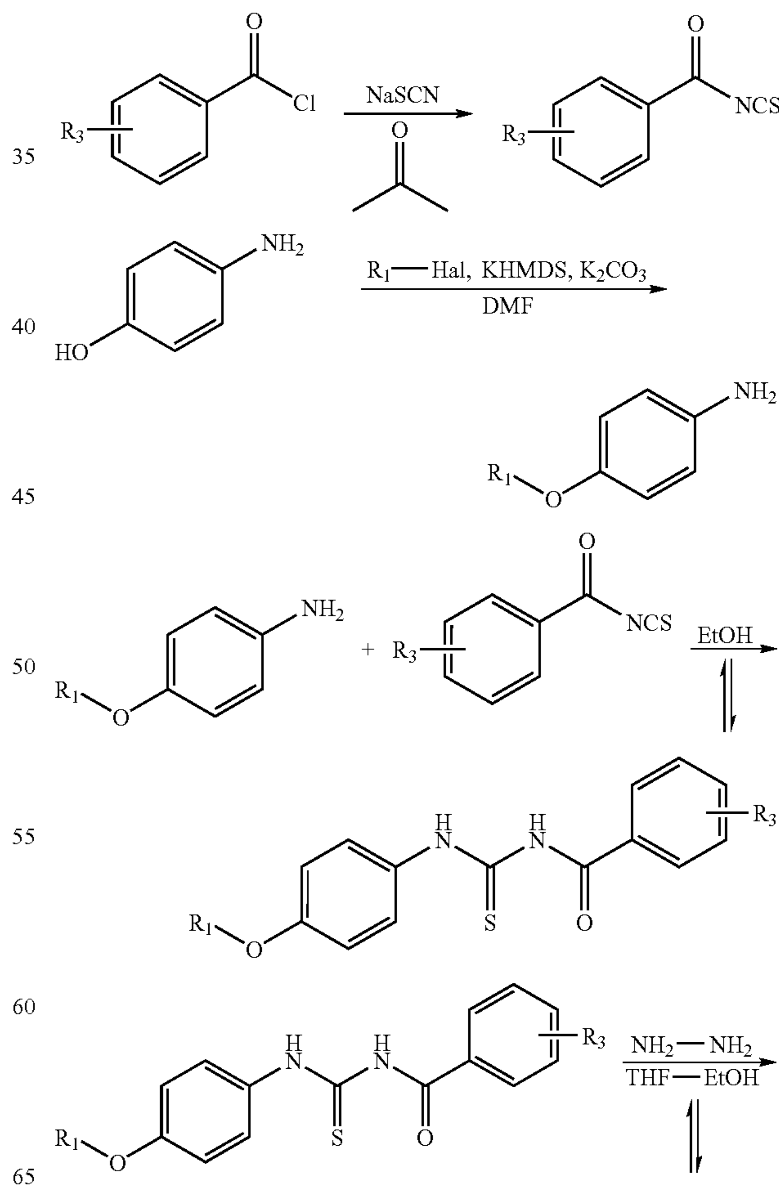
Scheme IX
