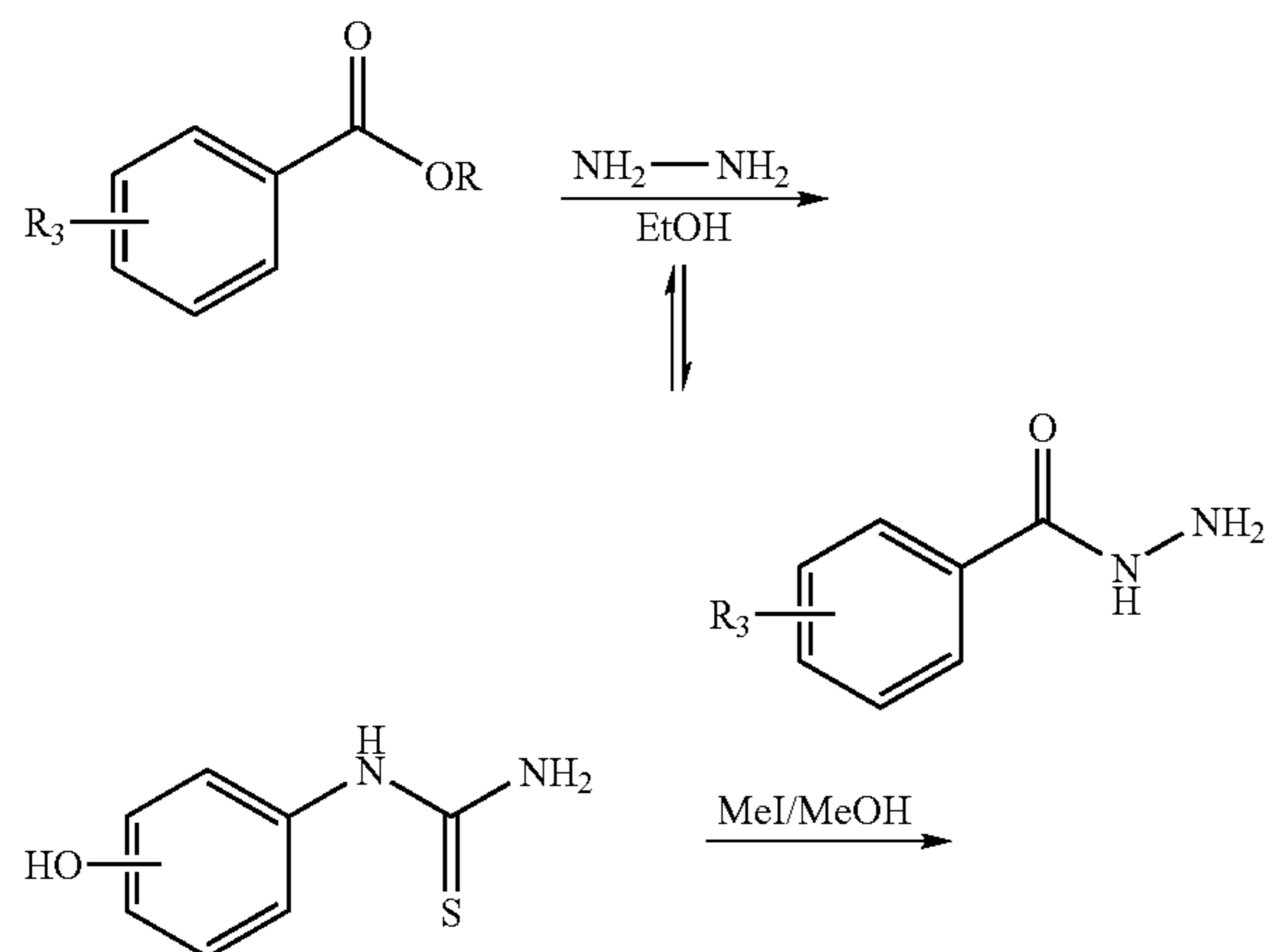
Scheme VIII
