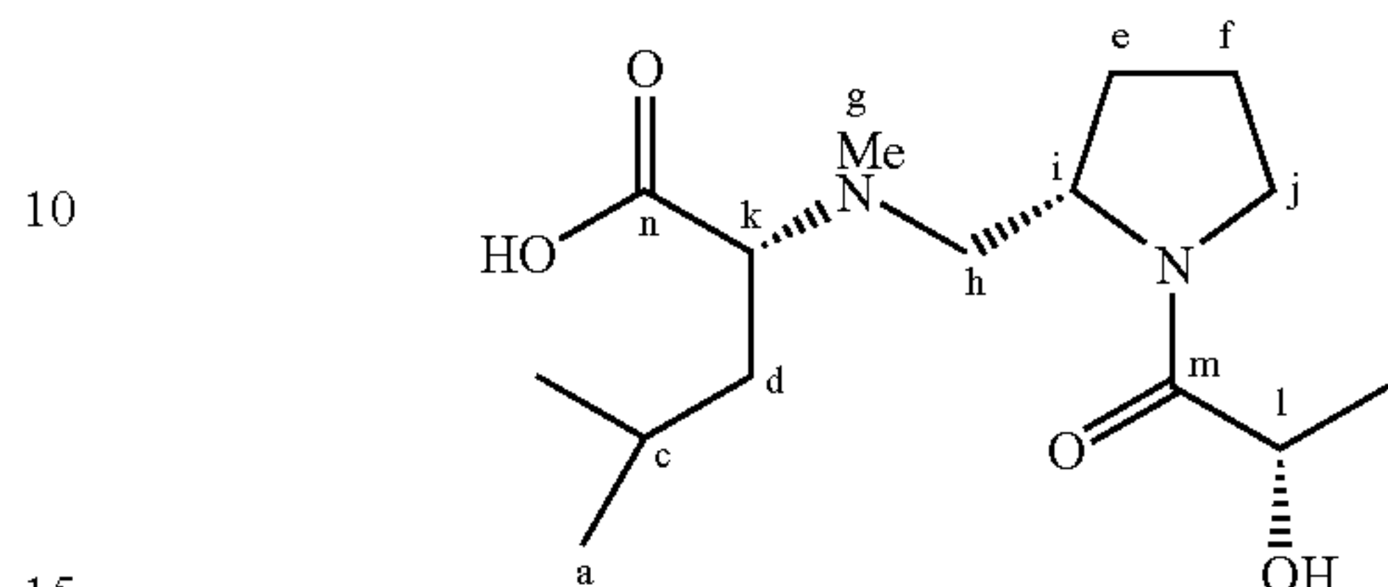
N-Methyl-leu \Psi(\text{NHCH}_2) lac-pro acid (compound 51a )
