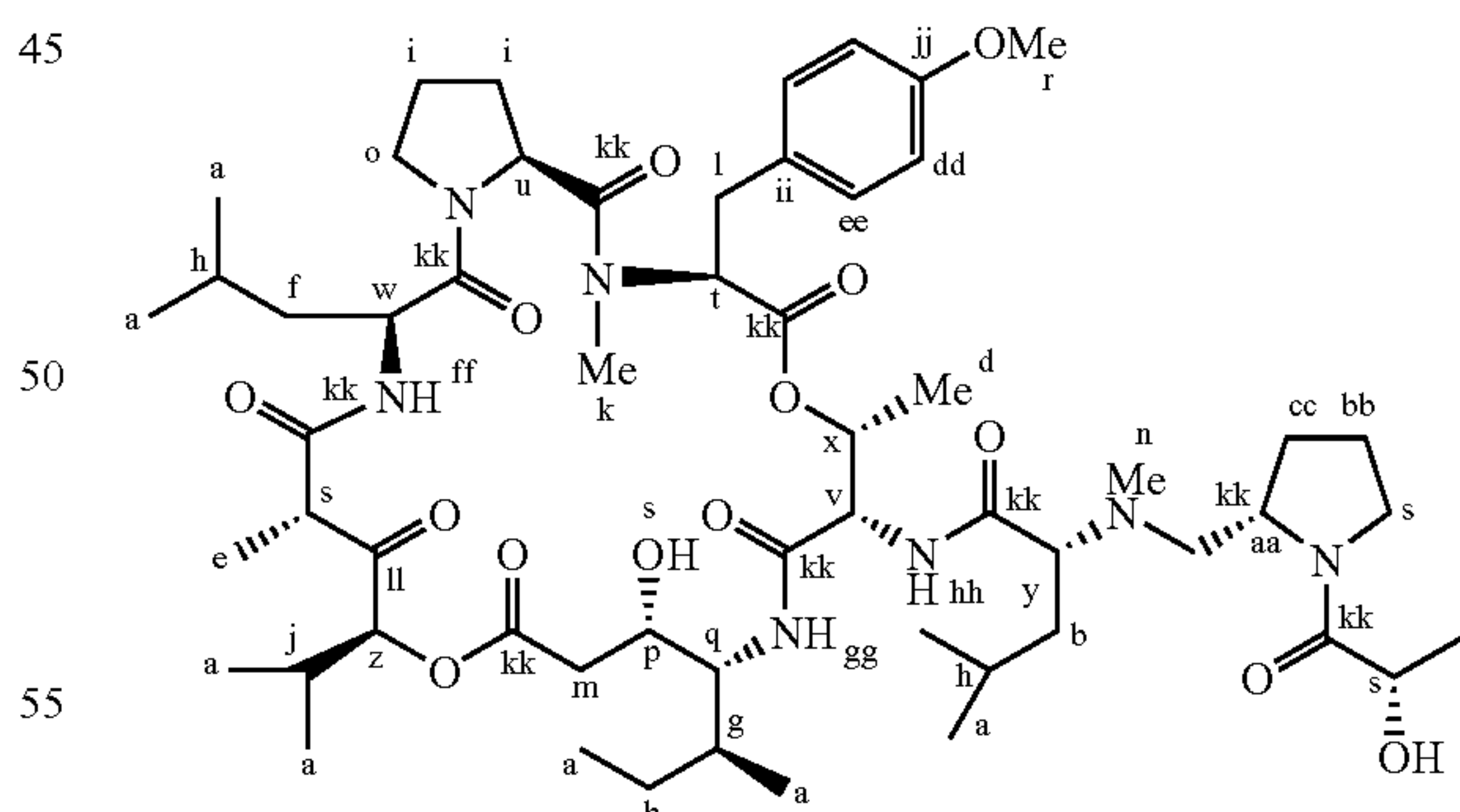
Cyclo[N-(N-3,4-didehydro-L-prolyl-N-methyl-D-leucyl)-O[[N-[(2S,3S,4S)-4-[(3S,4R,5S)-4-amino-3-hydroxy-5-methyl-heptanoyl]oxy-3-oxo-2,5-dimethylhexanoyl]-L-leucyl]-L-prolyl-N,O-dimethyl-L-tyrosyl]-L-threonyl] (compound 72a )
