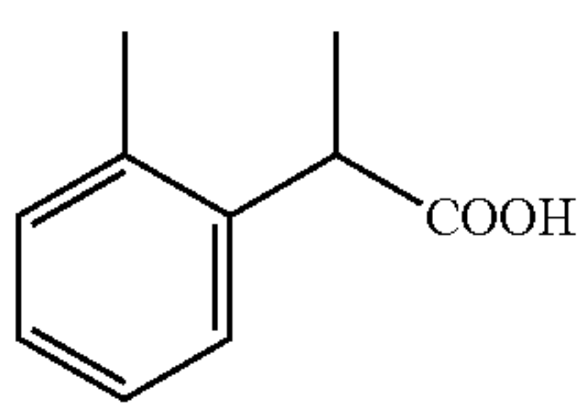
methyl-mandelic acid
