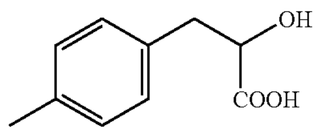
methyl phenyl lactic acid
