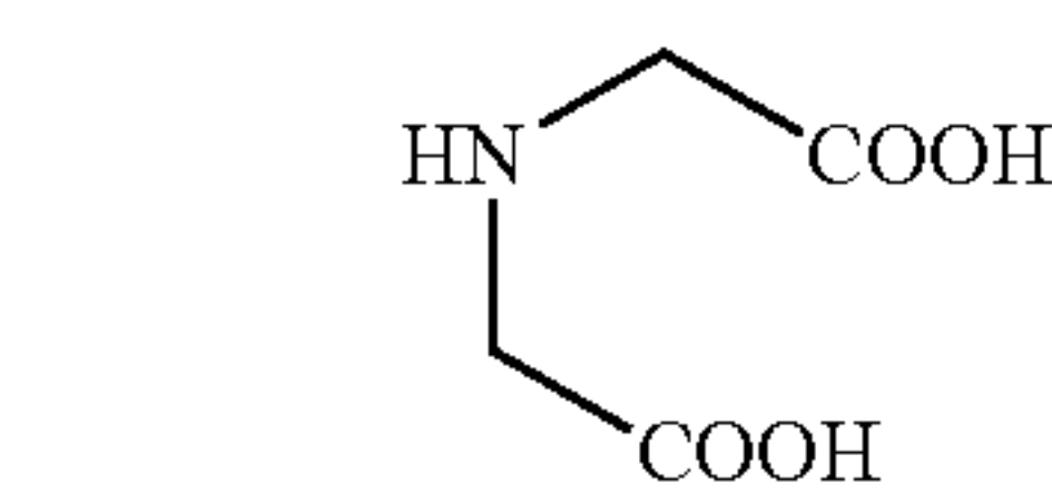
iminodiacetic acid
