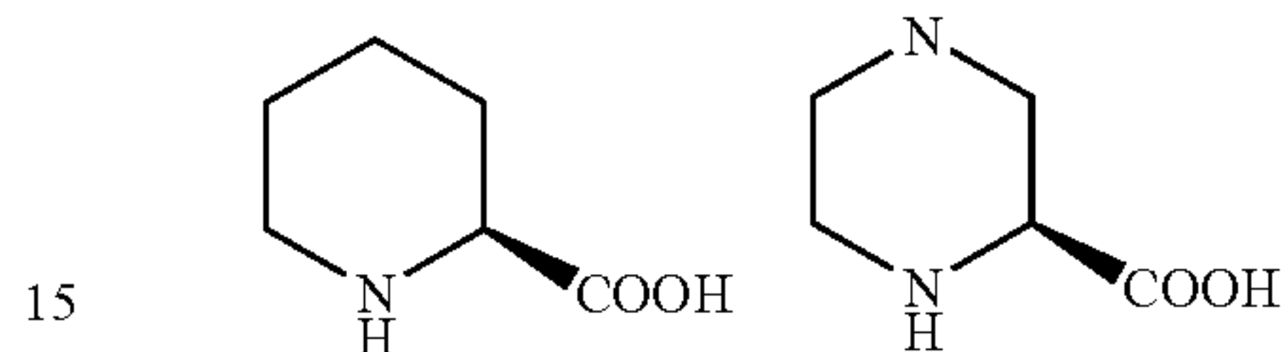
2-carboxy-piperidine
