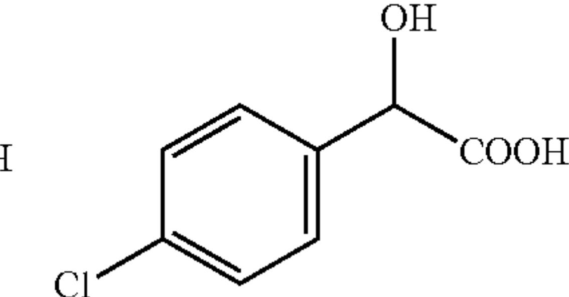
chloro-mandelic acid
