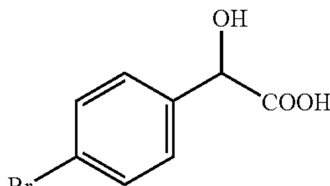
bromo-mandelic acid
