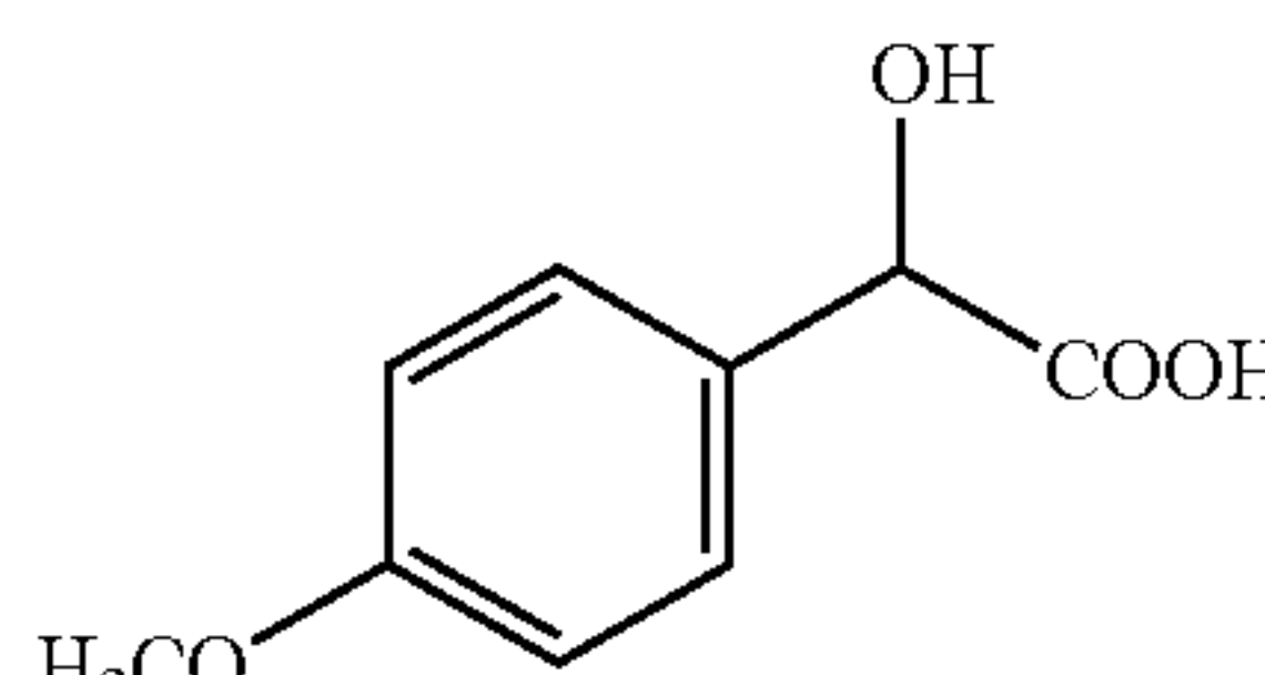
methoxy-mandelic acid
