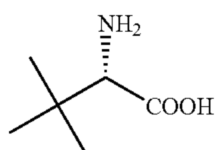
L-tertiary leucine
