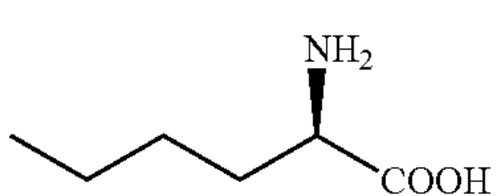
D-norleucine
