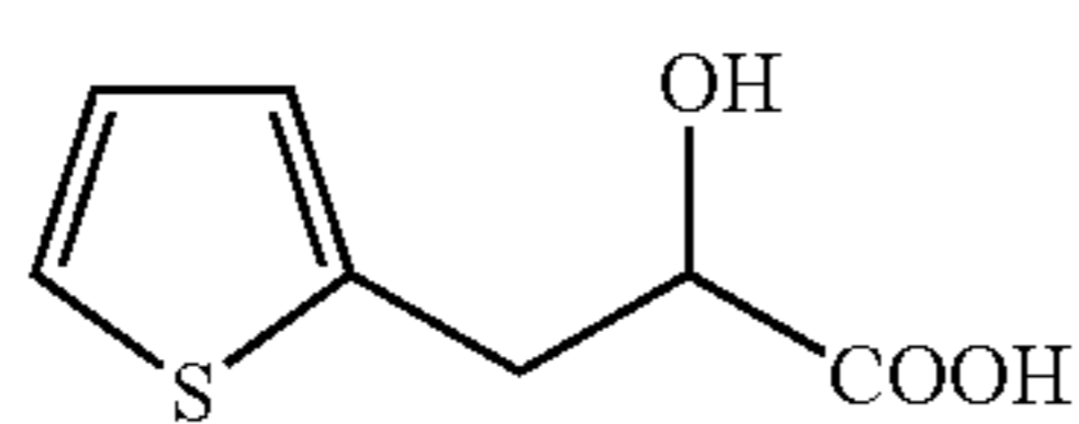
thienyl acetic acid
