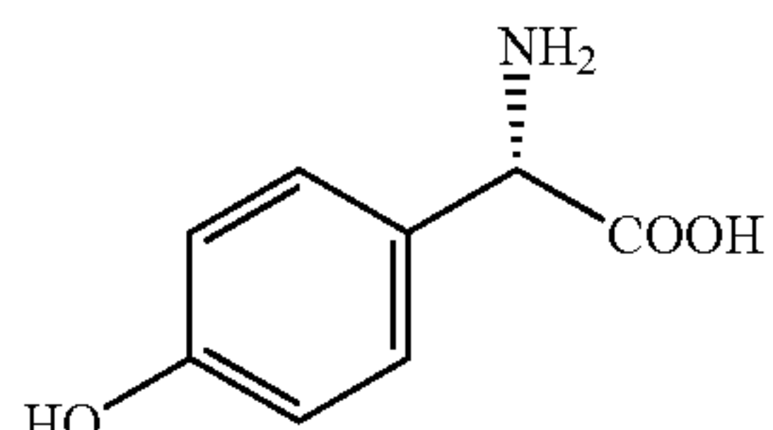
L-4-hydroxyl phenylglycine
