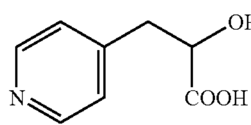
pyridyl acetic acid
