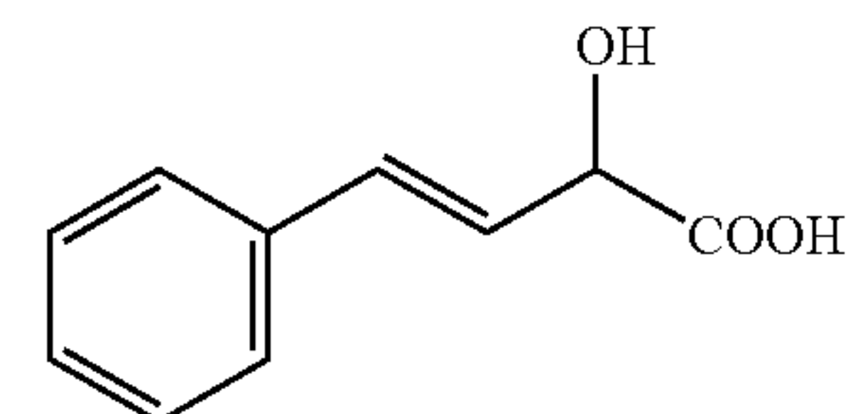
4-phenyl-2-hydroxy-3,4-butenoic acid
