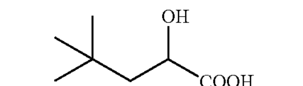
2-hydroxy-4-di-methyl-pentanoic acid
