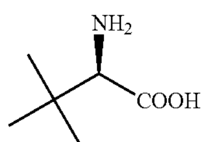
D-tertiary leucine
