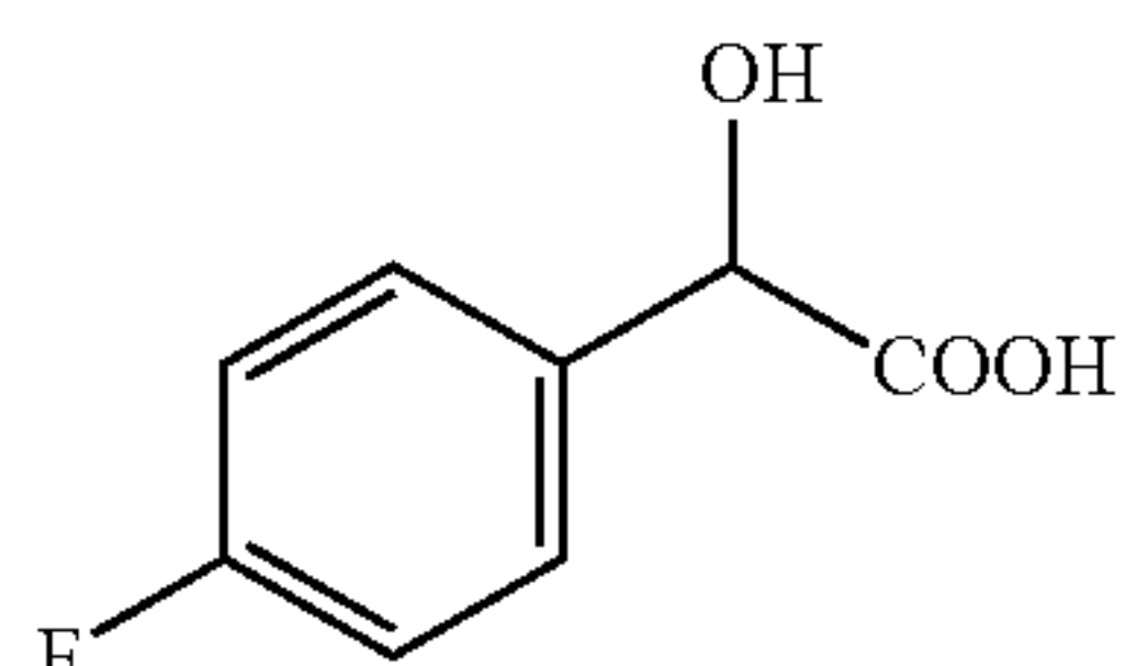
fluoro-mandelic acid
