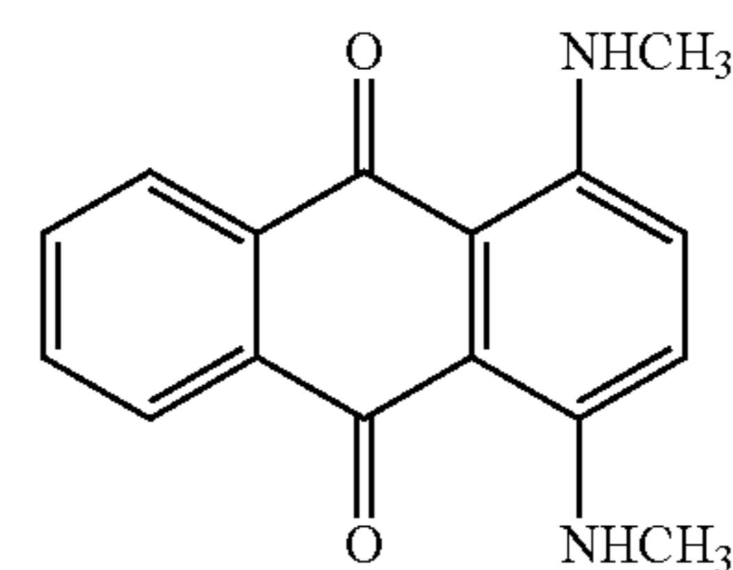
Dye 1 Disperse Blue 14
