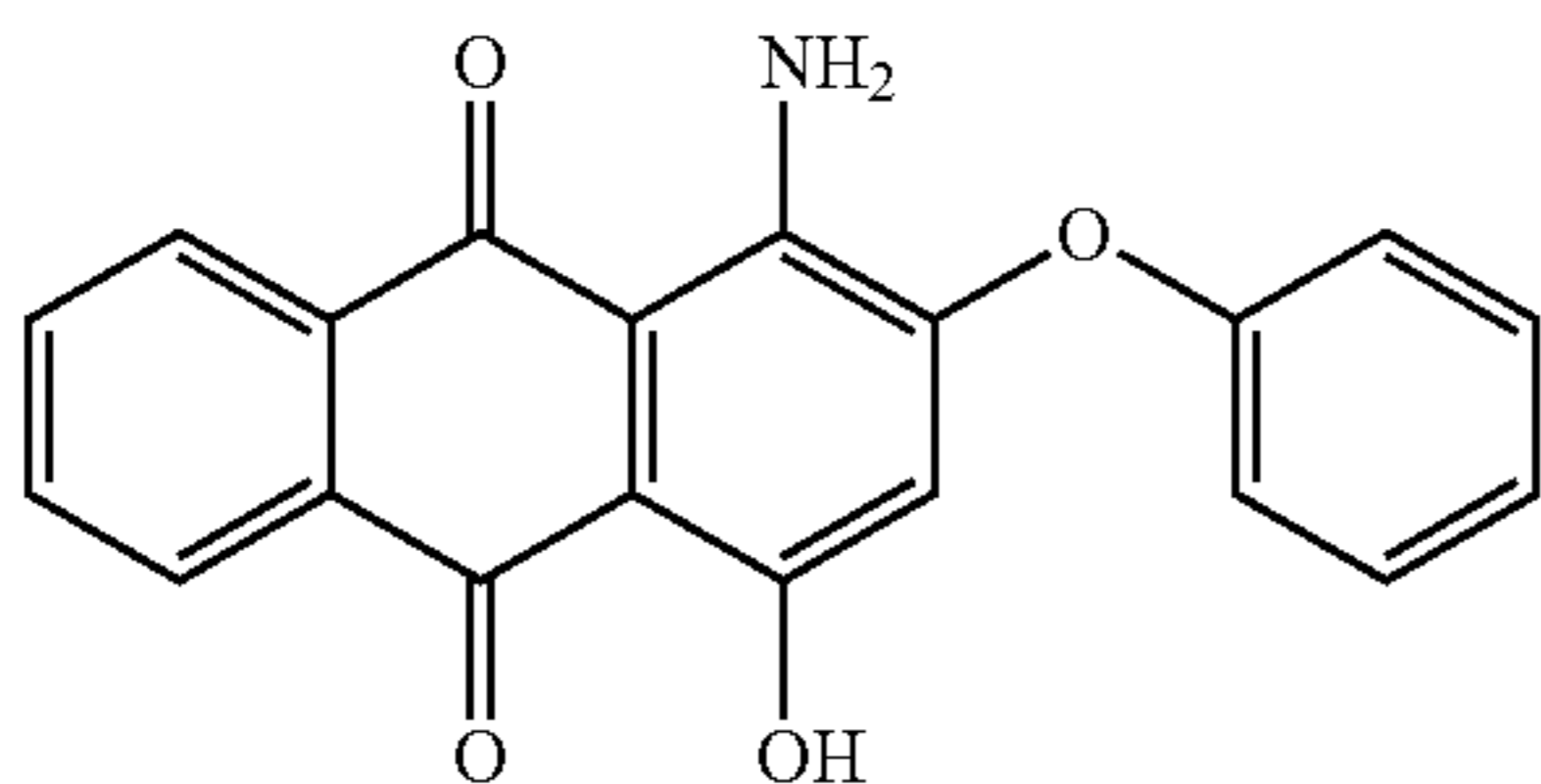
Dye 4 Disperse Red 60
