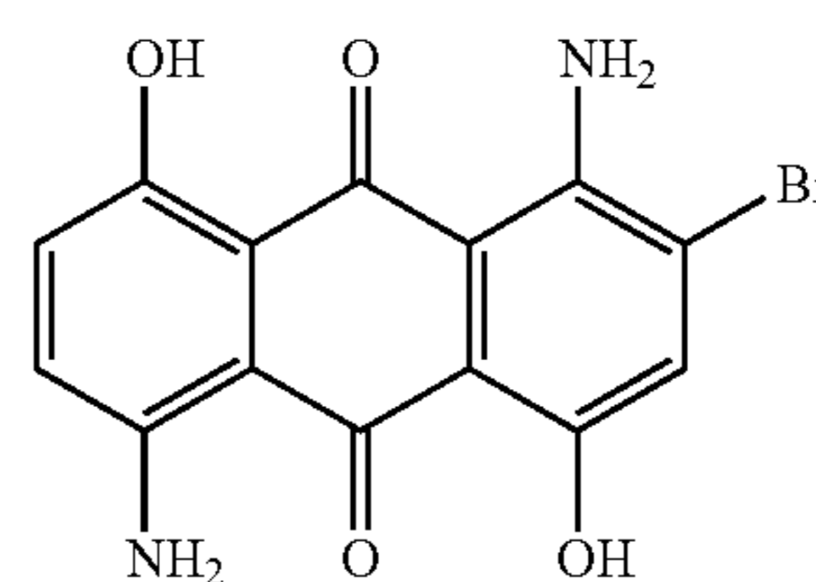
Dye 3 Disperse Blue 56
