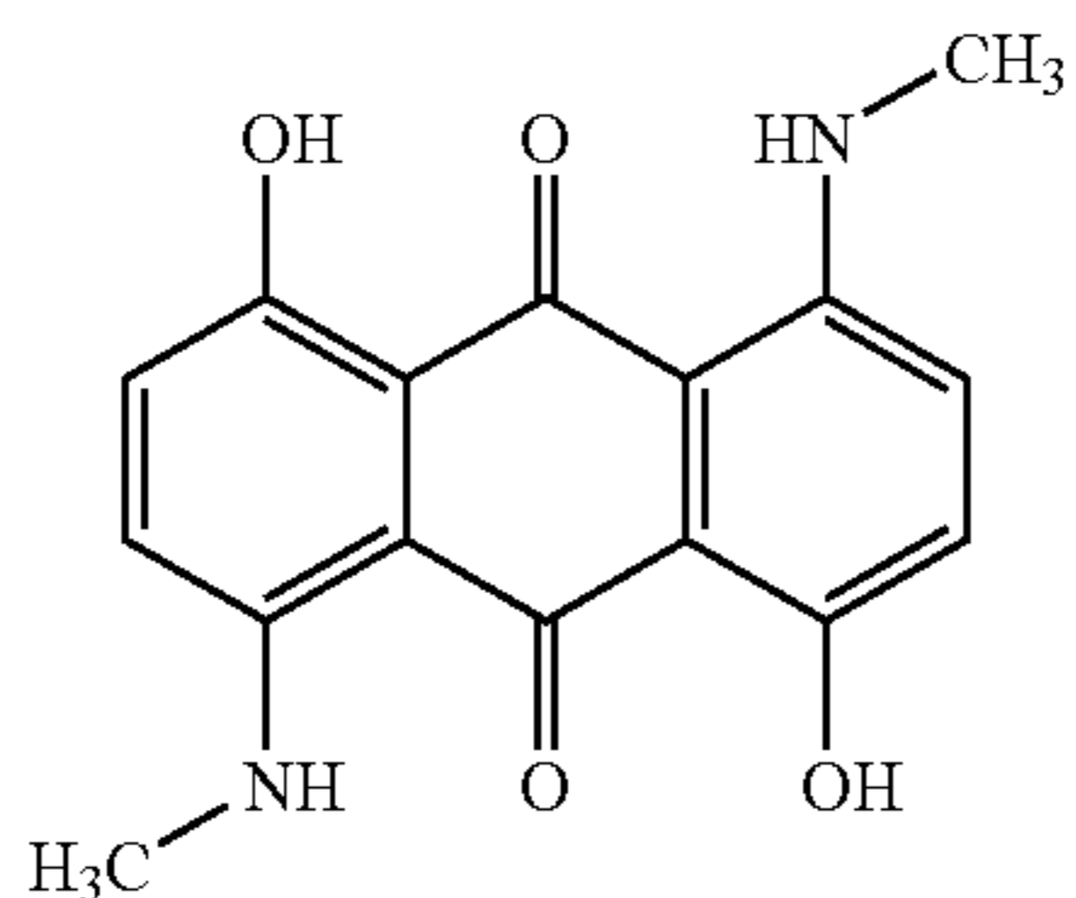
Dye 6 Disperse Blue 26
