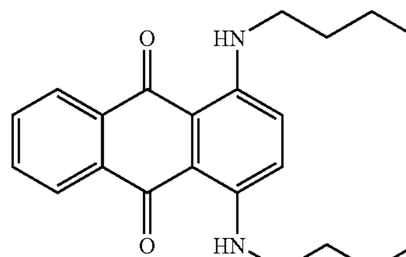
Dye 11 Solvent Blue 35
