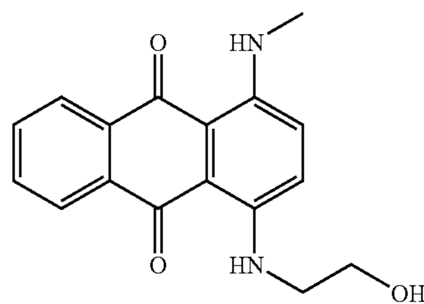
Dye 10 Disperse Blue 3
