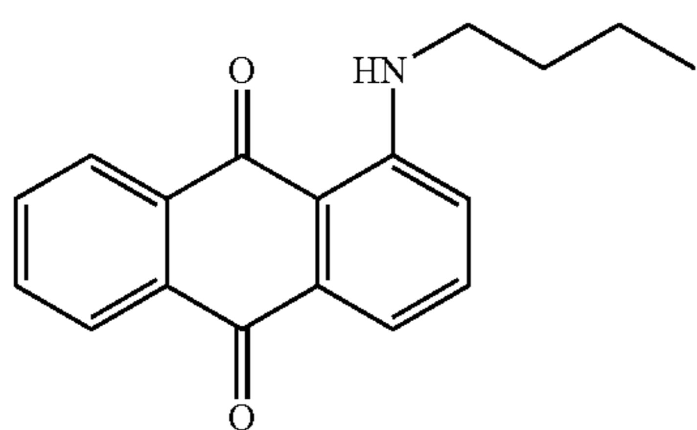
Dye 8 1-N-butyl-anthraquinone
