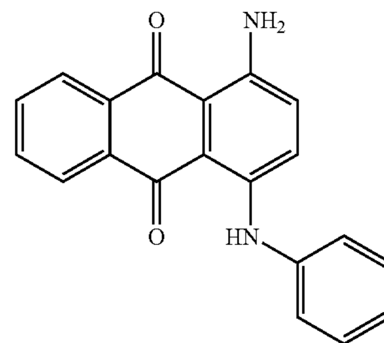
Dye 2 Disperse Blue 19
