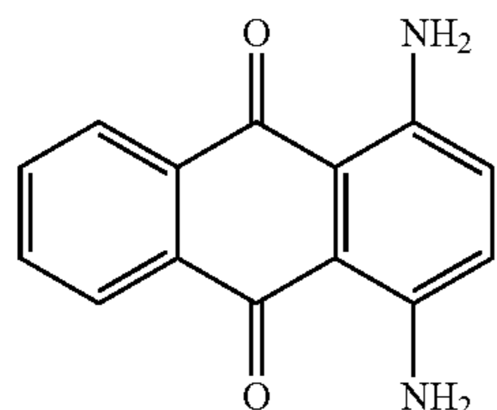
Dye 5 Disperse Violet 1
