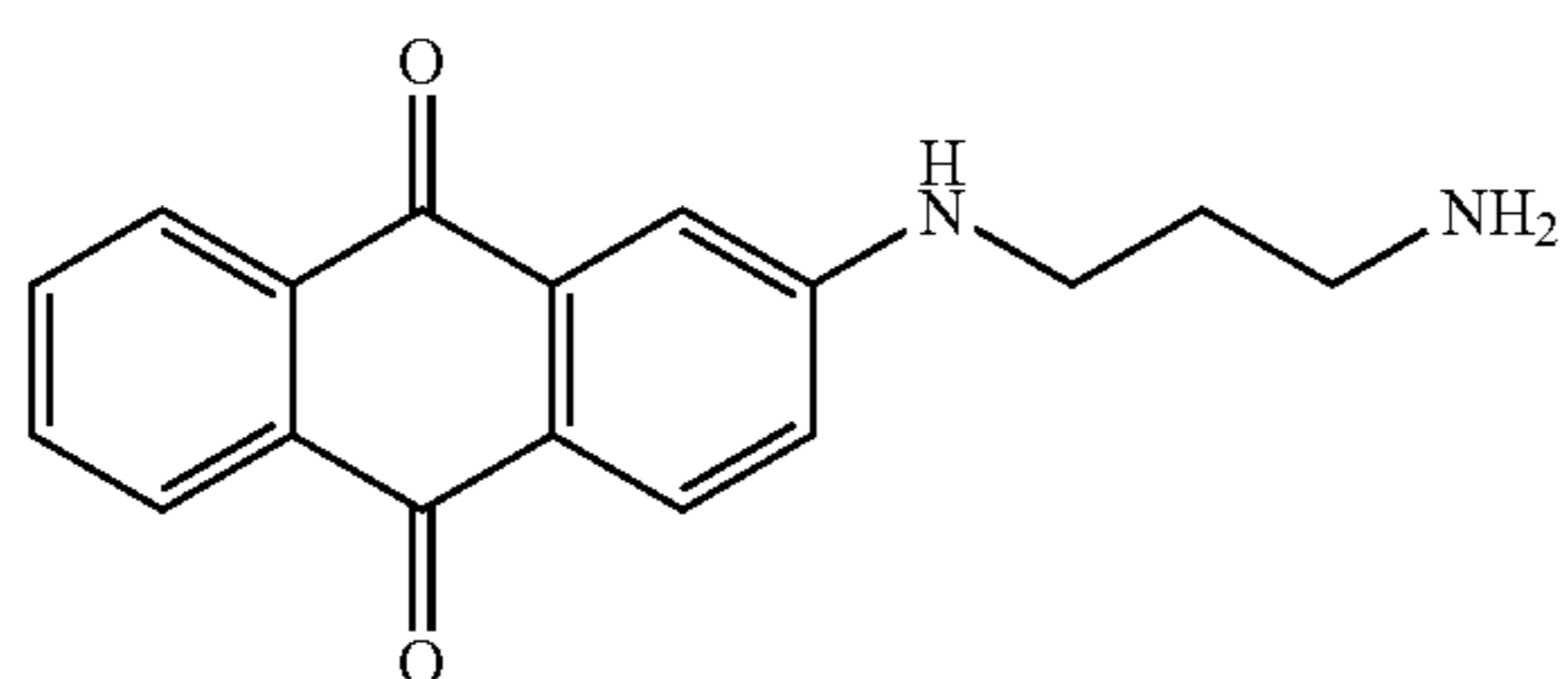
Dye 9 2-N,1-aminobutyl- anthraquinone
