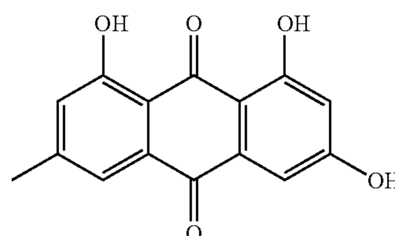
Dye 13 Emodin
