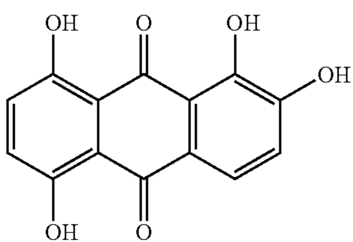
Dye 7 Quinalizarin
