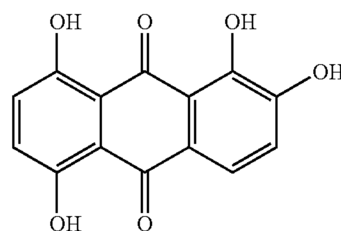
Dye 15 Quinalizarin
