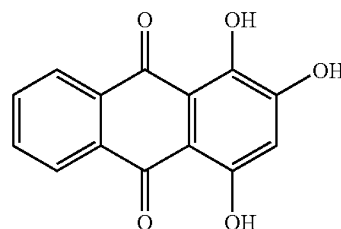
Dye 14 Purpurin
