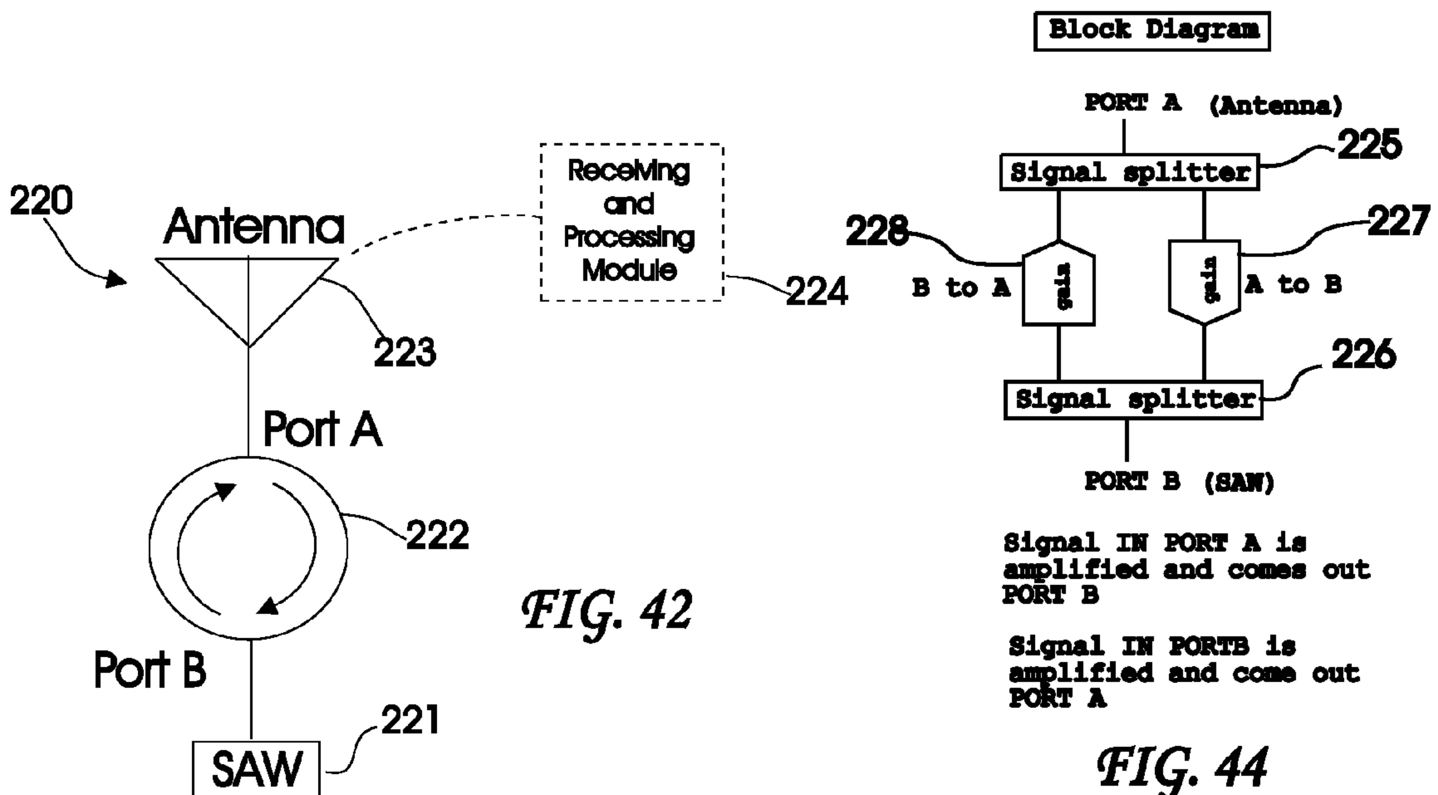
SAW 50 Ohm Antenna 50 Ohm
