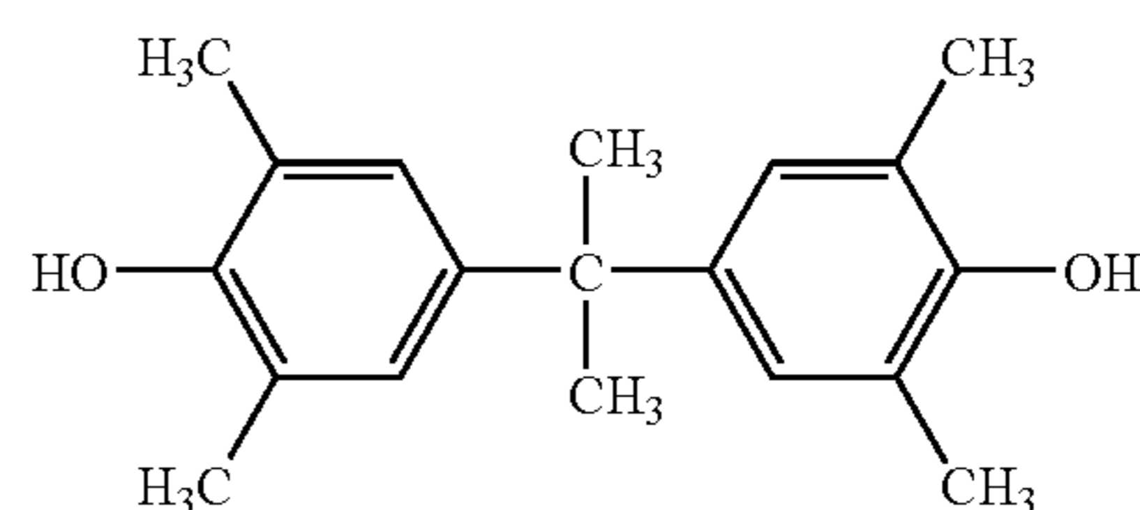
(Chemical Formula 11J) 15
