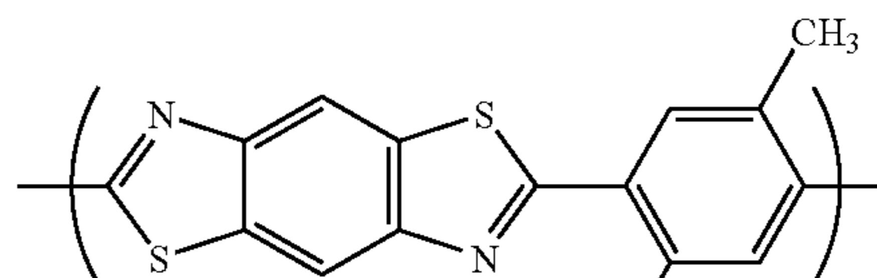
(Chemical Formula 26-6)
