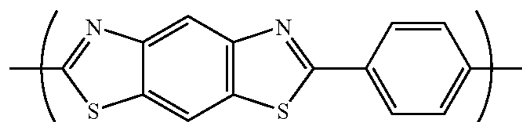
(Chemical Formula 25-2)
