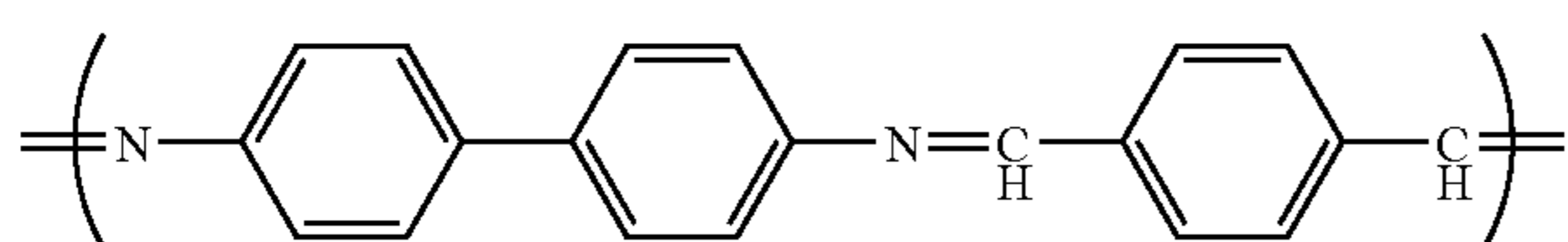
(Chemical Formula 45-5)
