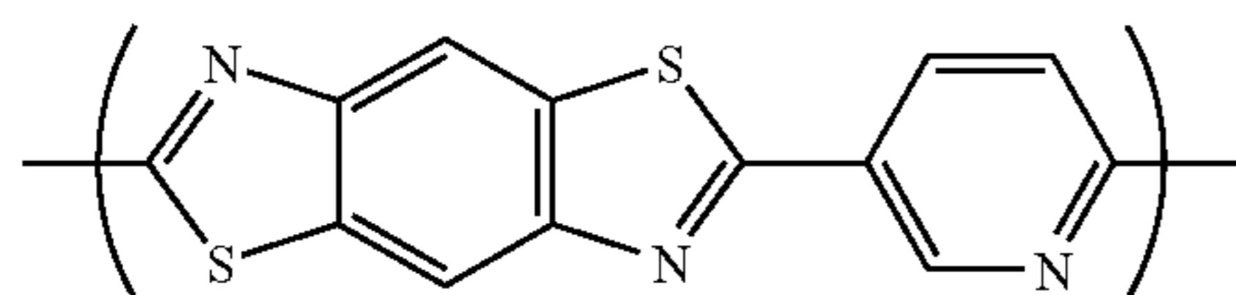
(Chemical Formula 25-7)
