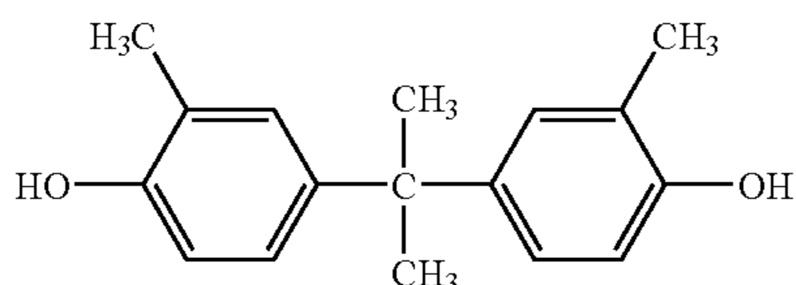
(Chemical Formula 19B)
