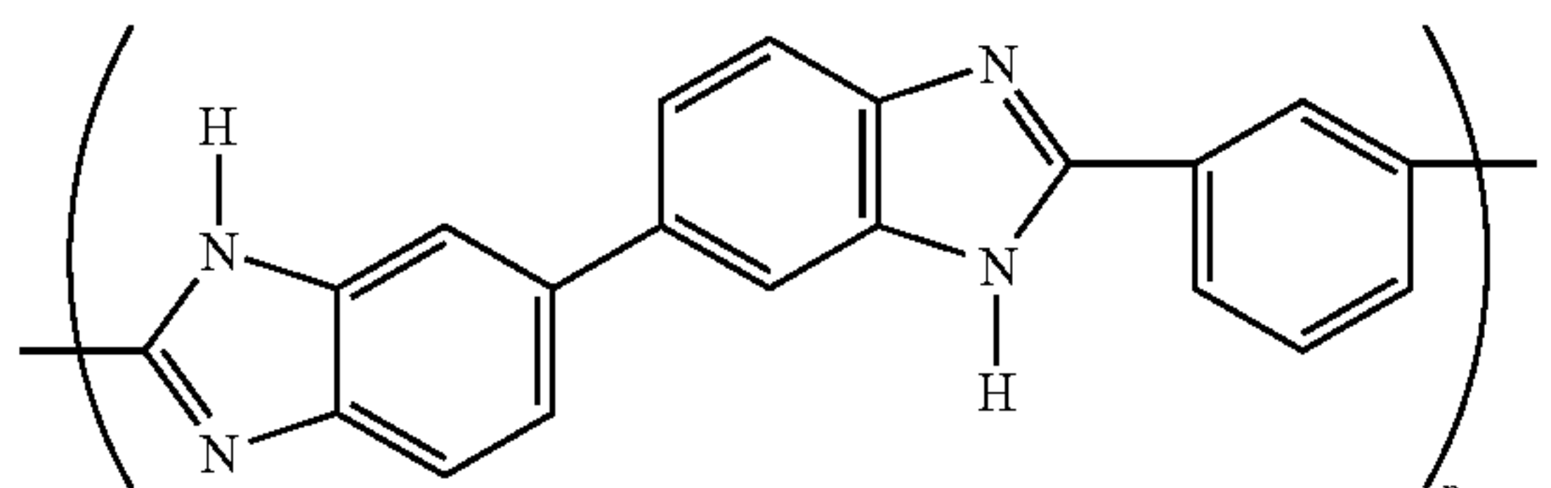
(Chemical Formula 27-3)
