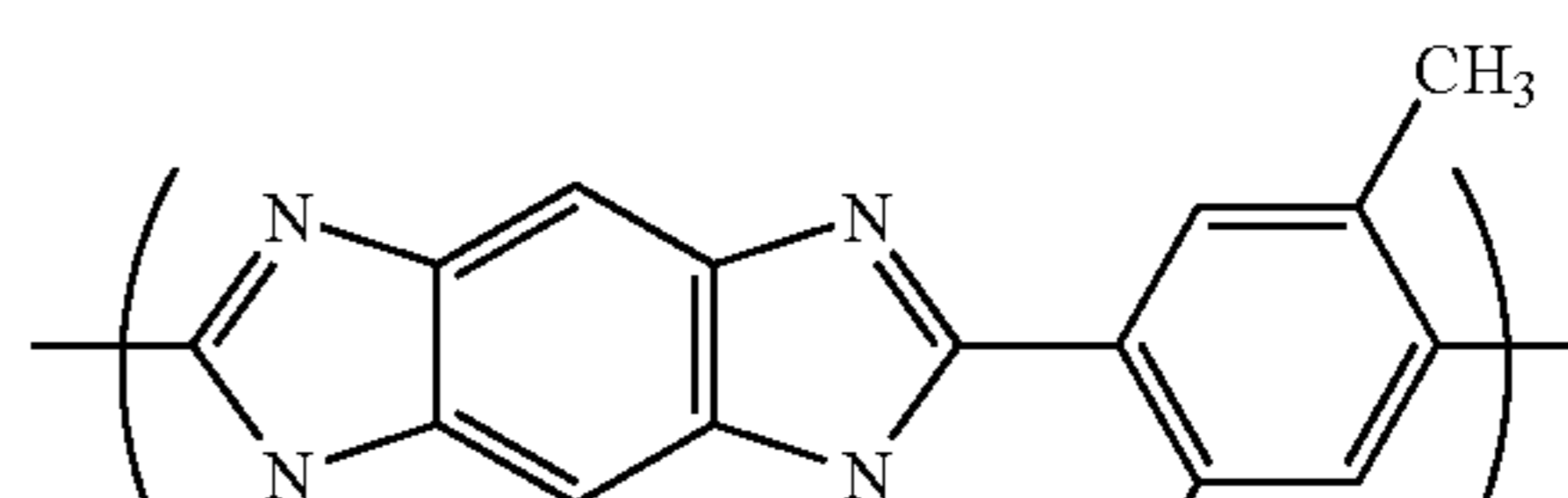
(Chemical Formula 26-7)
