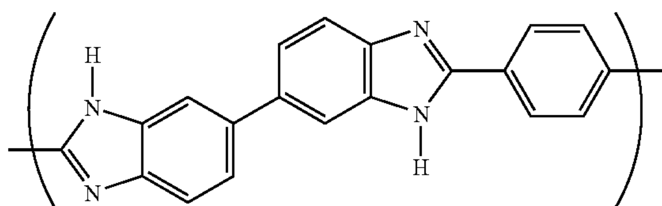
(Chemical Formula 27-2)
