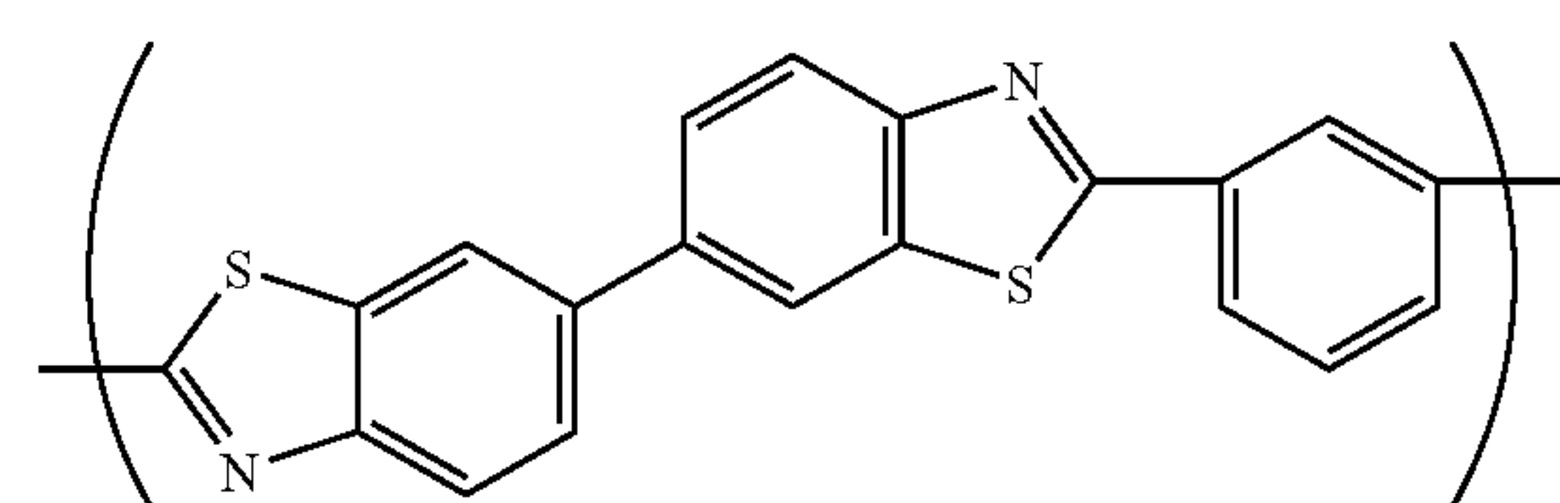
(Chemical Formula 27-7)
