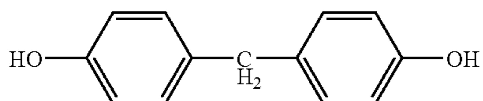
(Chemical Formula 11E) 40
