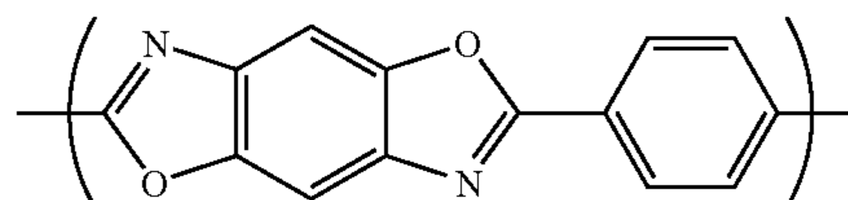
(Chemical Formula 26-1)
