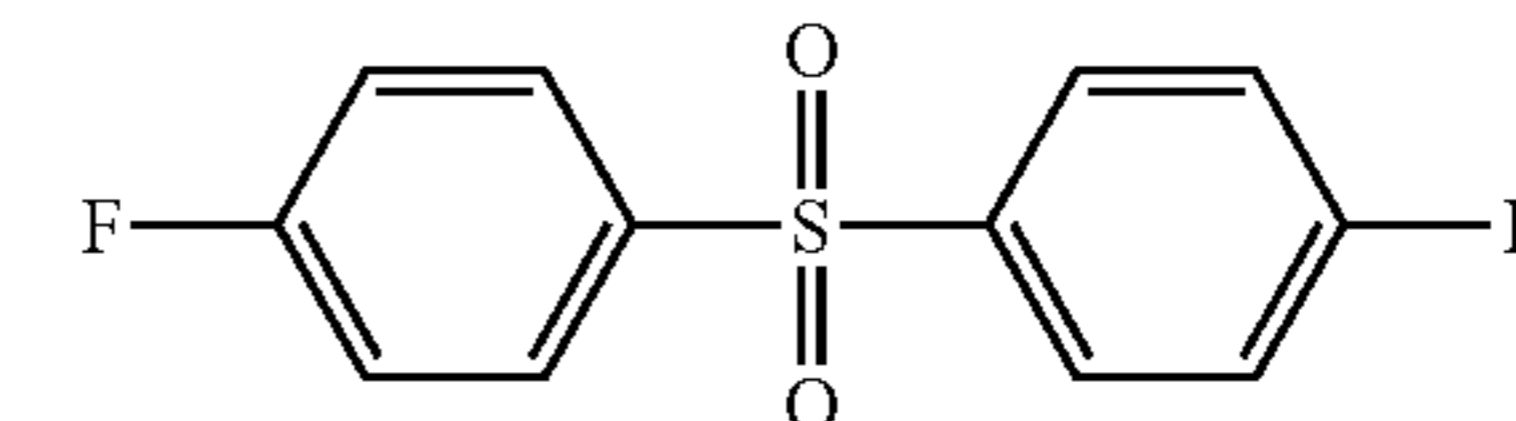
(Chemical Formula 10E)
