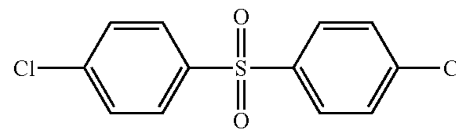
(Chemical Formula 10B)
