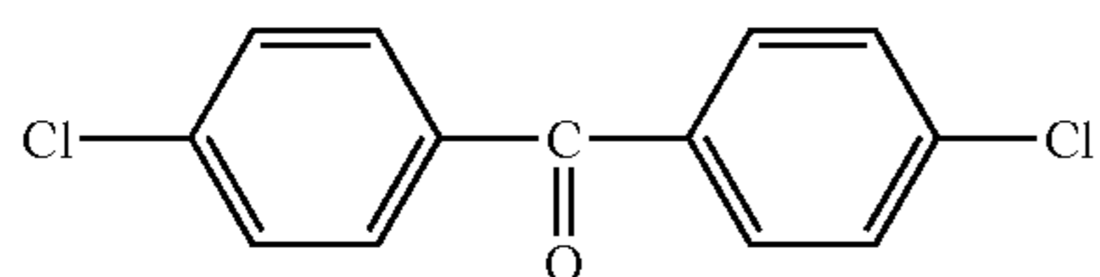
(Chemical Formula 18B)
