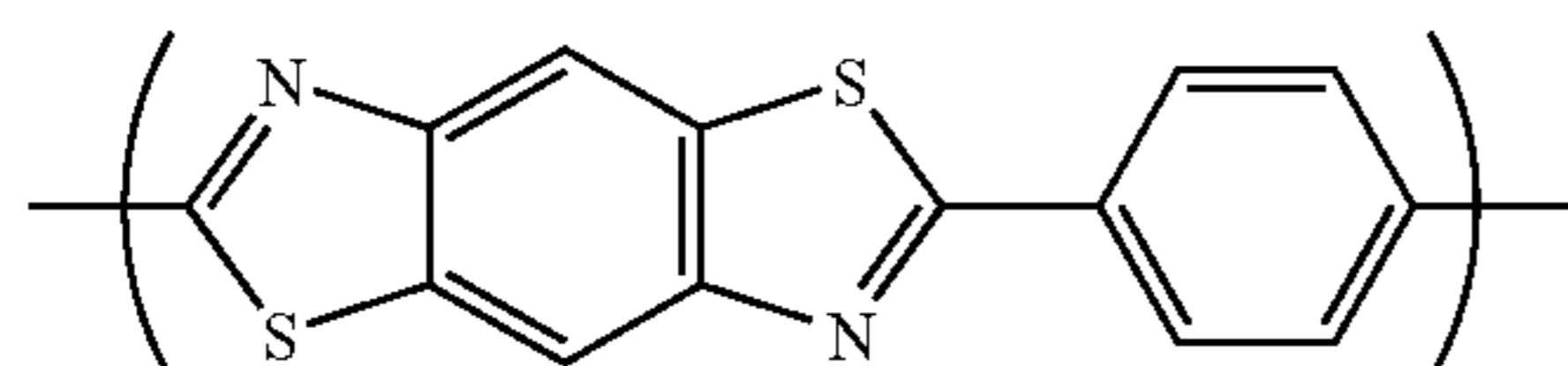
(Chemical Formula 25-3)
