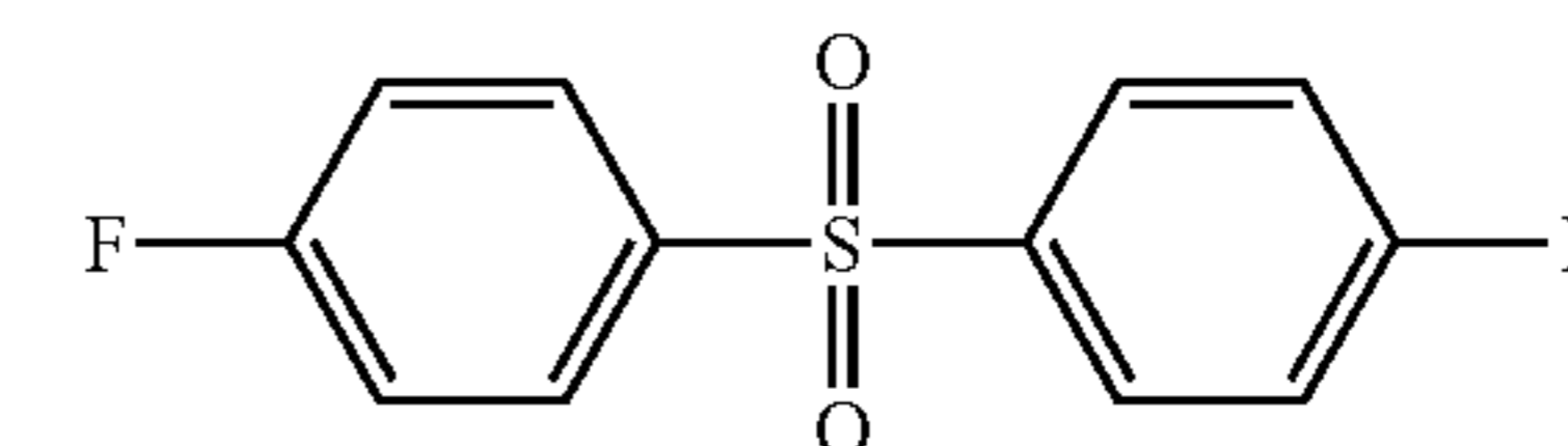
(Chemical Formula 10E)
