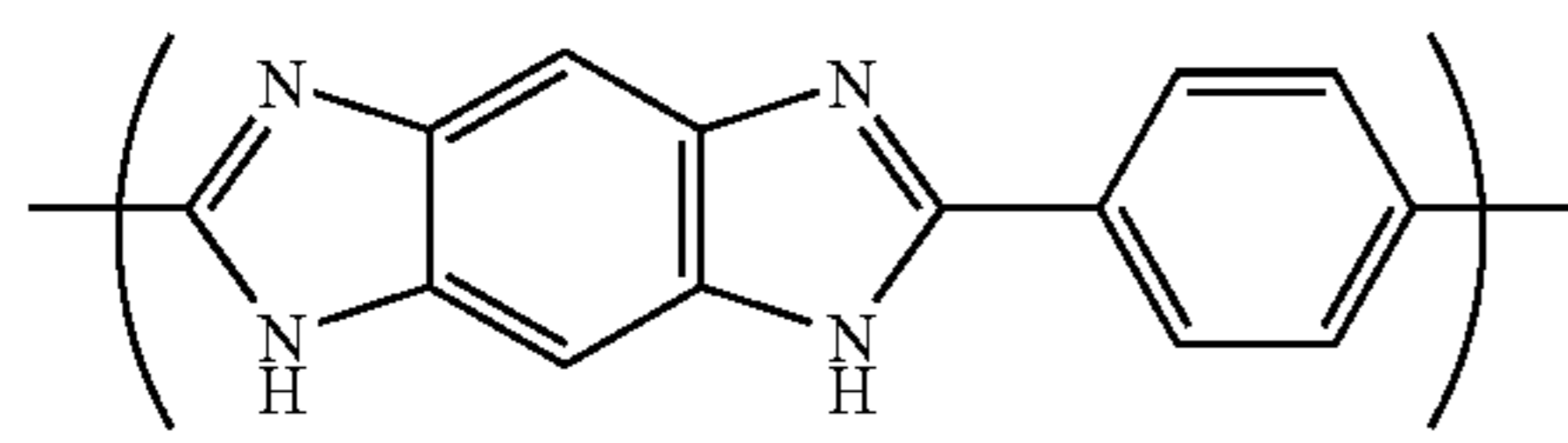
(Chemical Formula 25-4)
