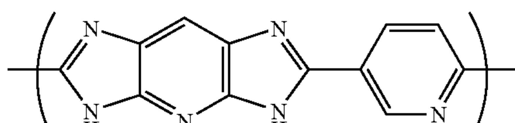
(Chemical Formula 25-9)
