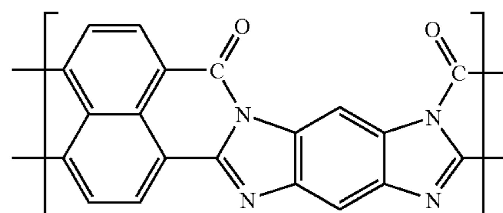
(Chemical Formula 47-2)
