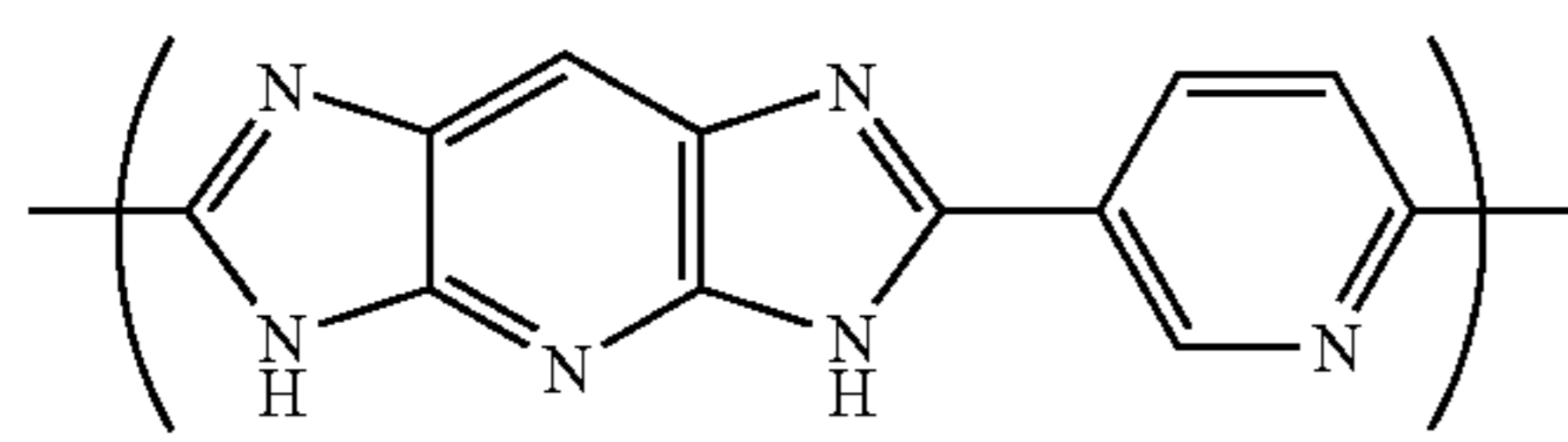
(Chemical Formula 25-9)
