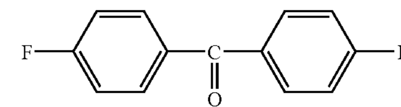
(Chemical Formula 10F)
