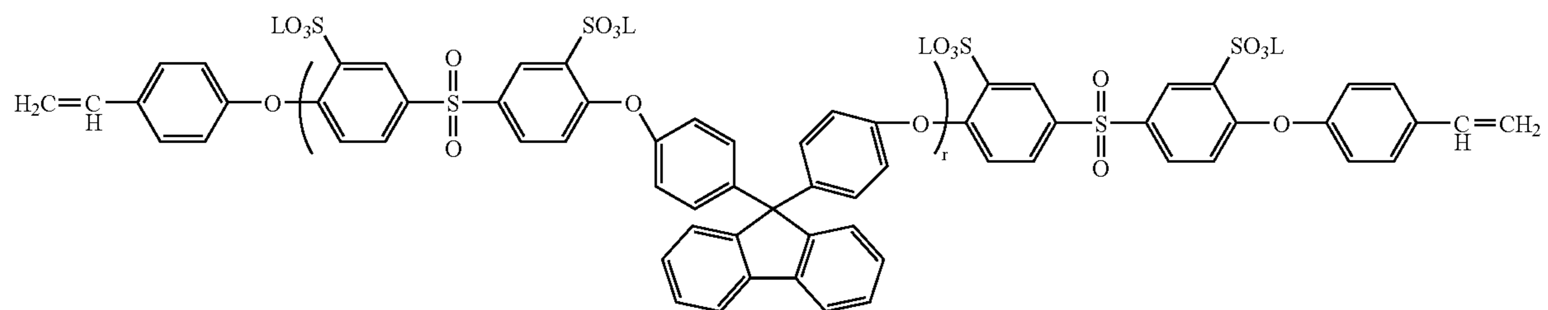
(Chemical Formula 20G)
