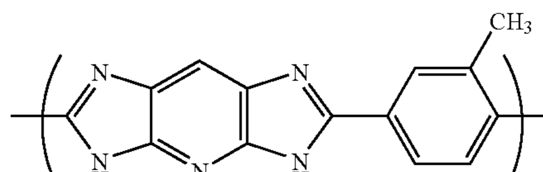
(Chemical Formula 26-4)
