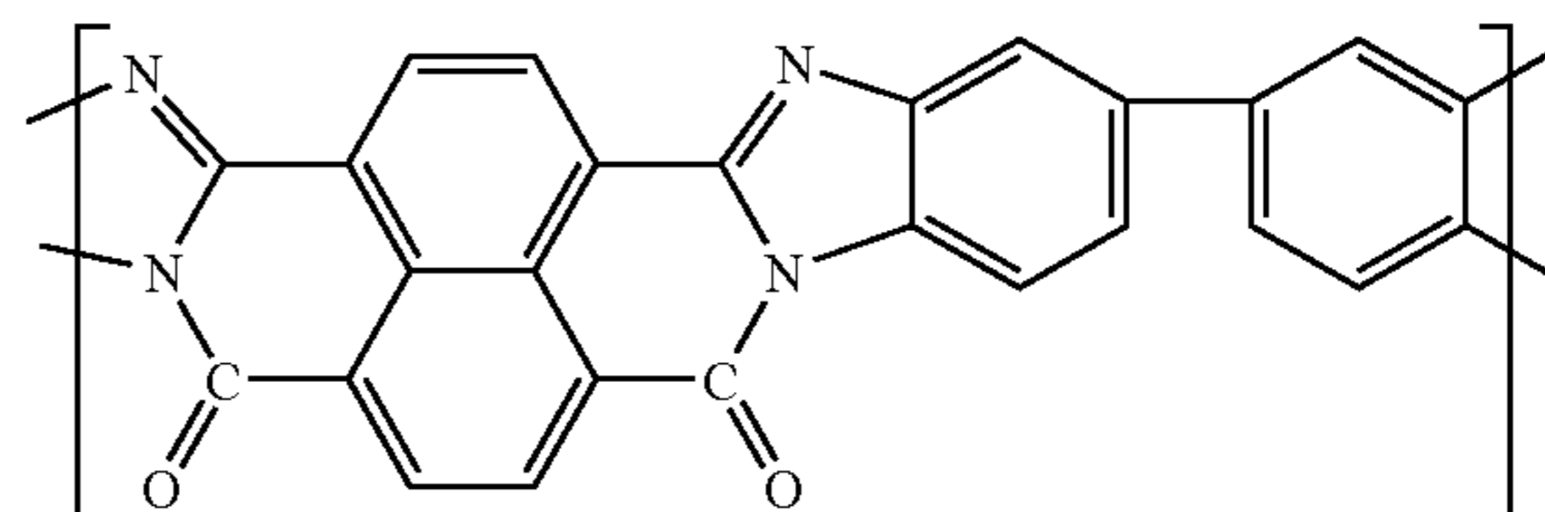
(Chemical Formula 47-2)
