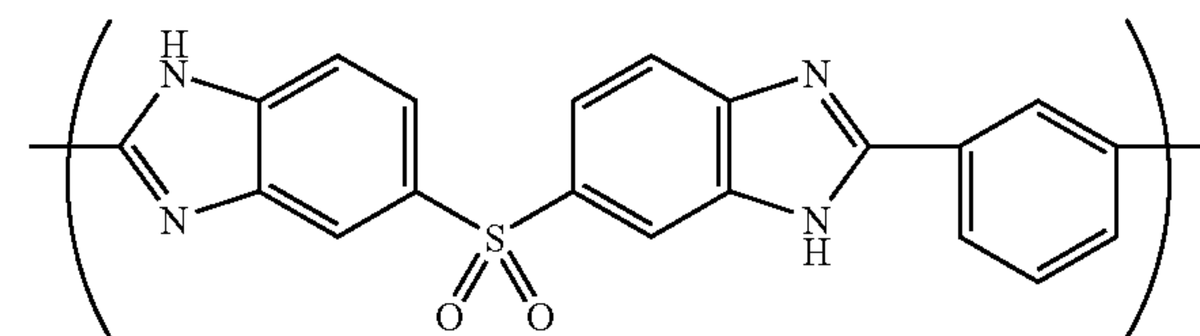
(Chemical Formula 27-9)
