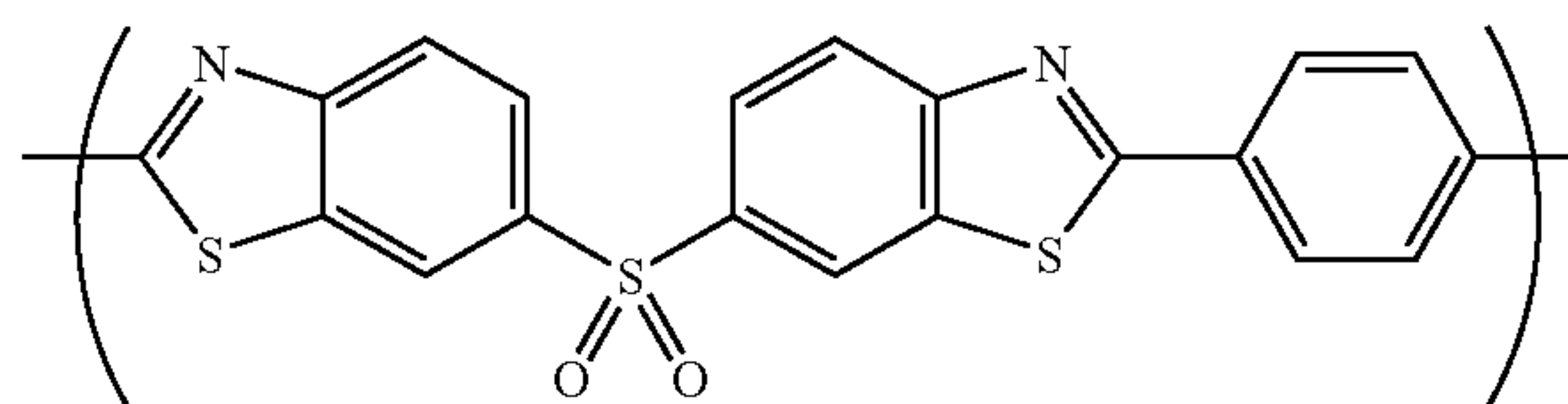
(Chemical Formula 27-12)
