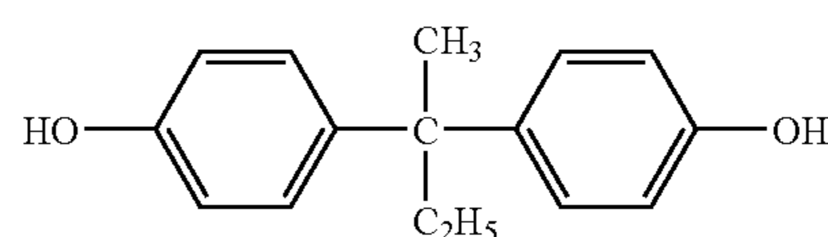
(Chemical Formula 11N) 35
