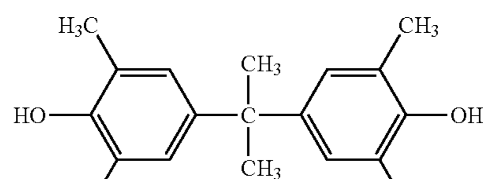
(Chemical Formula 19C)
