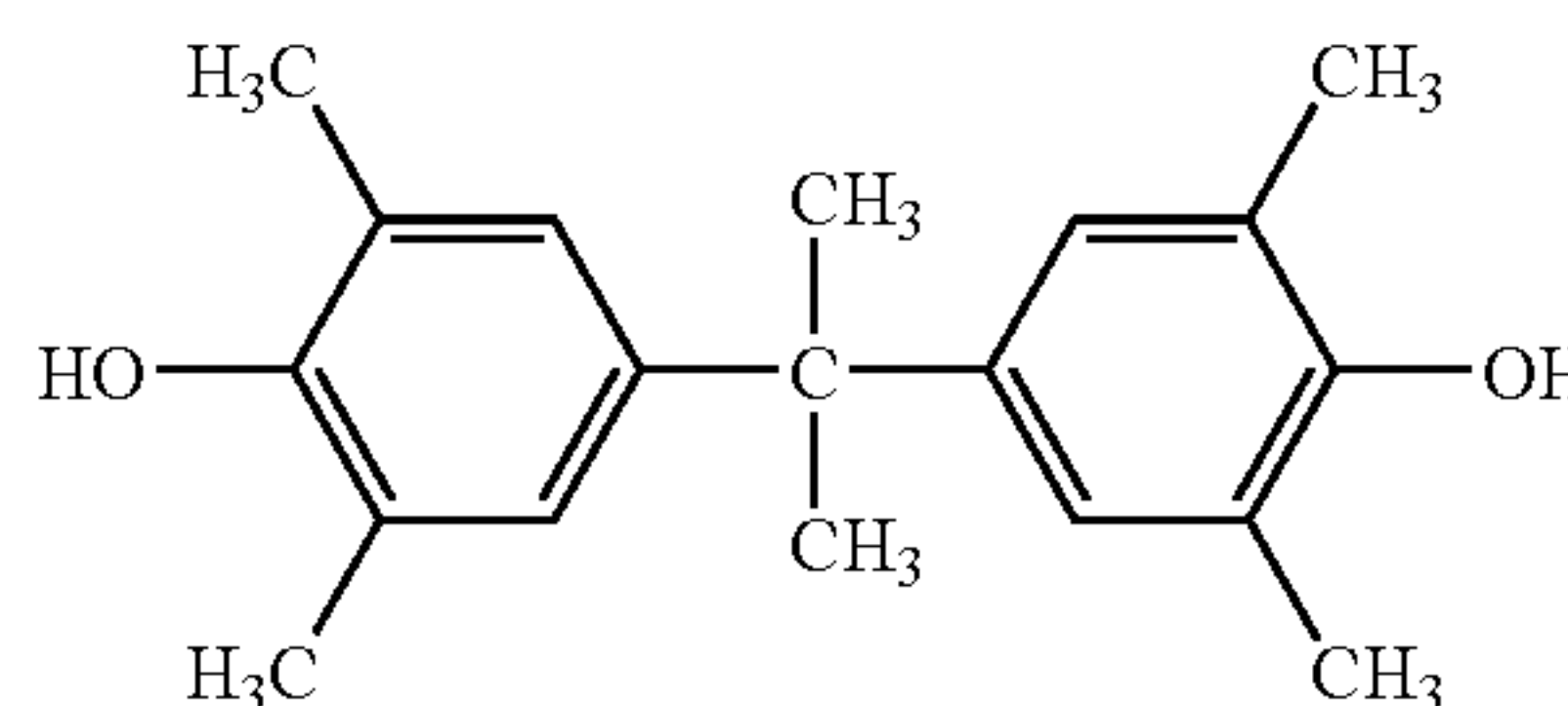
(Chemical Formula 11J)
