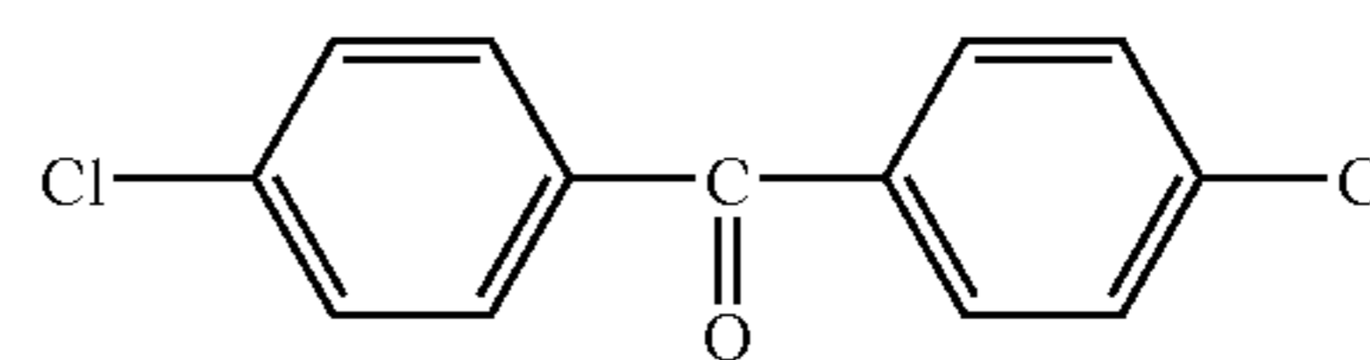
(Chemical Formula 10C)
