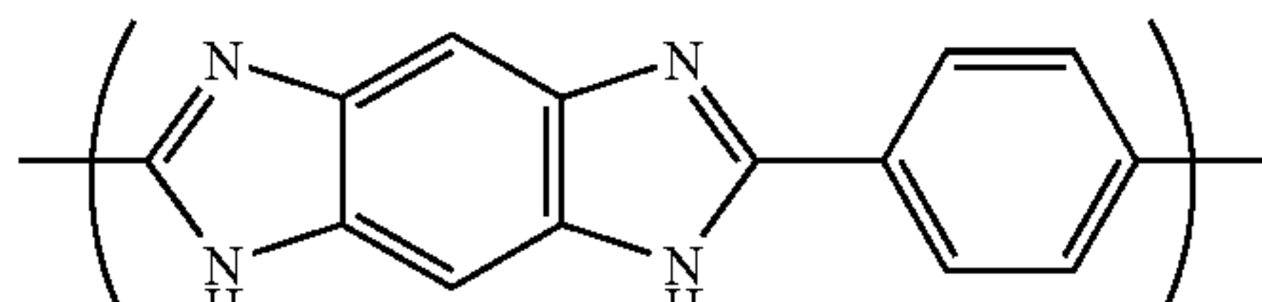
(Chemical Formula 25-4)
