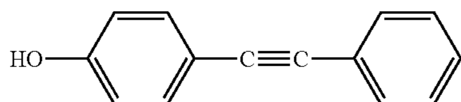
(Chemical Formula 16C)
