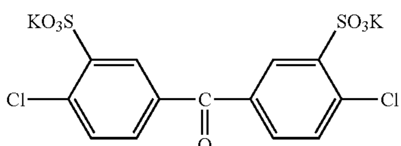
(Chemical Formula 9C)
