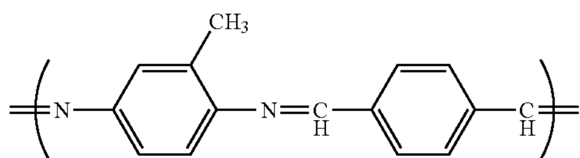
(Chemical Formula 45-3)
