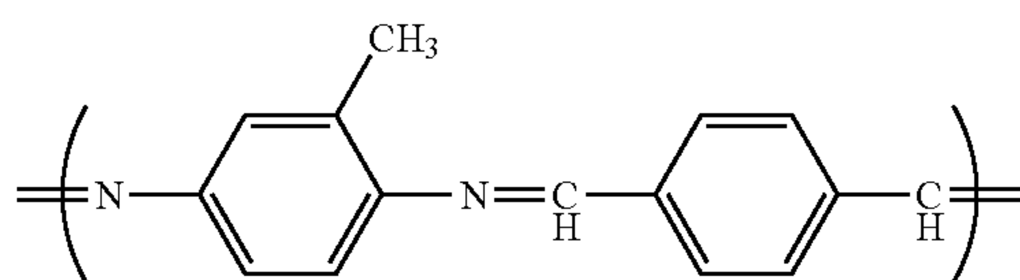
(Chemical Formula 45-3)
