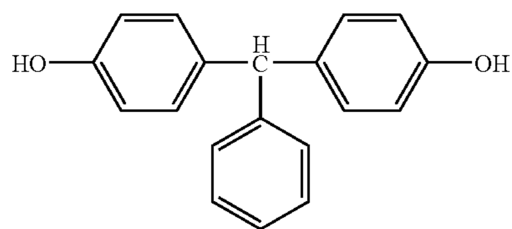
(Chemical Formula 11F) 45
