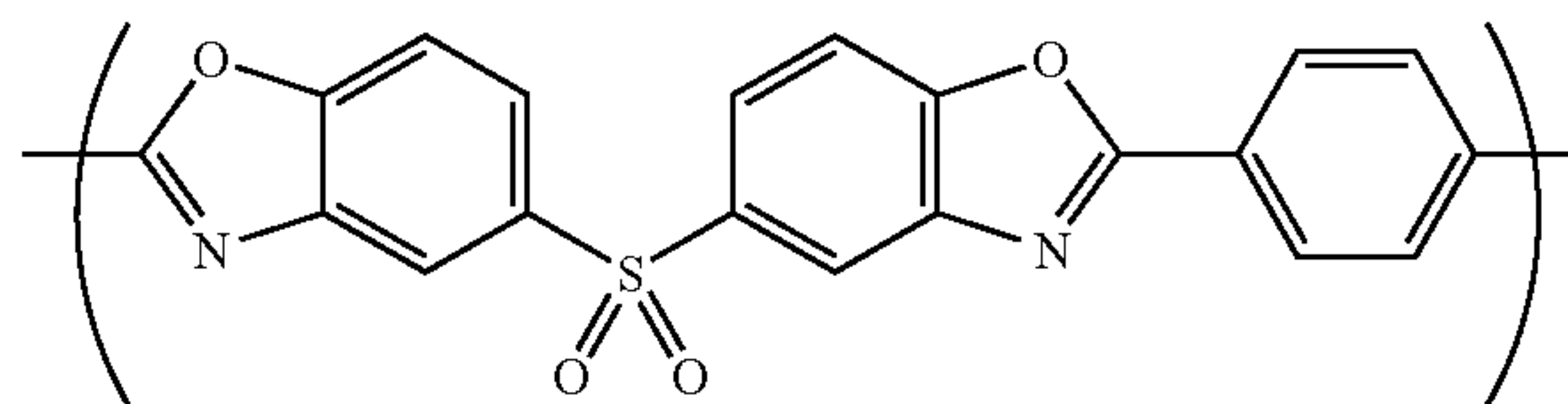
(Chemical Formula 27-10)
