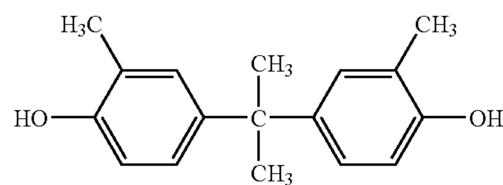
(Chemical Formula 11I) 10
