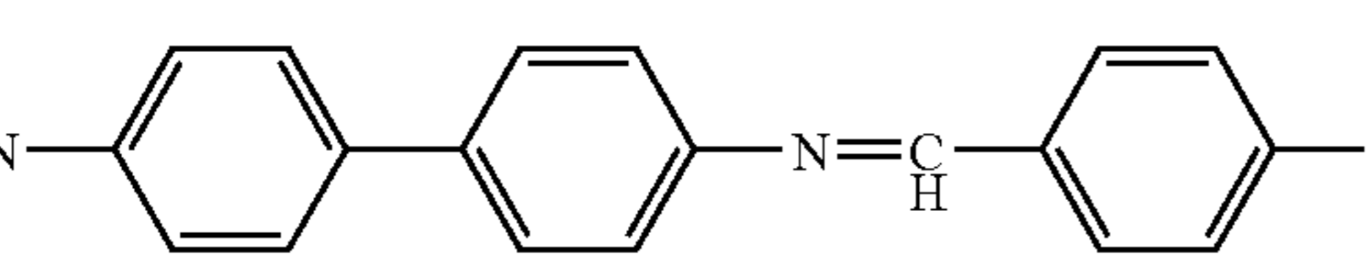
(Chemical Formula 45-5)
