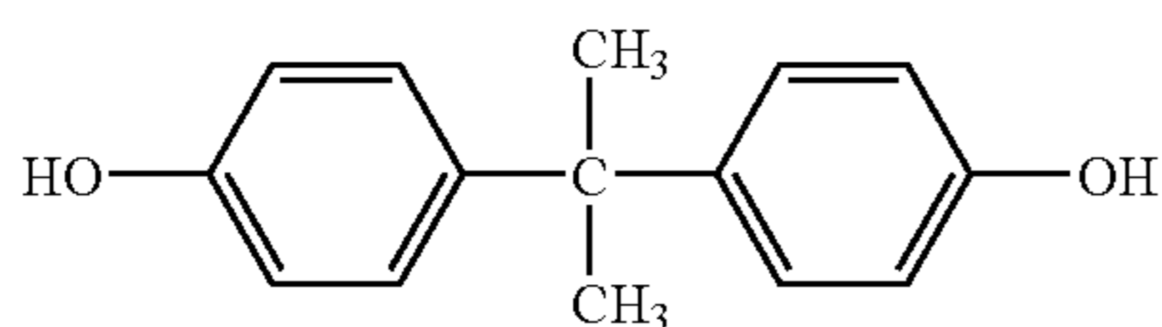
(Chemical Formula 19B)
