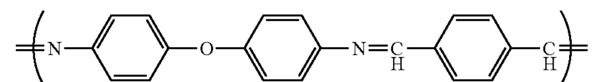
(Chemical Formula 45-5)
