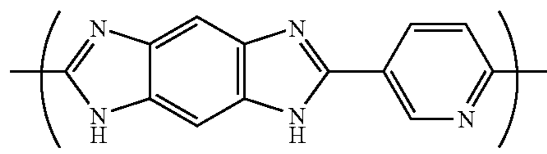
(Chemical Formula 25-8)
