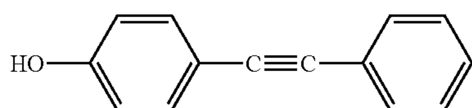
(Chemical Formula 16C)
