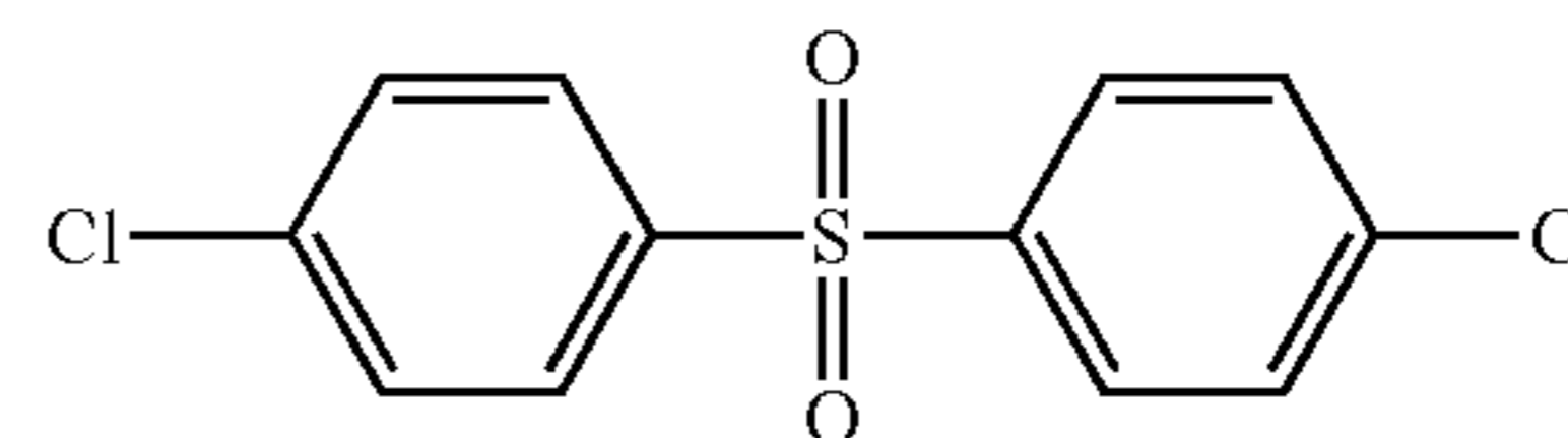
(Chemical Formula 10B)
