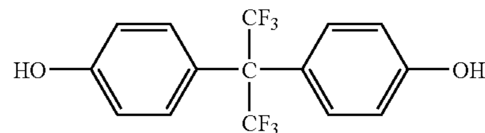
(Chemical Formula 11M) 30
