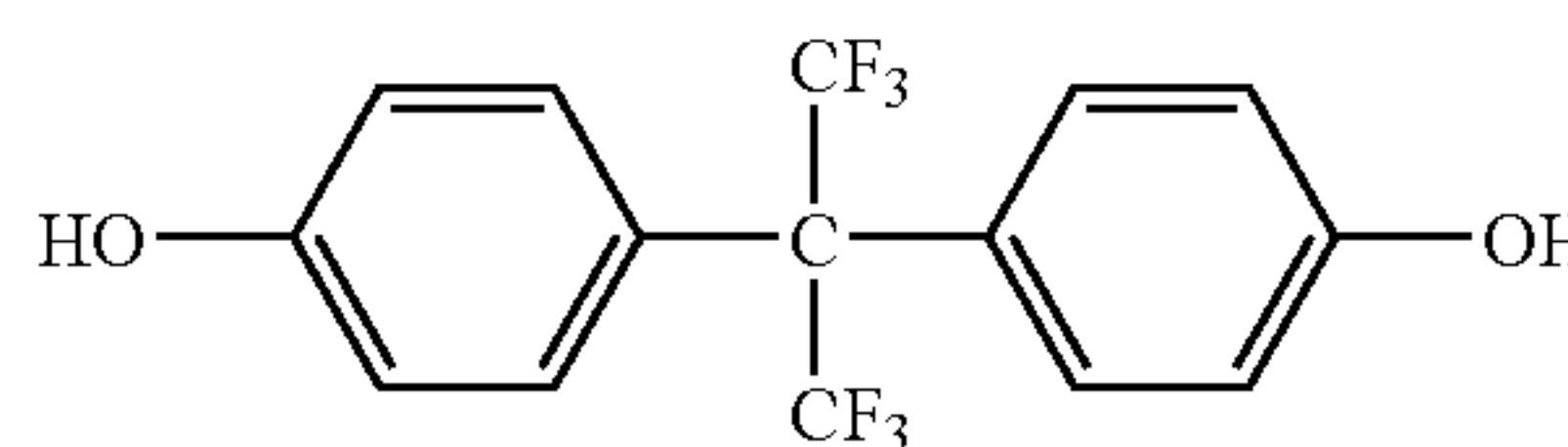
(Chemical Formula 11M)
