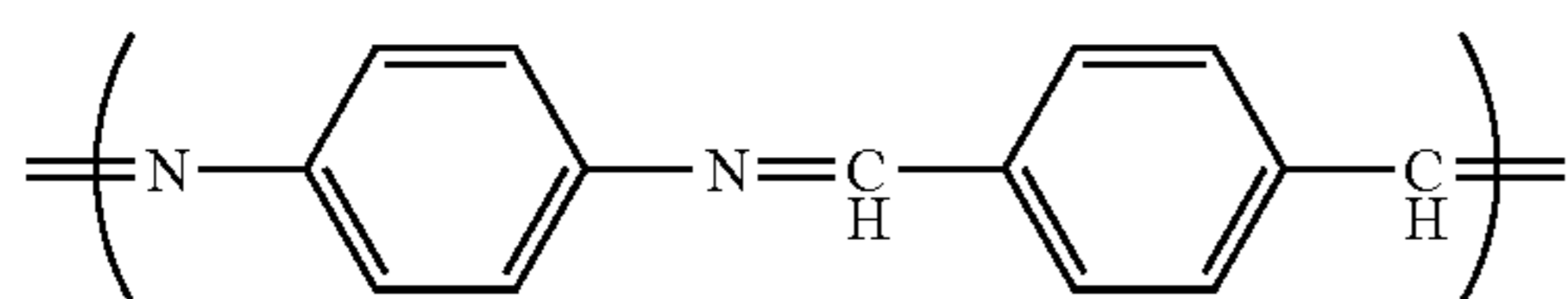
(Chemical Formula 45-2)
