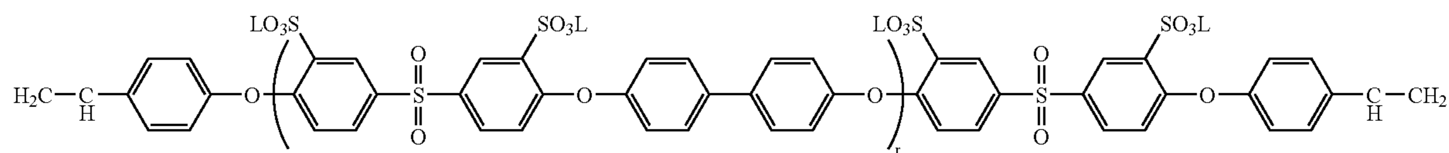
(Chemical Formula 20C)
