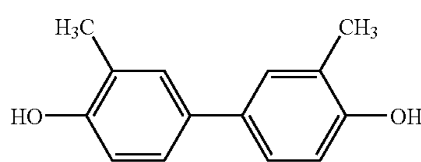
(Chemical Formula 11K) 20
