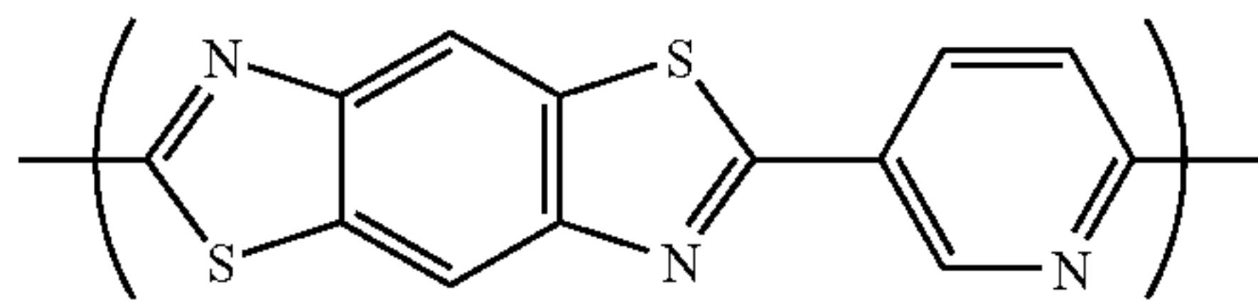
(Chemical Formula 25-7)
