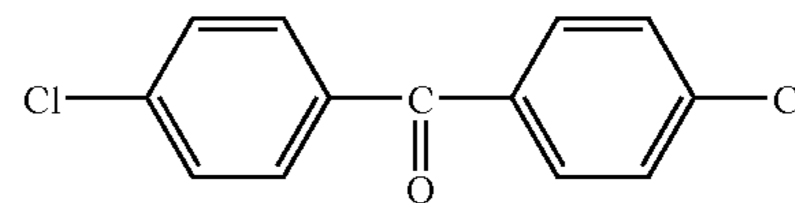
(Chemical Formula 10C)
