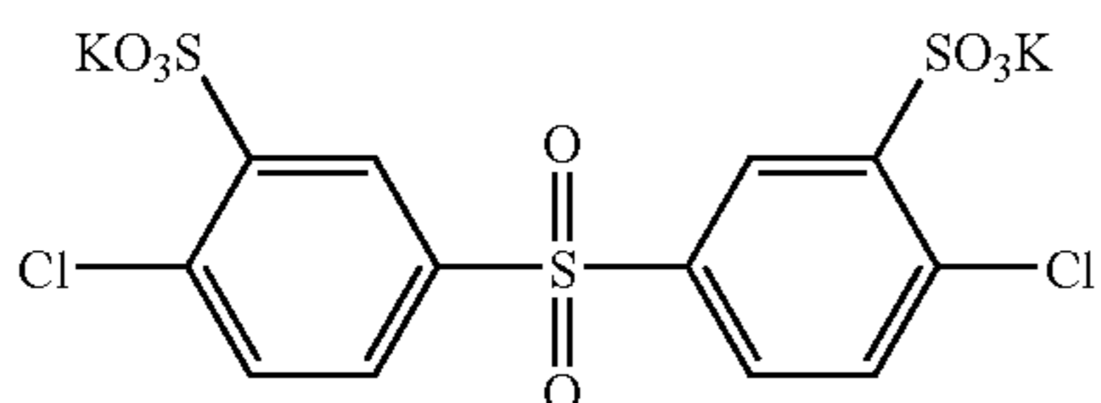
(Chemical Formula 8C)
