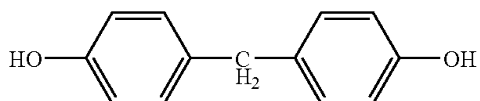
(Chemical Formula 11E)
