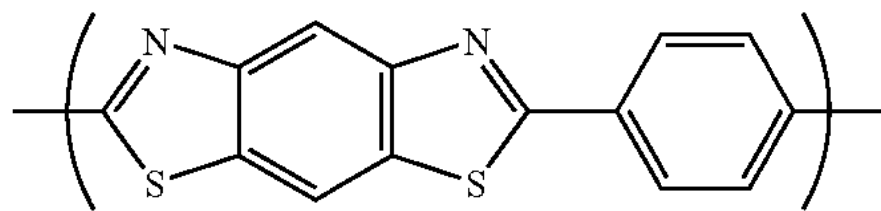
(Chemical Formula 25-2)
