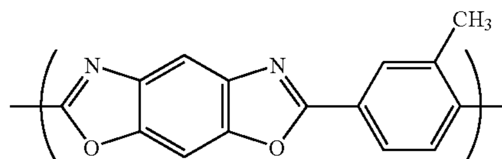
(Chemical Formula 26-2)
