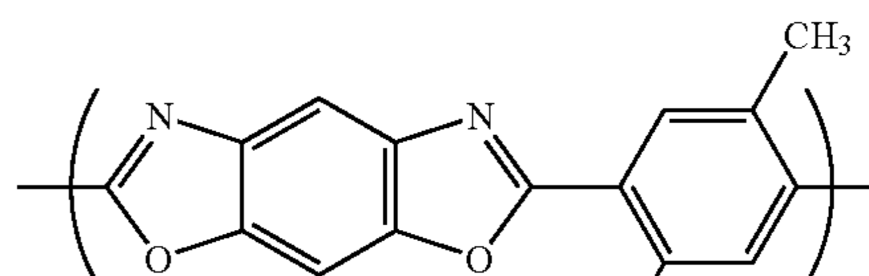
(Chemical Formula 26-5)
