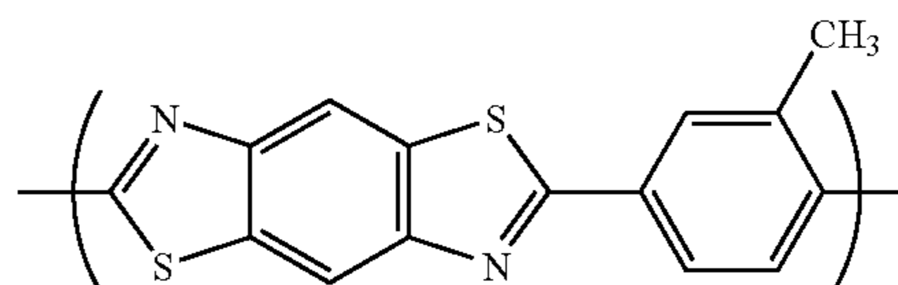
(Chemical Formula 26-3)
