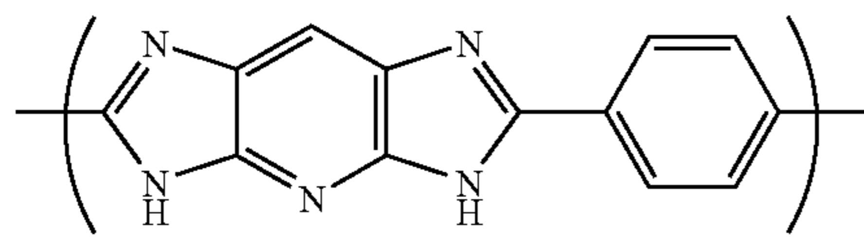
(Chemical Formula 25-5)
