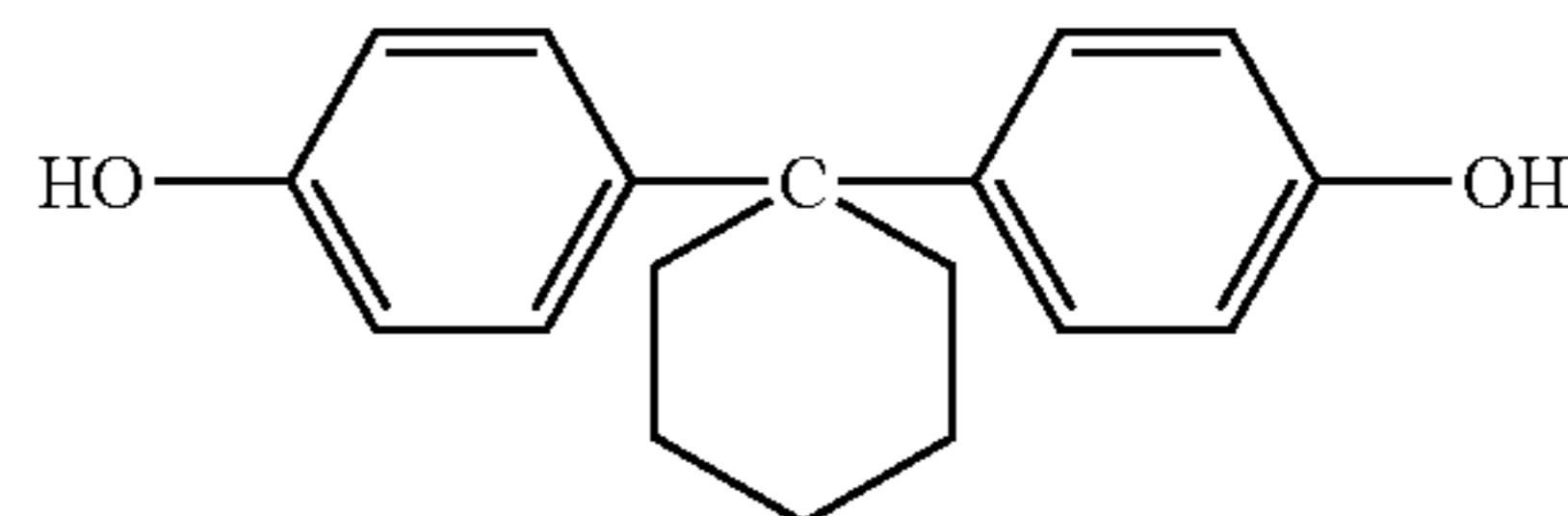
(Chemical Formula 19E)
