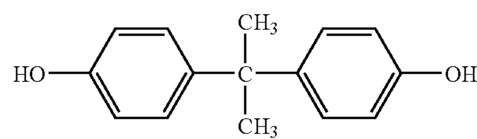
(Chemical Formula 11H) 5
