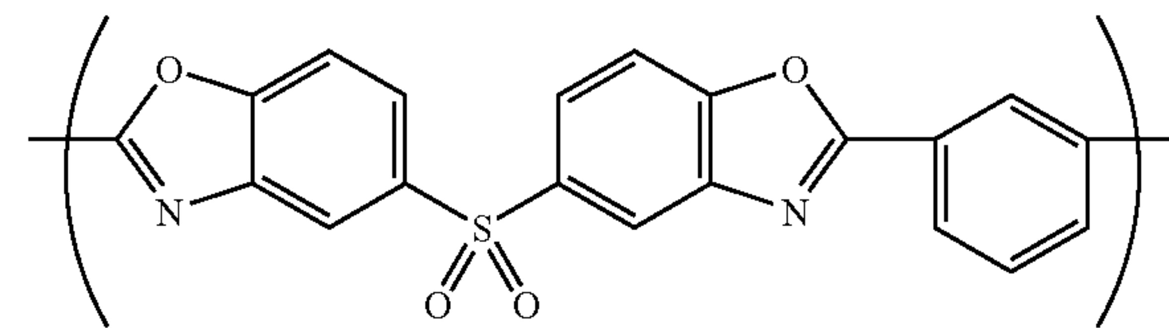
(Chemical Formula 27-11)
