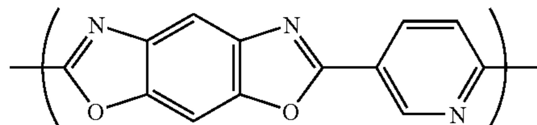
(Chemical Formula 25-6)
