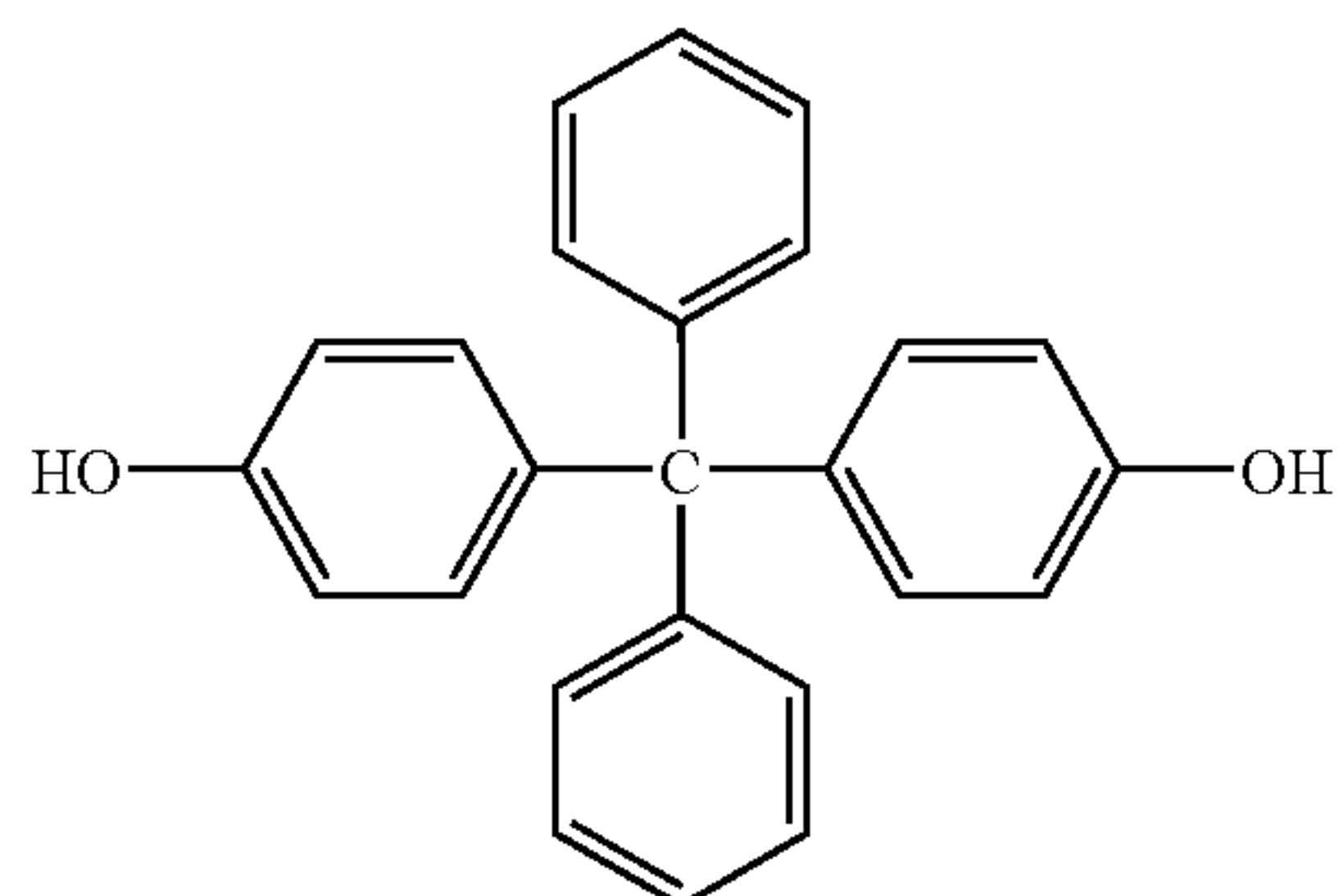
(Chemical Formula 11G)
