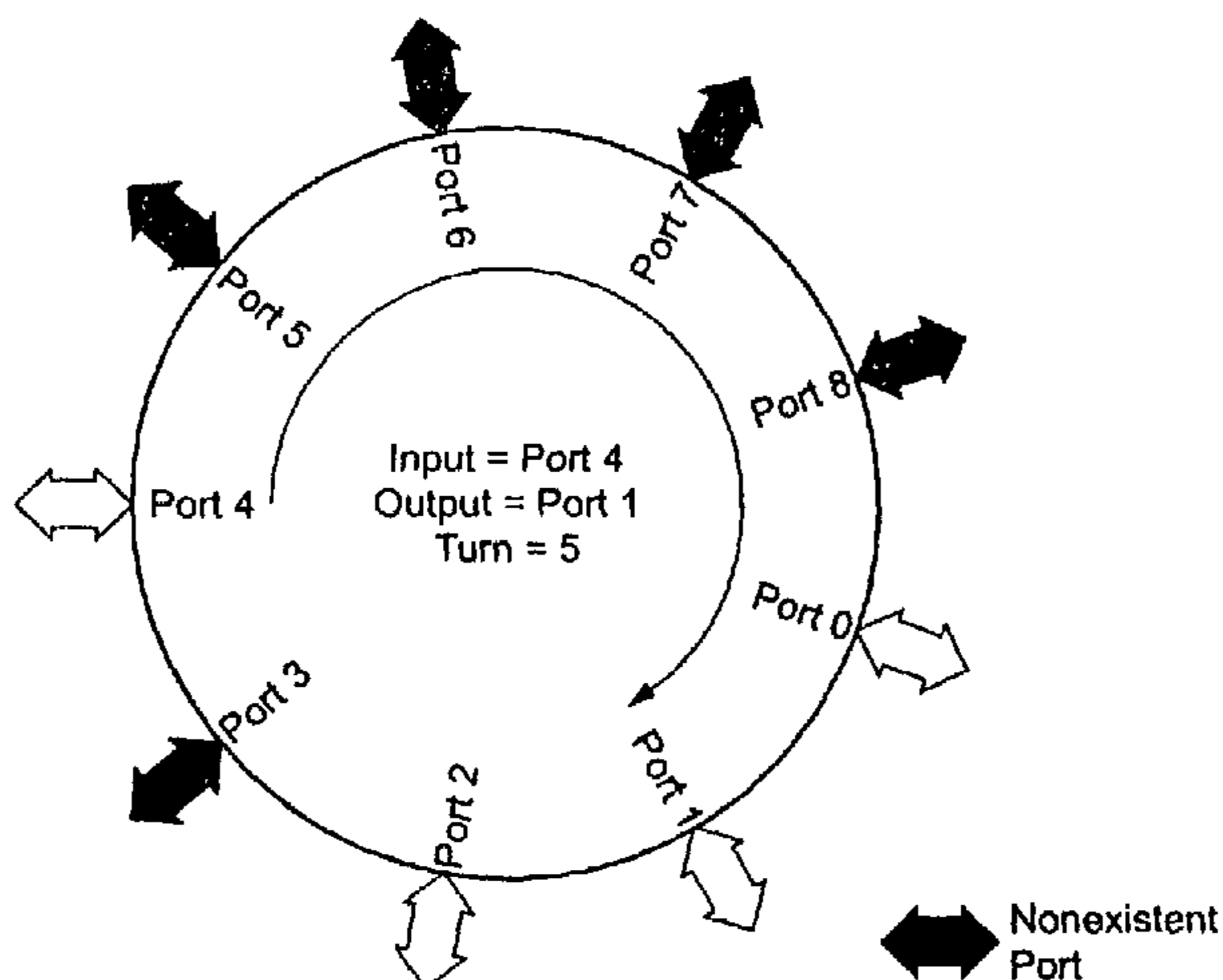
Path Specification View of Switch Ports
