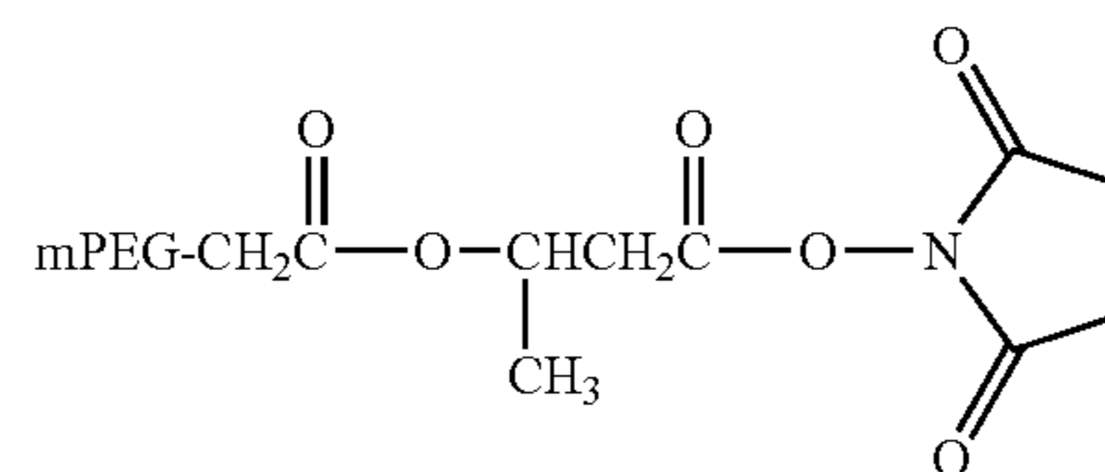
mPEG-CM-HBA-NHS (CM = carboxymethyl; HBA = Hydroxy butyric acid)
