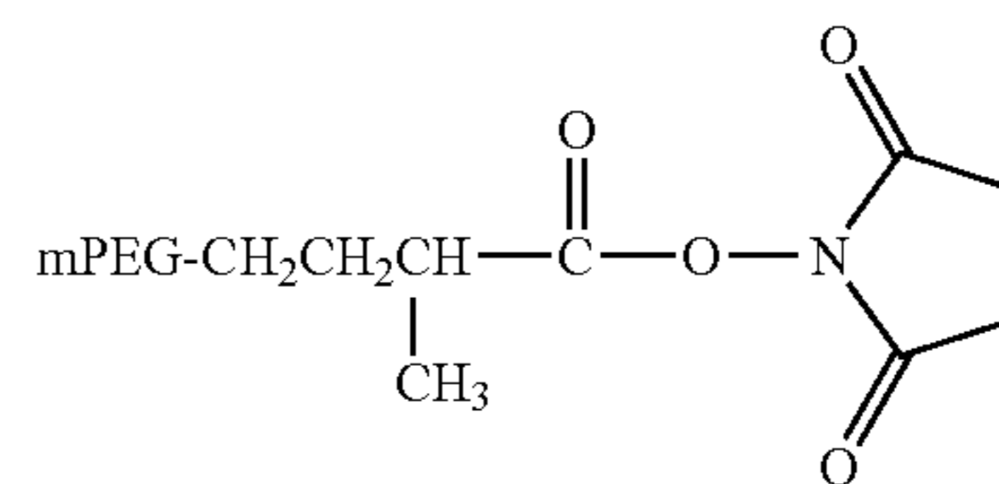
mPEG-CM-HBA-NHS (CM = carboxymethyl; HBA = Hydroxy butyric acid)
