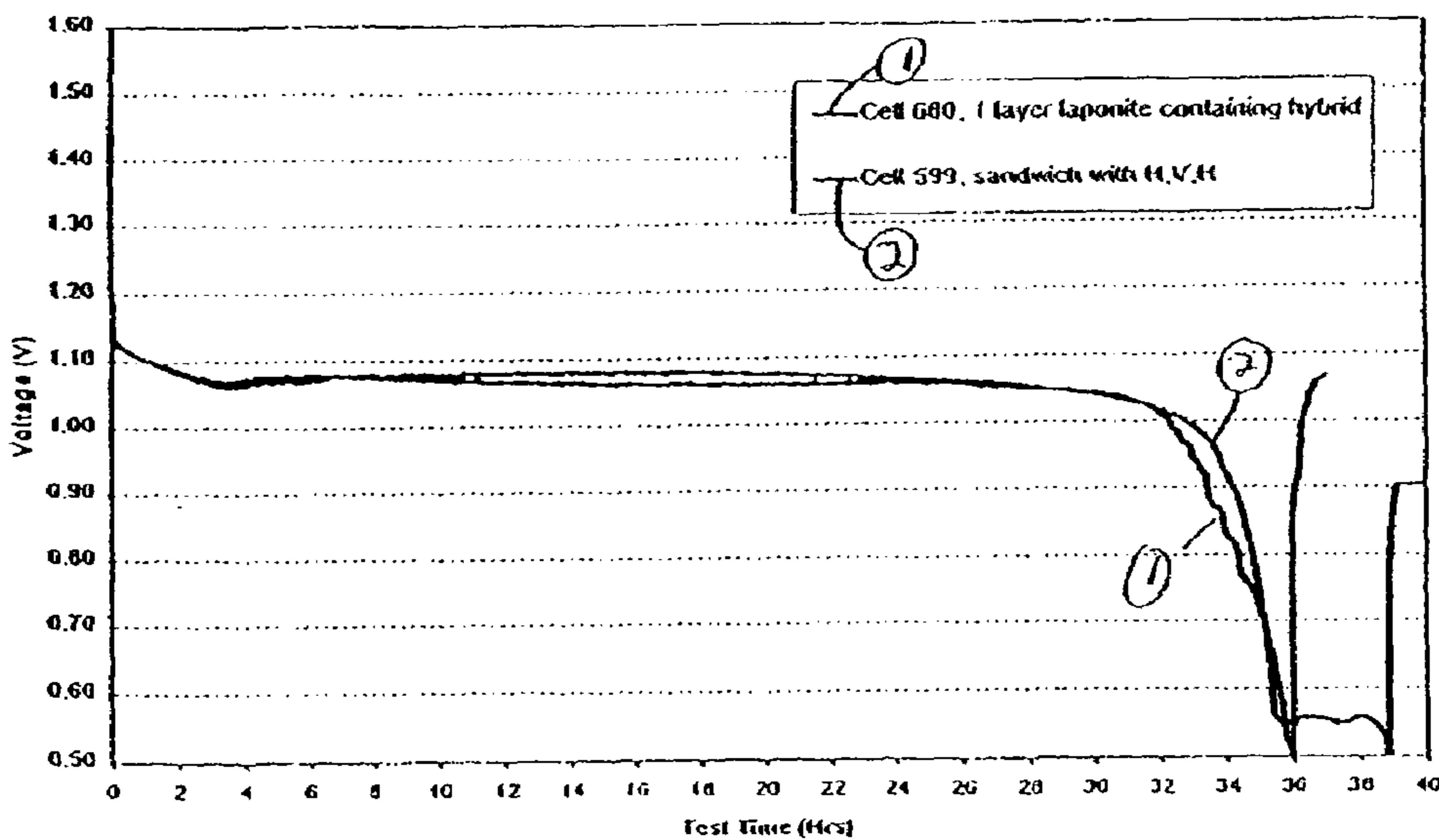
Cells 599,680, 1:1M JMCuO/CuS, Discharged at 5mA 599 discharged after 1 day, 680 discharged after 4 days
