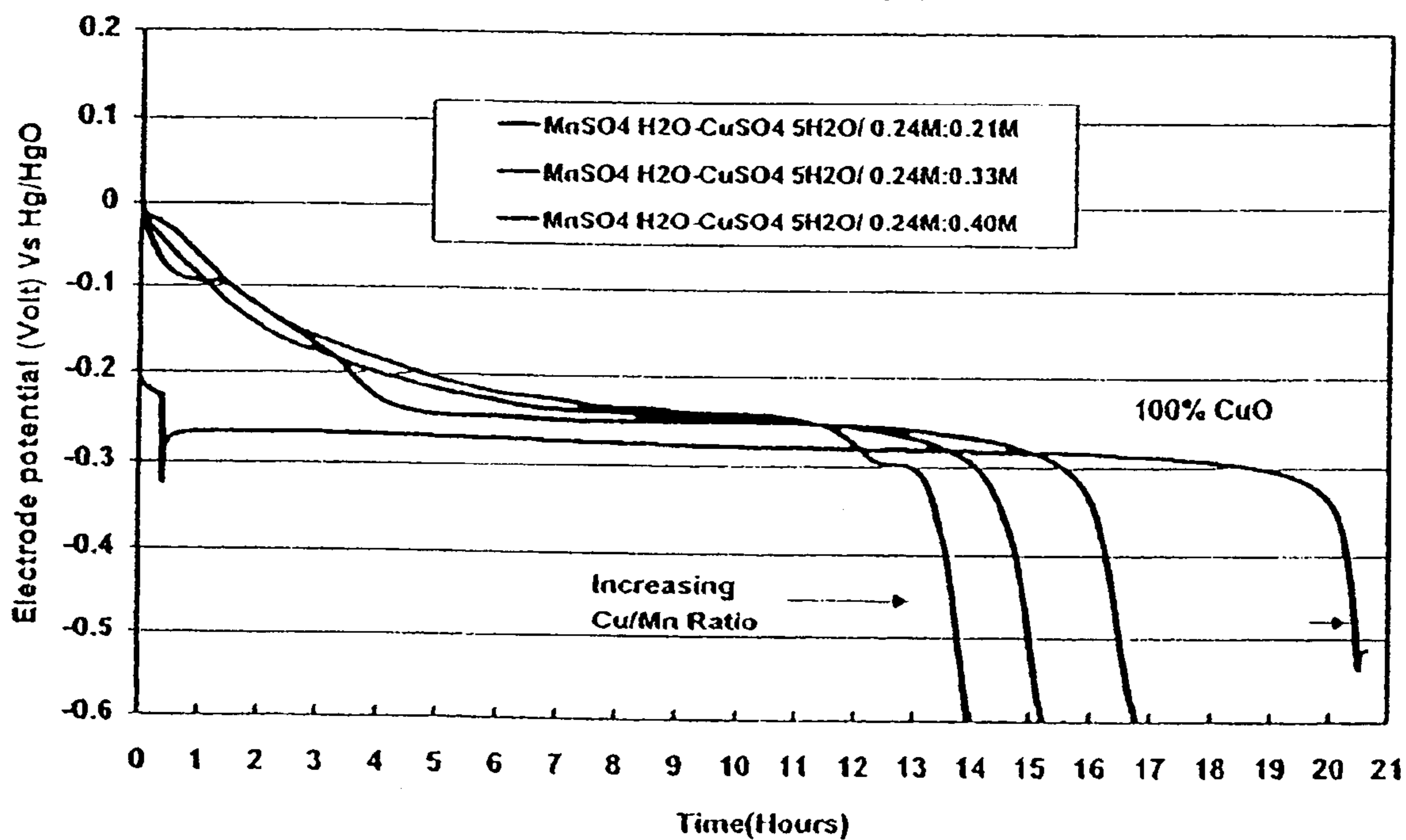
Effect of increasing Proportion of Cu/Mn in Cathode Material vs. Pure CuO 5 mA Continuous Discharge, 28-2 Electrolyte, Half-cell
