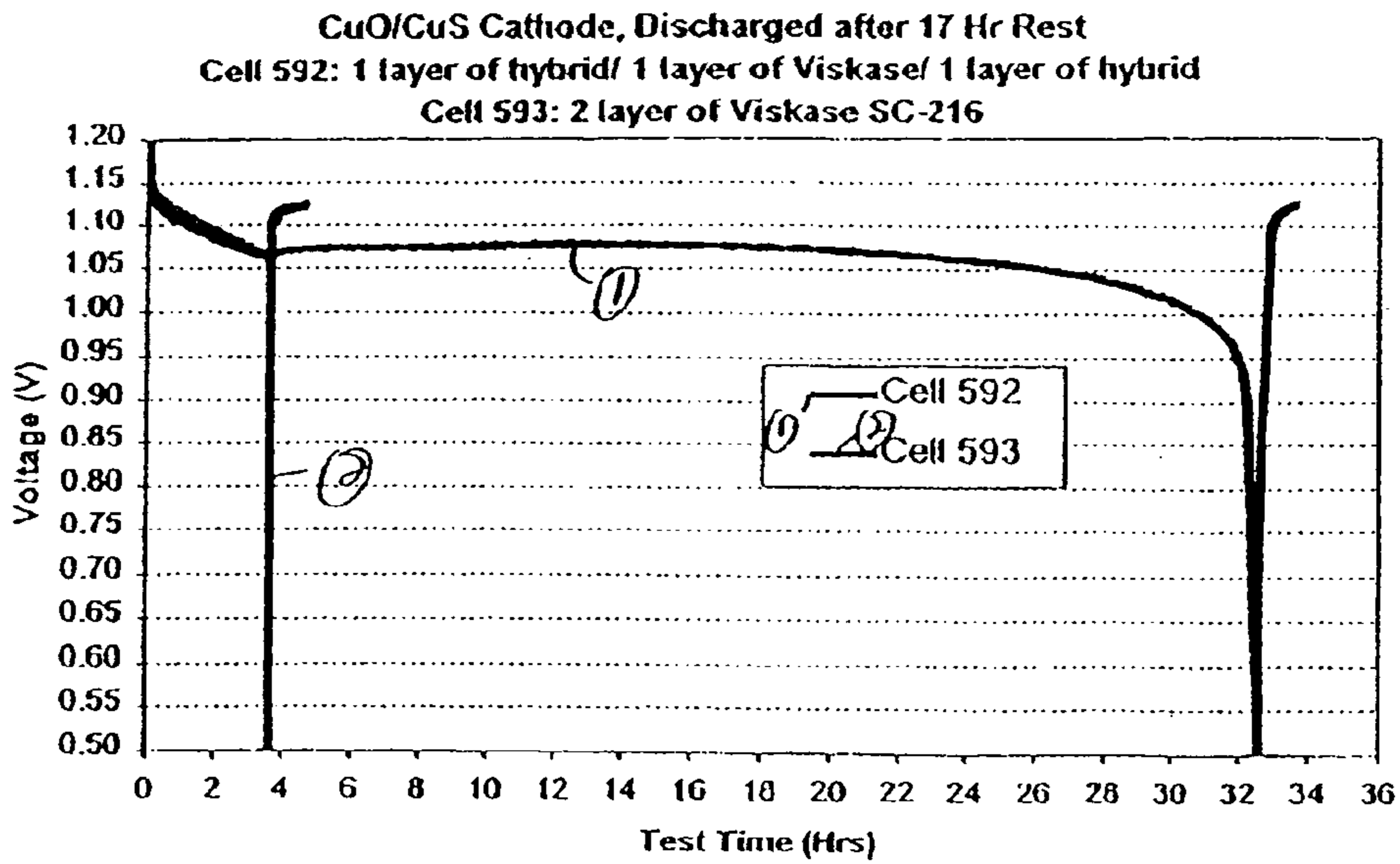
The effect of separator types on cathode material made from CuO (Aldrich) and CuS (Alfa) mixture.
