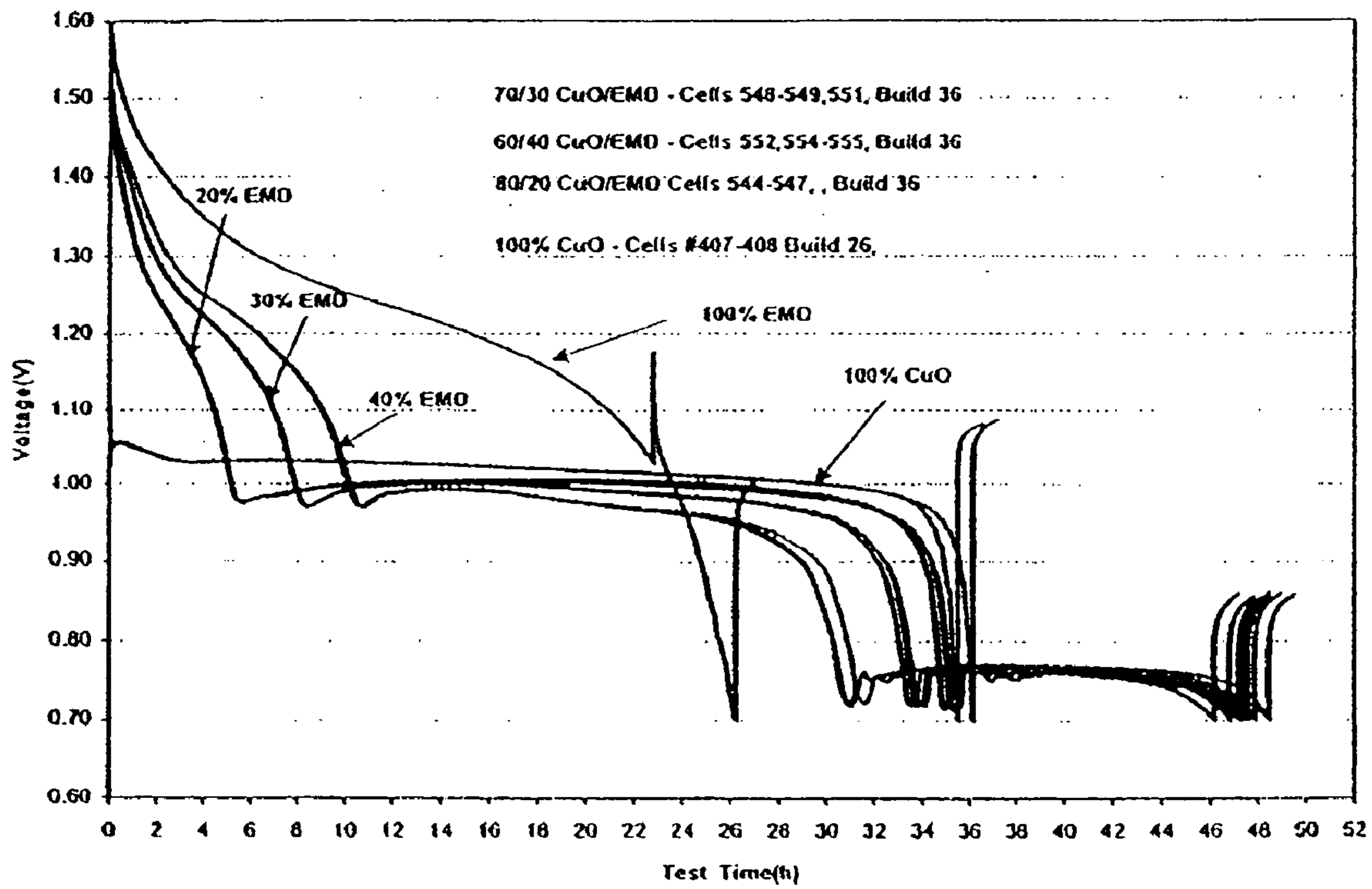
Behavior of EMD / CuO Physical Mixtures and CuO vs. Zinc in 357 Button Cells Jet-Milled CuO, 34-2 Electrolyte, 5 mA Discharge
