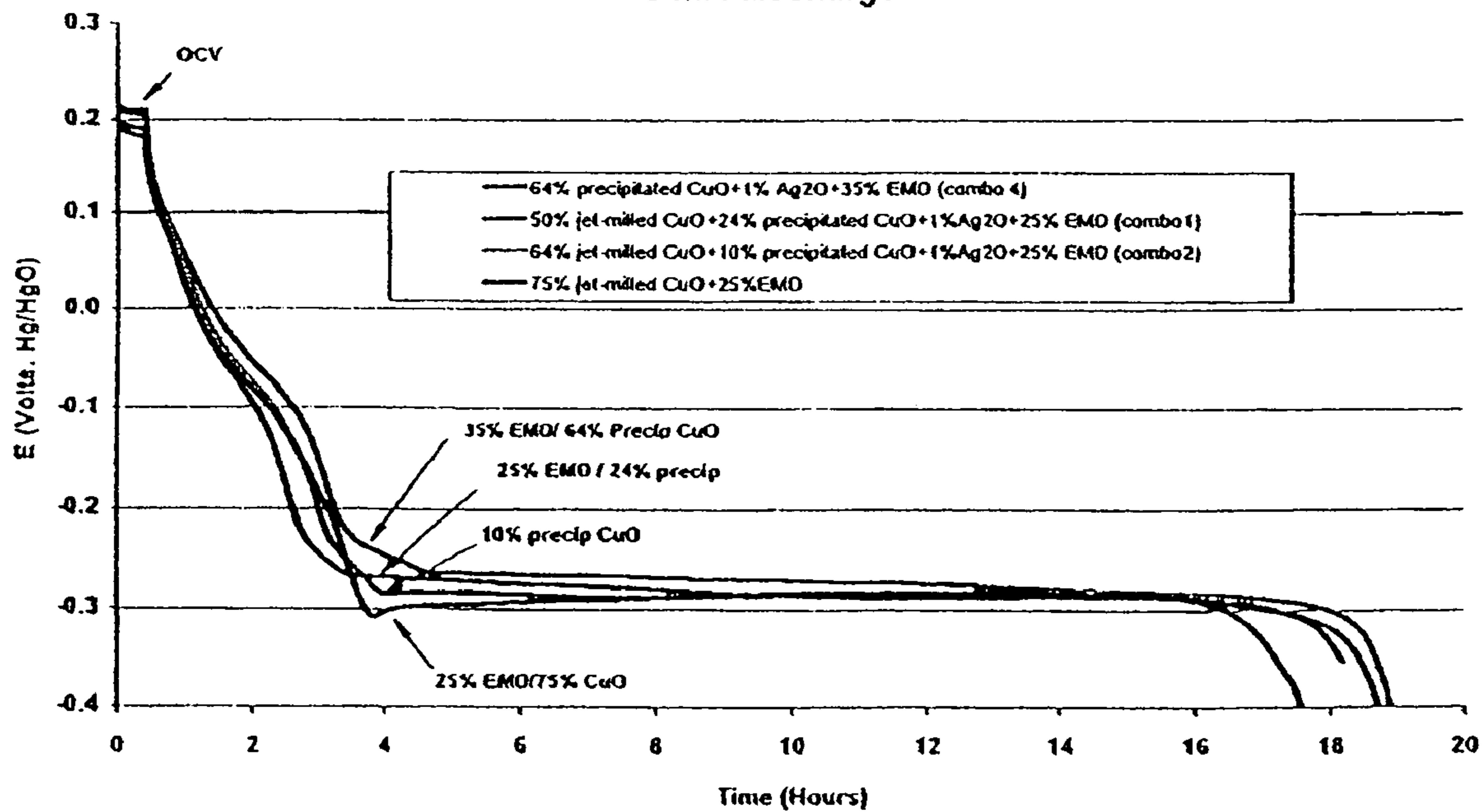
Smoothing EMD/CuO transition by chemically precipitated CuO 5 mA discharge
