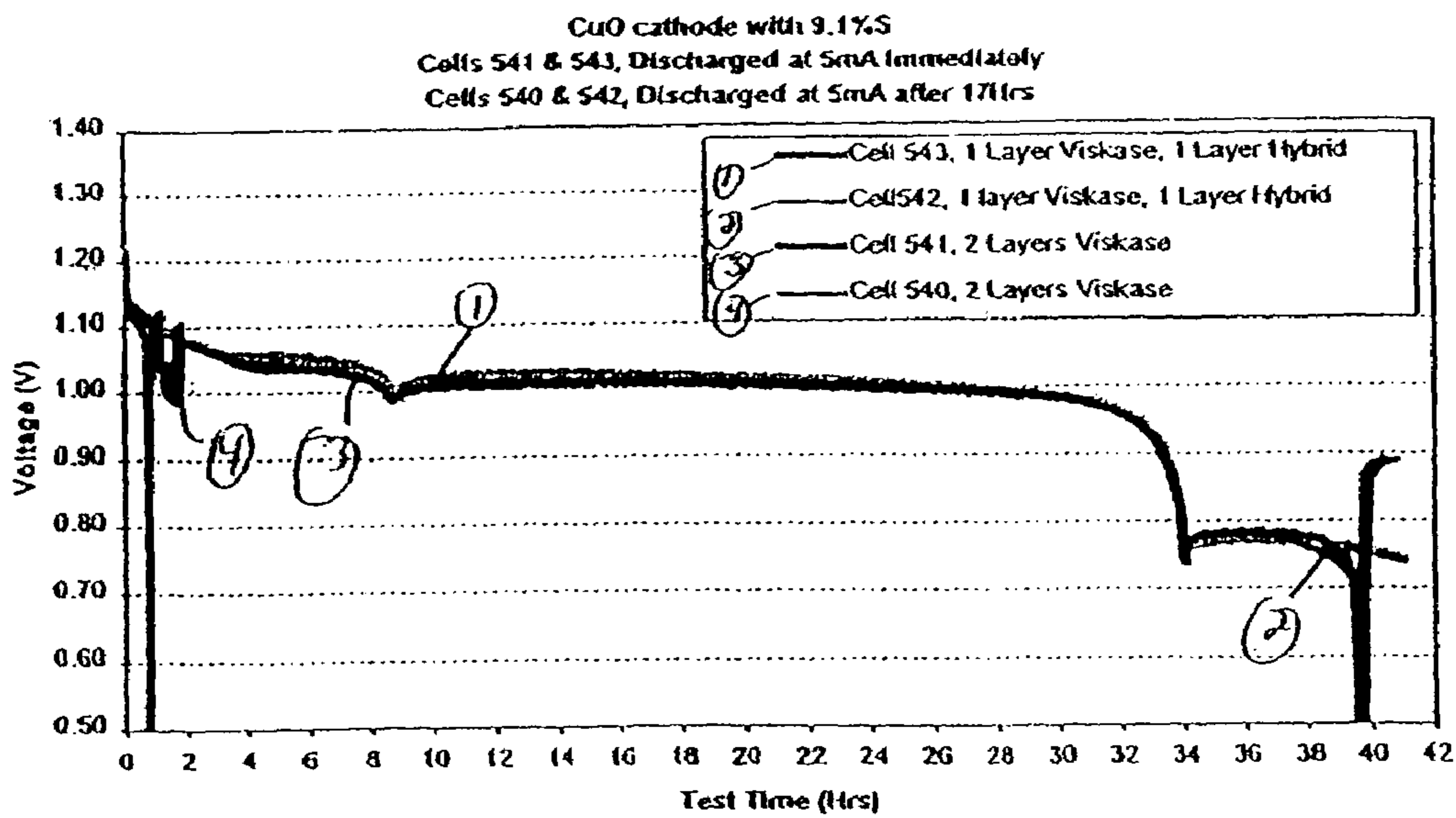
Effect of separators for cathode made from CuO and S mixture.
