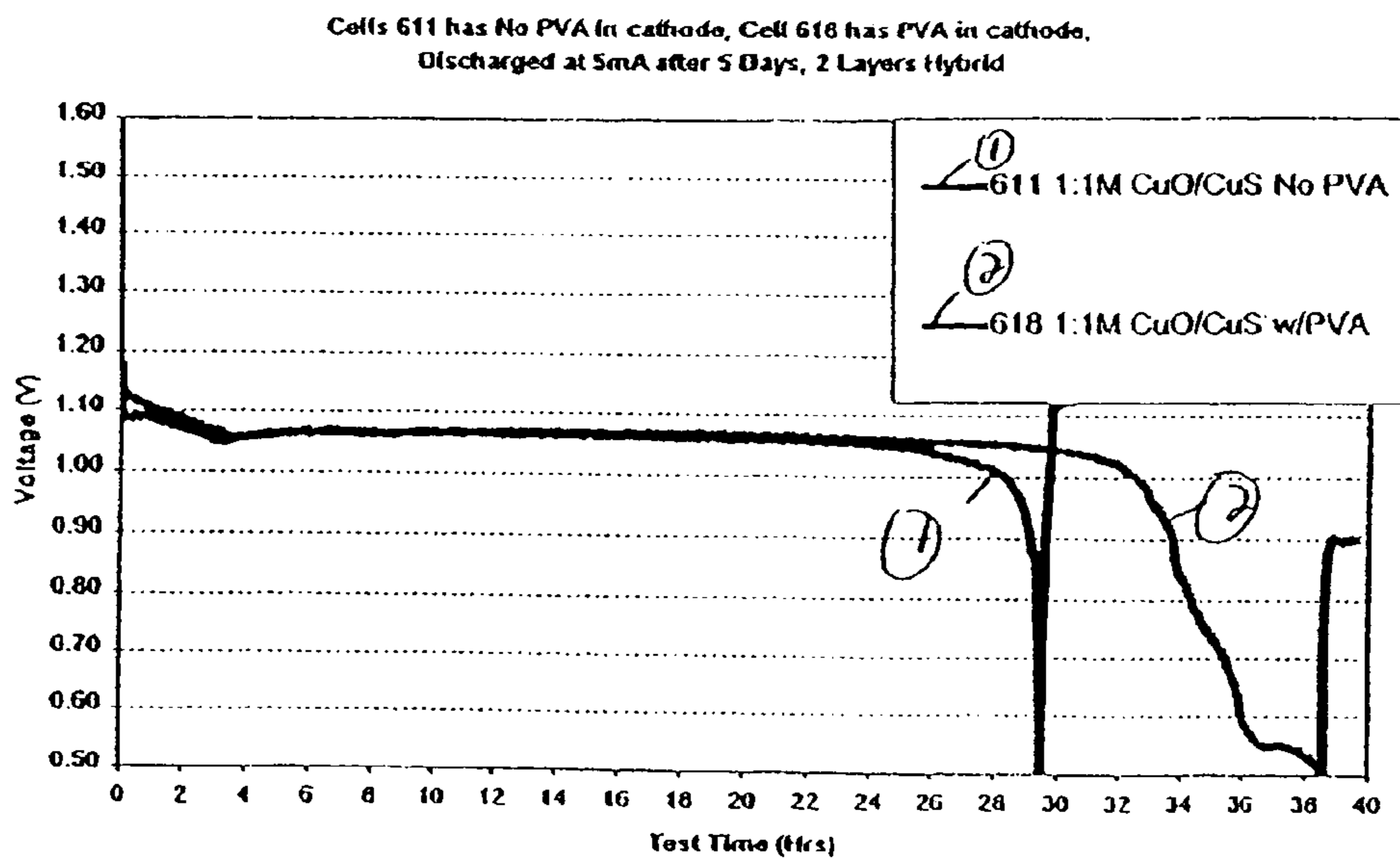
Effect of PVA in the cathode with 2 layers of hybrid separator.
