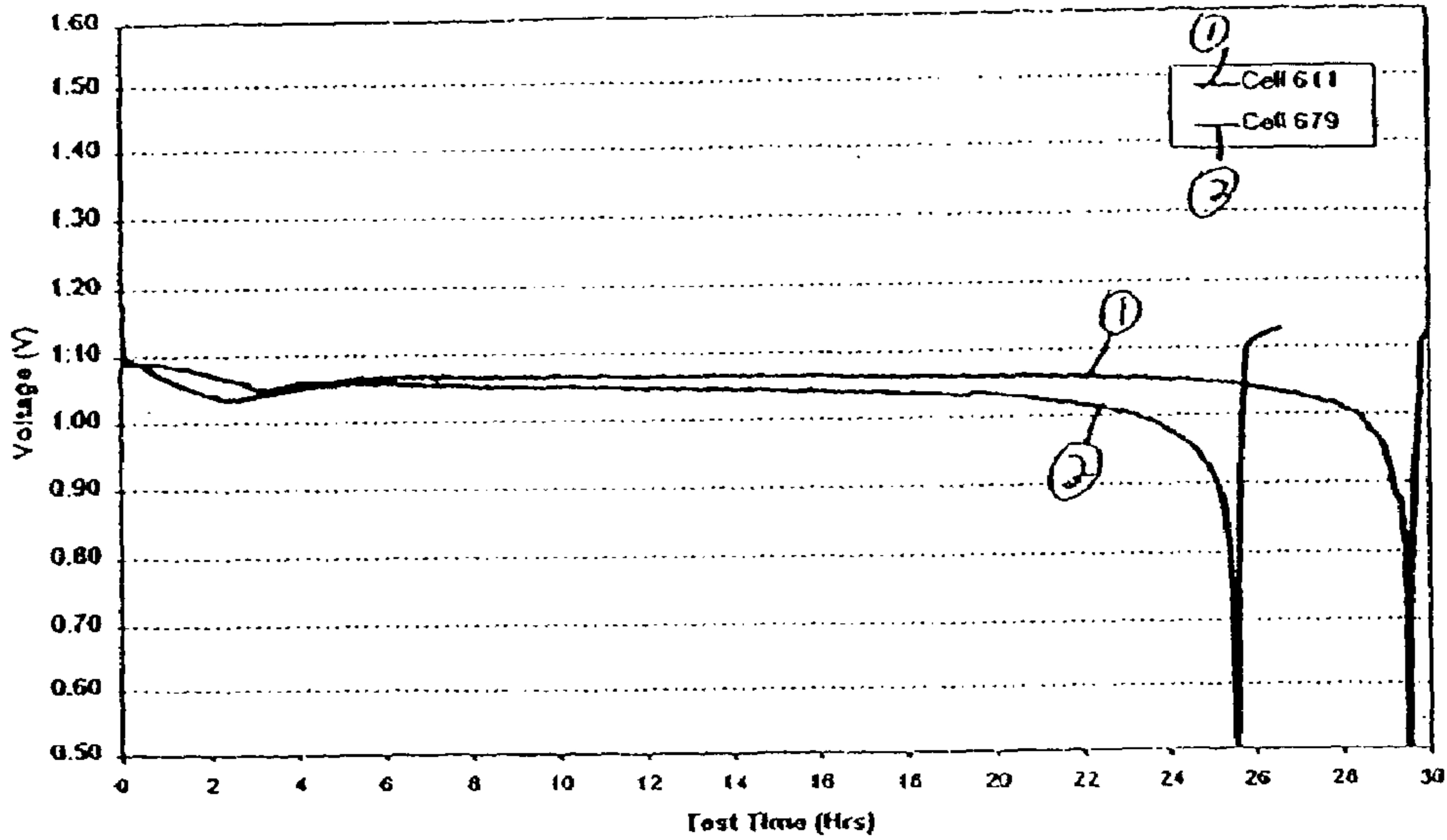
Discharge comparison of 357 cells made with 1:1 M CuO and CuS mixture. The cell 611 has two layers of hybrid (cross linked PVA coating on F3T23) separator. The cell 679 has one layer of EVA emulsion coated F3R23 (supplied by Kararay) hybrid separator.
