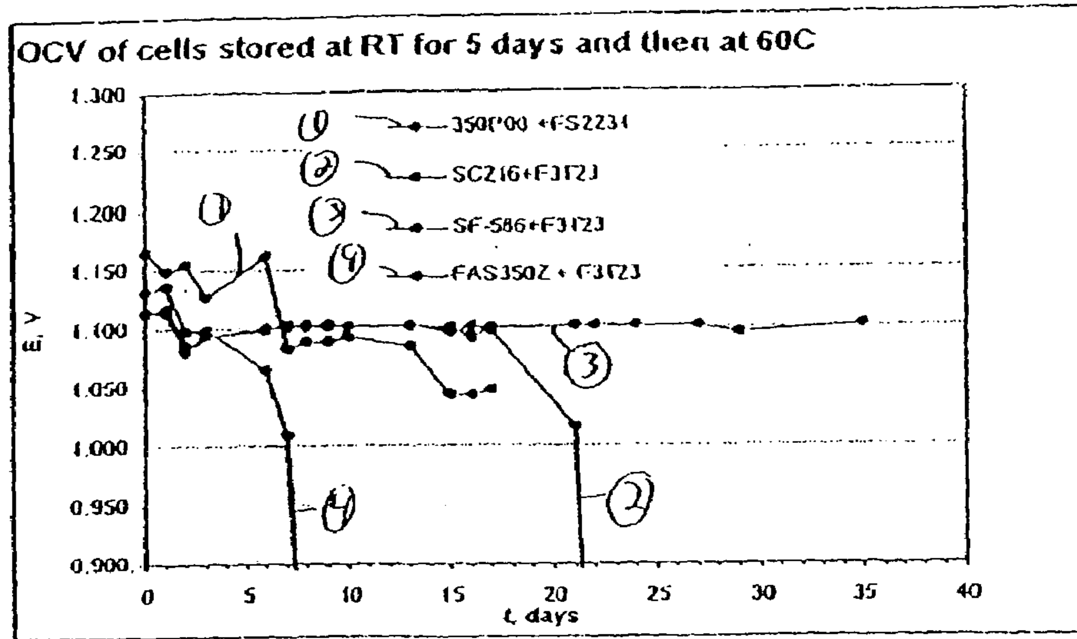
357 cell made with CuO and various separator, long term storage results.
