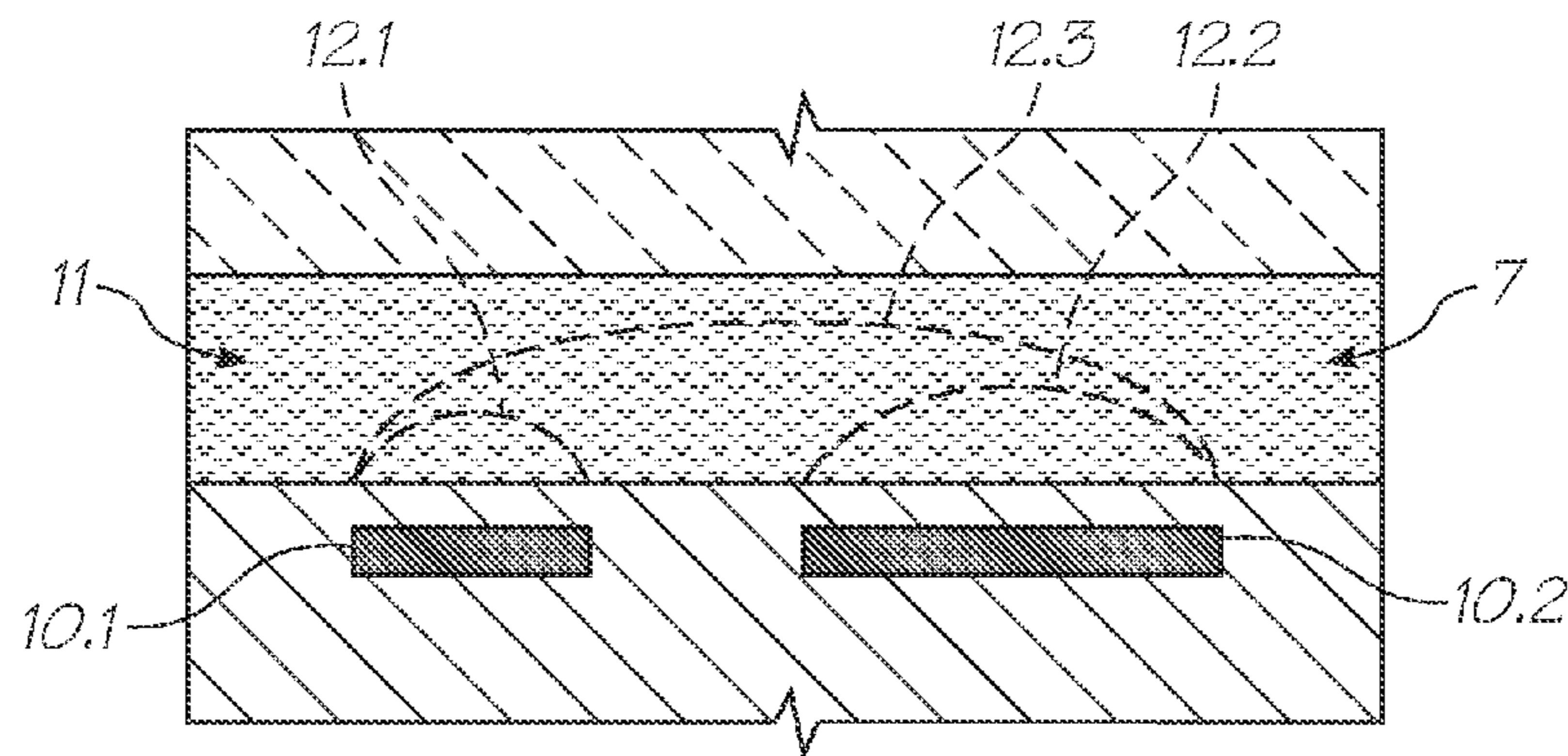
FIG. 52 (PRIOR ART)
