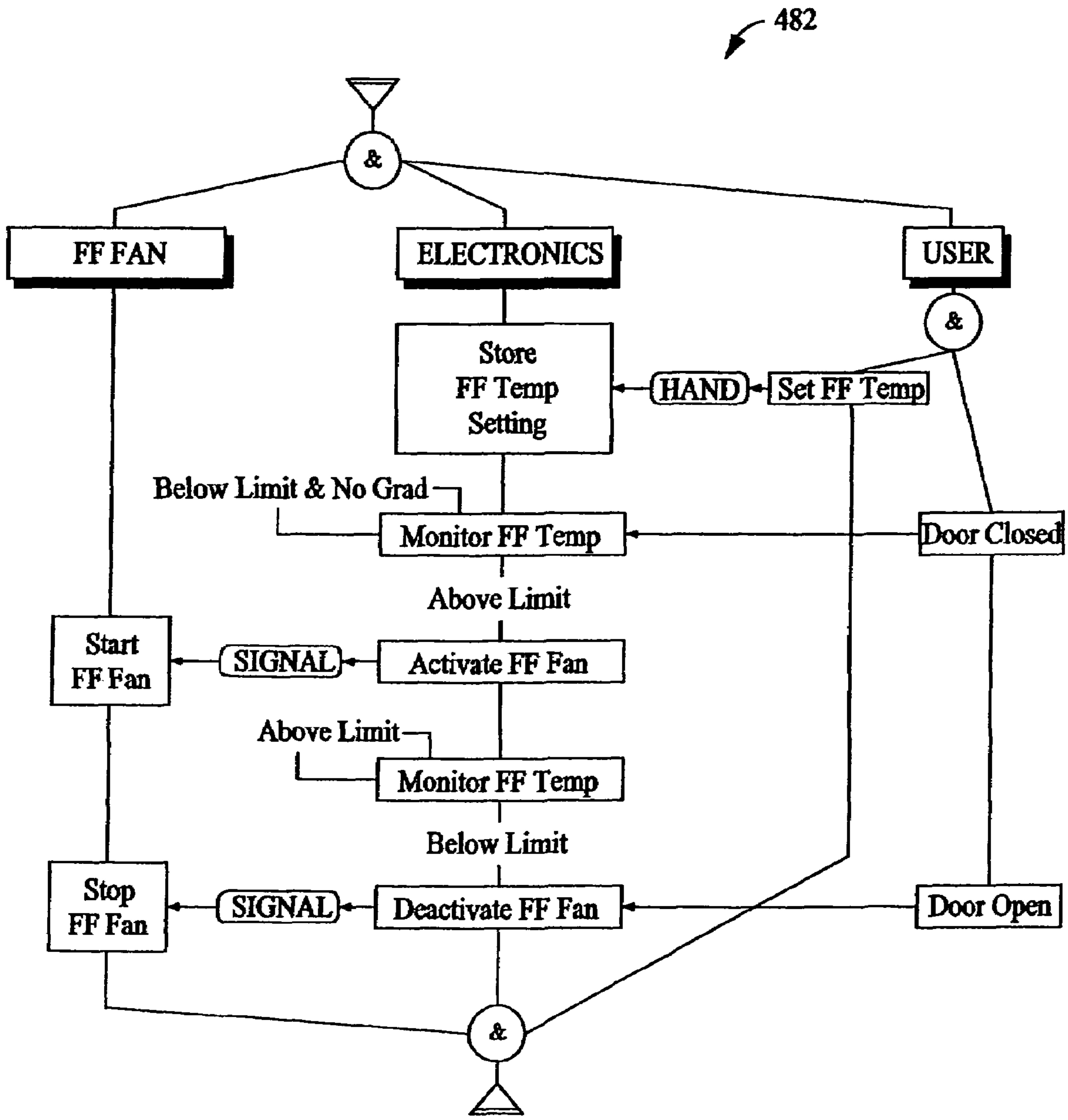
Fresh Food Fan Behavior Diagram
