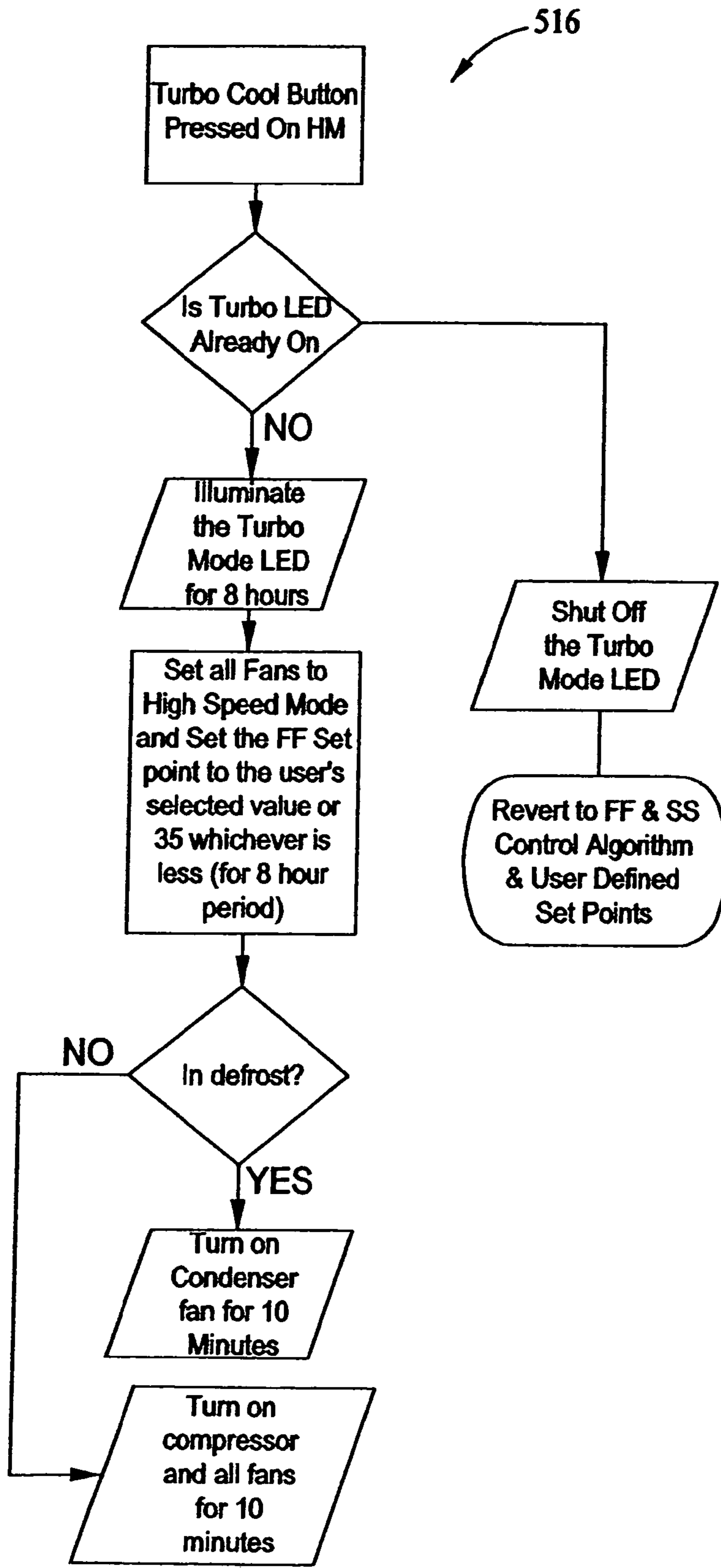
Turbo Cycle Algorithm
