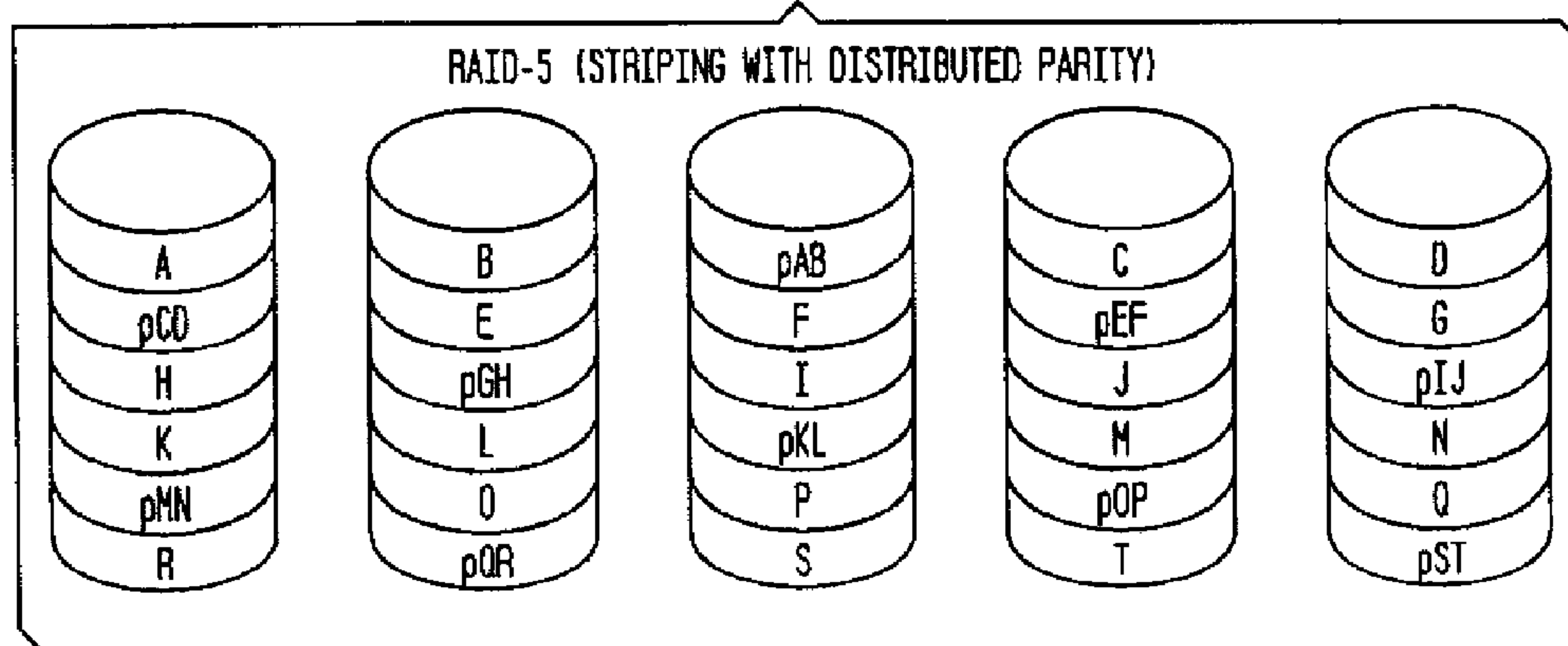
FIG. 4 (PRIOR ART)
