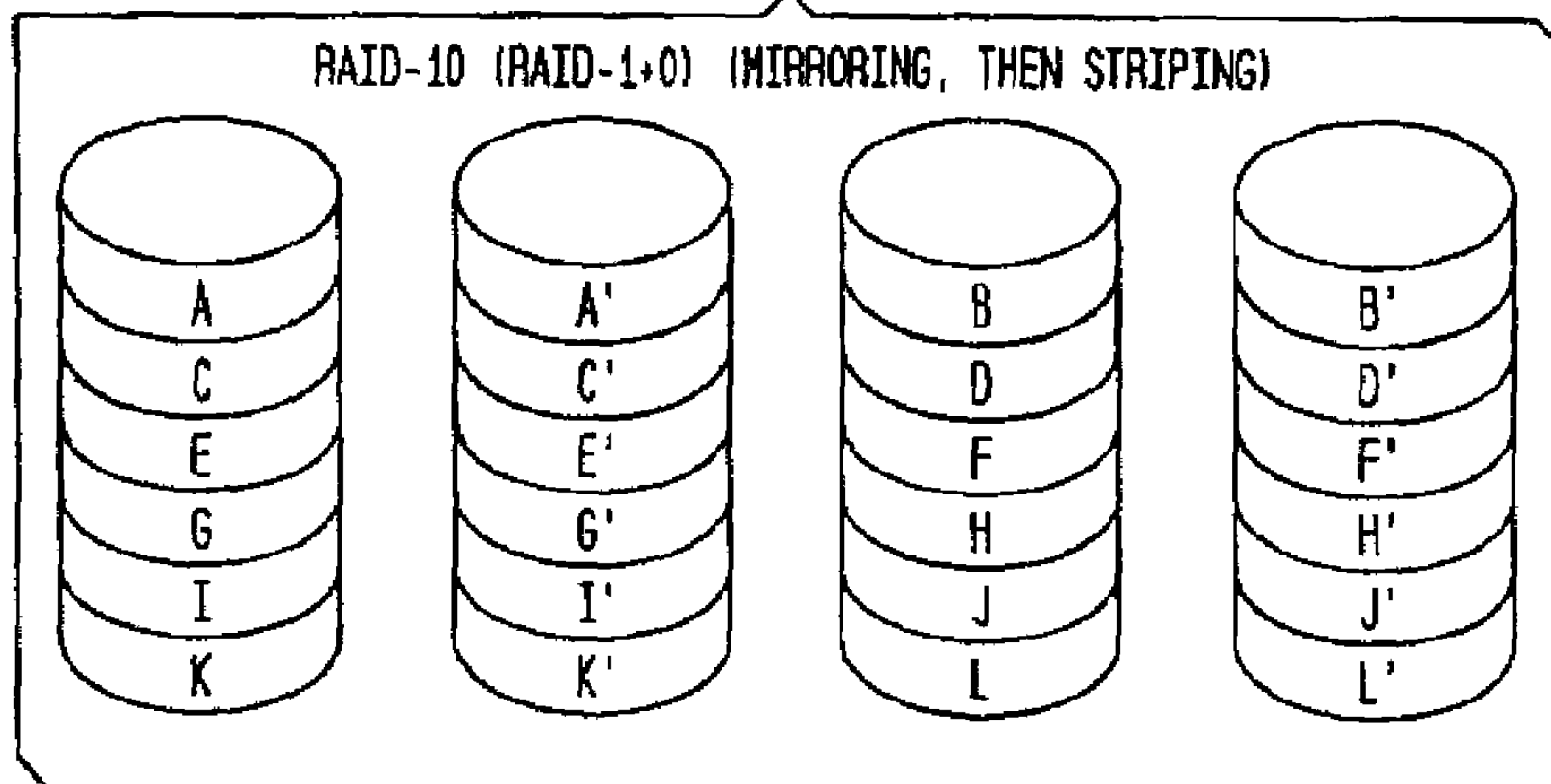
FIG. 5 (PRIOR ART)
