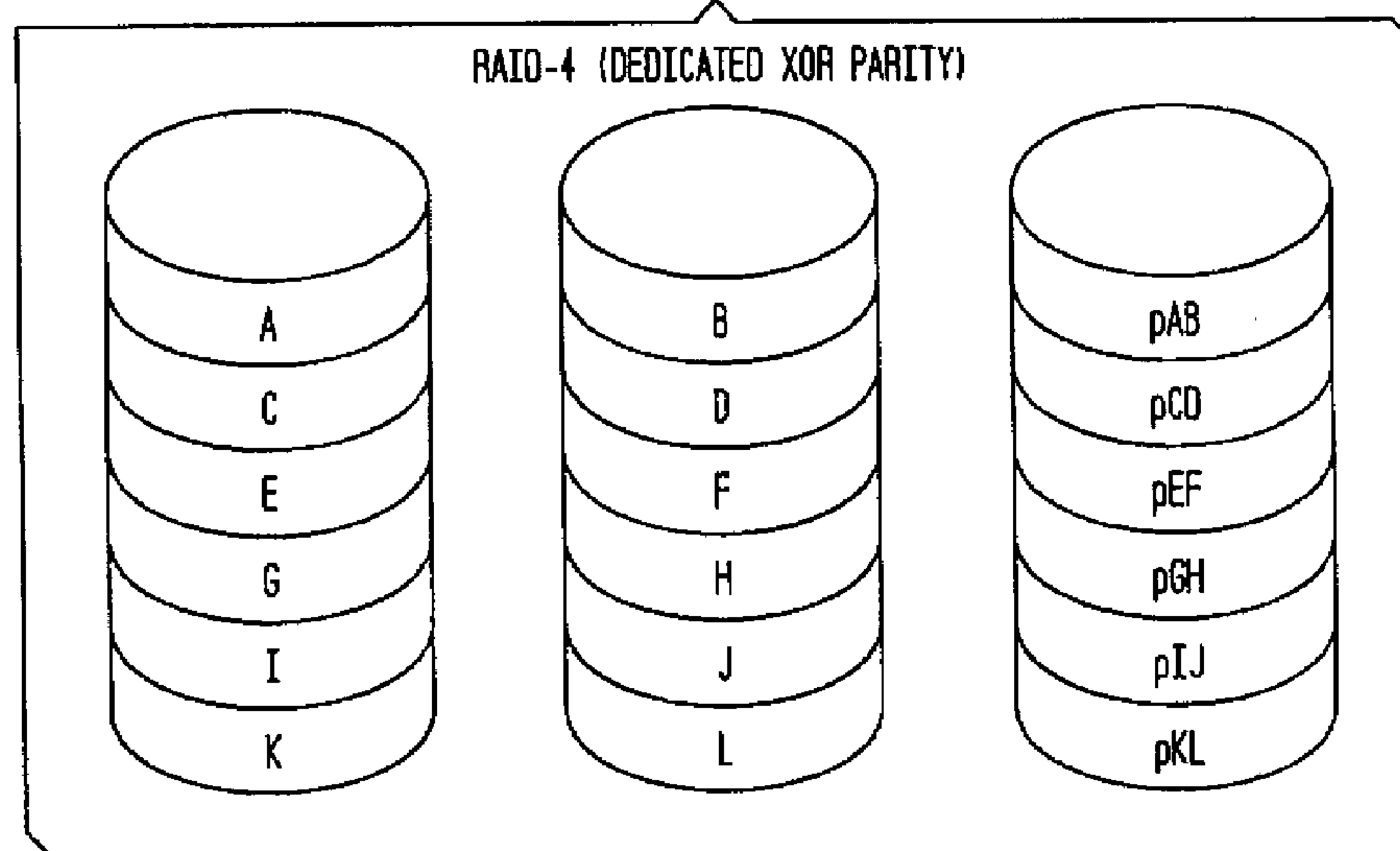
FIG. 3 (PRIOR ART)
