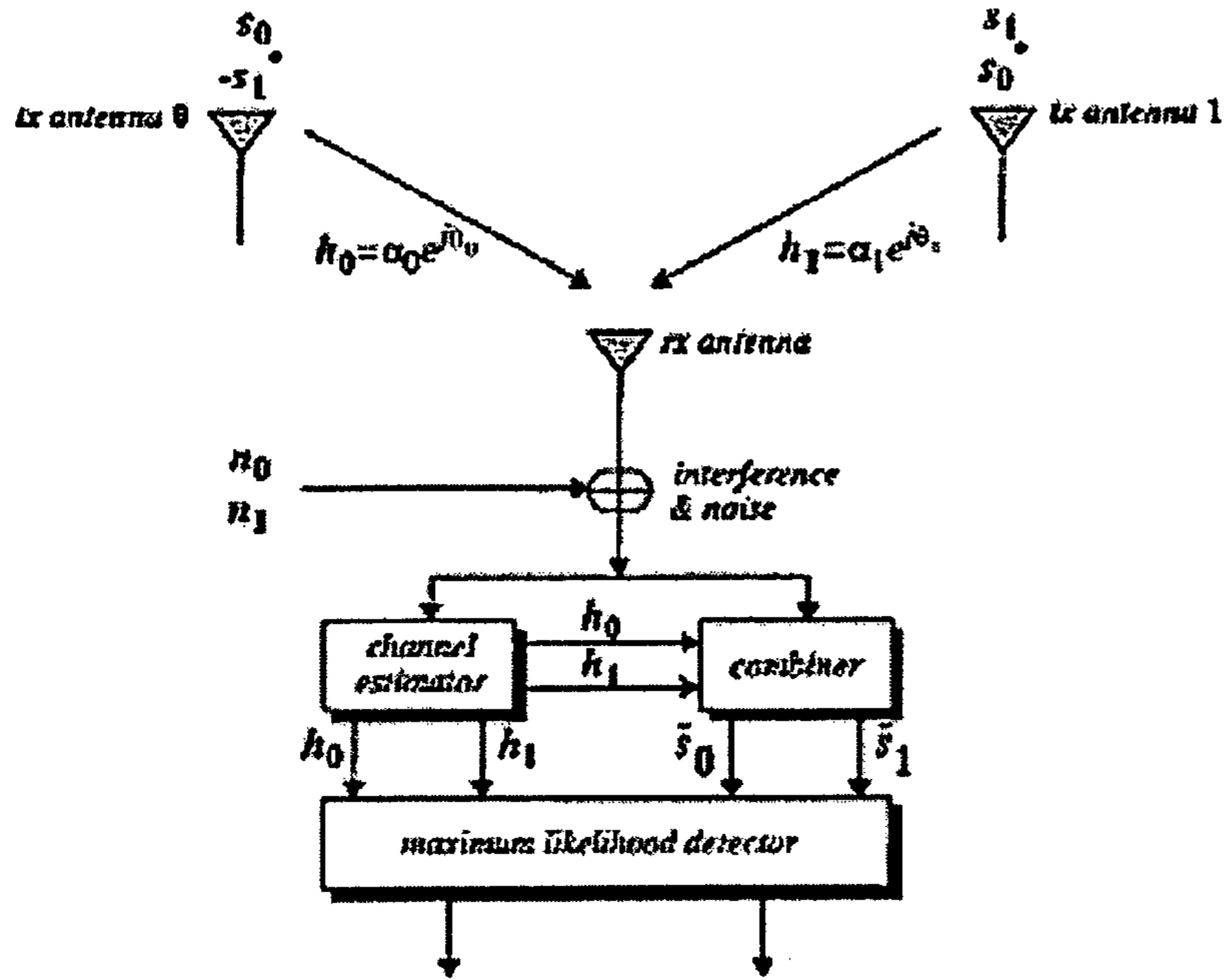
FIG. 3 (PRIOR ART)
