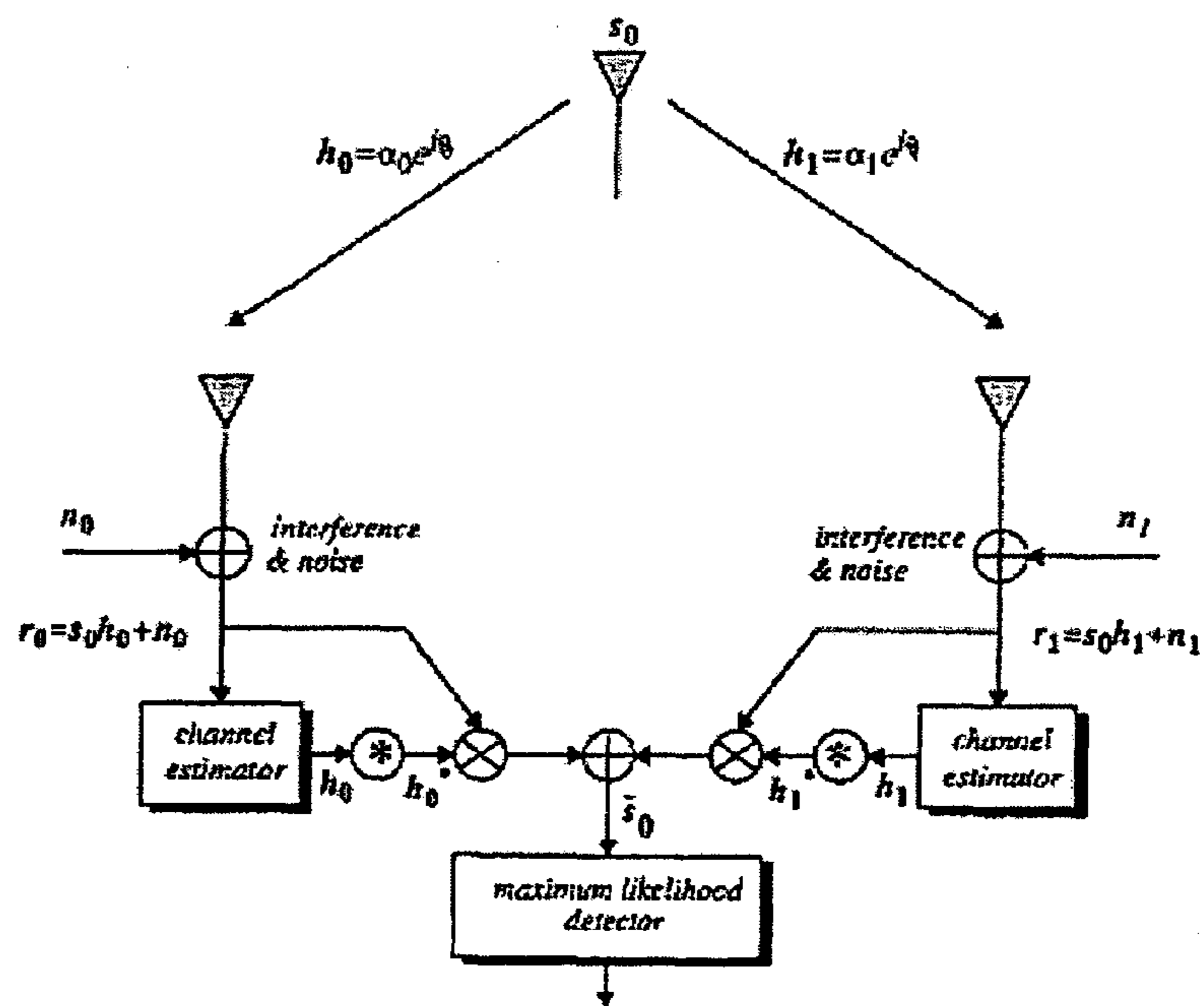
FIG. 2 (PRIOR ART)
