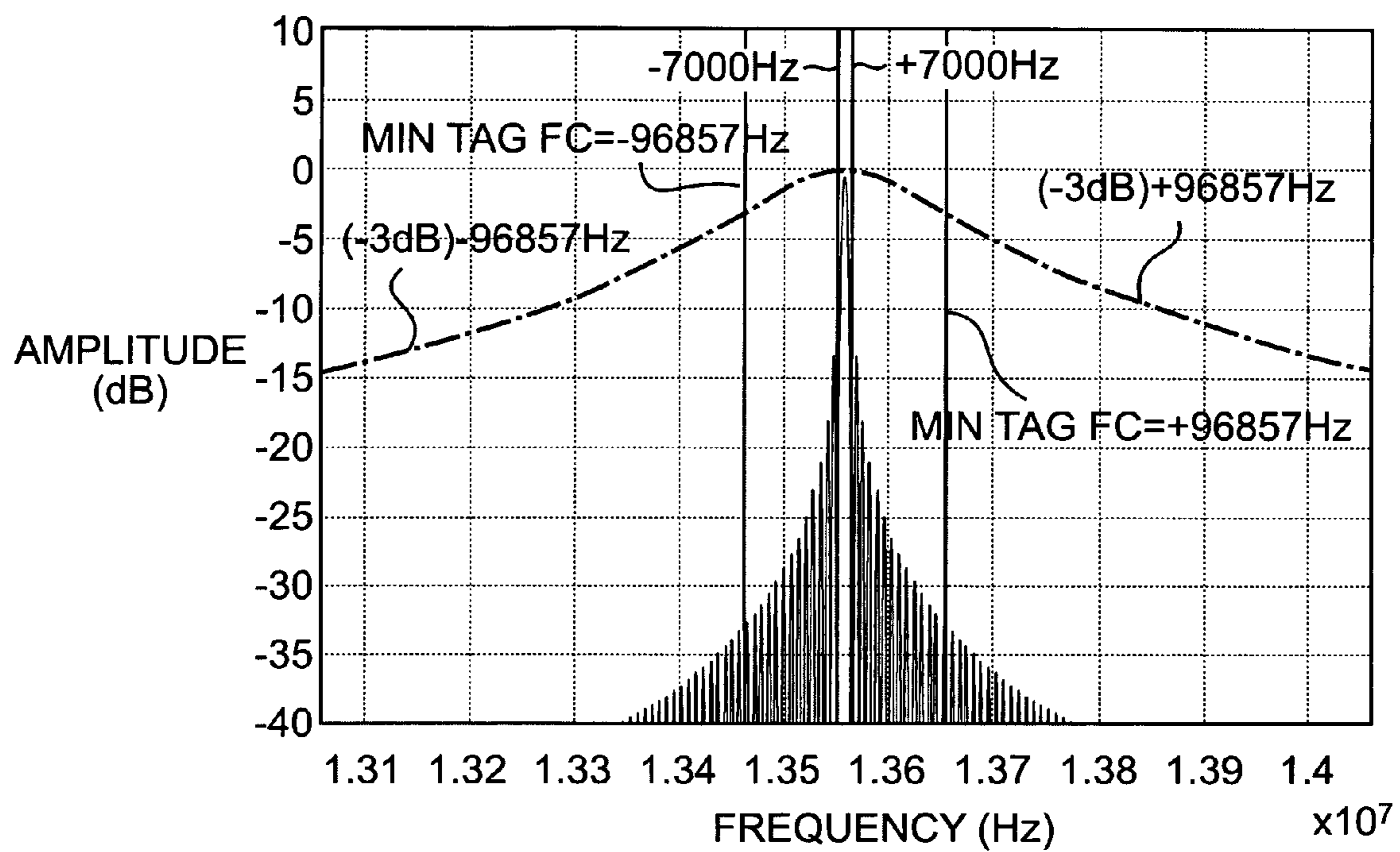
SPECTRUM OF TRANSMITTER OUTPUT WITH PULSE WIDTH OF 0.000143 SECONDS
