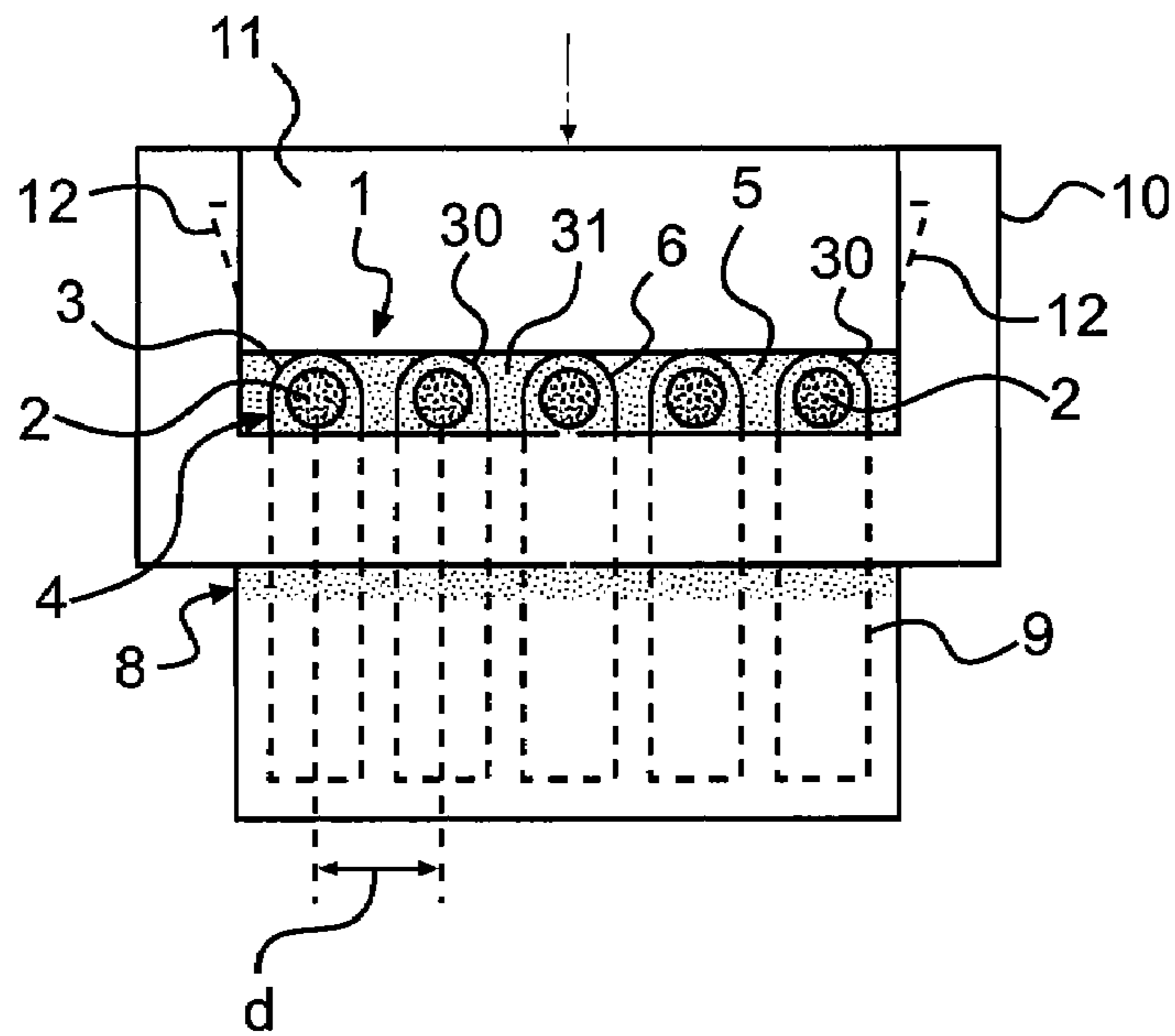
FIG. 2 PRIOR ART
