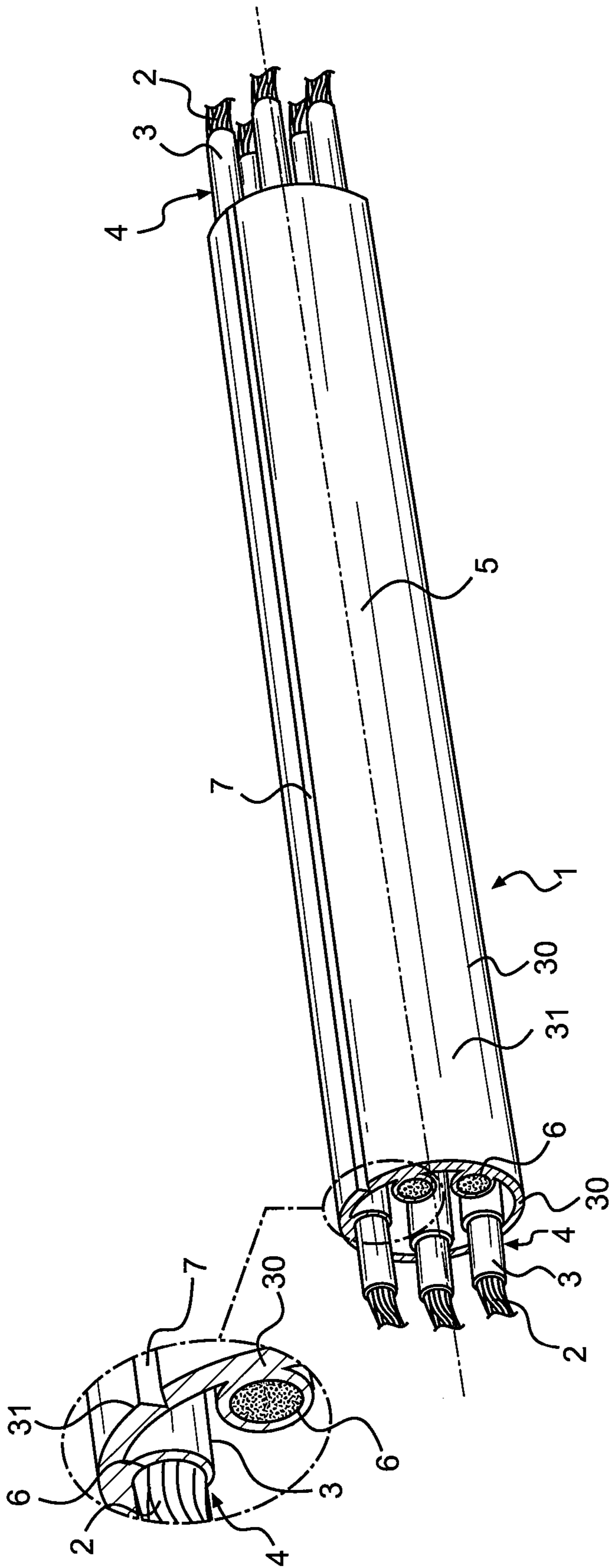
FIG. 9 PRIOR ART
