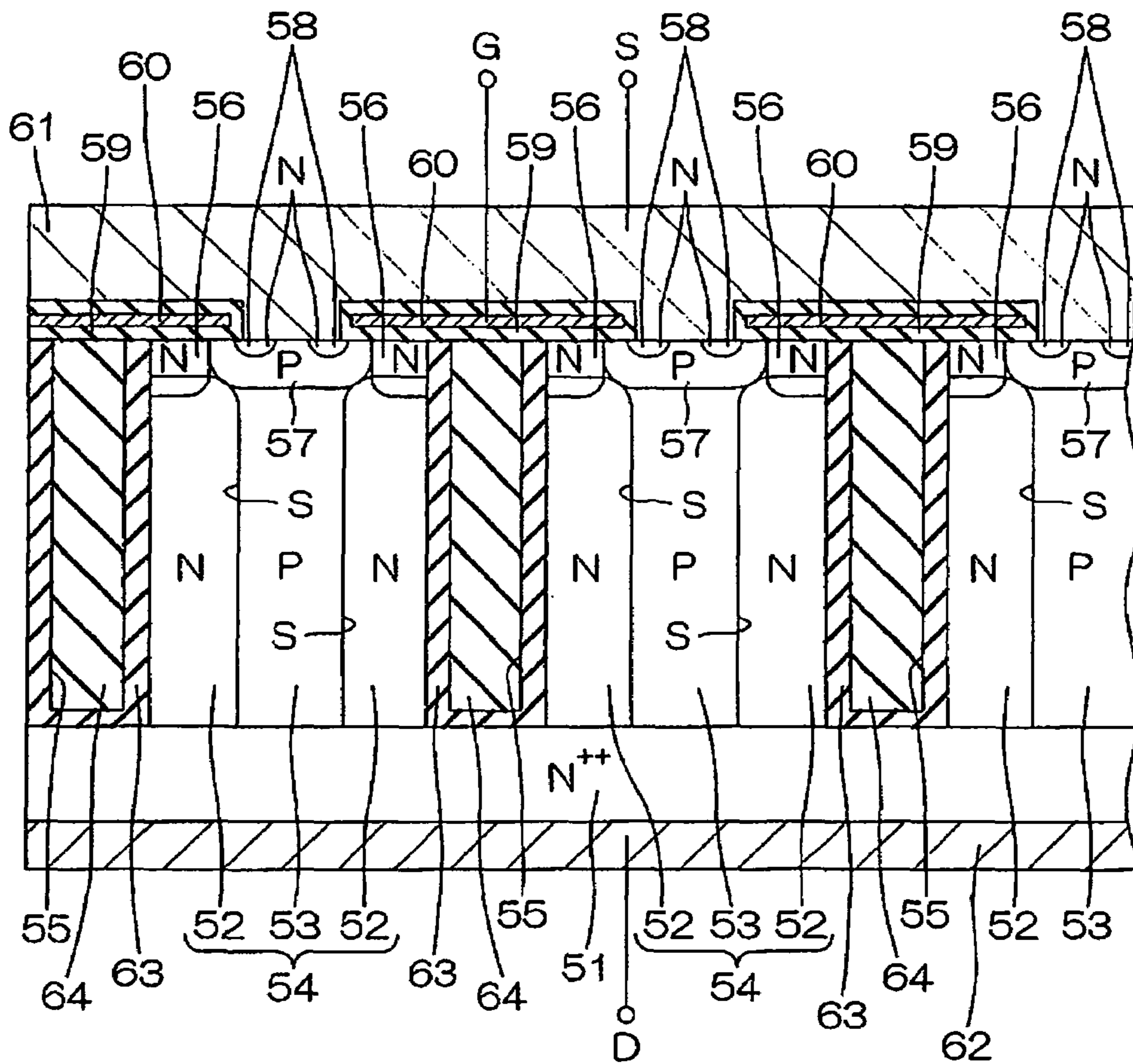
FIG. 6 PRIOR ART
