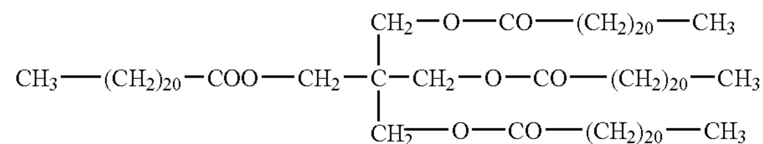
Compound 19
