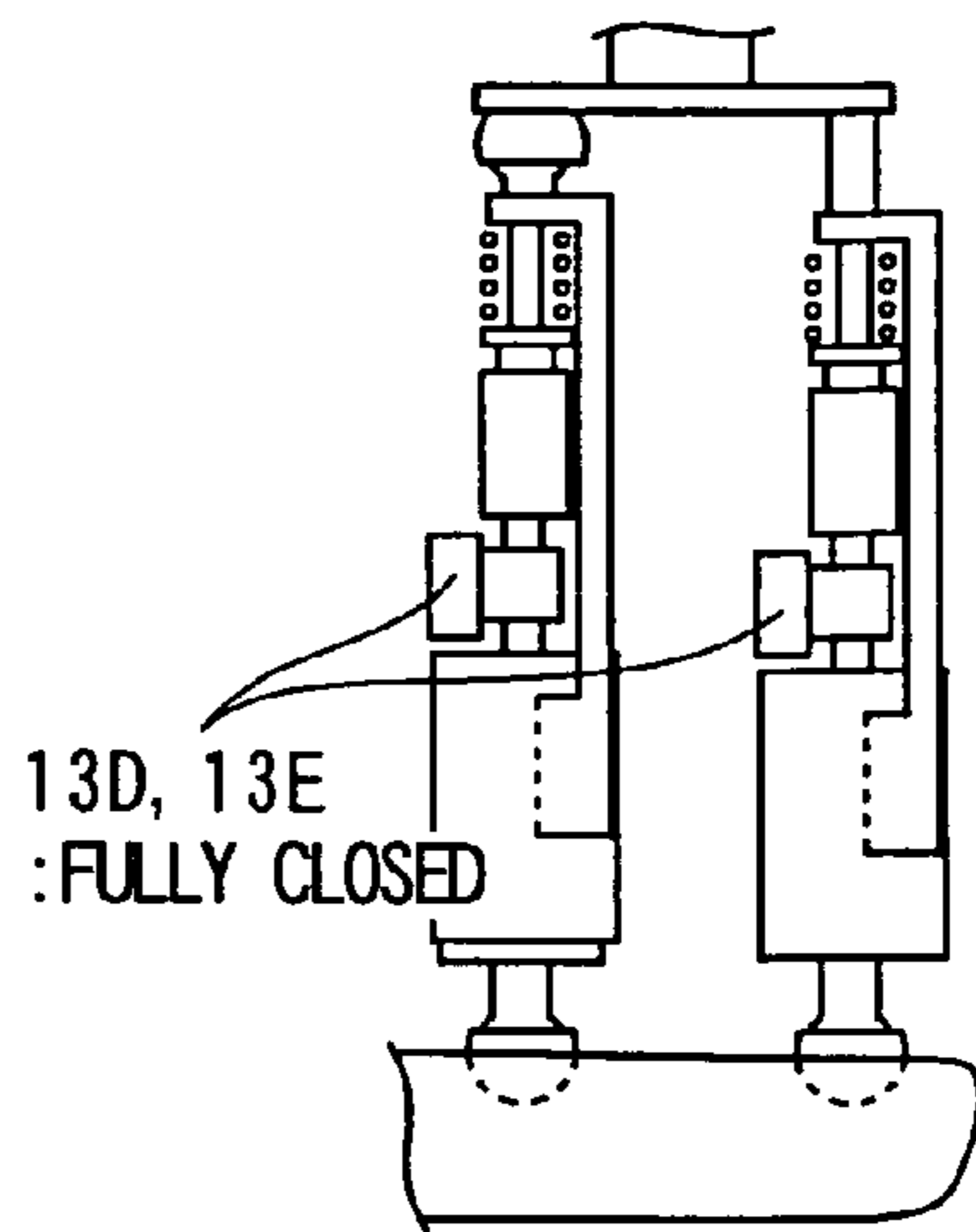
FIG. 11C DURING PRESSURE MAINTAINING TIME
