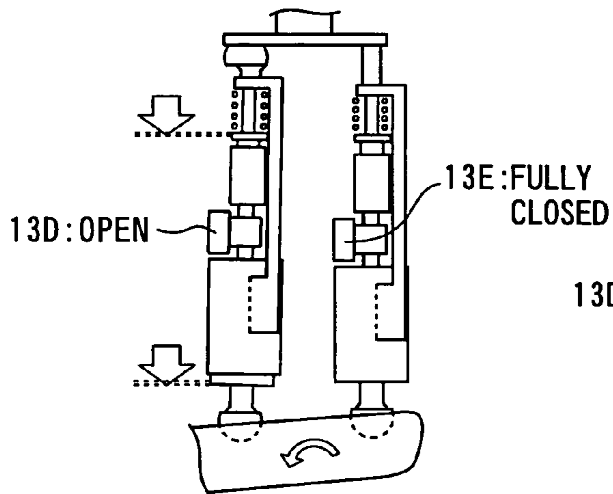
FIG. 11D DURING DOWNWARD ROTATION OF FOOT MEMBER (KICKING MOTION)
