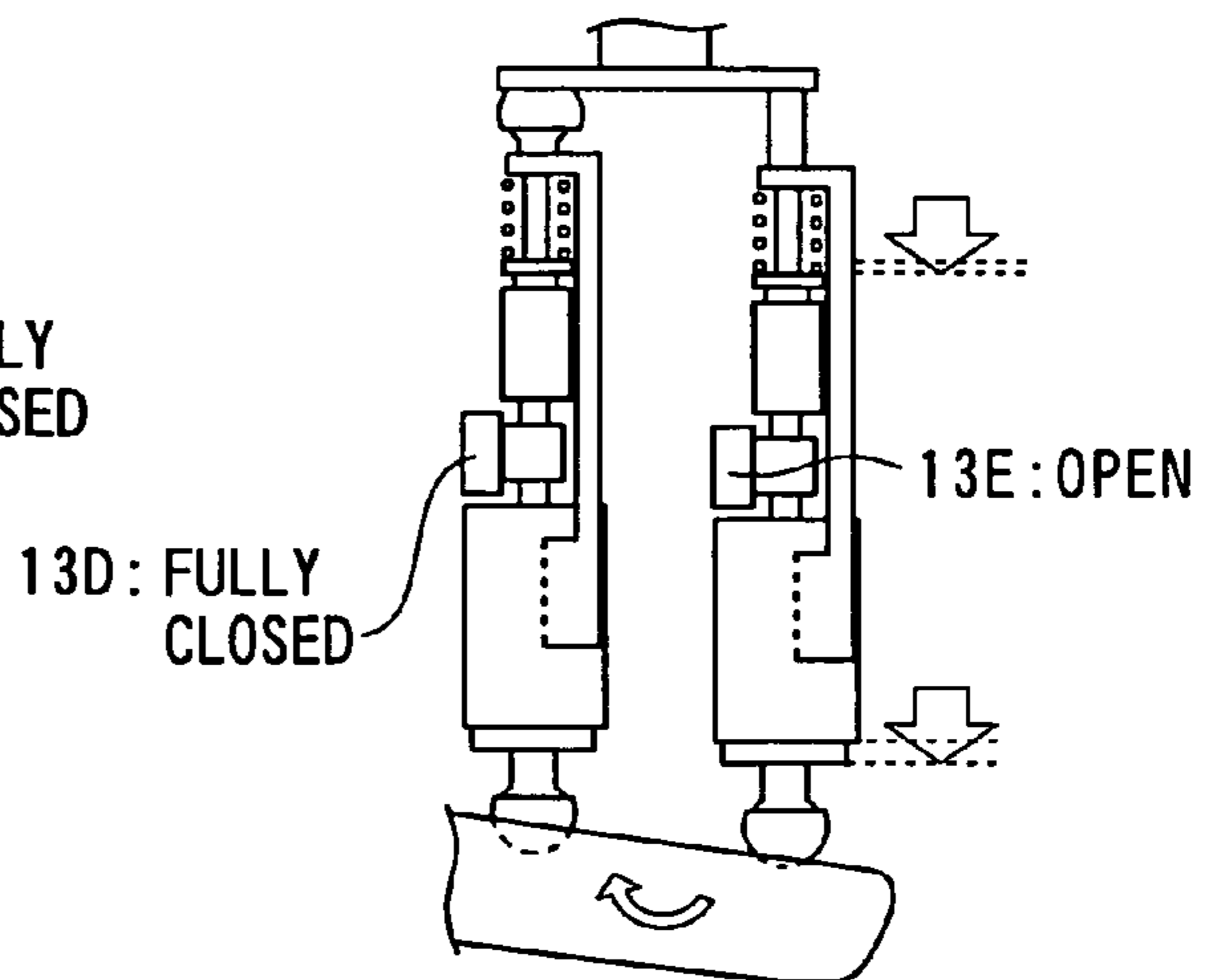
FIG. 11E DURING UPWARD ROTATION OF FOOT MEMBER (TOE-UP MOTION)
