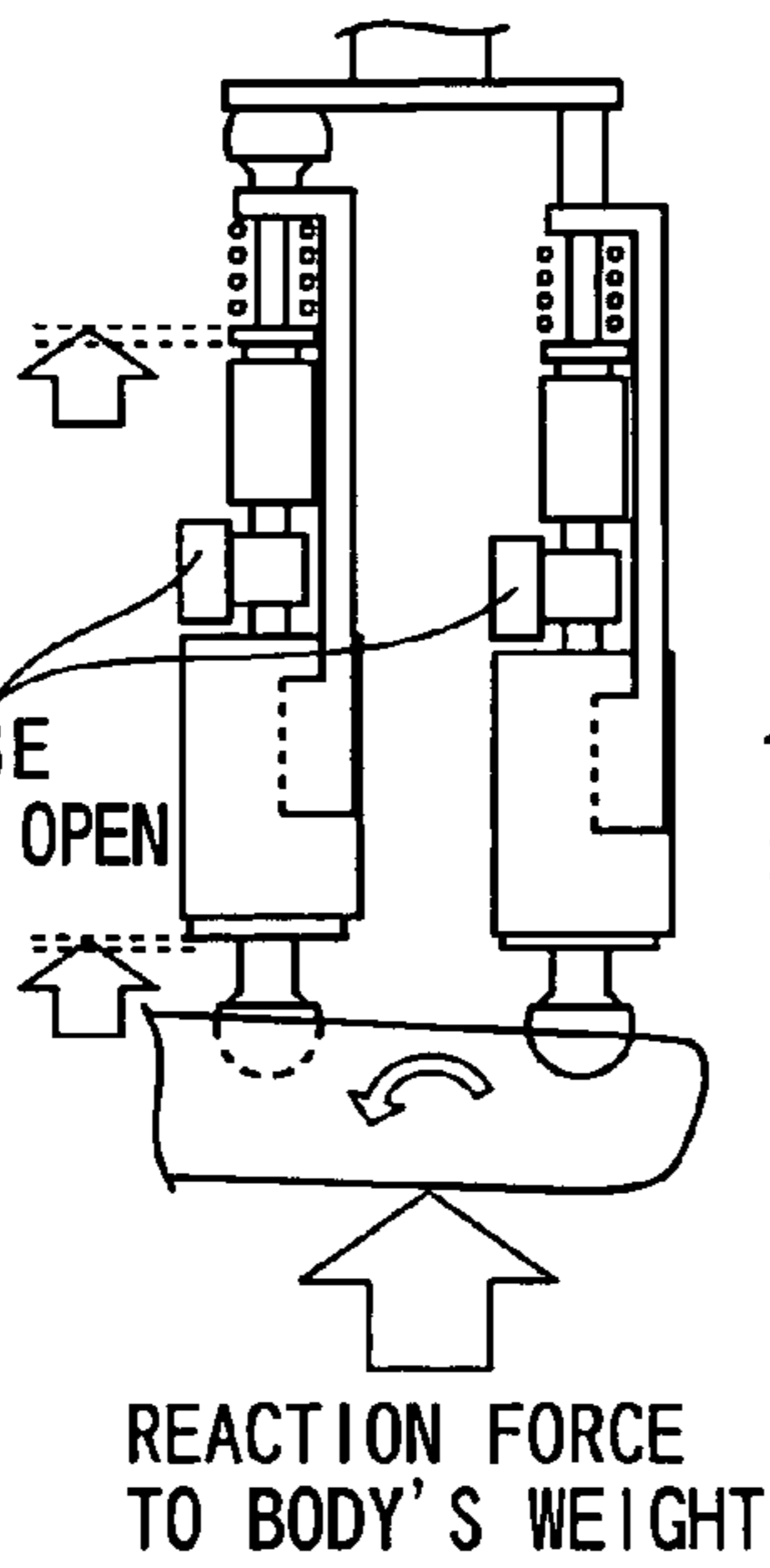
FIG. 11B DURING WEIGHT APPLICATION
