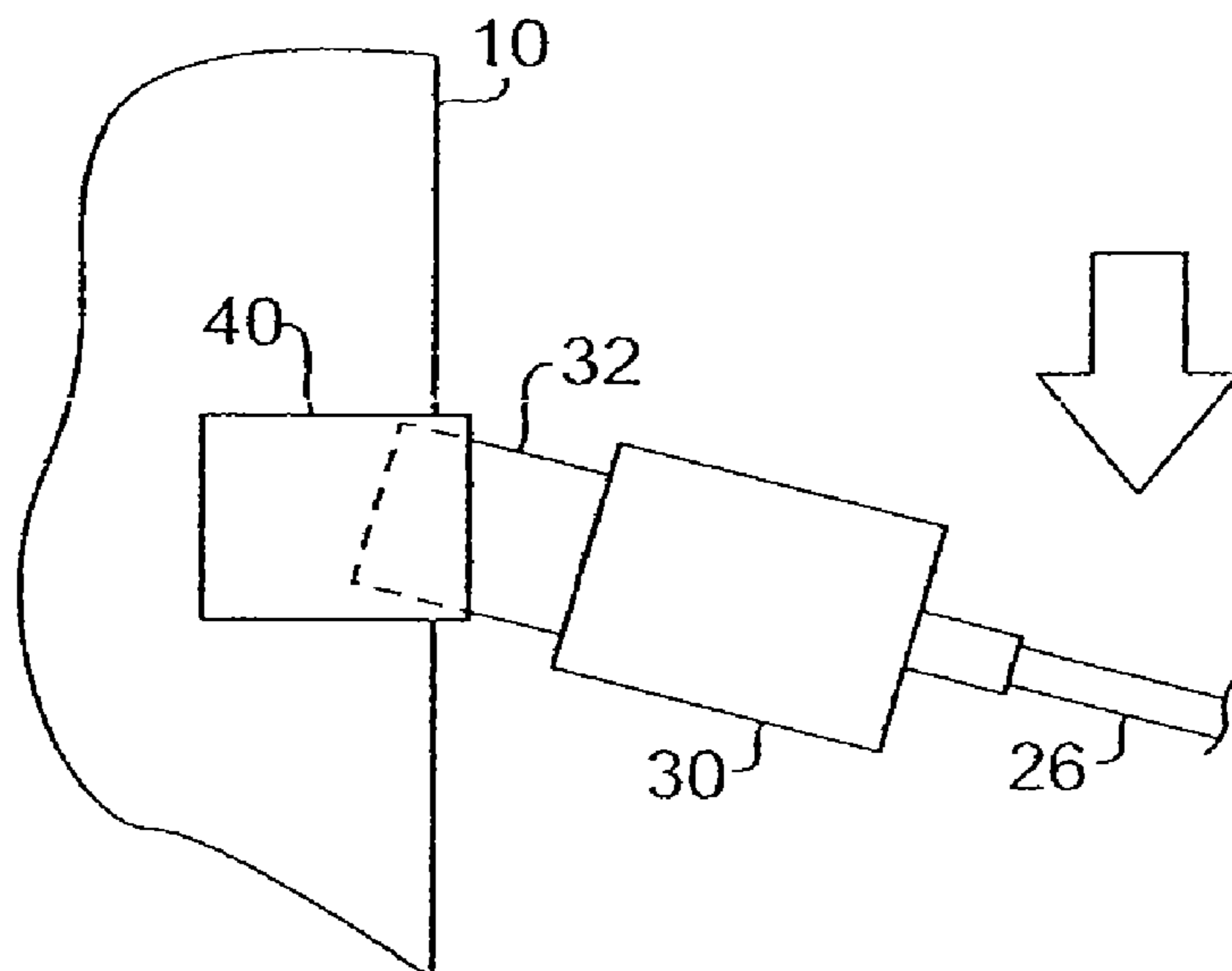
FIG. 2 (Prior Art)
