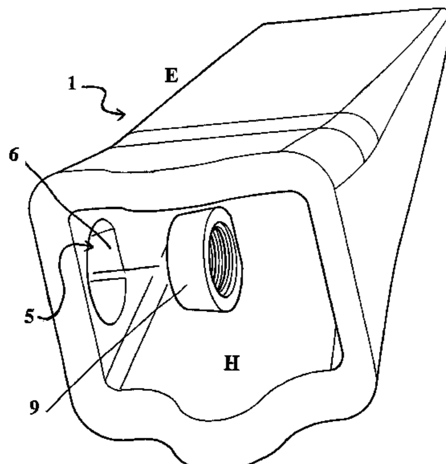
PIN RETAINER READY FOR INSTALLATION IN WEAR MEMBER
