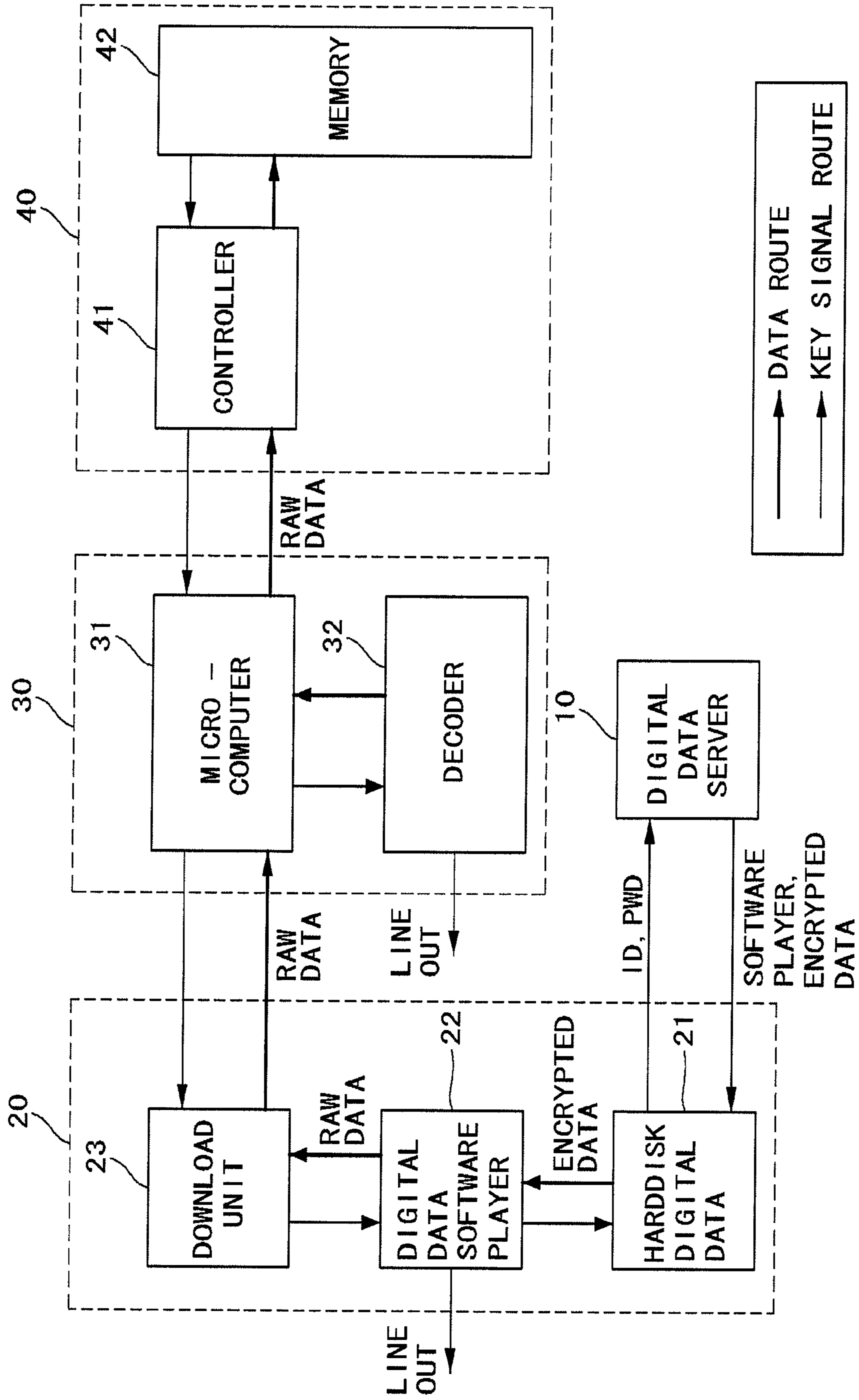
FIG.1 (CONVENTIONAL ART)
