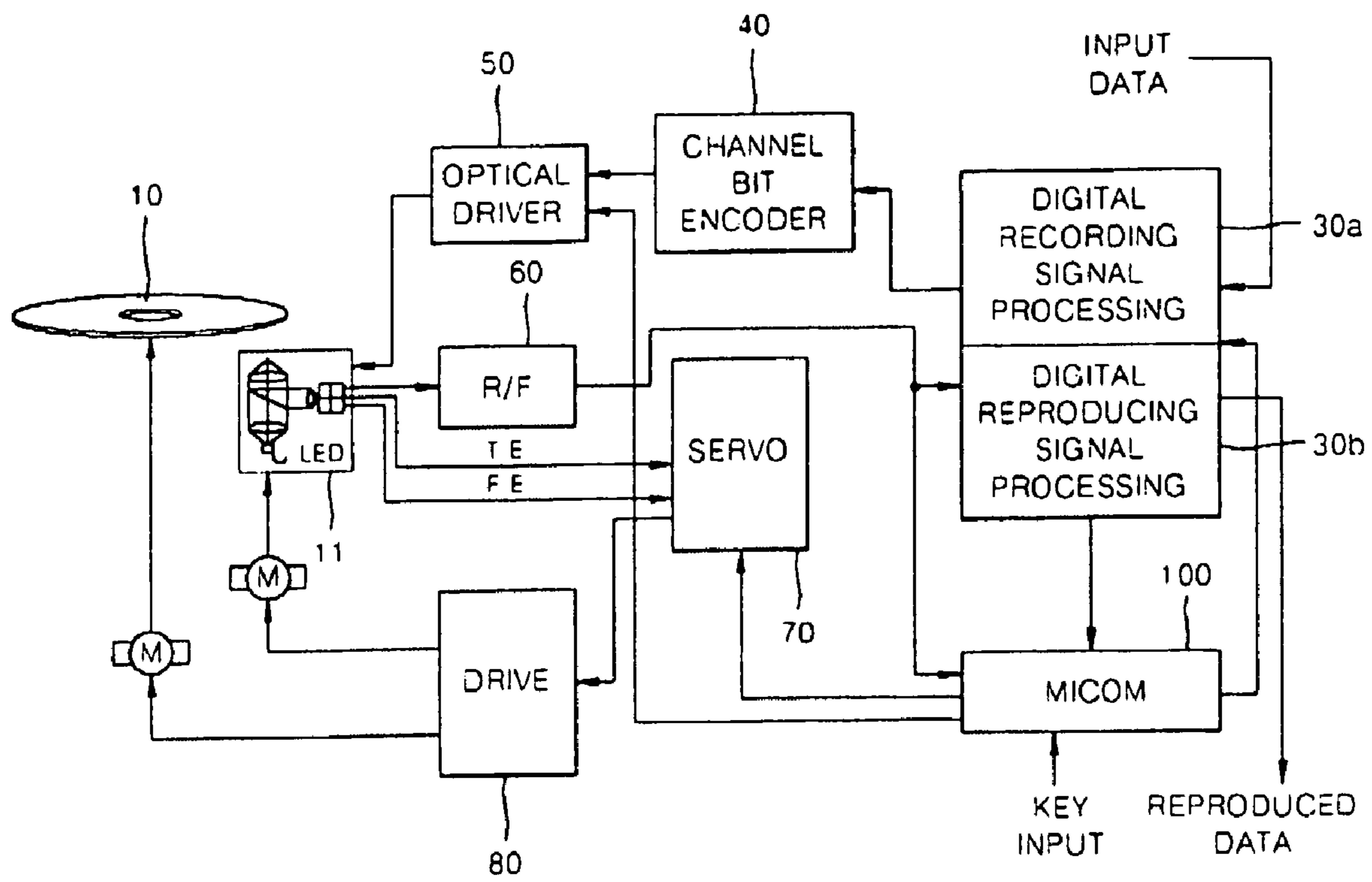
Fig. 1 Prior Art
