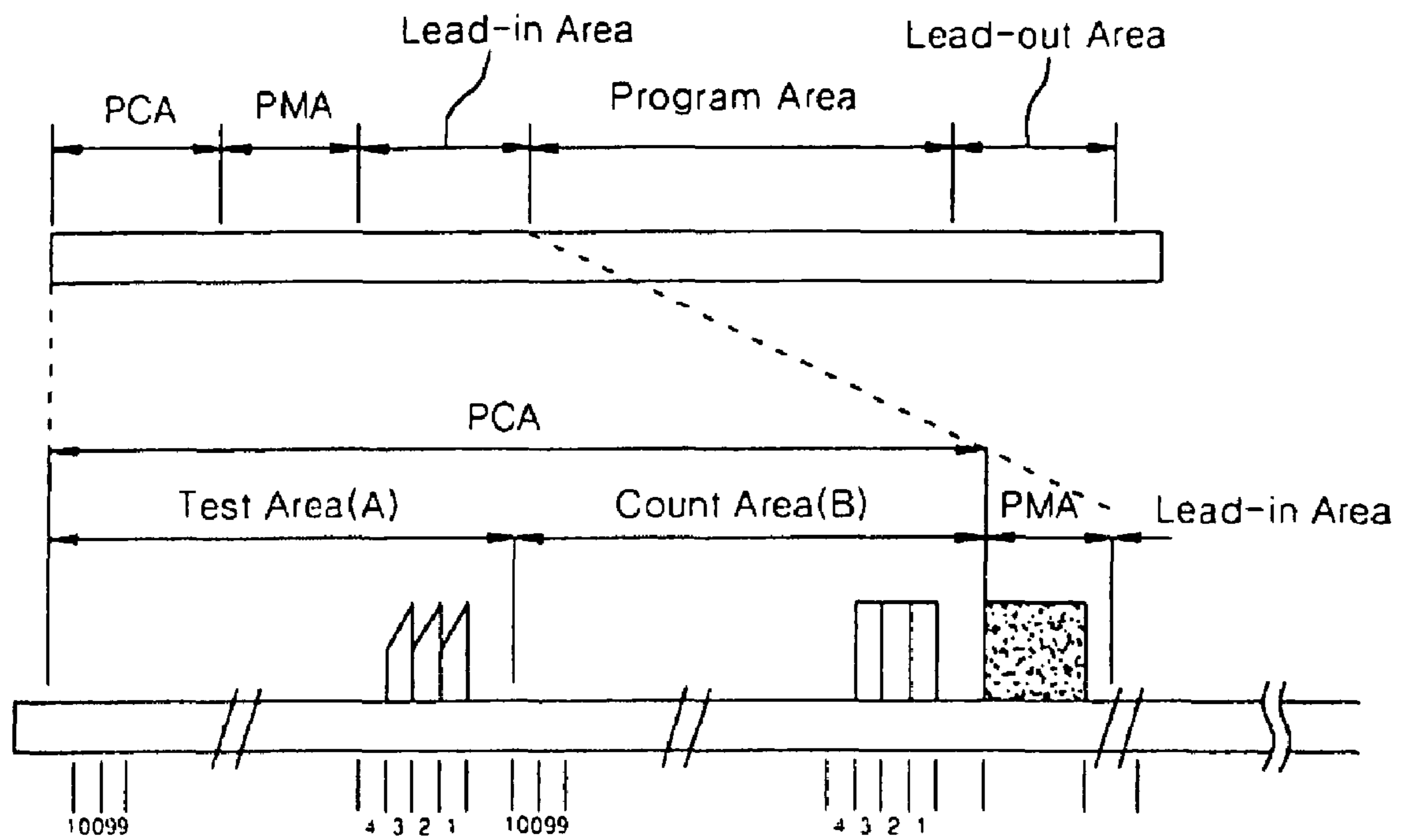
Fig.4 Prior Art
