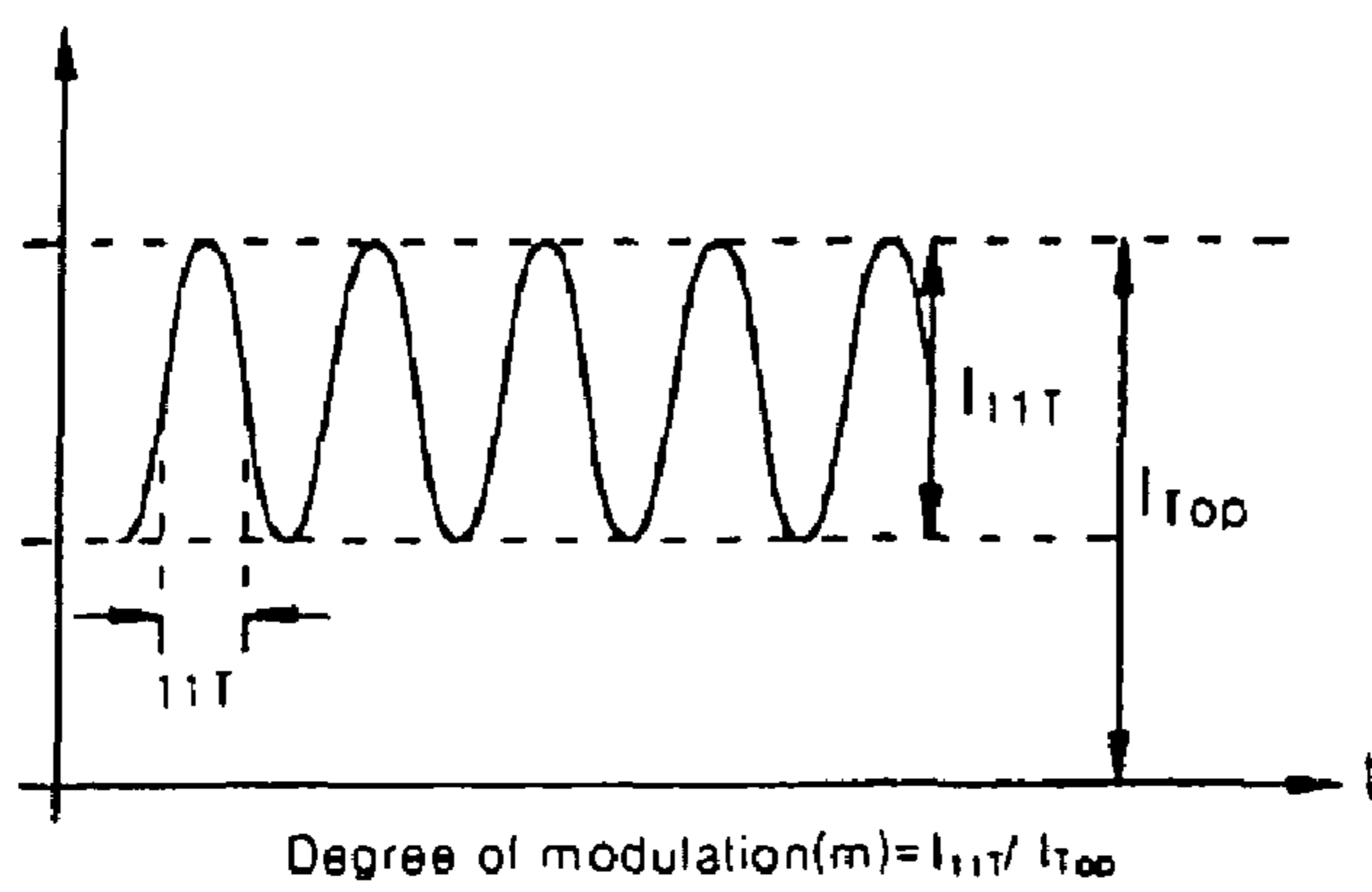
Fig.5 Prior Art
