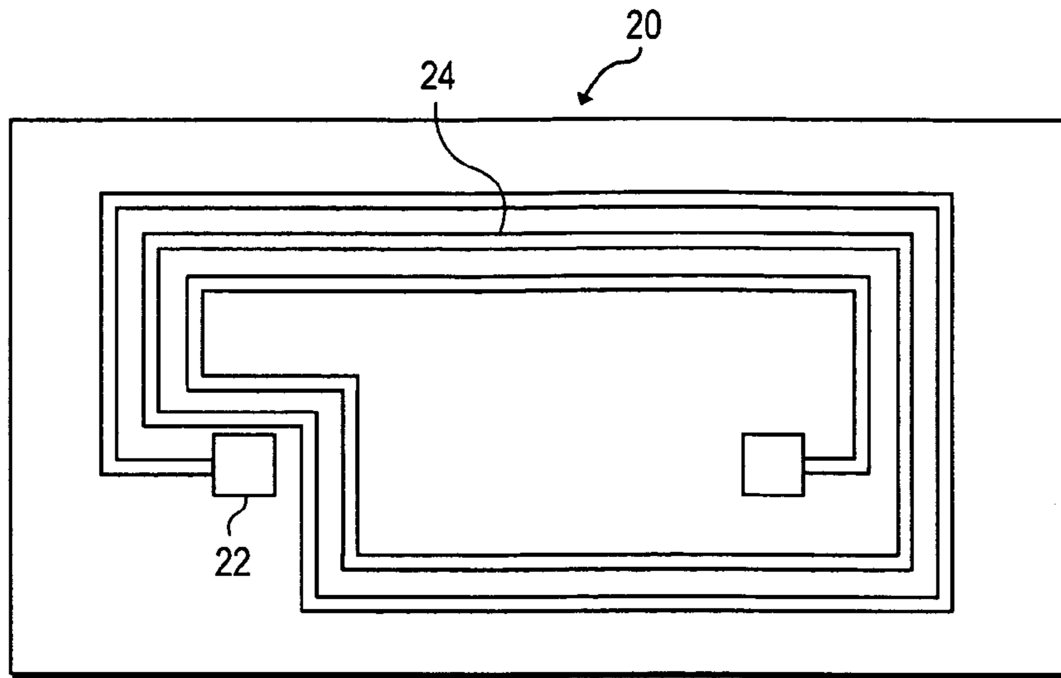
FIG. 1 (PRIOR ART)
