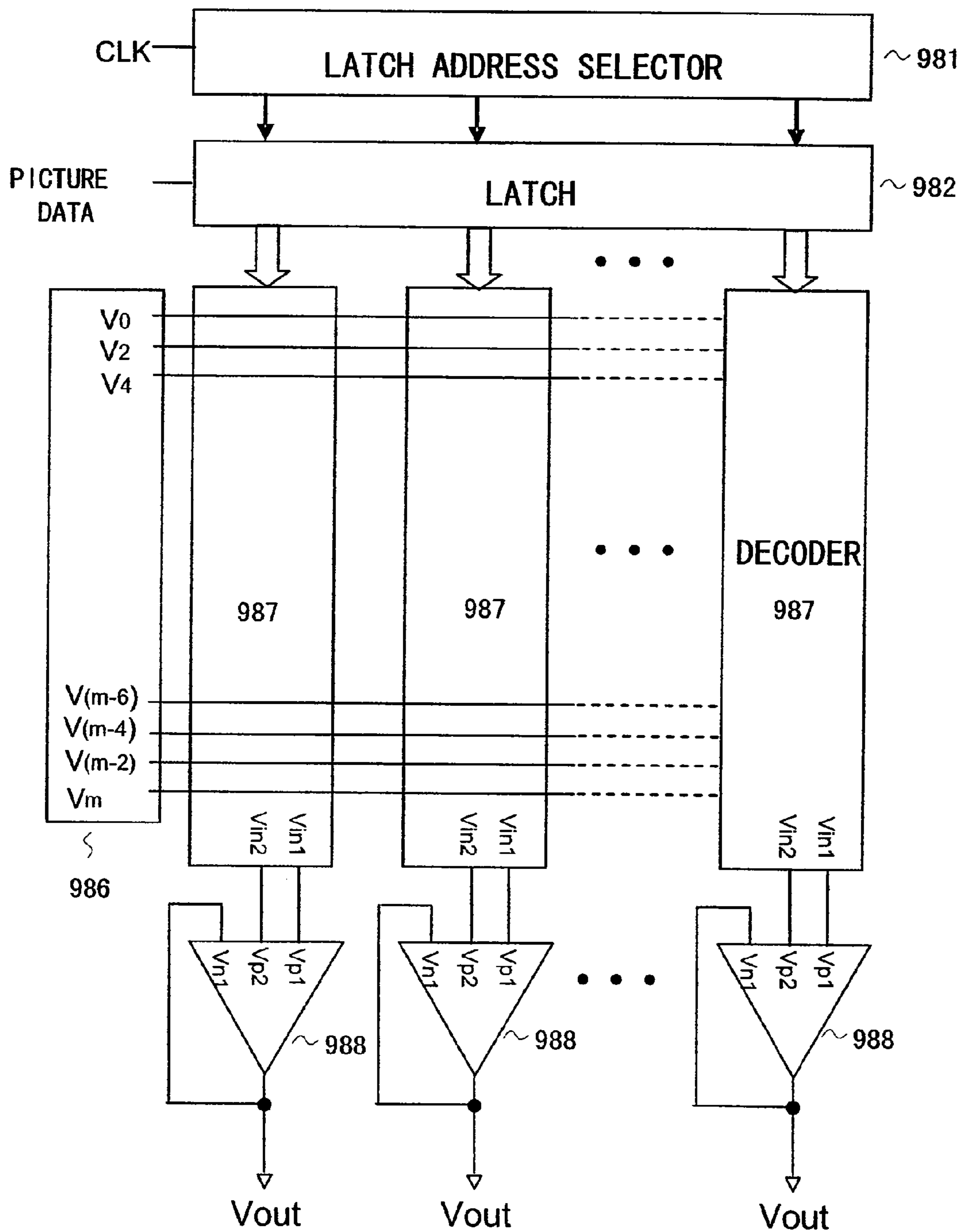
FIG. 17 PRIOR ART
