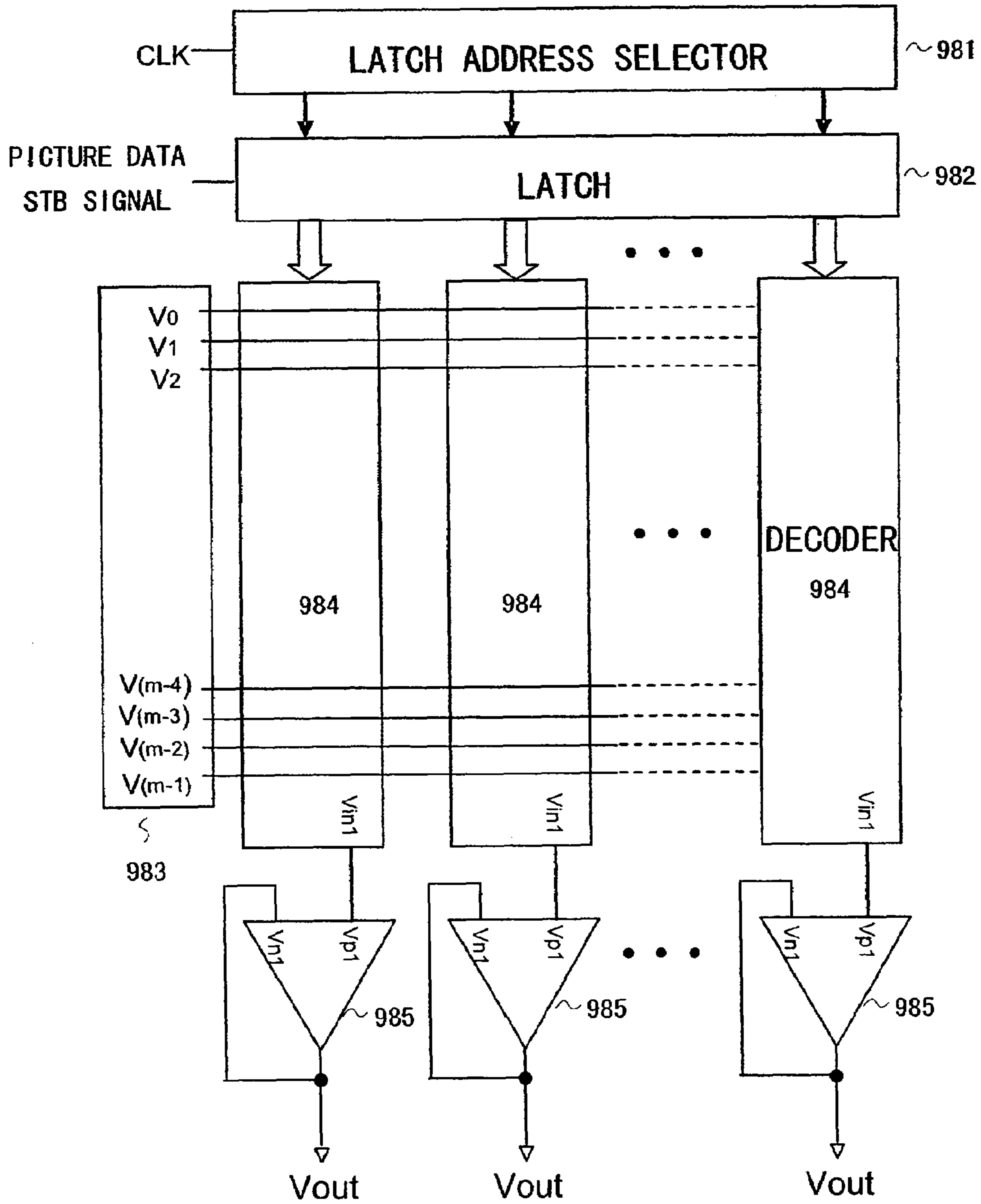
FIG. 16 PRIOR ART
