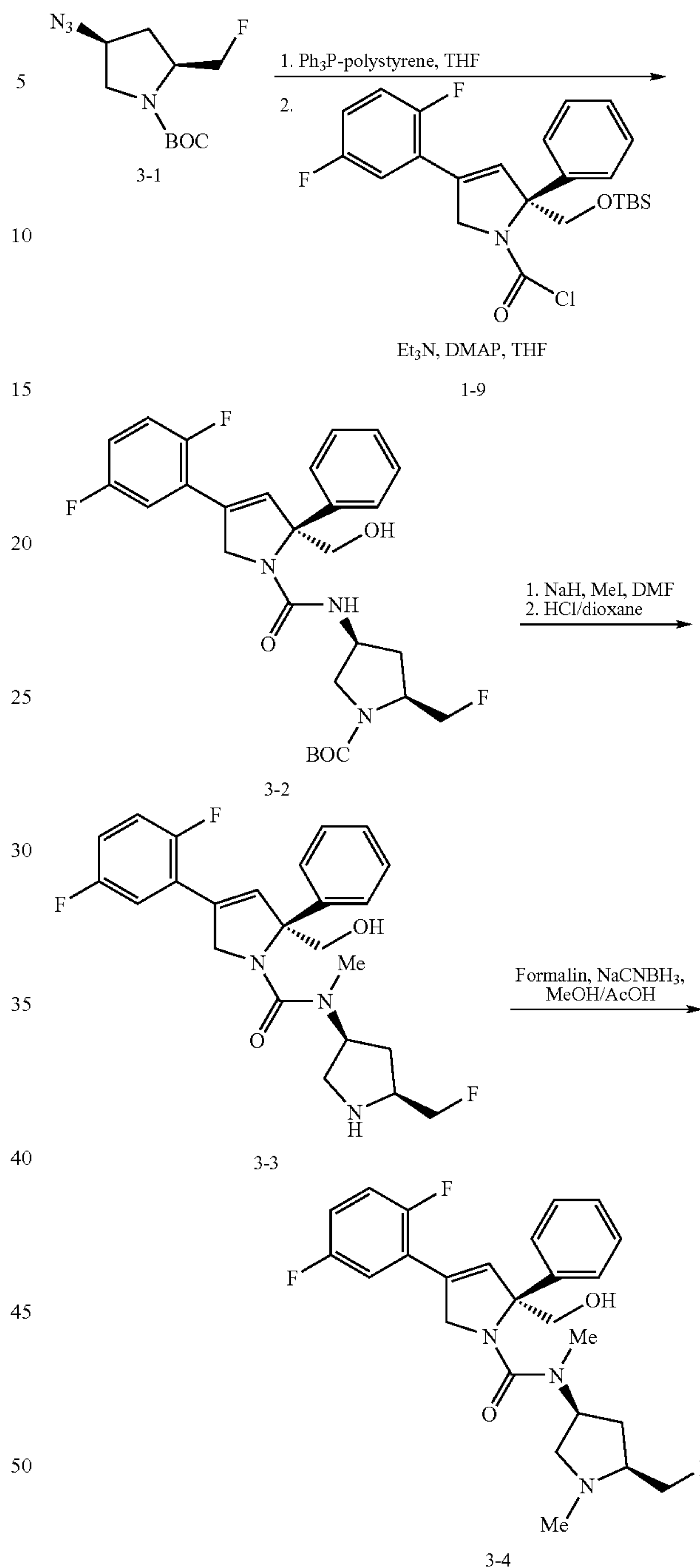
SCHEME 3
