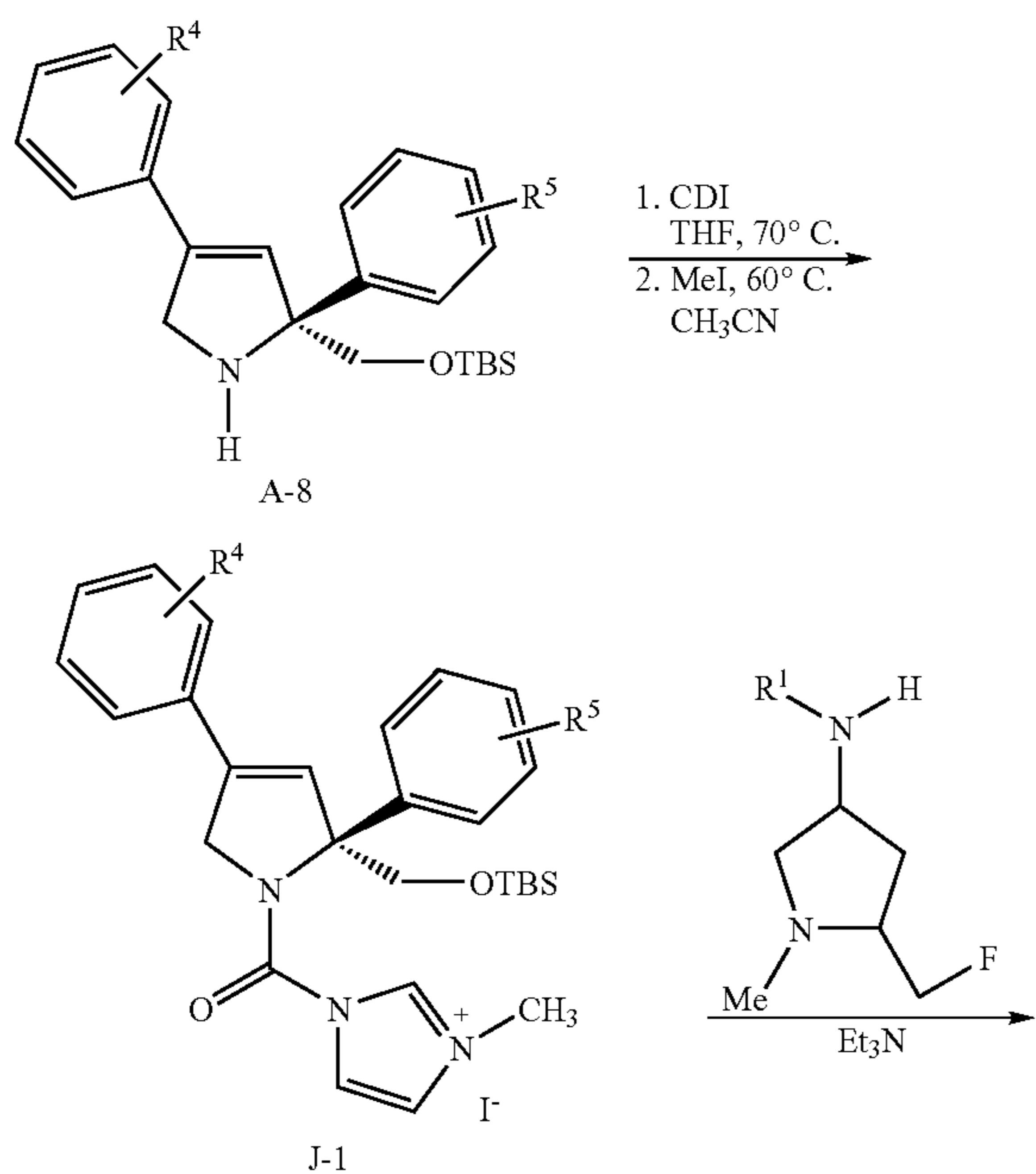
SCHEME I
