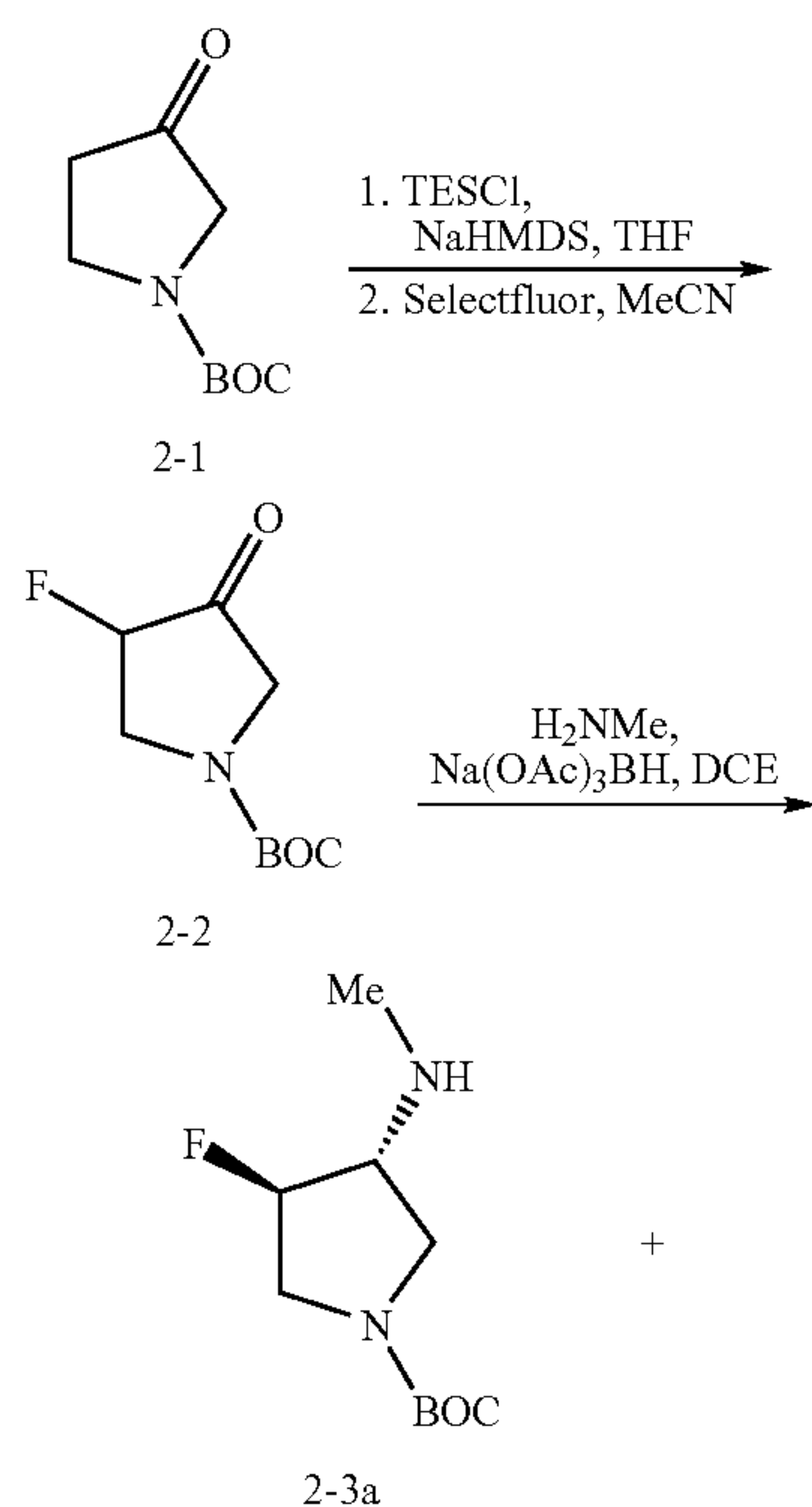
SCHEME 2
