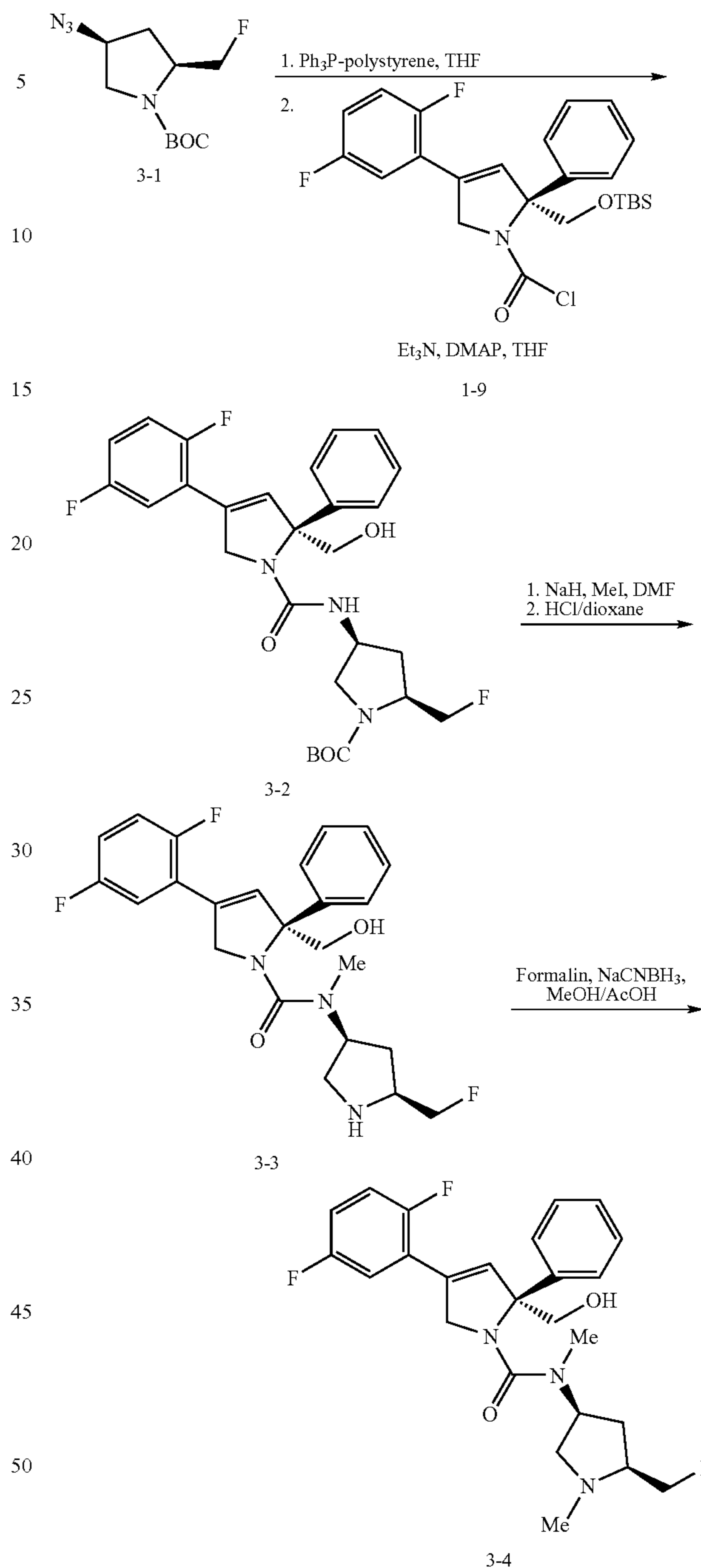
SCHEME 3
