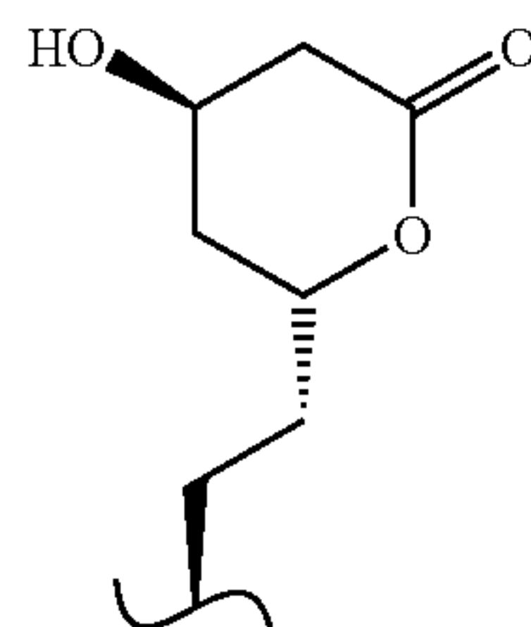
Lactone I
