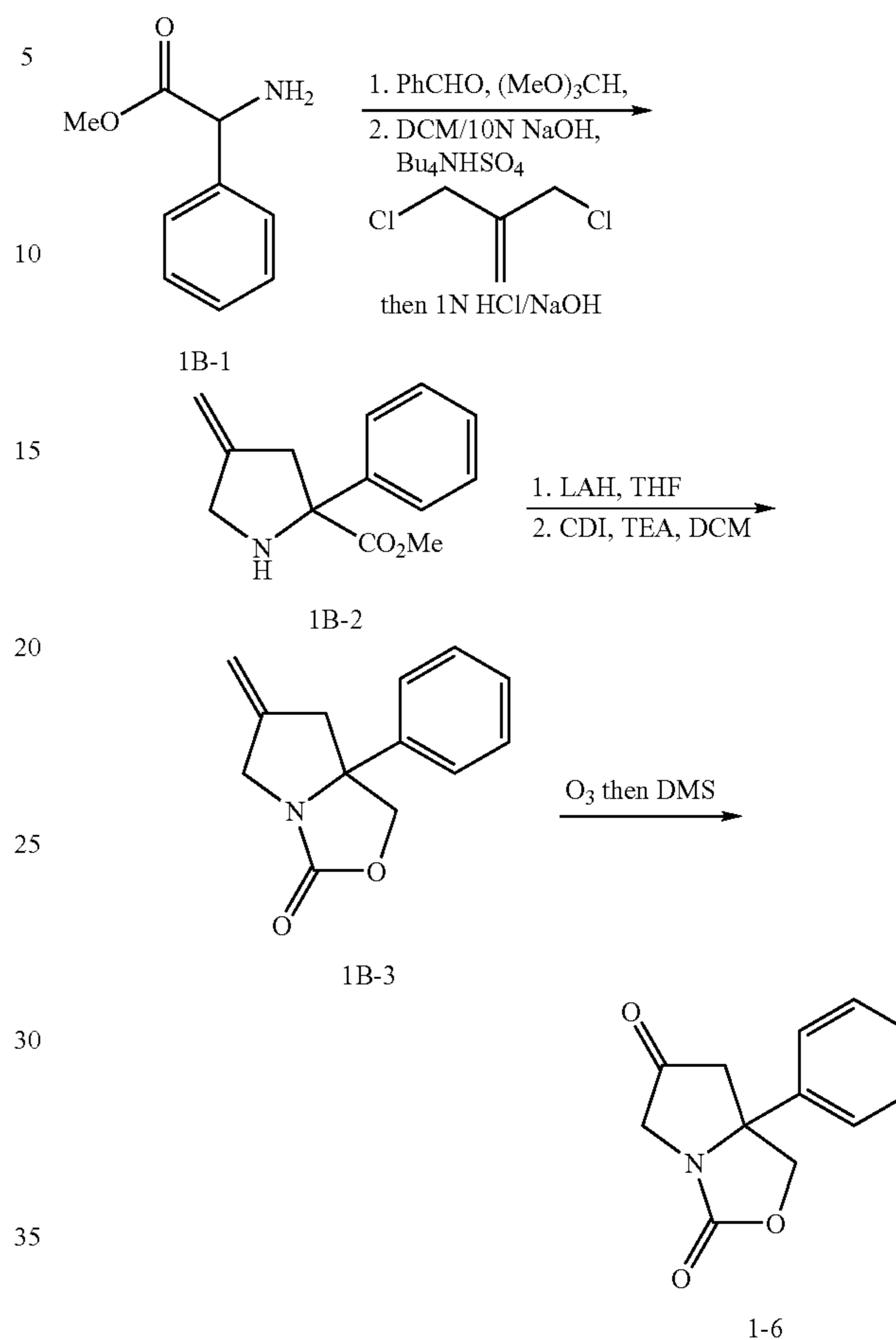
SCHEME 1B
