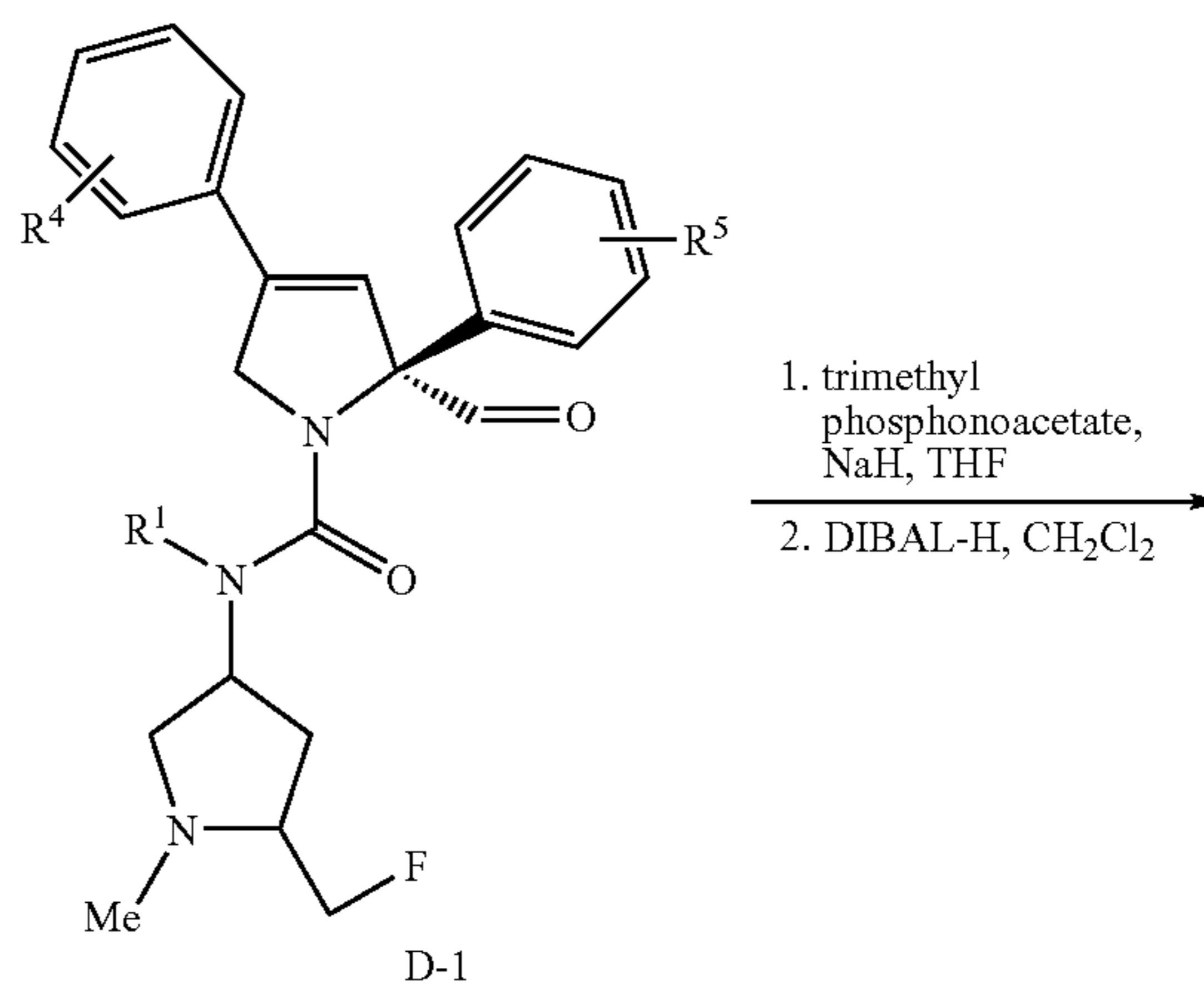
SCHEME K
