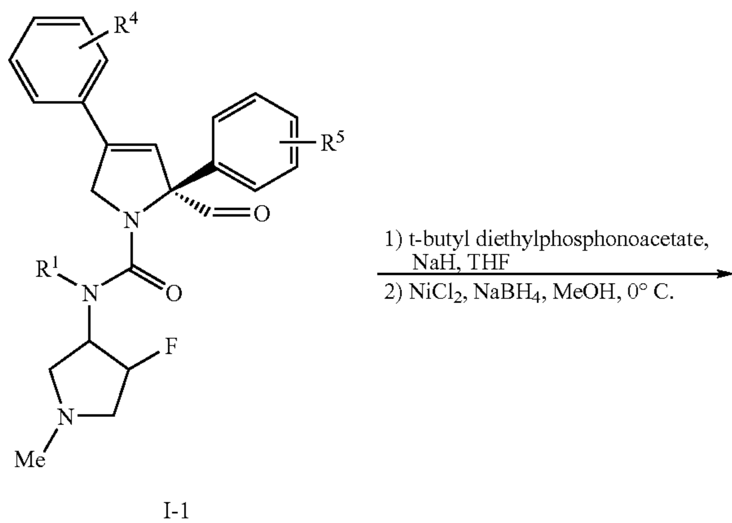
SCHEME N
