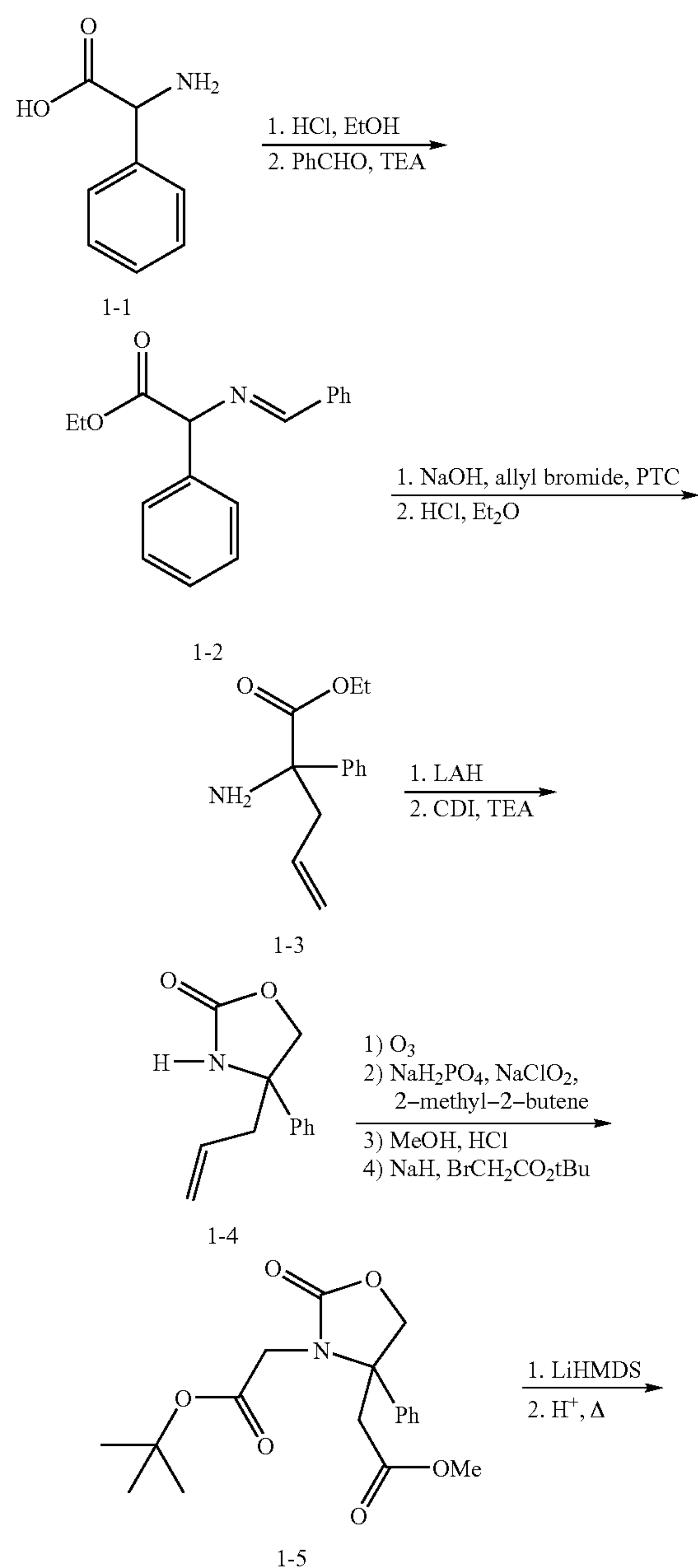
SCHEME 1
