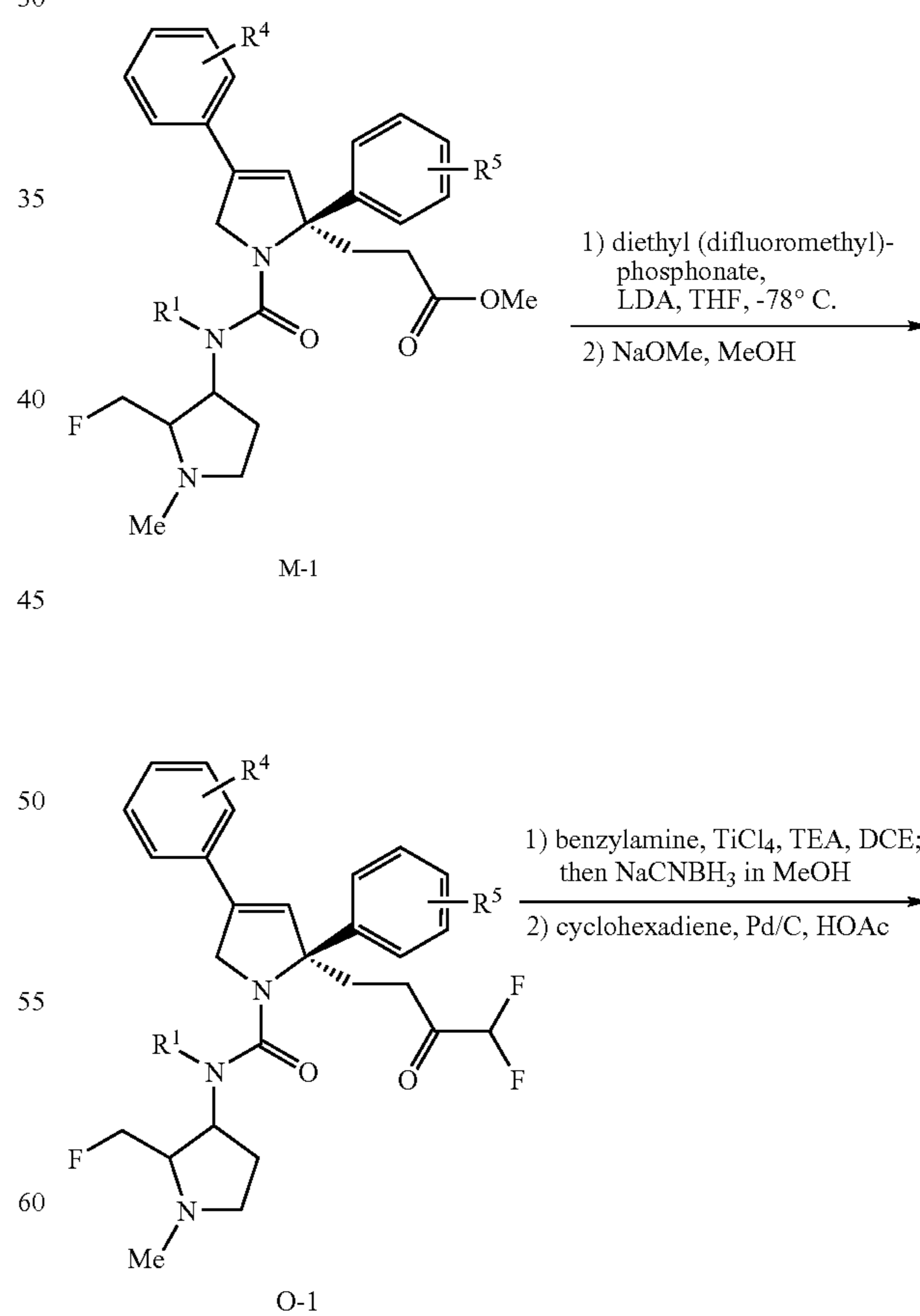
SCHEME O
