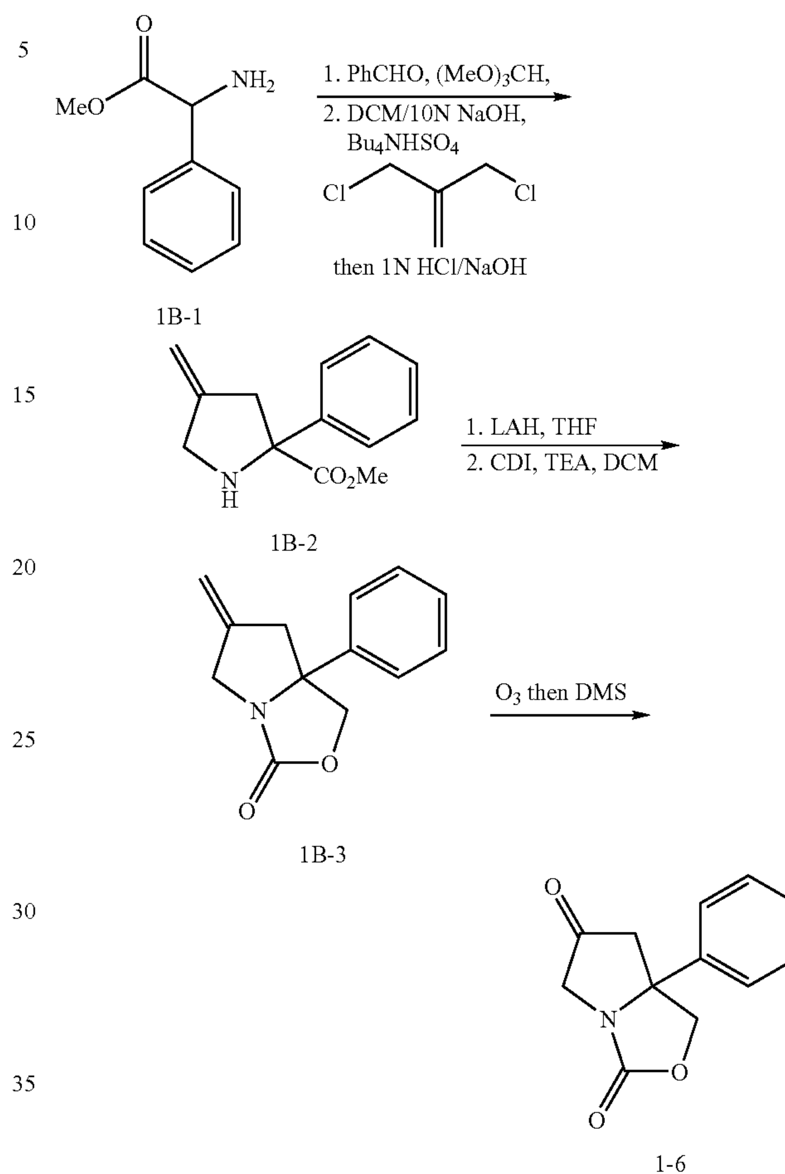
SCHEME 1B
