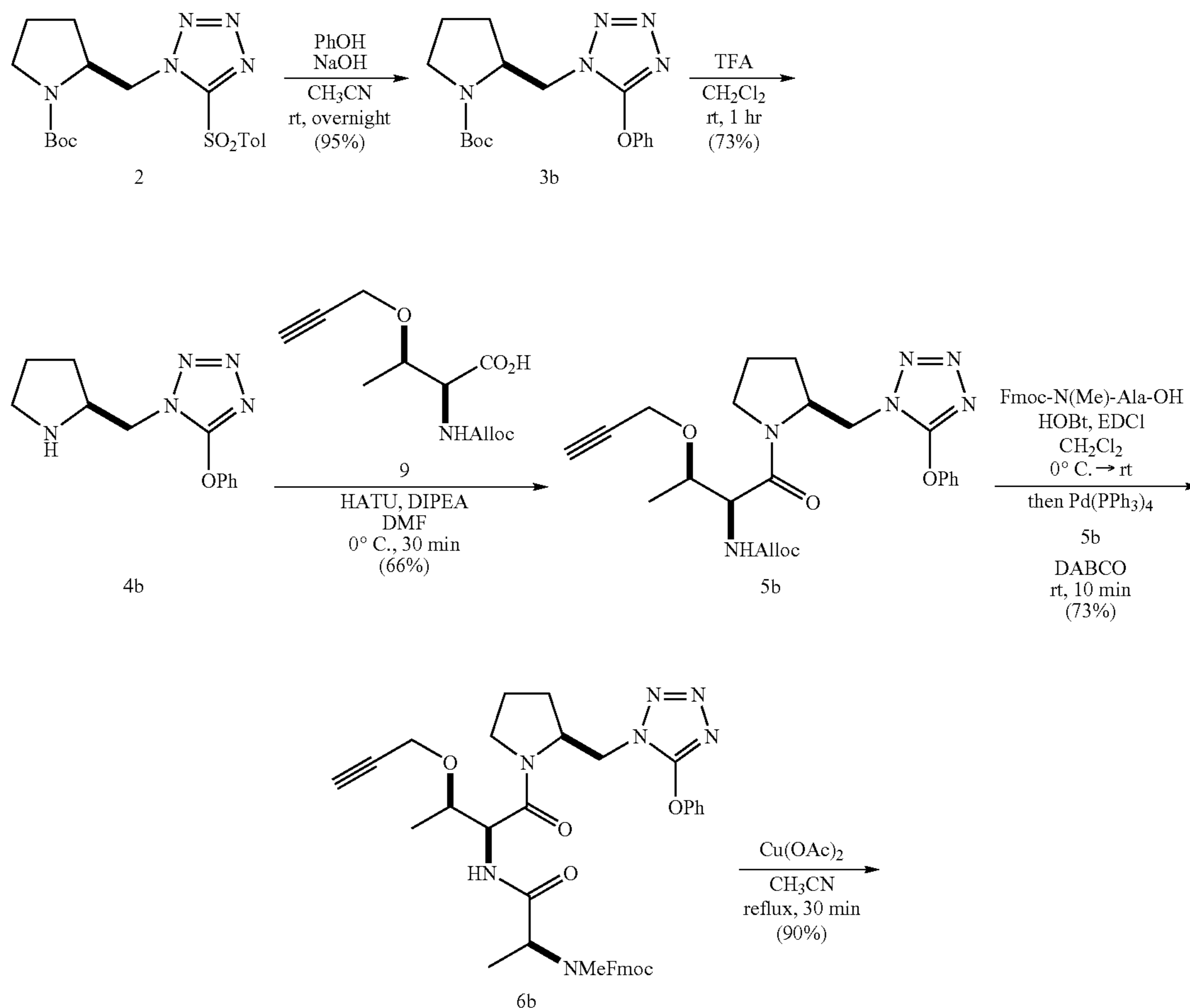
Scheme 2
