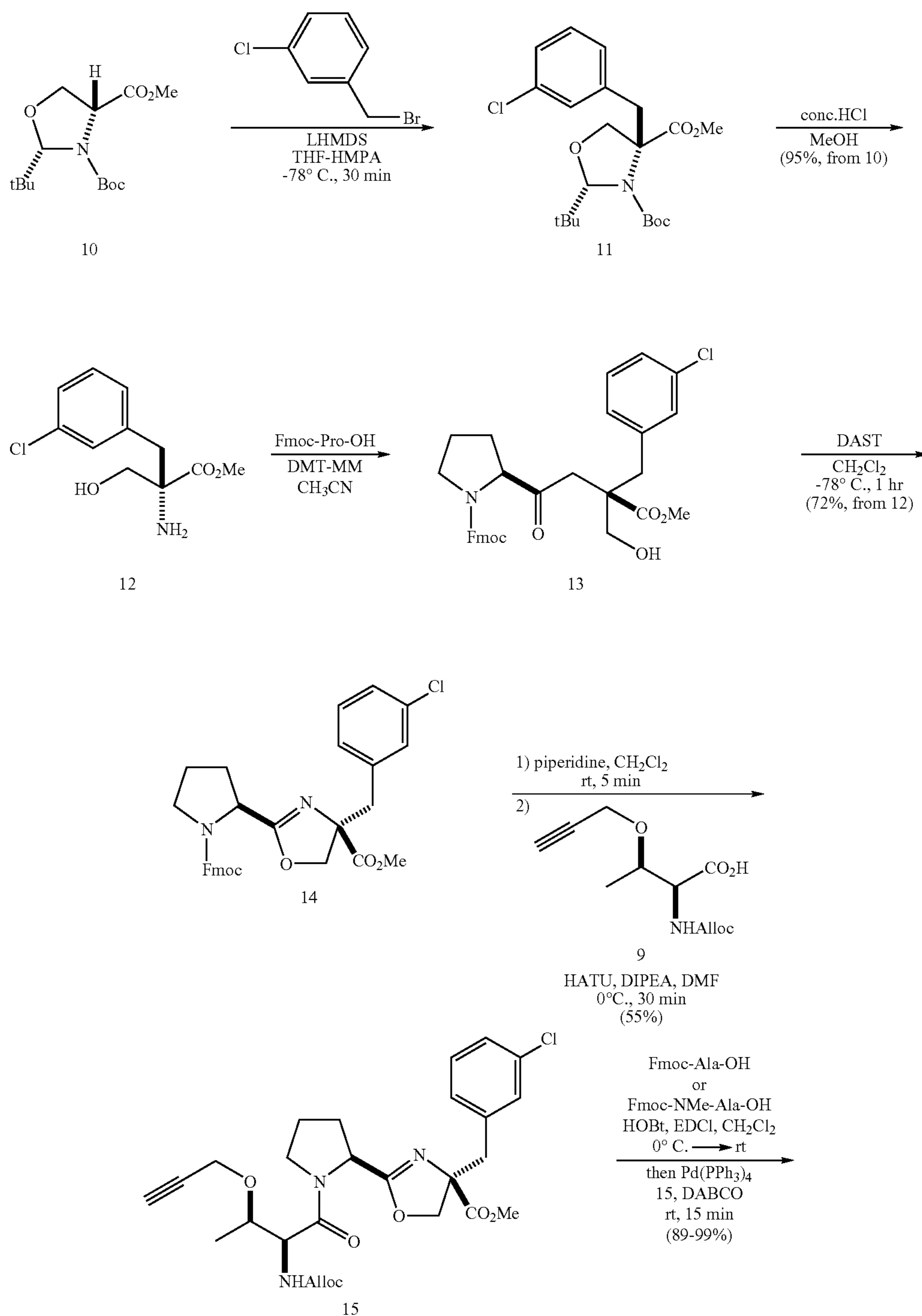
Scheme 6
