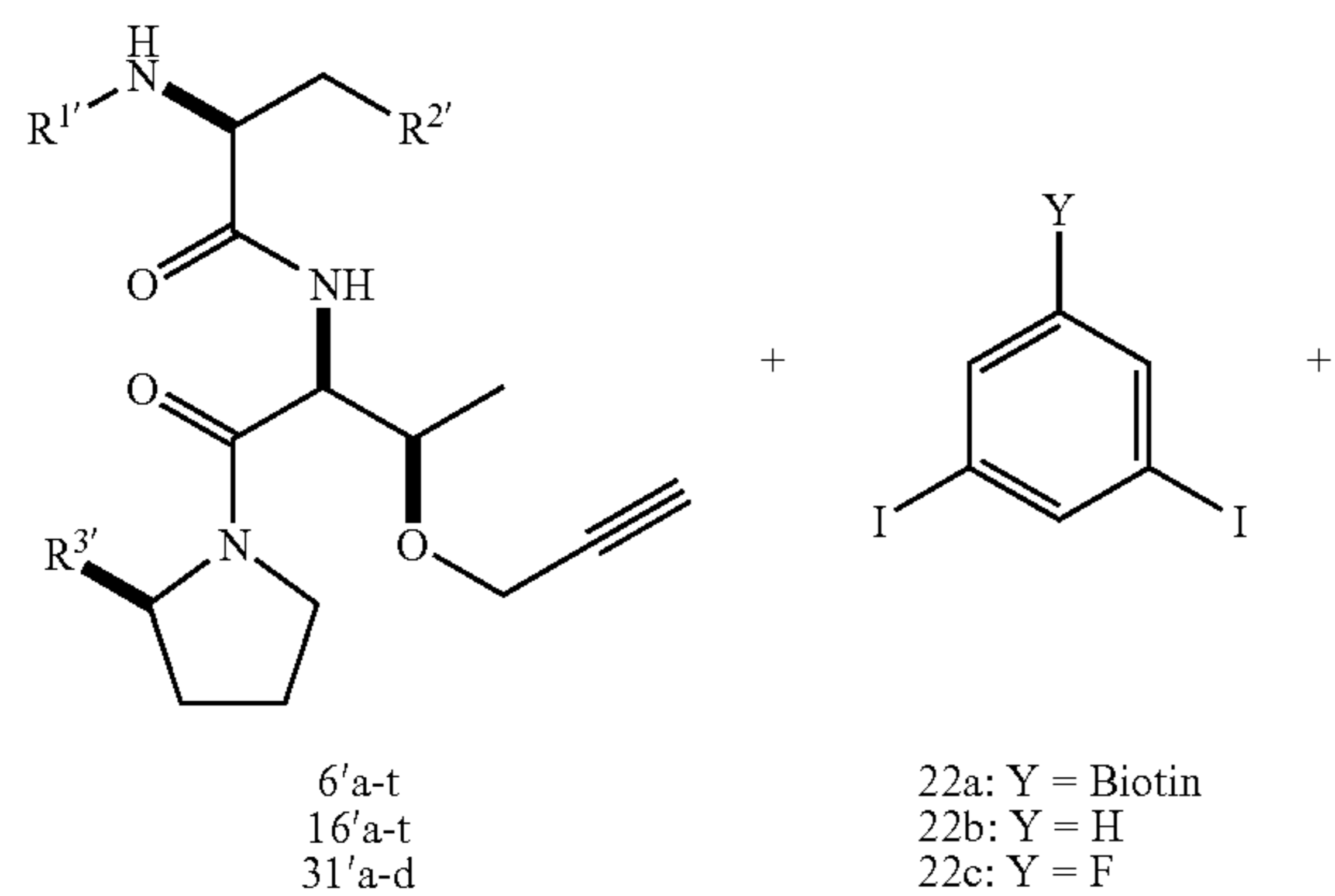
Scheme 13
