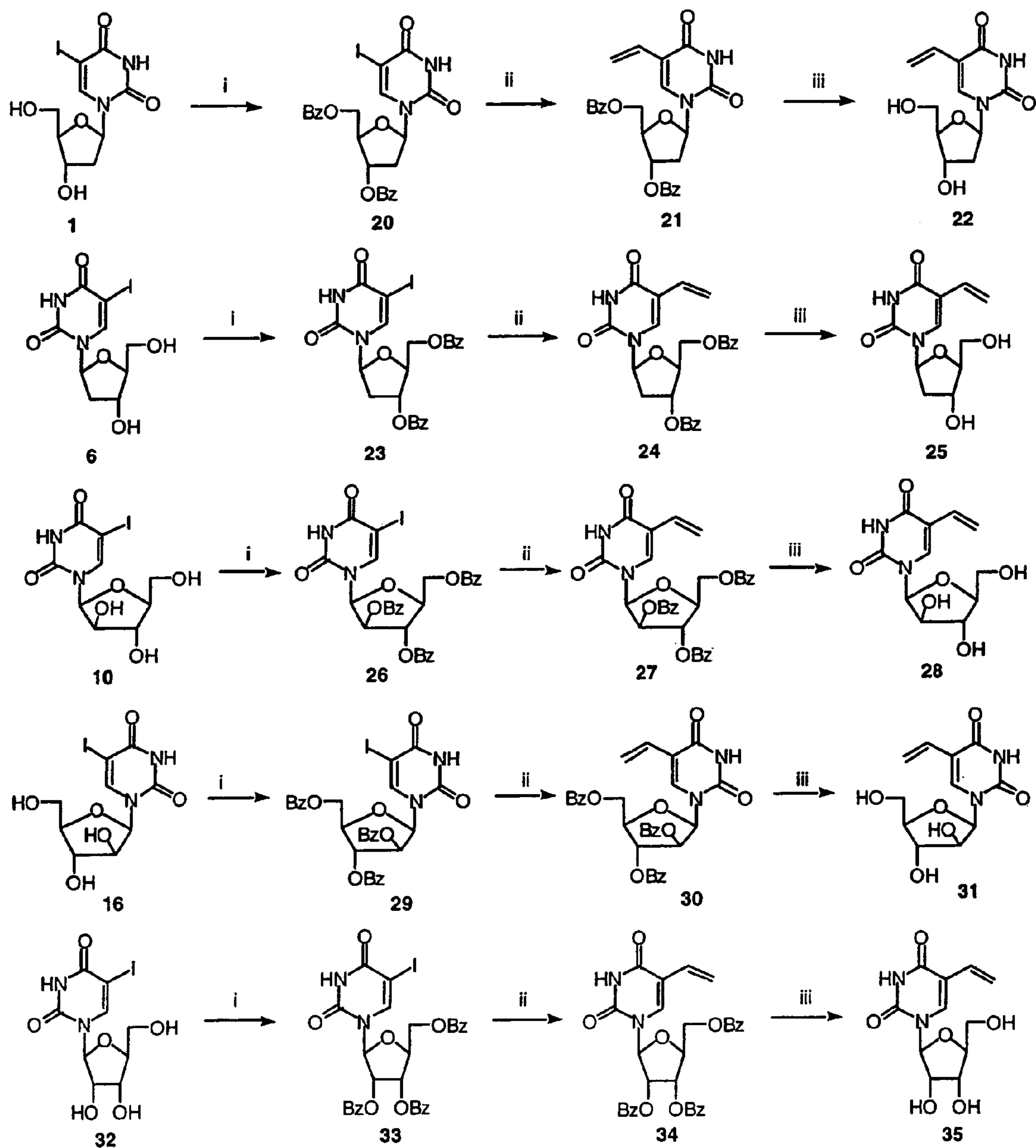
FIGURE 2. SYNTHESIS OF 5-VINYLRACIL NUCLEOSIDES
