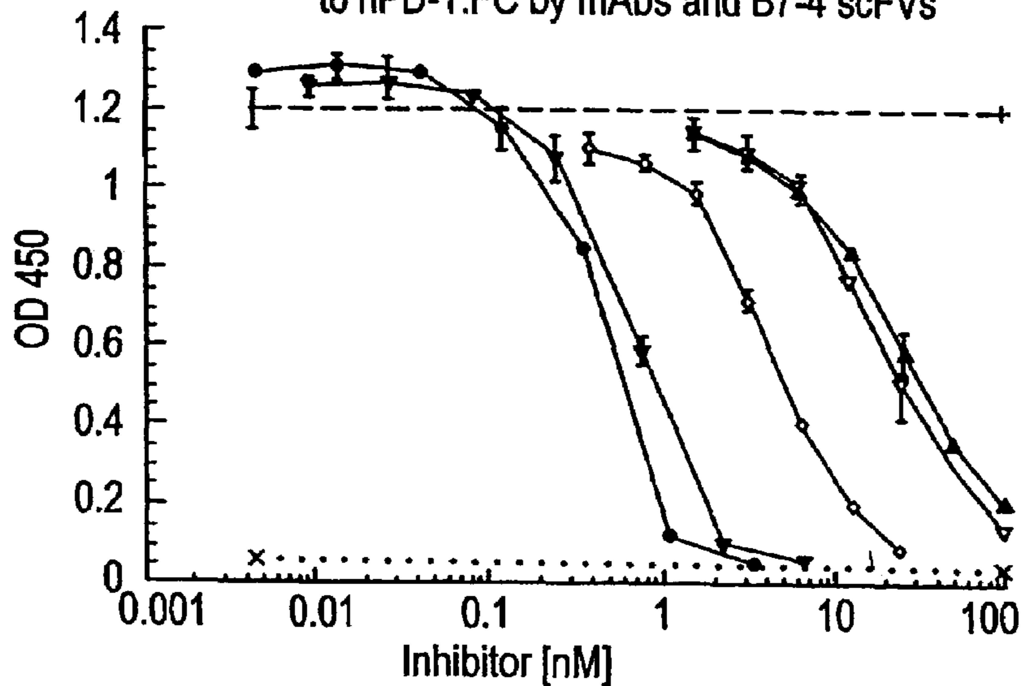
KM89 Binding curve of bio hB7-4.FC binding to hPD-1.FC by mAbs and B7-4 scFVs
